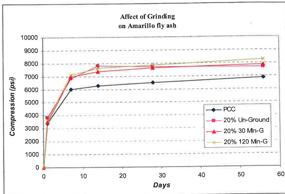
Figure 5.26 Effect of grinding duration on 20% Amarillo fly ash concrete
