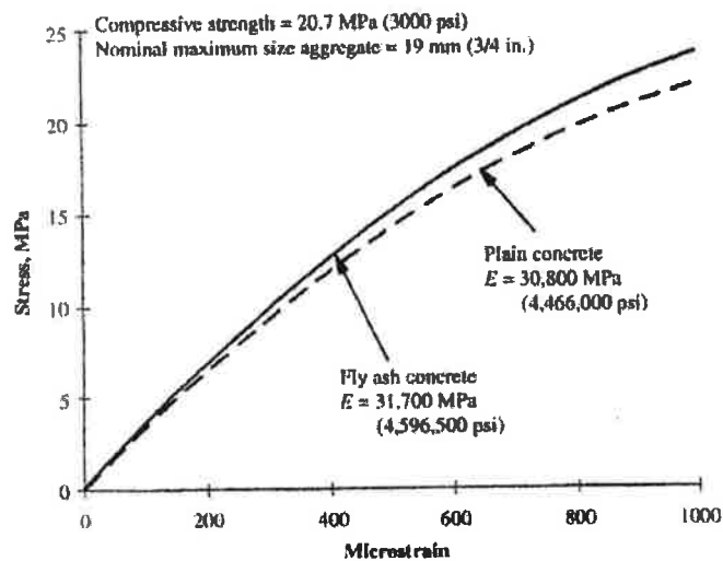
Figure 2.4 Stress-strain relationship at 90 days (Tennessee Valley Authority 1981).
