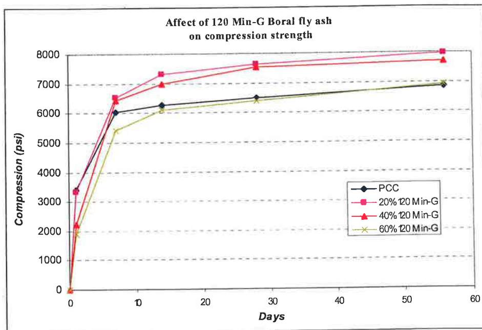
Figure 5.43 Effect of fly ash content on 120 minutes ground Boral fly ash concrete
