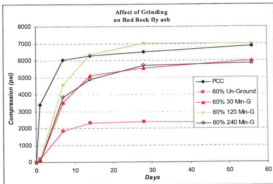
Figure 5.16 Effect of grinding duration on 60% Red Rock fly ash concrete
