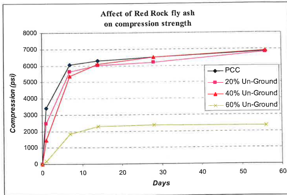
Figure 5.8 Effect of un-ground Red Rock fly ash on the compression strength of the concrete.
