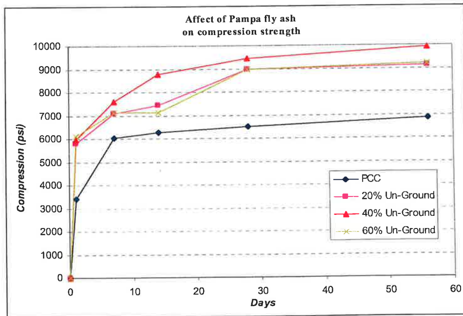
Figure 5.13 Effect of un-ground Pampa fly ash on the compression strength of the concrete.
