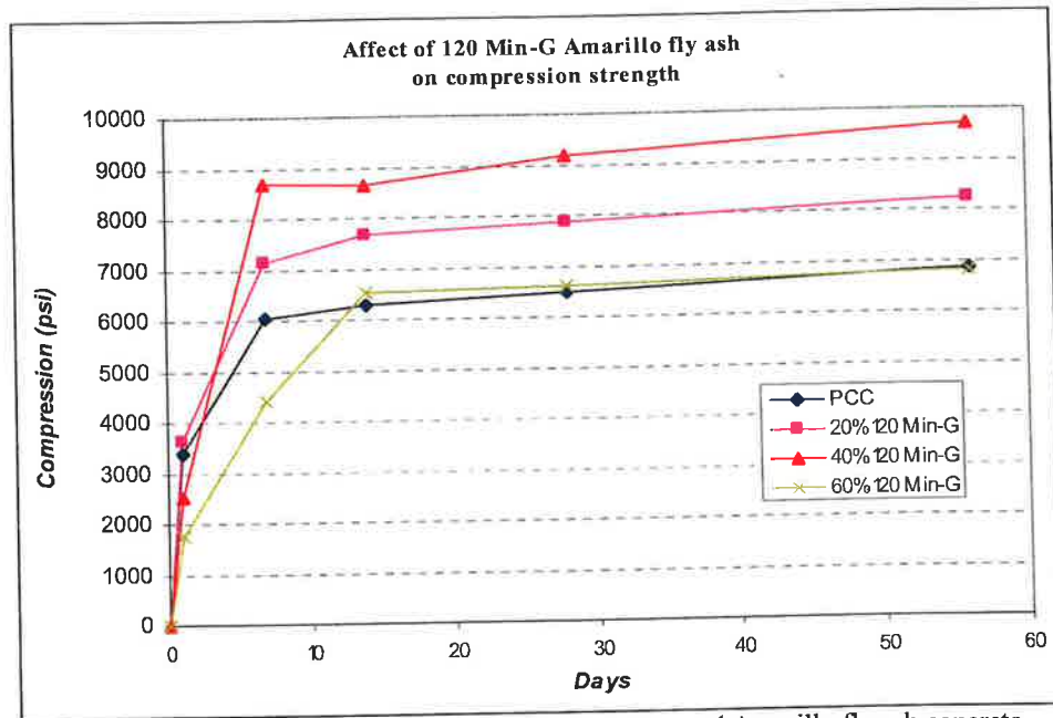
Figure 5.46 Effect of fly ash content on 120 minutes ground Amarillo fly ash concrete
