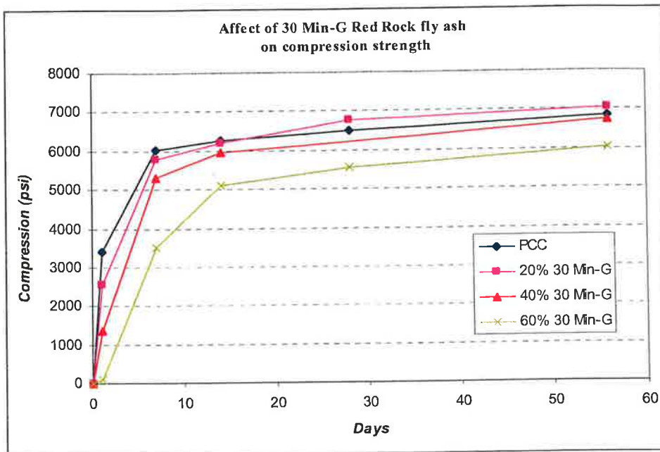
Figure 5.33 Effect of fly ash content on 30 minutes Red Rock fly ash concrete
