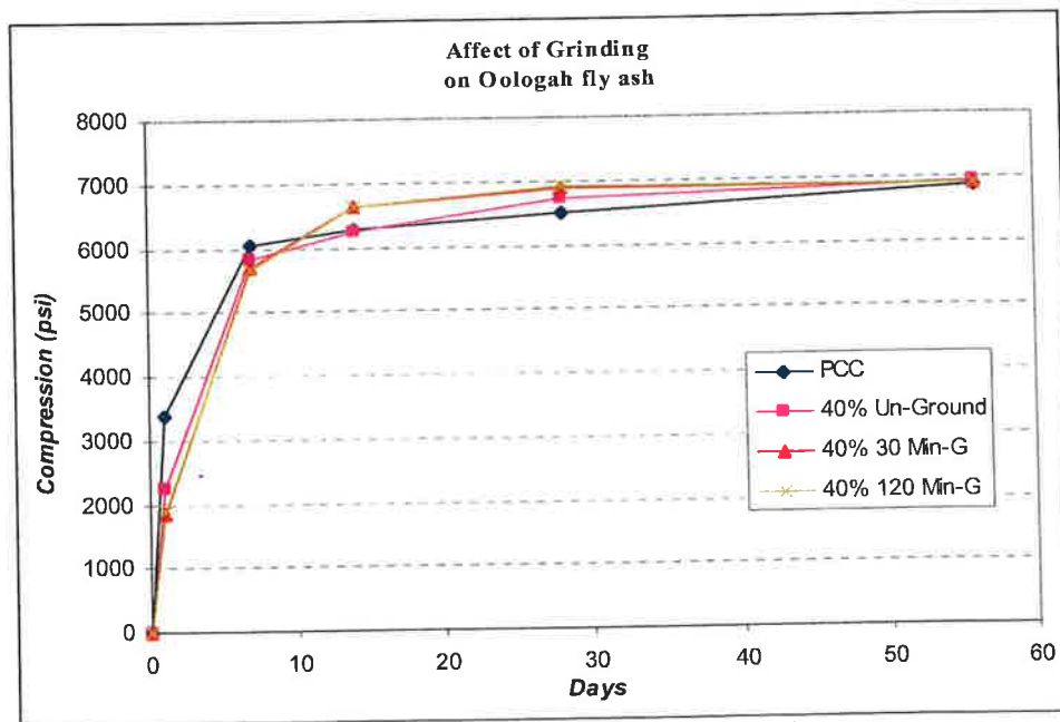
Figure 5.18 Effect of grinding duration on 40% Oologah fly ash concrete
