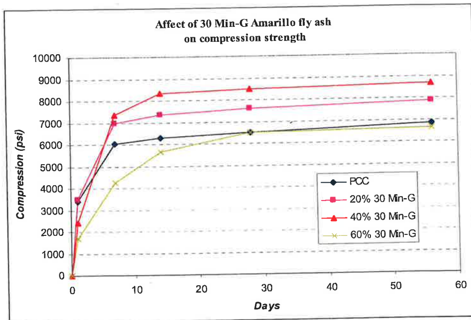
Figure 5.45 Effect of fly ash content on 30 minutes ground Amarillo fly ash concrete
