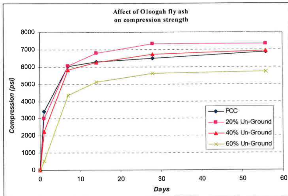
Figure 5.9 Effect of un-ground Oologah fly ash on the compression strength of the concrete.
