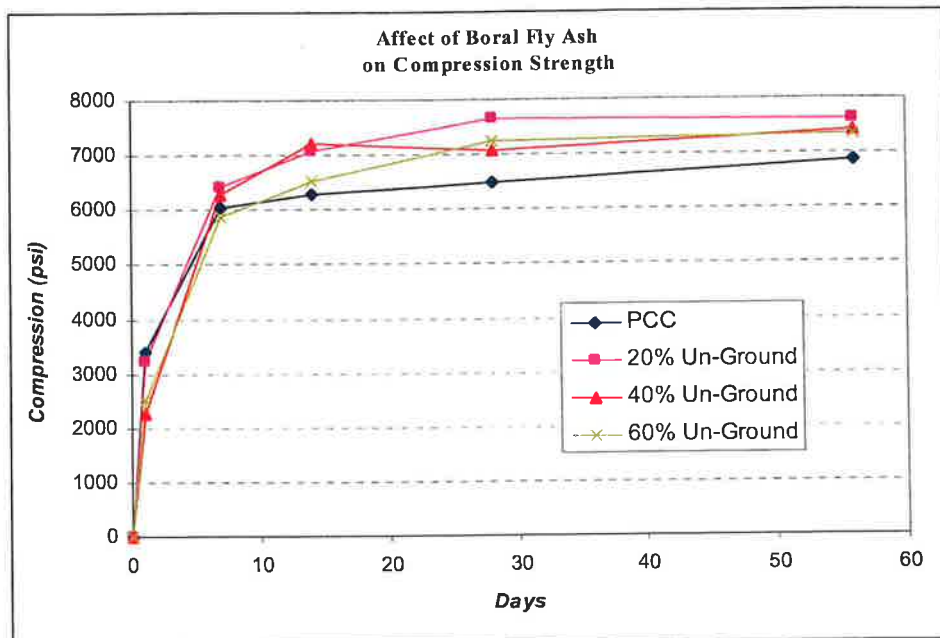
Figure 5.11 Effect of un-ground Boral fly ash on the compression strength of the concrete.
