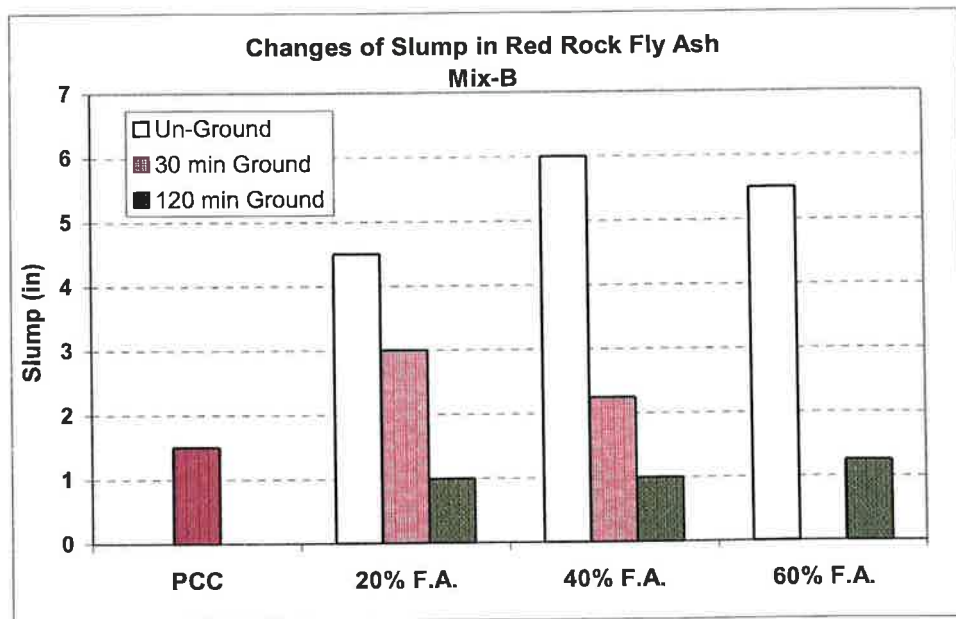
Figure 5.6 Changes of slump in Red Rock fly ash concrete due to changes of fly ash portion and grinding duration (Mix-B).
