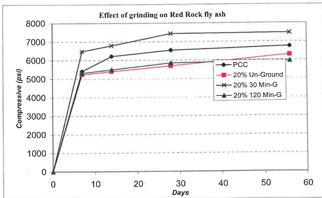
Figure 5.56 Effect of grinding duration on 20% Red Rock fly ash concrete (Mix-C).
