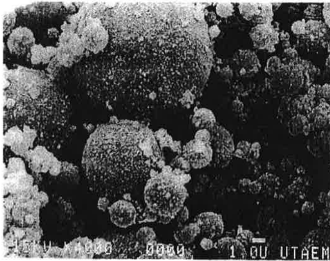
Figure 2.2 Fly ash at 4000× magnification.
