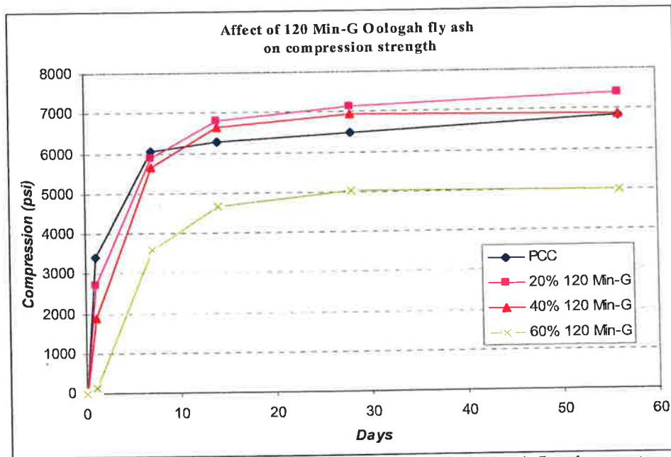
Figure 5.37 Effect of fly ash content on 120 minutes ground Oologah fly ash concrete
