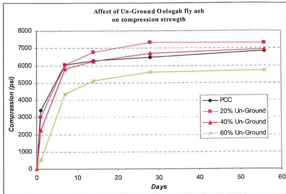
Figure 5.35 Effect of fly ash content on un-ground Oologah fly ash concrete
