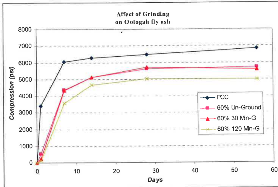
Figure 5.19 Effect of grinding duration on 60% Oologah fly ash concrete
