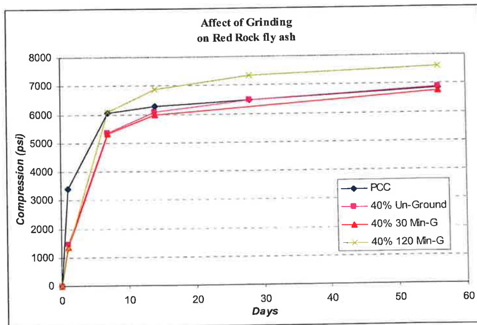
Figure 5.15 Effect of grinding duration on 40% Red Rock fly ash concrete
