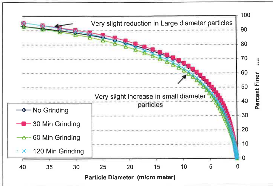
Figure 3.2 Changes of fly ash size distribution due to grinding.
