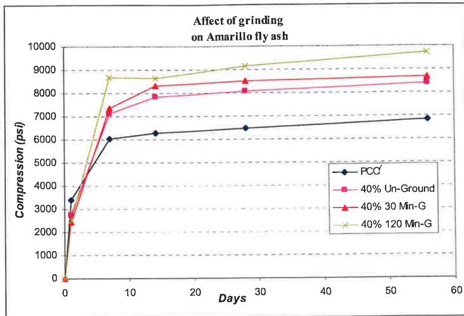
Figure 5.27 Effect of grinding duration on 40% Amarillo fly ash concrete
