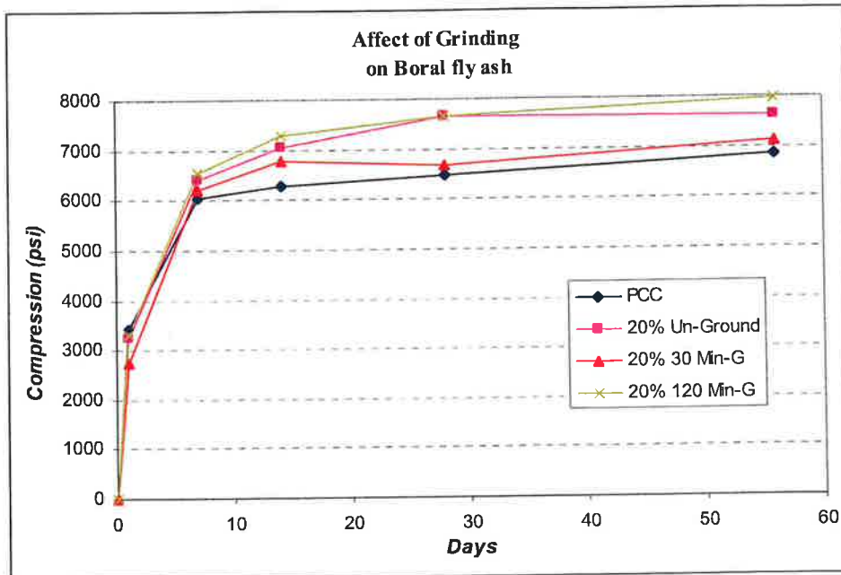
Figure 5.23 Effect of grinding duration on 20% Borol fly ash concrete
