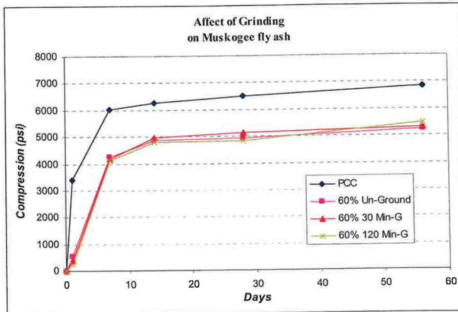
Figure 5.22 Effect of grinding duration on 60% Muskogee fly ash concrete
