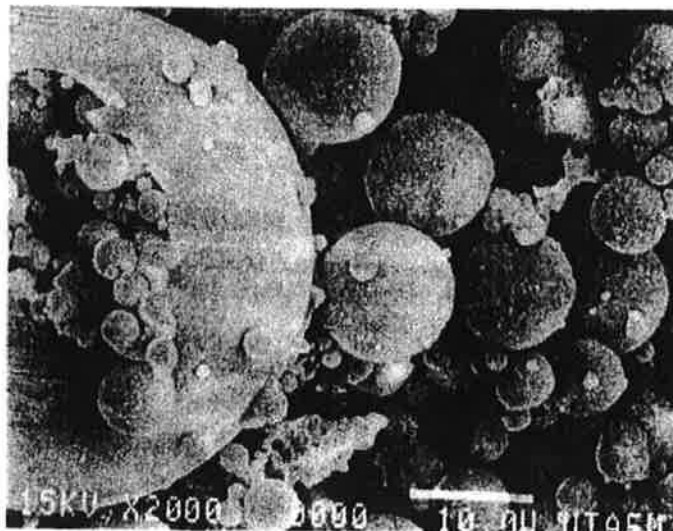
Figure 2.3 Fly ash showing plerospheres at 2000× magnification.
