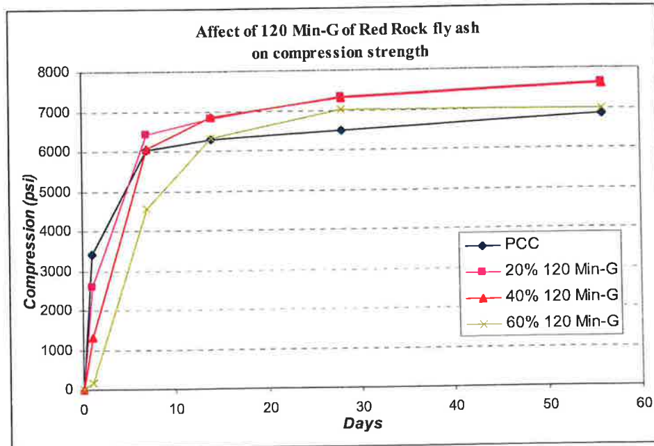
Figure 5.34 Effect of fly ash content on 120 minutes Red Rock fly ash concrete
