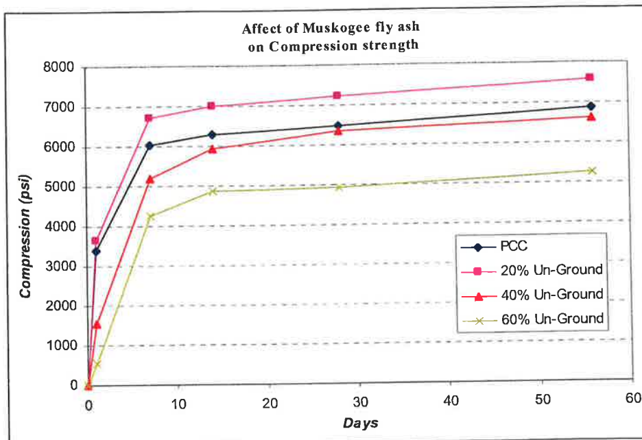
Figure 5.10 Effect of un-ground Muskogee fly ash on the compression strength of the concrete.
