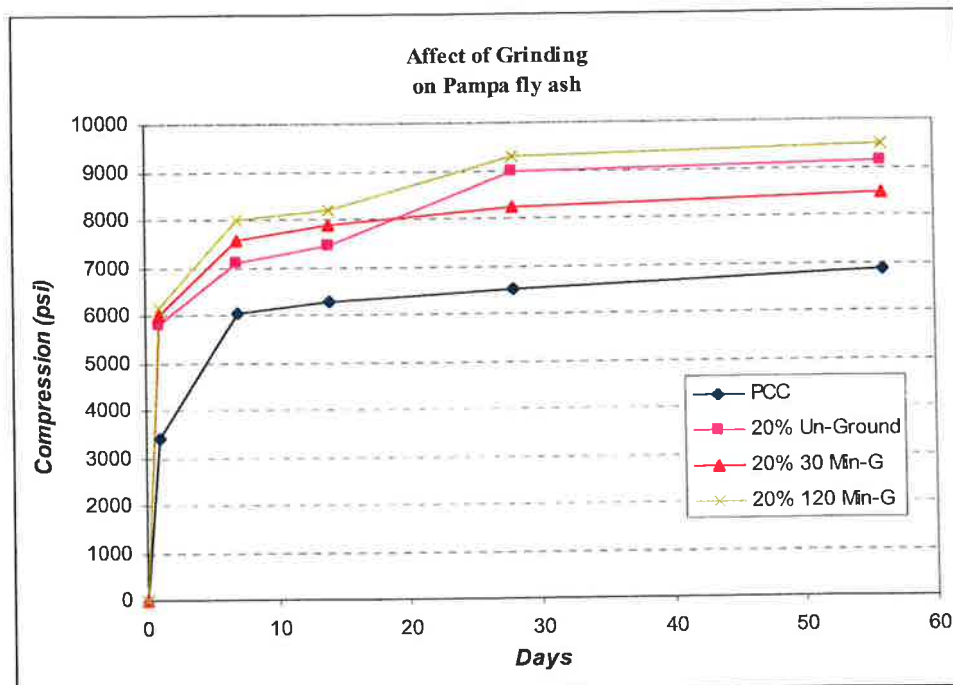
Figure 5.29 Effect of grinding duration on 20% Pampa fly ash concrete
