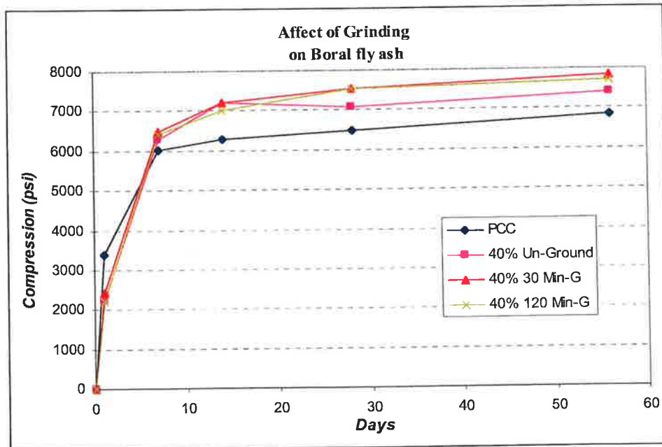
Figure 5.24 Effect of grinding duration on 40% Borol fly ash concrete
