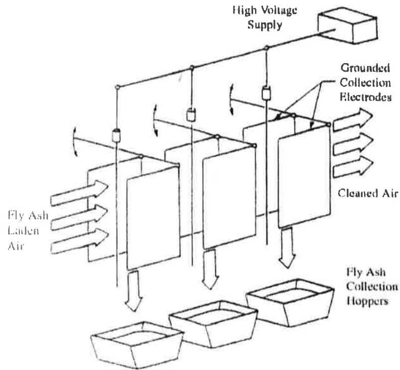
Figure 2.1 Electrostatic precipitator
