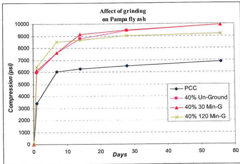
Figure 5. 30 Effect of grinding duration on 40% Pampa fly ash concrete
