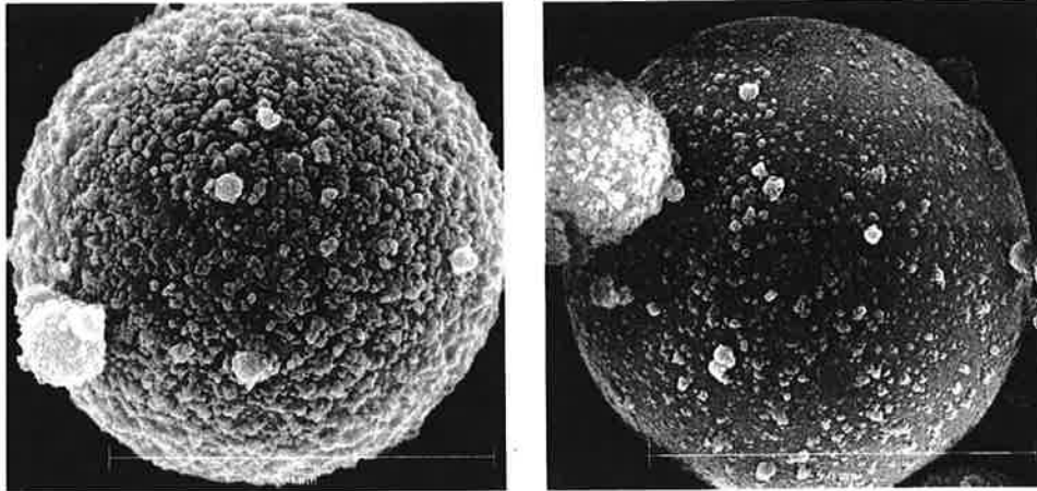
Figure 3.1 Fly ash particles before and after grinding
