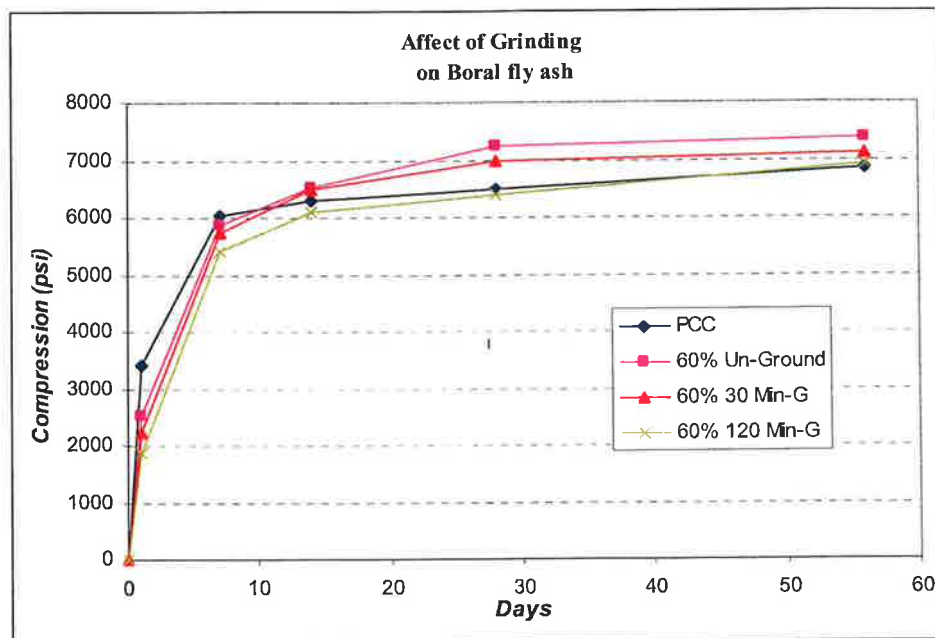
Figure 5.25 Effect of grinding duration on 60% Boral fly ash concrete
