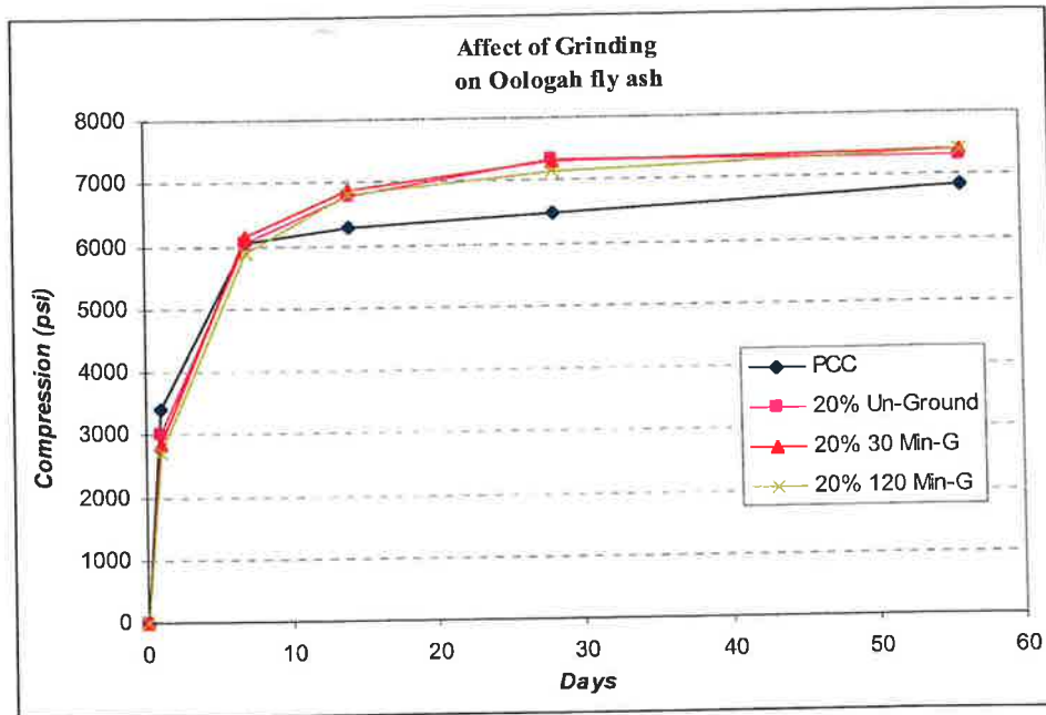
Figure 5.17 Effect of grinding duration on 20% Oologah fly ash concrete
