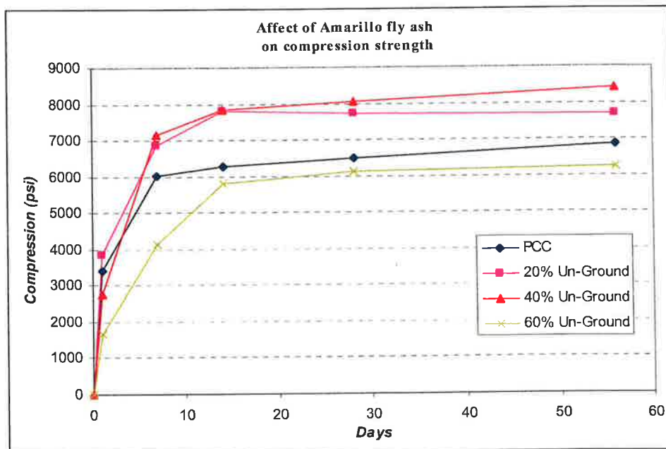
Figure 5. 12 Effect of un-ground Amarillo fly ash on the compression strength of the concrete.
