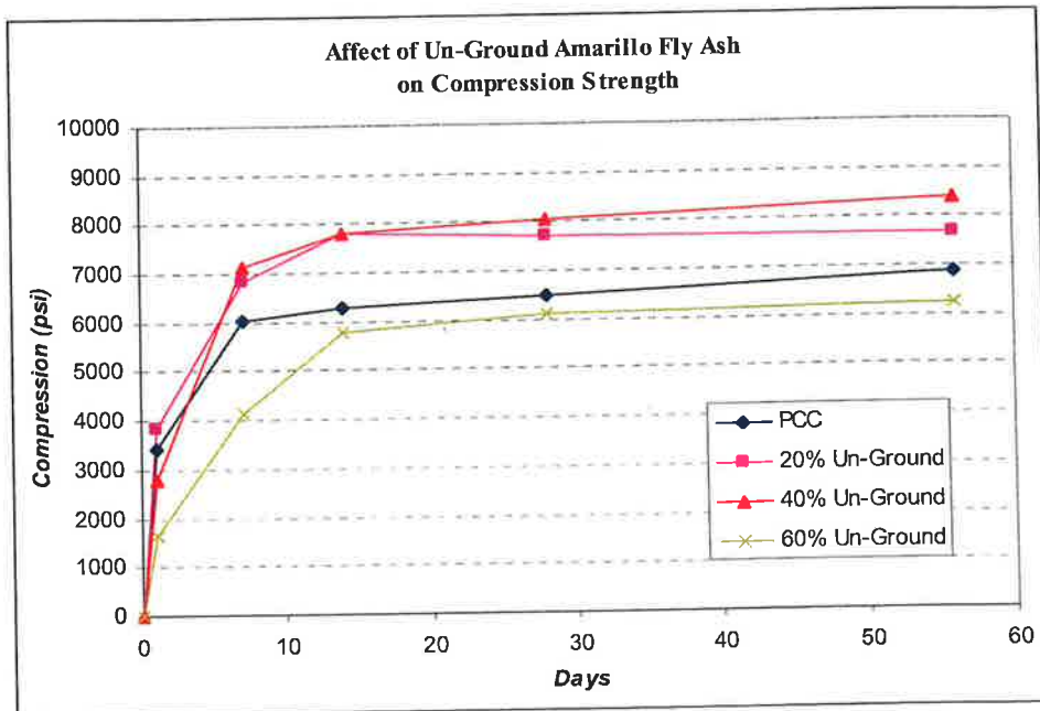
Figure 5.44 Effect of fly ash content on un-ground Amarillo fly ash concrete
