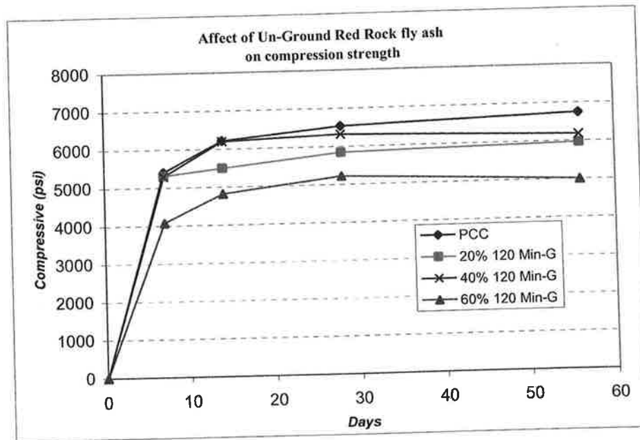
Figure 5.61 Effect of fly ash content on 120 minutes Red Rock fly ash concrete (Mix-C)
