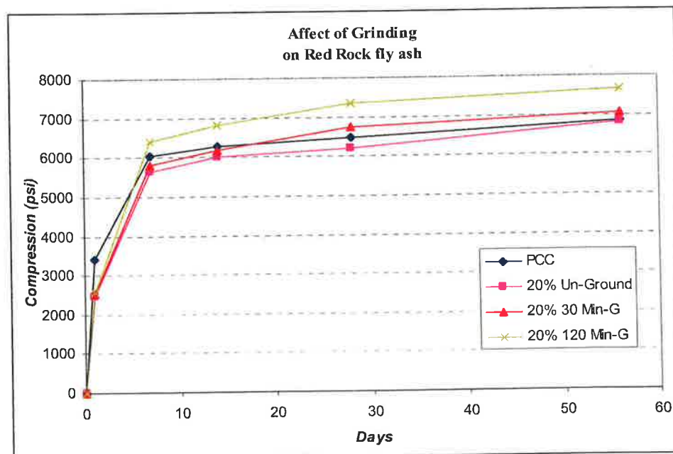
Figure 5.14 Effect of grinding duration on 20% Red Rock fly ash concrete
