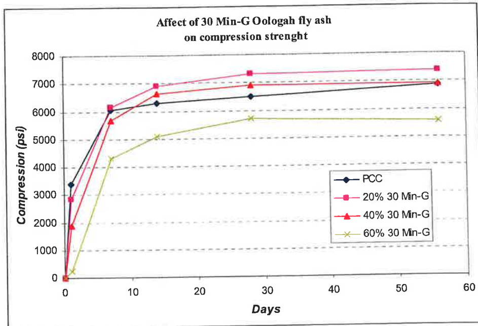
Figure 5.36 Effect of fly ash content on 30 minutes ground Oologah fly ash concrete
