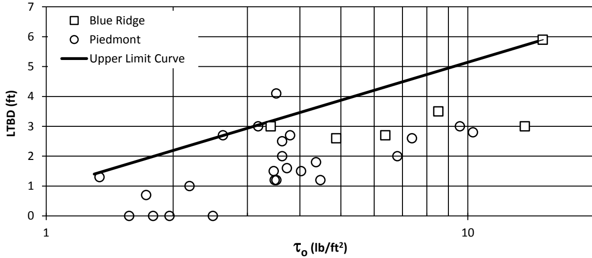
Figure 4.4. Conservative upper limit of LTBD as a function of \tau_o .
