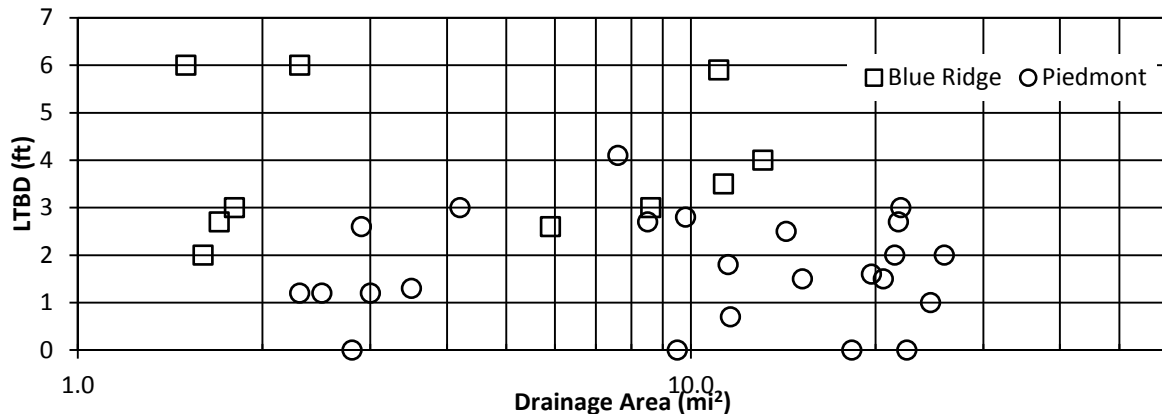
Figure 4.1. Variation of LTBD with drainage area for each physiographic province.
