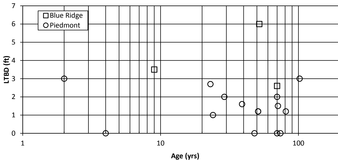
Figure 4.7. Variation of LTBD with structure’s age.
