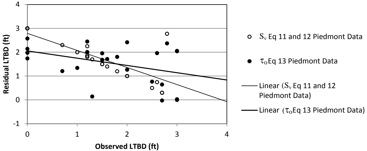
Figure 4.8. Comparison of residual LTBD values and observed LTBD for the Piedmont data.
