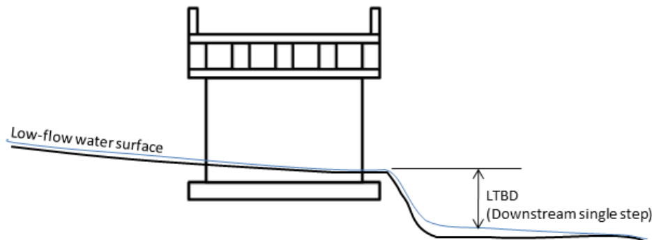
Figure 3.4. LTBD: uniform degradation and single step downstream.
