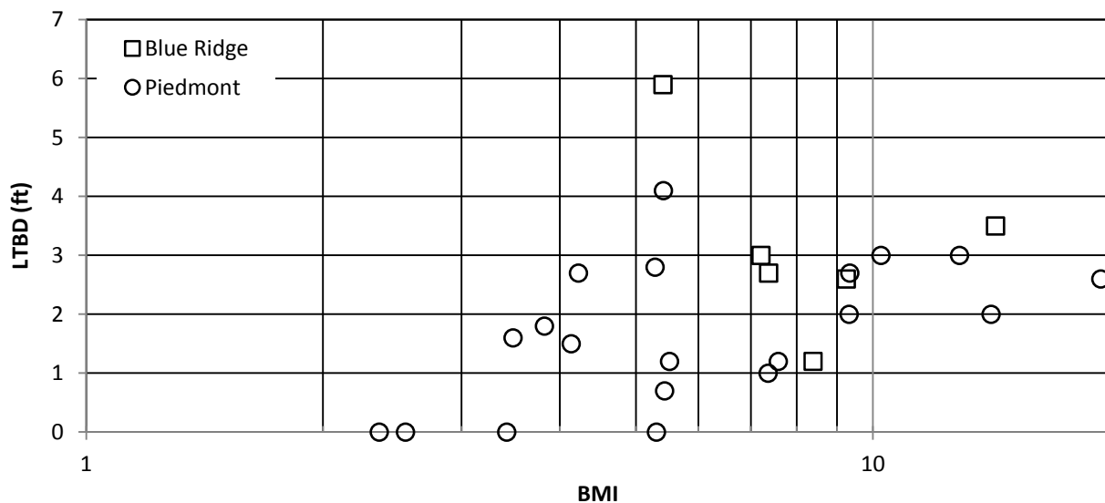
Figure 4.5. LTBD as a function of the bed mobility index.
