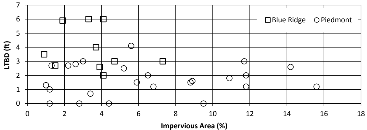
Figure 4.2. LTBD as a function of impervious area.
