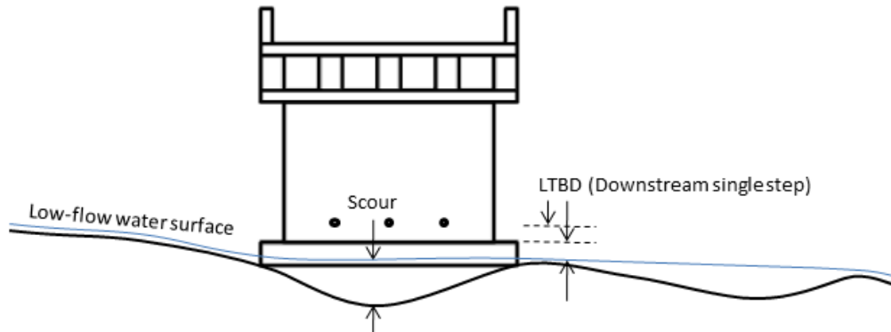
Figure 3.6. LTBD with scour: single step downstream.
