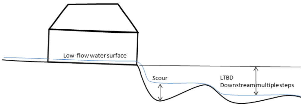
Figure 3.3. Typical bed profile of a culvert with downstream bed degradation and a scour pool.
