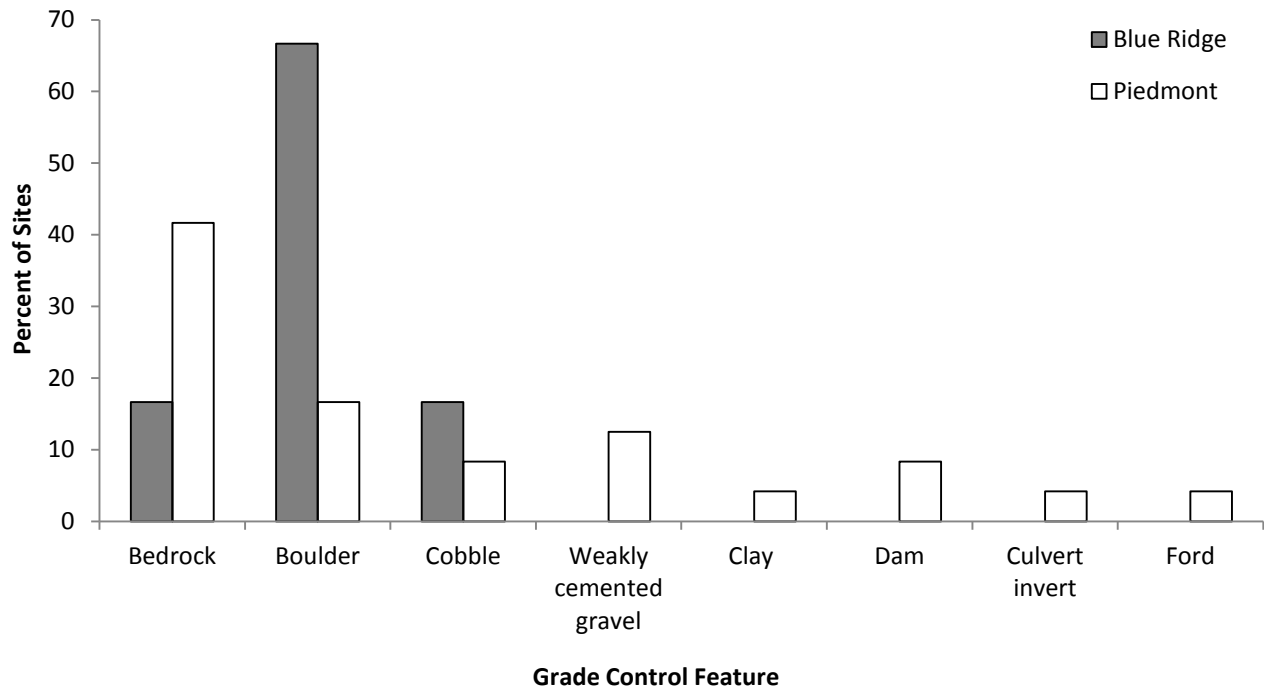
Figure 4.6. Grade control features identified in Blue Ridge and western Piedmont streams.
