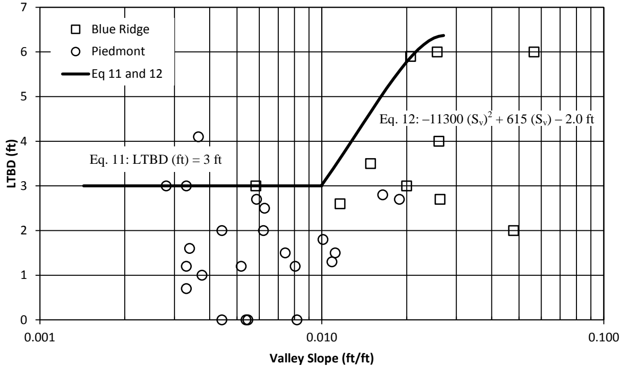
Figure 4.3. LTBD as a function of valley slope.
