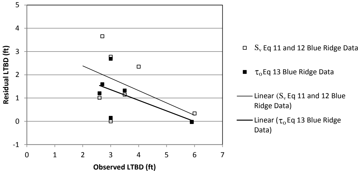
Figure 4.9. Comparison of predicted LTBD values and observed LTBD for the Blue Ridge data.
