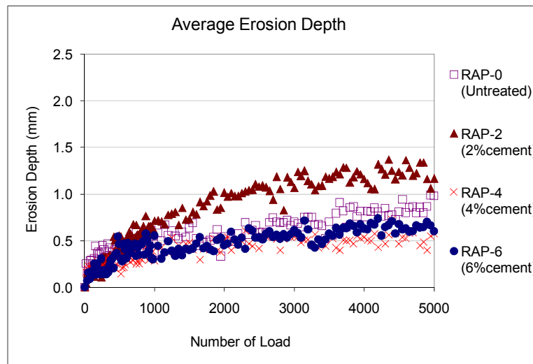
Figure 14 Mean Erosion Depth of 11 Measuring Spots versus Number of Load by HWTB Test.
