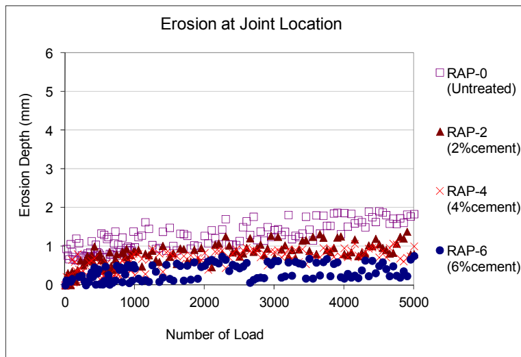
Figure 13 Maximum Erosion Depth at Joint Location versus Number of Load by HWTB Test.
