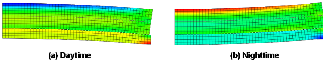
Figure 60 Stress Distributions at Daytime and Nighttime Temperature Conditions.
