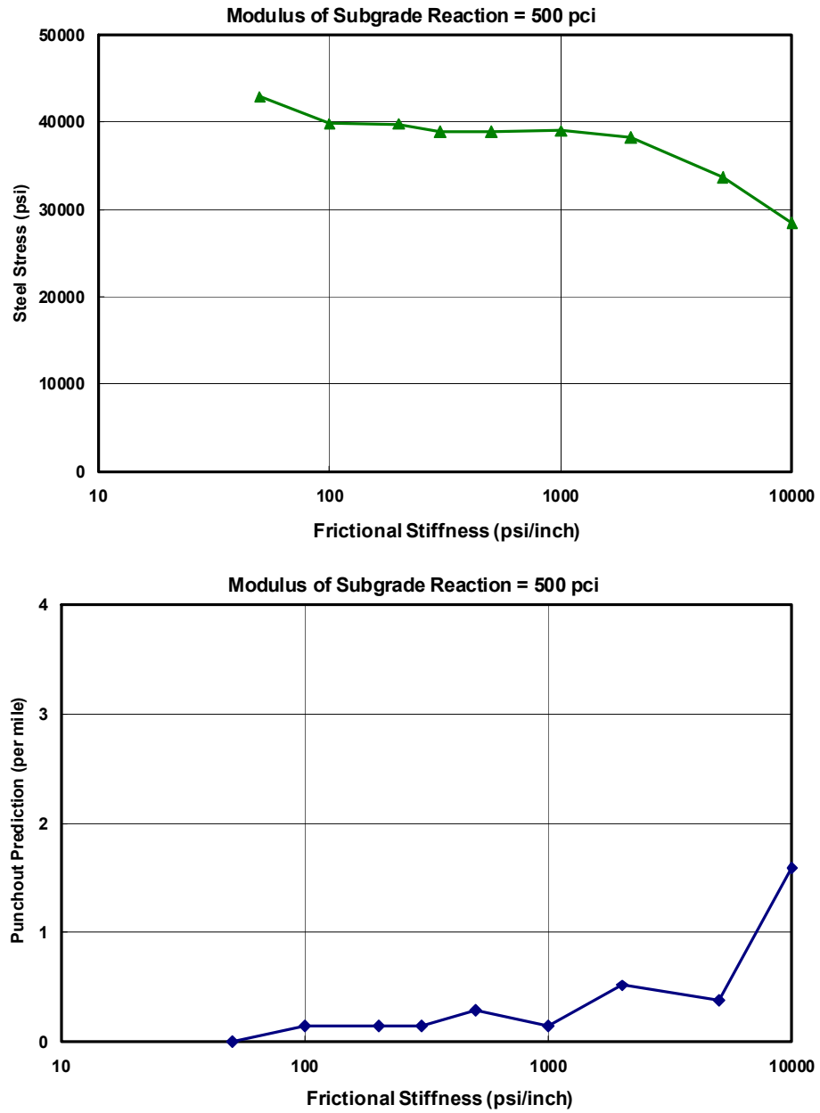
Figure 21 Analysis of Frictional Effects: Steel Stress and Punchout.
