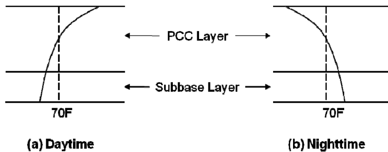
Figure 59 Temperature Gradients for Analysis Input.
