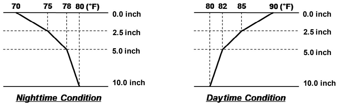
Figure 29 Temperature Loading Conditions.
