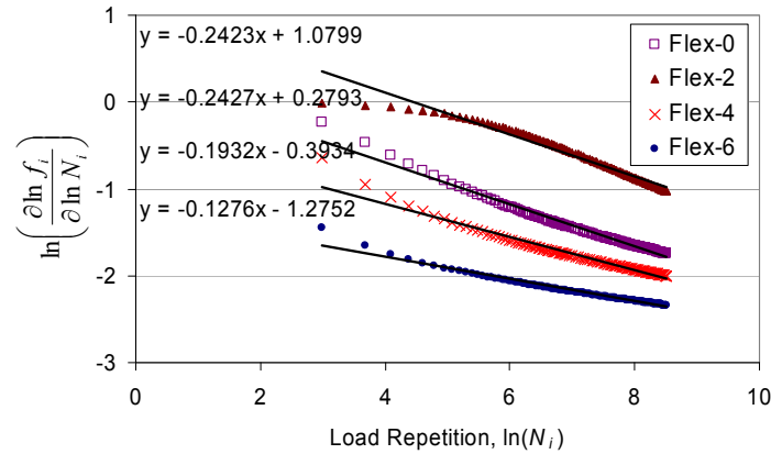
Figure 16 Log Plot to Acquire a and \rho from HWTB Test.
