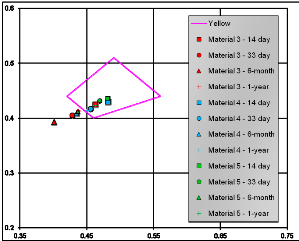
Figure 21. Average Daytime Color (D65) with 2° Standard Observer Test Deck 5.
