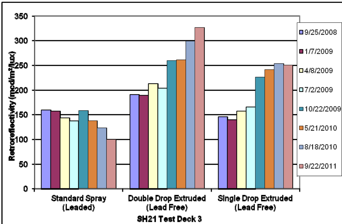
Figure 13. Average Retroreflectivity Test Deck 3.
