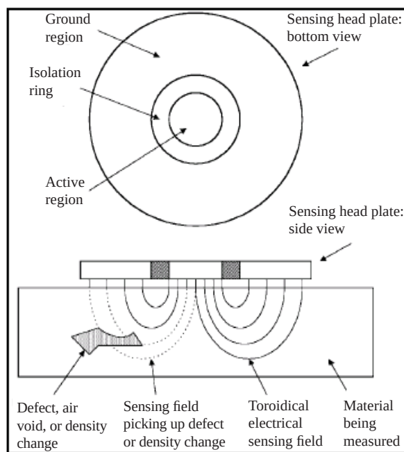
Operational theory schematic of PQI 301
