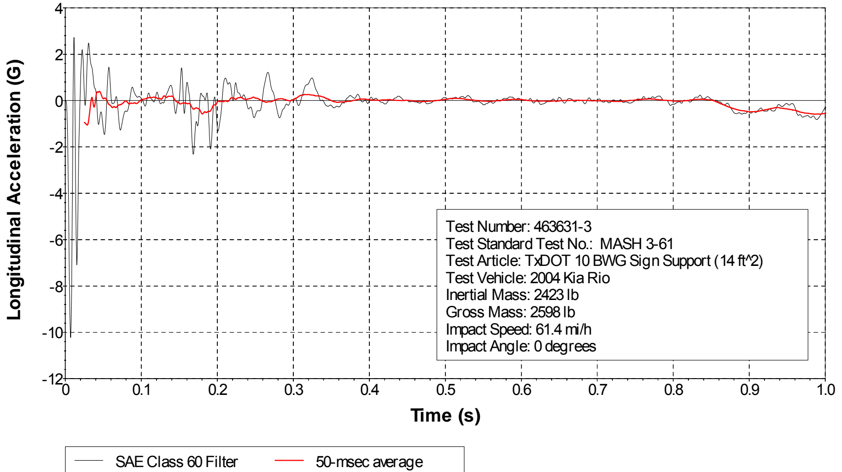
Figure J7. Vehicle Longitudinal Accelerometer Trace for Test No. 463631-3 (Accelerometer Located over Rear Axle).
