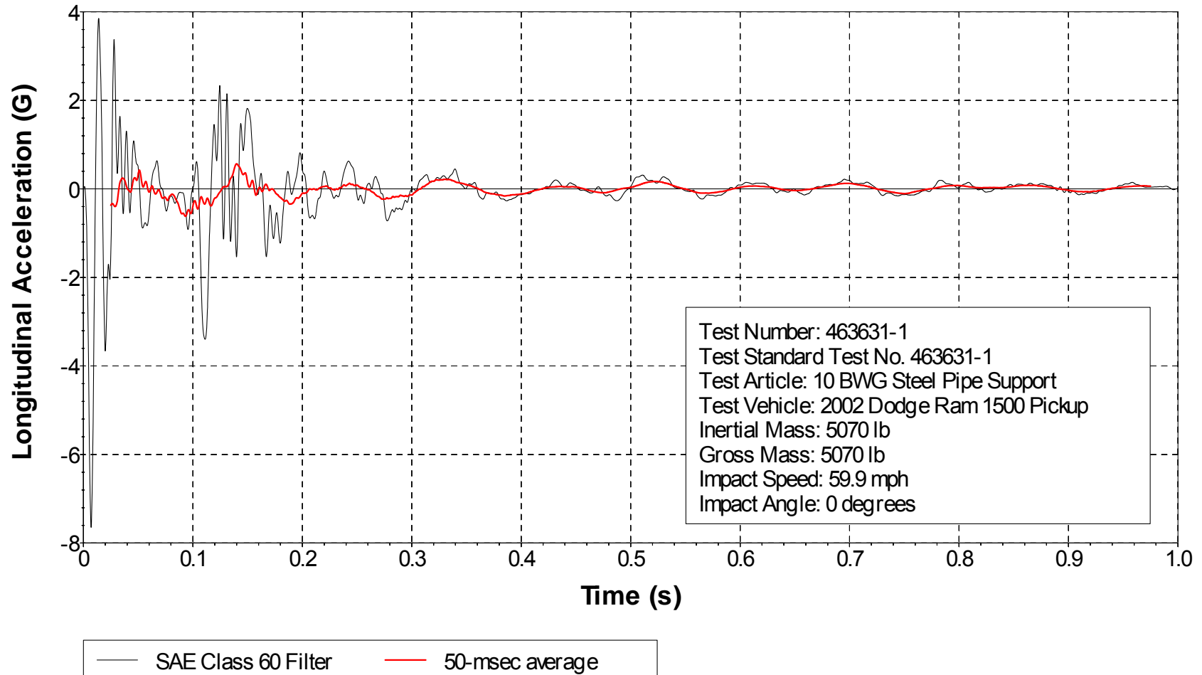
Figure H4. Vehicle Longitudinal Accelerometer Trace for Test No. 463631-1 (Accelerometer Located at Center of Gravity).
