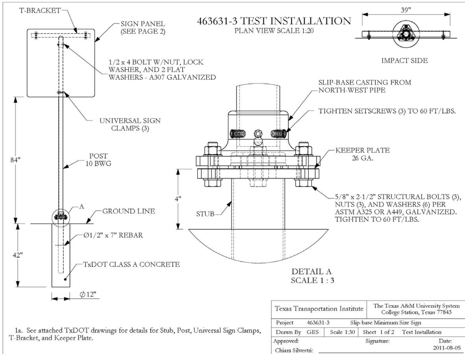
Figure 9.50. Details of the Sign Support System Used for Test No. 463631-3.
