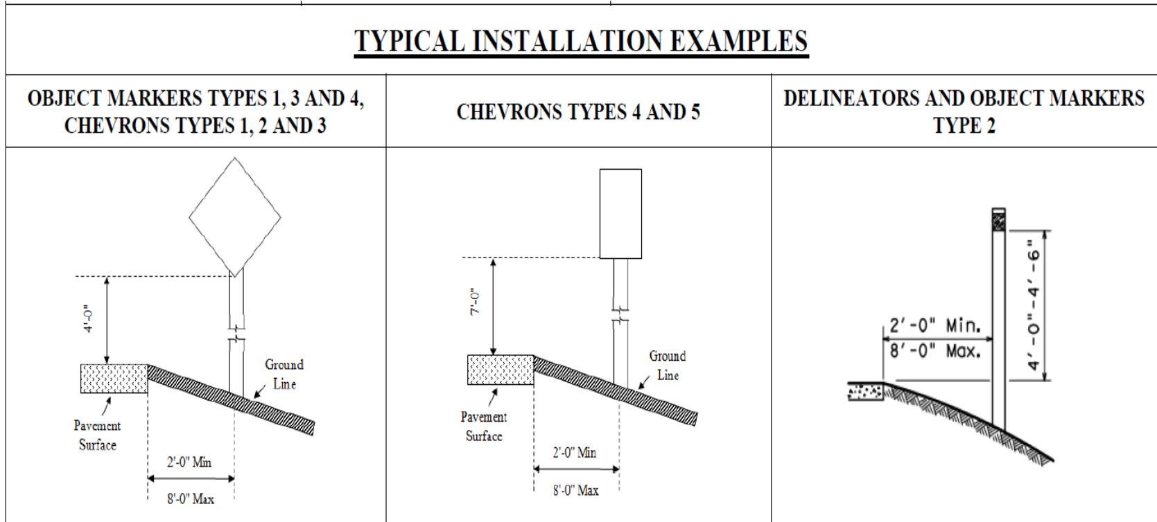
Figure 10.15. “Typical Installation Examples” Section in the Proposed New Layout TxDOT D&OM(1)-11, Options #1 and #2.
