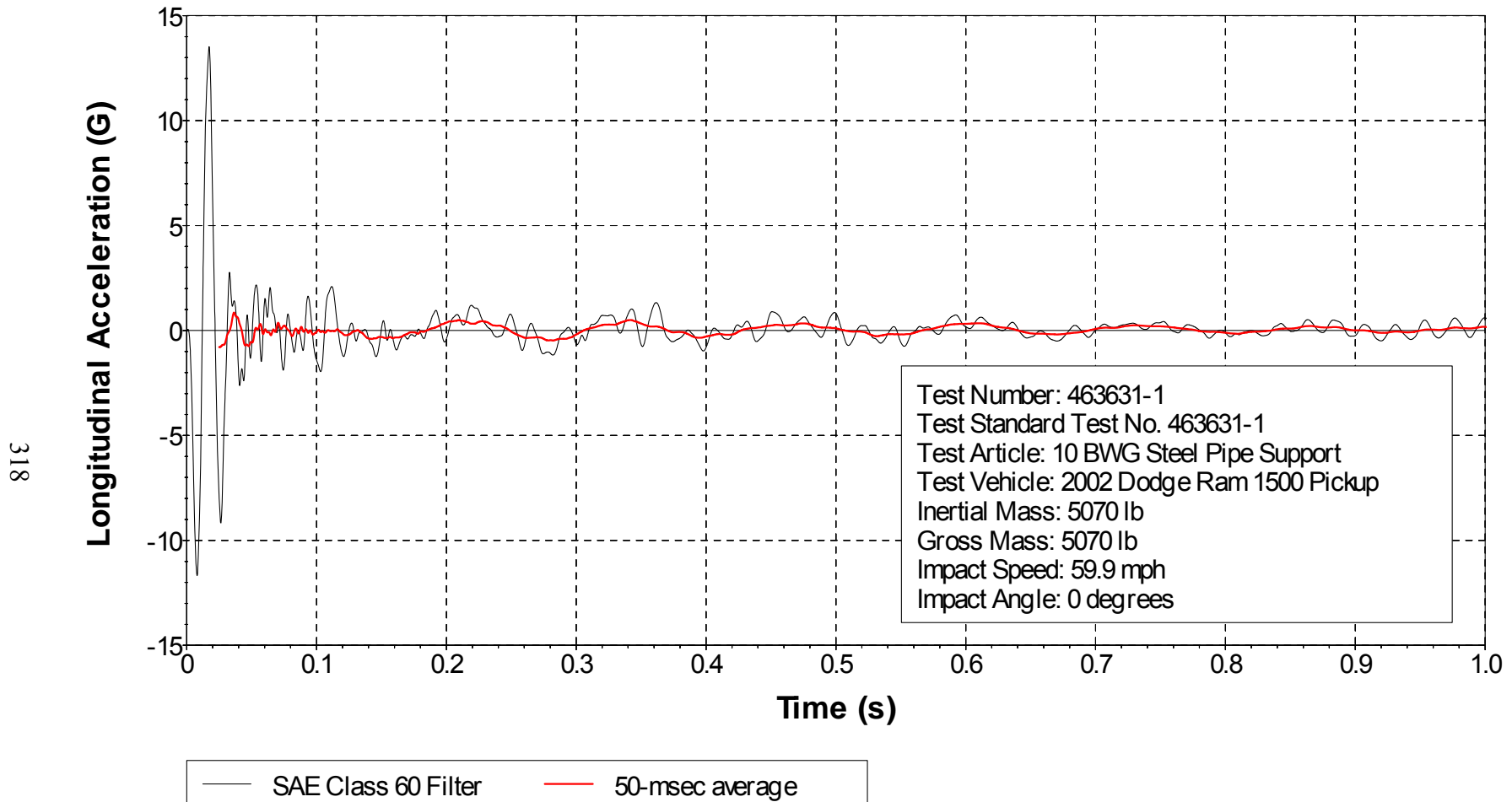
Figure H7. Vehicle Longitudinal Accelerometer Trace for Test No. 463631-1 (Accelerometer Located over Rear Axle).
