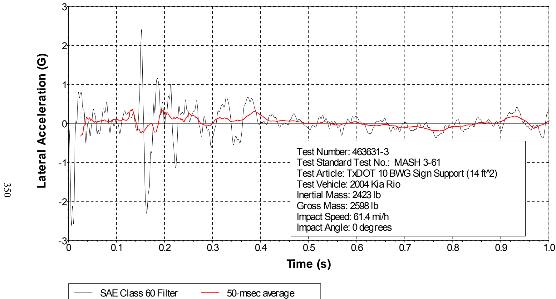
Figure J8. Vehicle Lateral Accelerometer Trace for Test No. 463631-3 (Accelerometer Located over Rear Axle).
