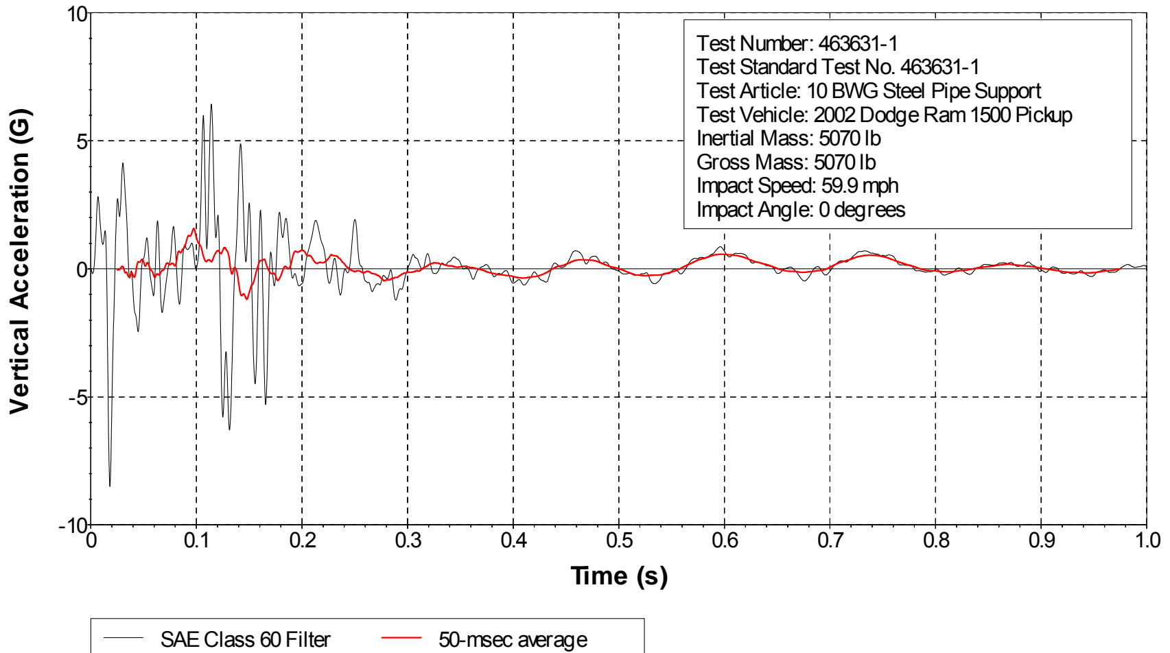
Figure H6. Vehicle Vertical Accelerometer Trace for Test No. 463631-1 (Accelerometer Located at Center of Gravity).
