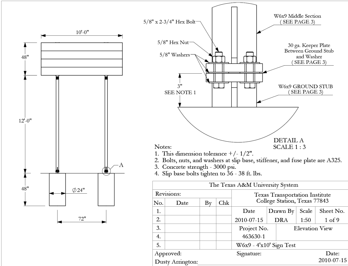
Figure 7.15. Details of the TxDOT W6x9 – 4-ft x 10-ft Large Sign Support Test Installation.
