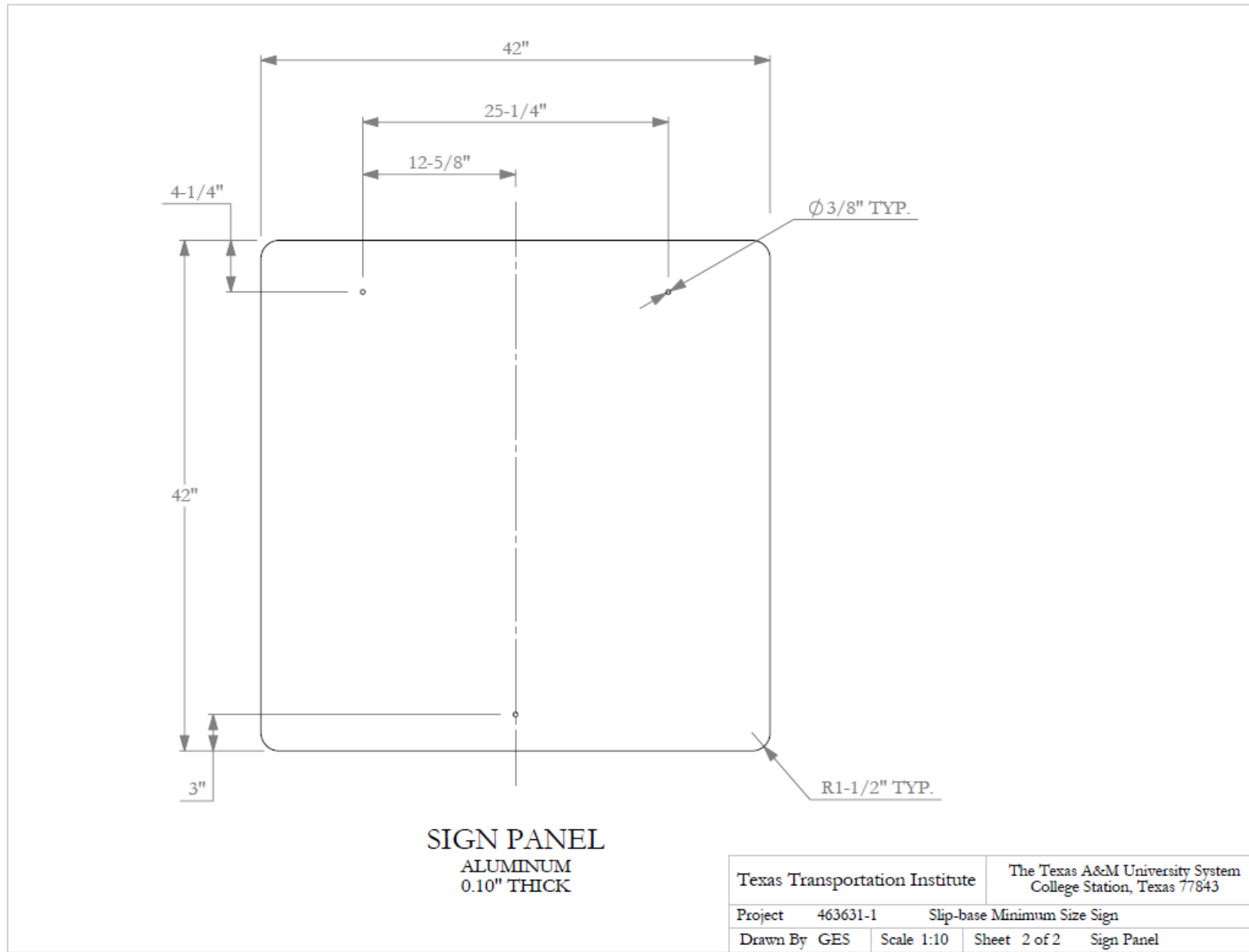
Figure 9.28. Details of the Sign Panel Used in Test Nos. 463631-1 and 463631-2.
