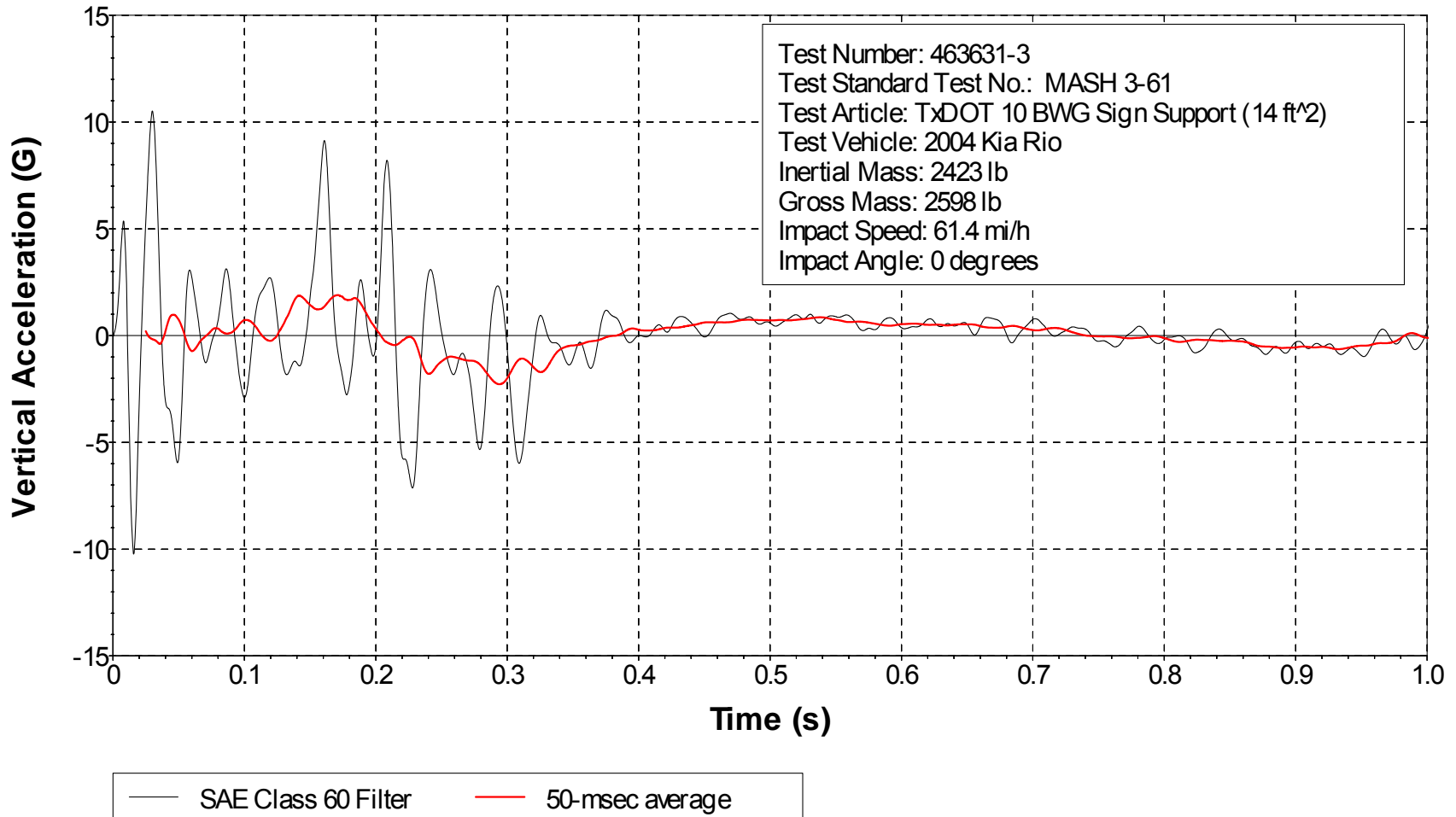
Figure J9. Vehicle Vertical Accelerometer Trace for Test No. 463631-3 (Accelerometer Located over Rear Axle).
