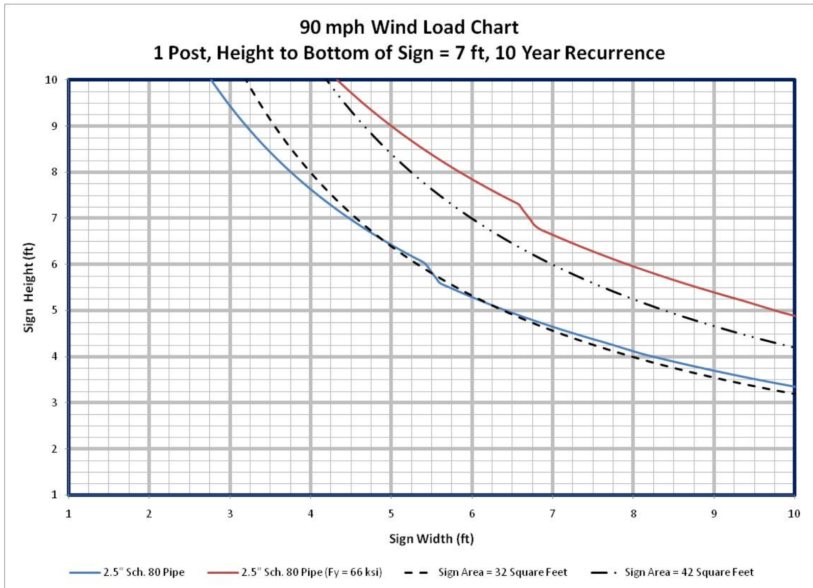
Figure 3.4. Updated Schedule 80 Wind Load Chart (Current Pressure Method).
