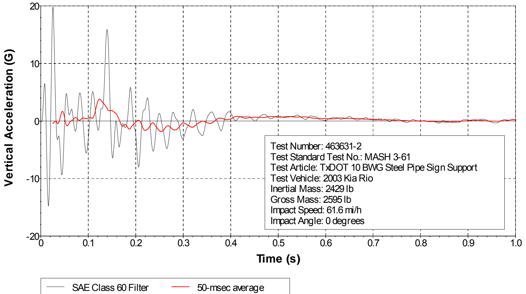
Figure I8. Vehicle Vertical Accelerometer Trace for Test No. 463631-2 (Accelerometer Located over Rear Axle).
