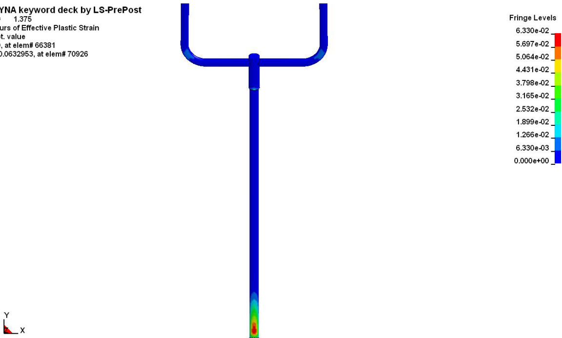
Figure 11.7. Simulation of Modified Nipple Design.
