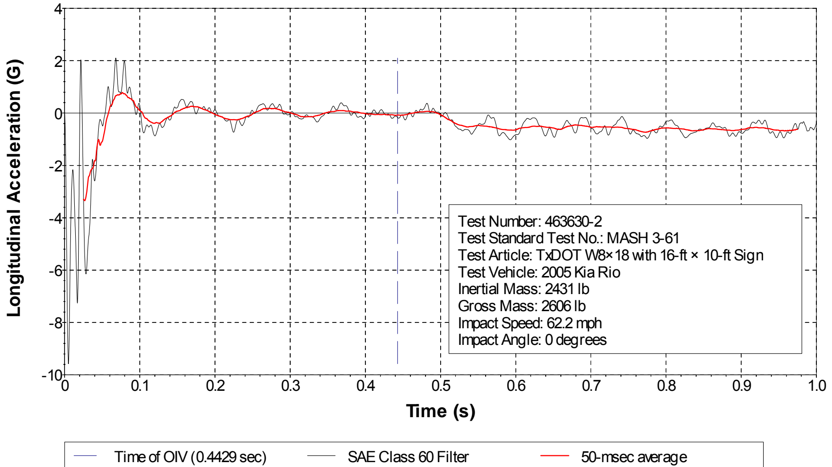
Figure F4. Vehicle Longitudinal Accelerometer Trace for Test No. 463630-2 (Accelerometer Located at Center of Gravity).
