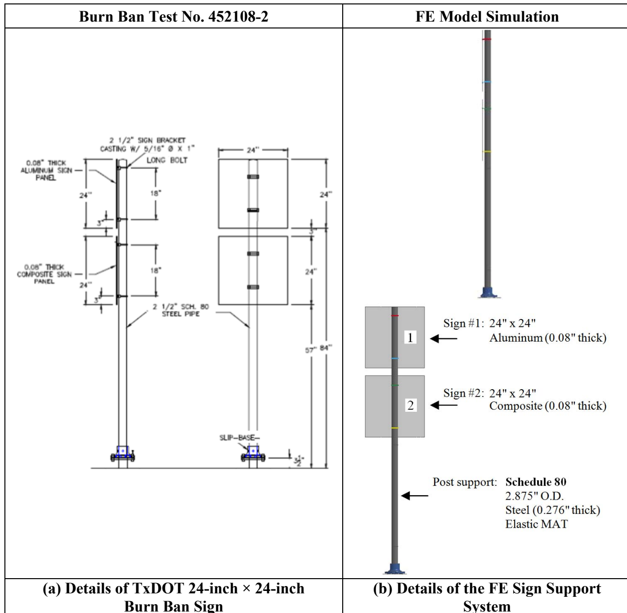
Figure 9.3. Comparison between Burn Ban Test No. 452108-2 and FE Model Sign Support Slipbase System Configurations.
