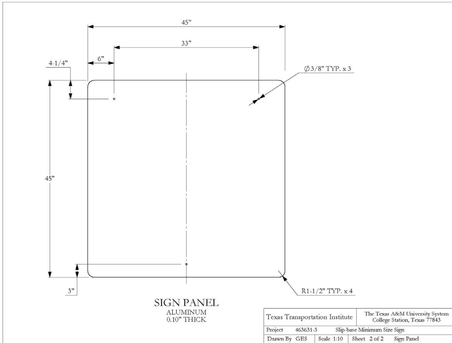
Figure 9.51. Details of the Sign Panel Used for Test No. 463631-3.
