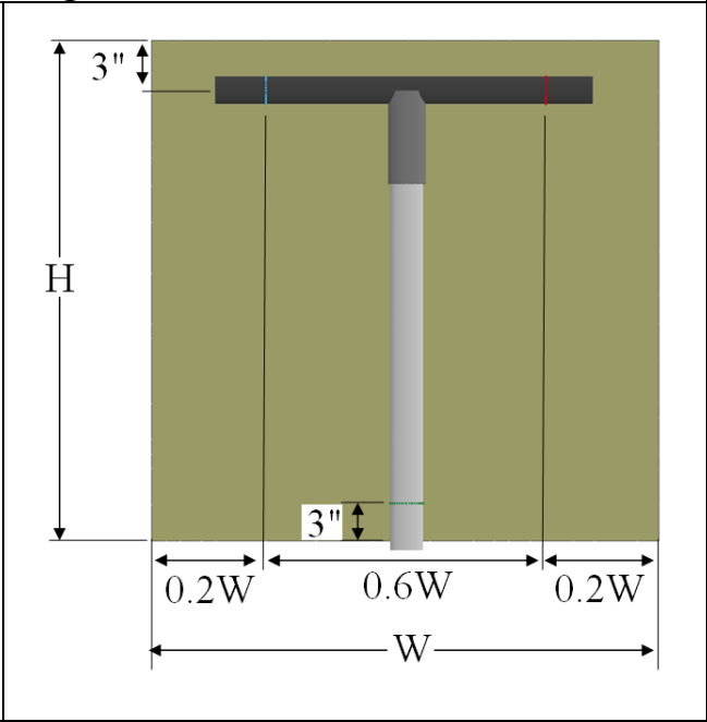
(c) Details T-Bracket Configuration #2
