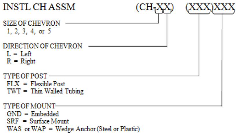
Figure 10.9. "Chevrons" Section in the Proposed New Layout TxDOT D&OM(1)-11, Option #1.
