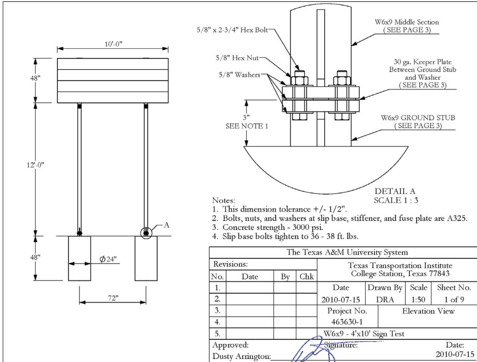
Figure E1. Details of the W6x9 with 4-ft x 10-ft Sign.
