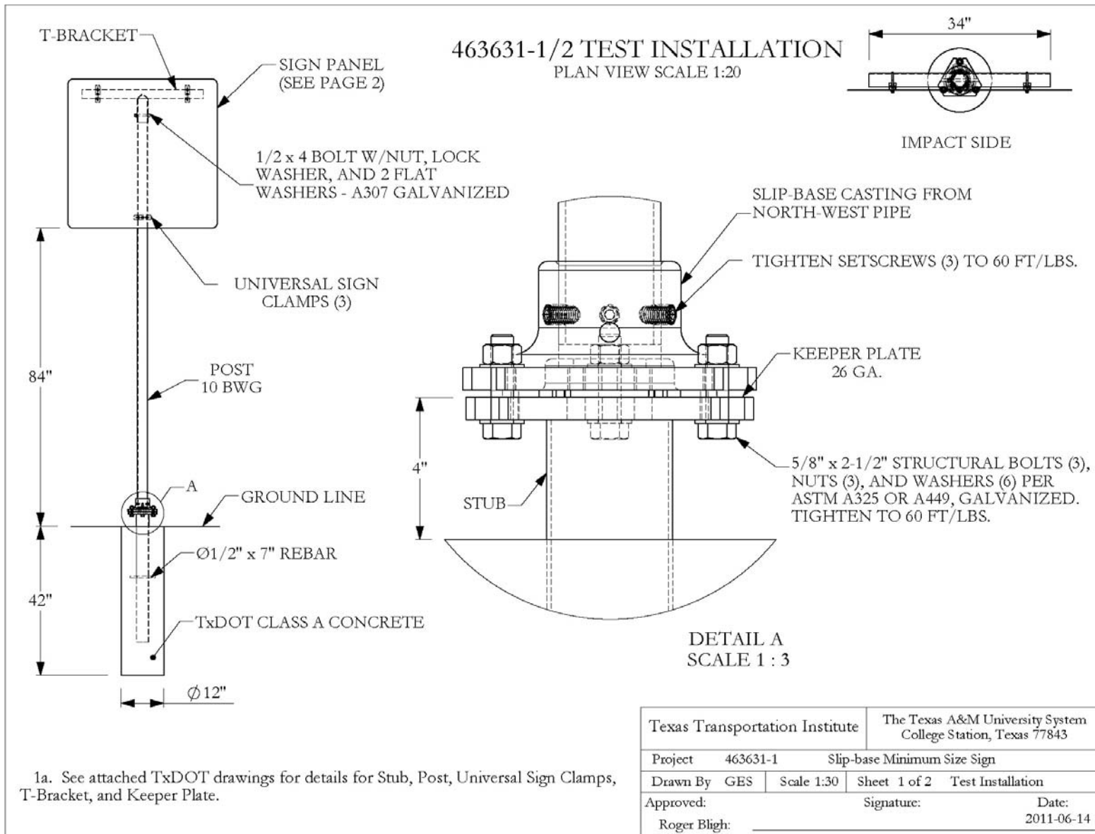
Figure H1. Details of the 10 BWG Steel Pipe Support with 12 ft 2 Sign.
