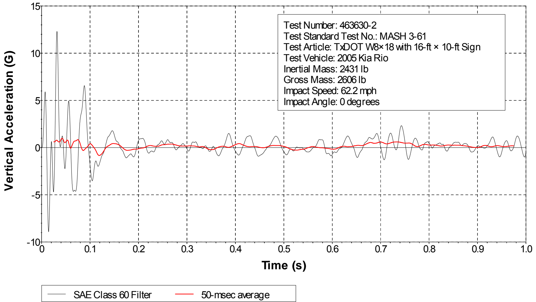
Figure F9. Vehicle Vertical Accelerometer Trace for Test No. 463630-2 (Accelerometer Located over Rear Axle).
