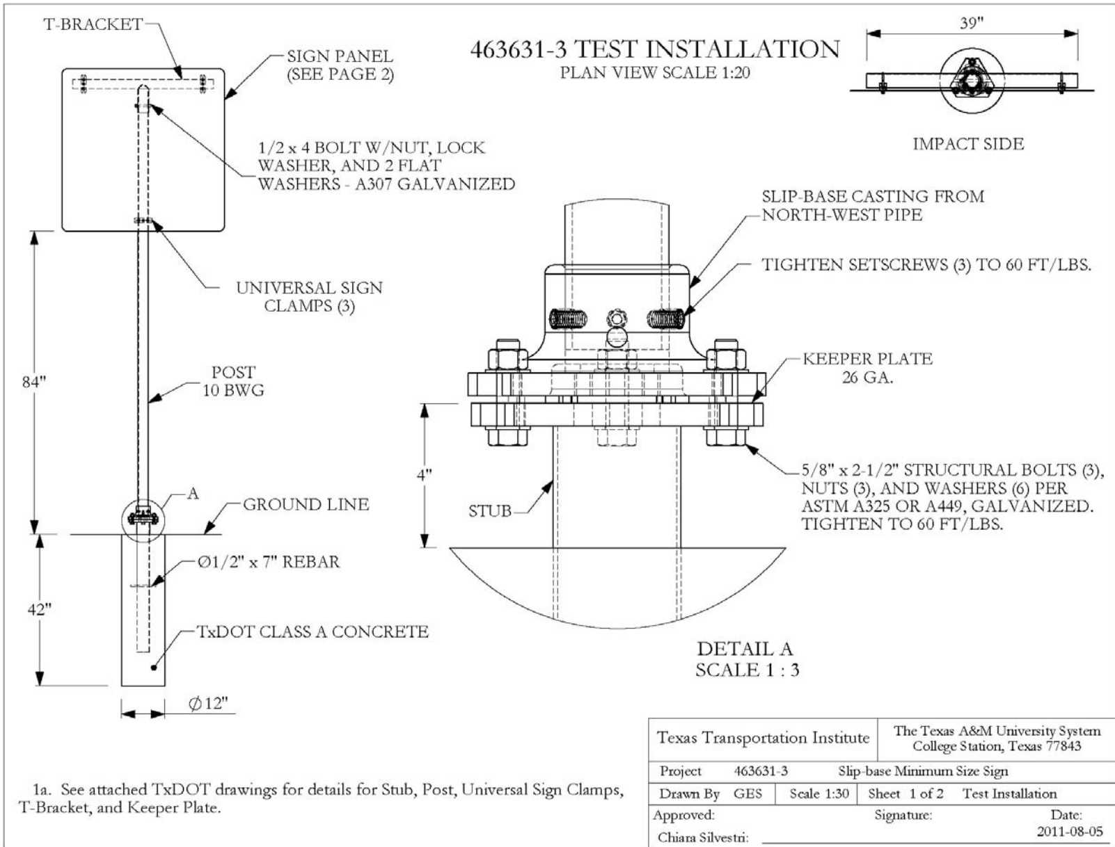
Figure J1. Details of the 10 BWG Steel Support with 14 ft 2 Sign.
