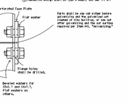
Figure 5.4. Current TxDOT Large Guide Sign Supports Slipbase and Fuse Plate Details.
