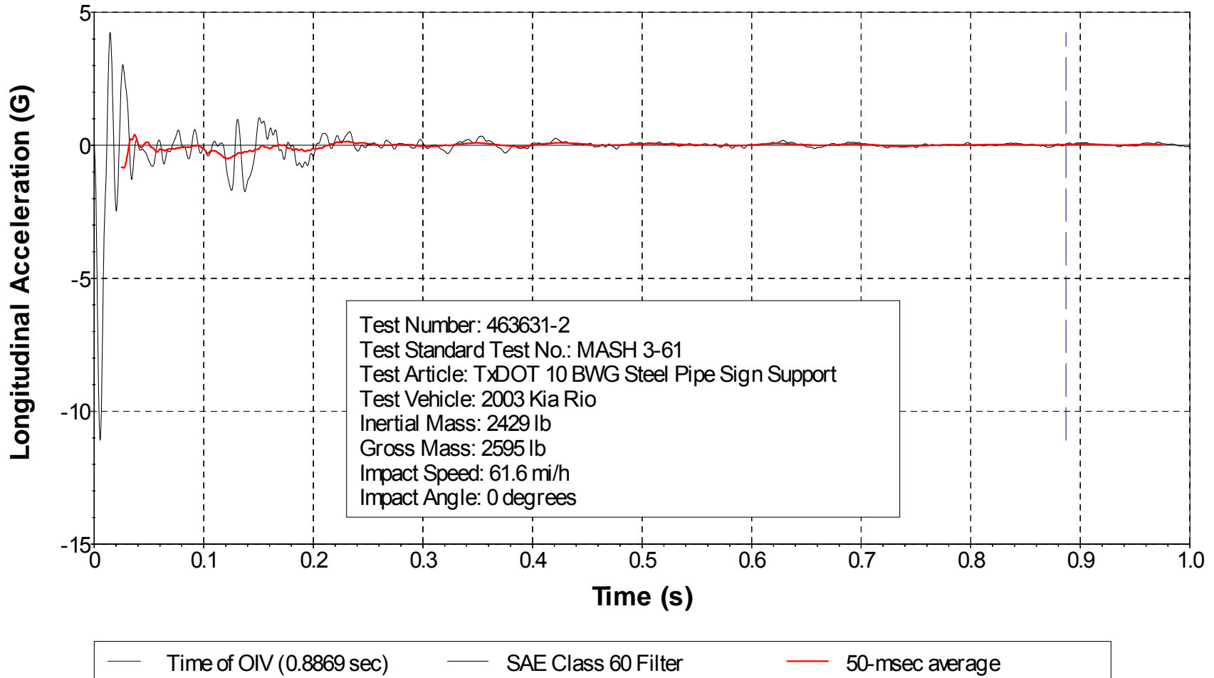
Figure I3. Vehicle Longitudinal Accelerometer Trace for Test No. 463631-2 (Accelerometer Located at Center of Gravity).
