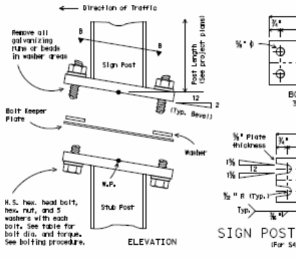
Figure 5.4. Current TxDOT Large Guide Sign Supports Slipbase and Fuse Plate Details.
