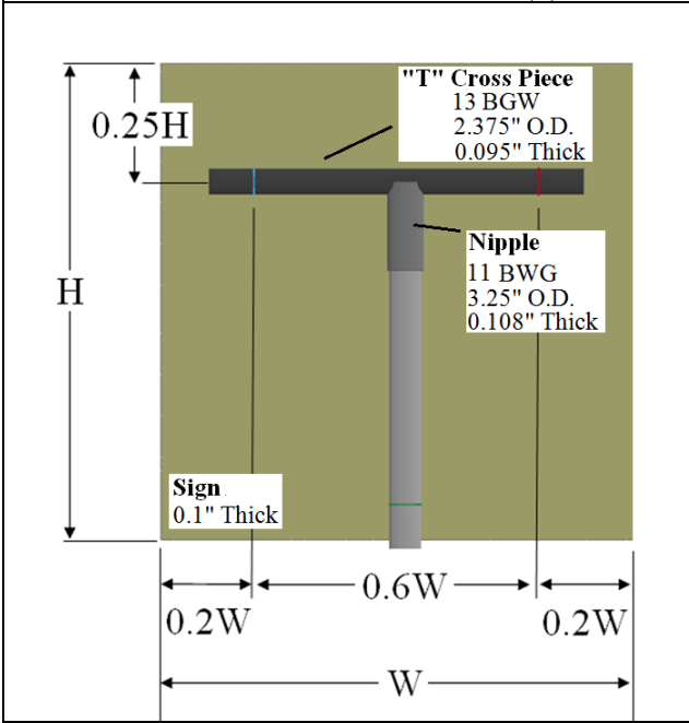
(b) Details T-Bracket Configuration #1
