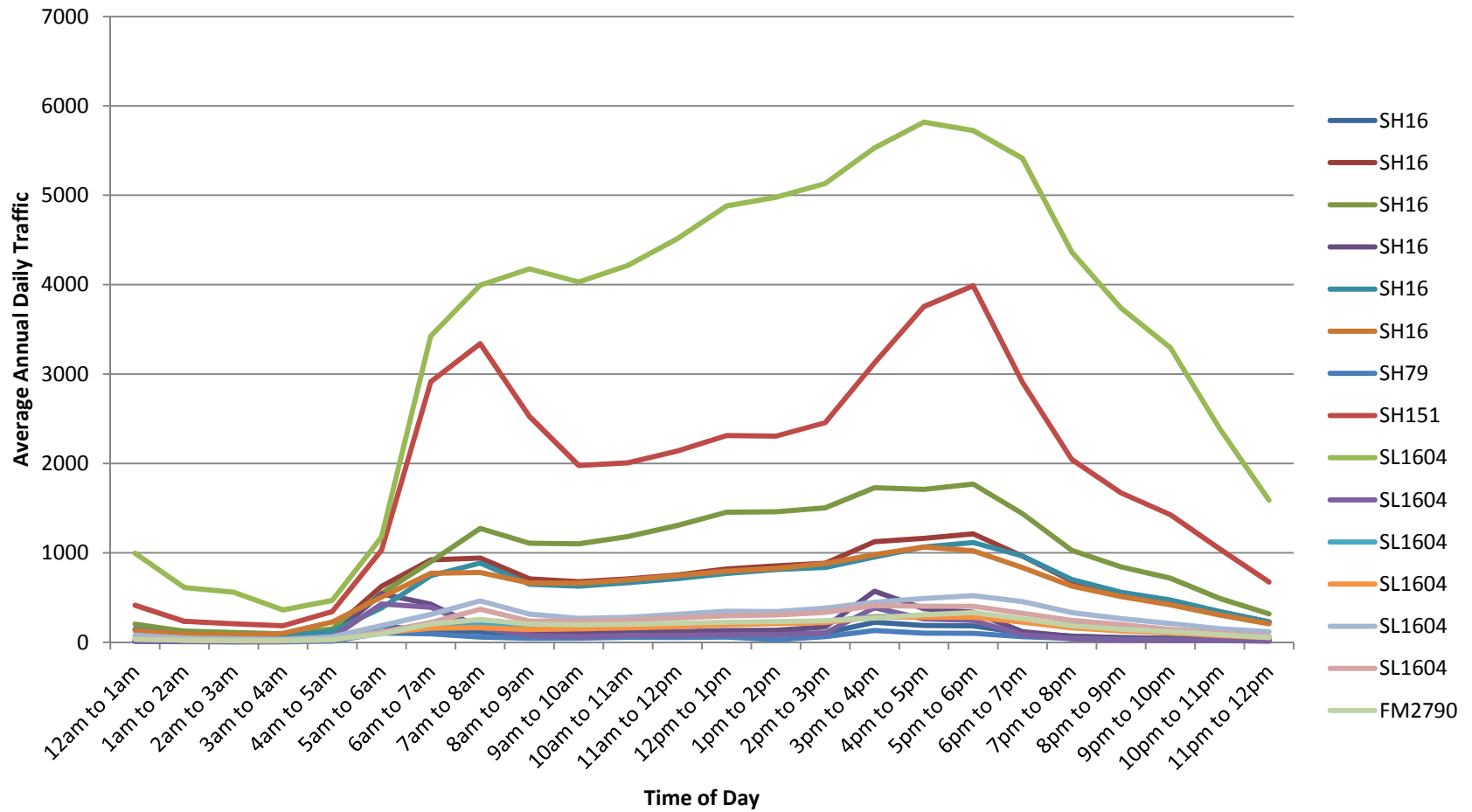
Figure 14. 2009 Hourly Counts (San Antonio)—State Highways, State Loop Roads, and Farm-to-Market.
