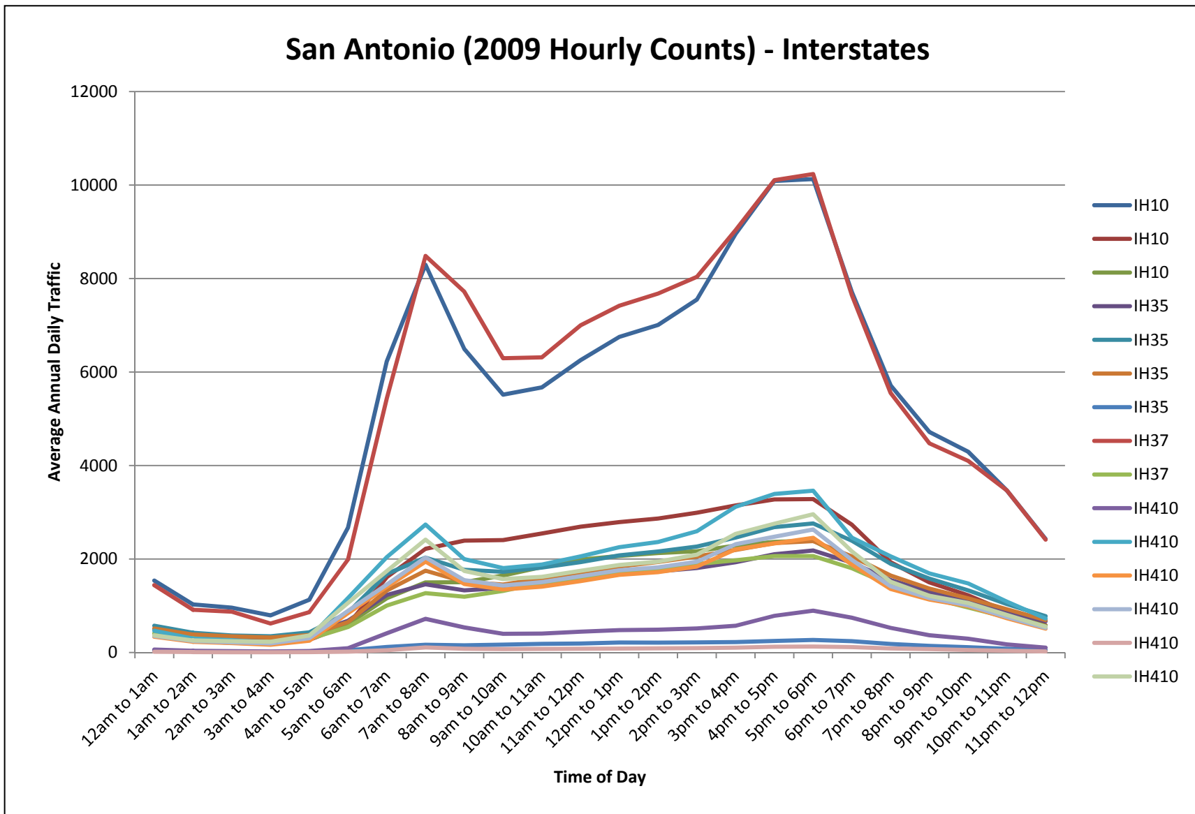
Figure 12. 2009 Hourly Counts (San Antonio)–Interstates Only.
