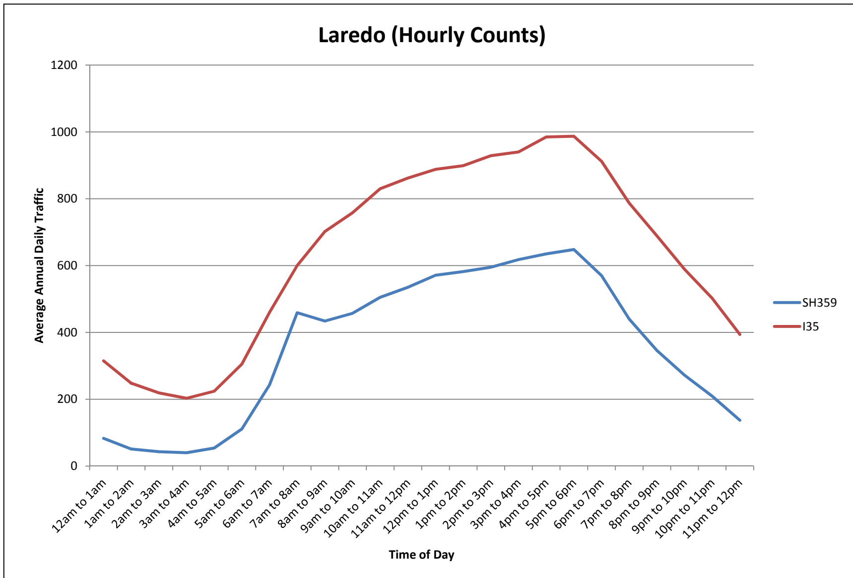
Figure 9. 2009 Hourly Counts (Laredo).
