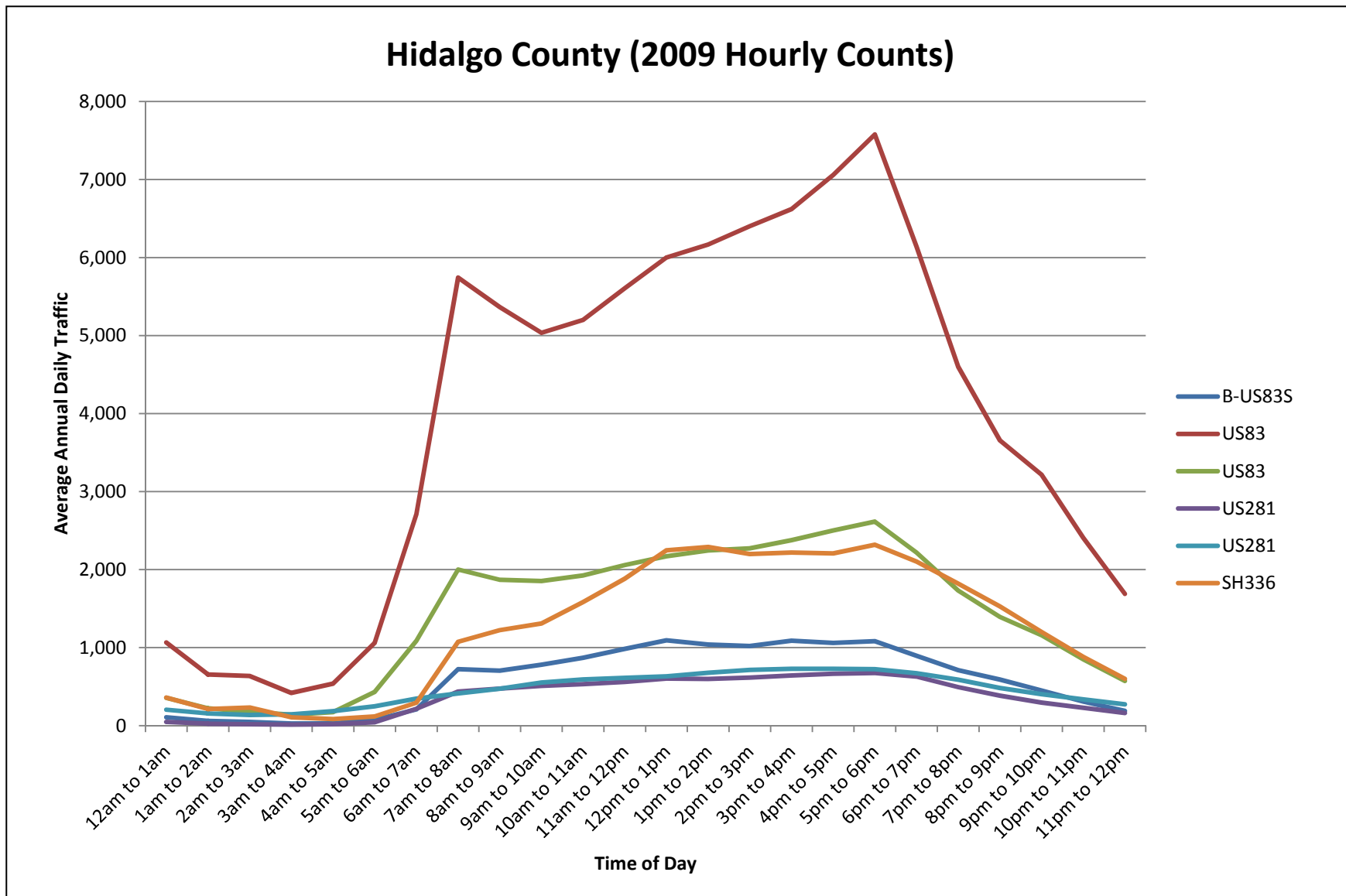
Figure 8. 2009 Hourly Counts (Hidalgo County).
