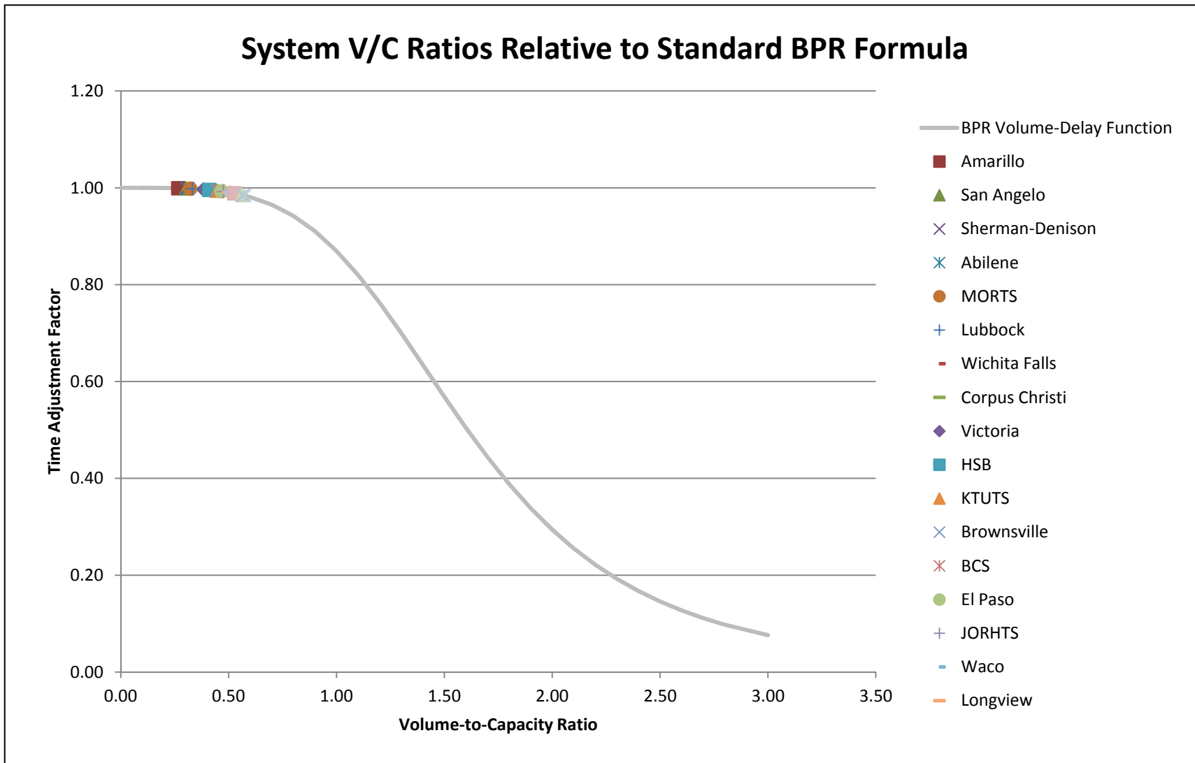
Figure 19. System Volume-to-Capacity Ratios Relative to BPR Formulation.
