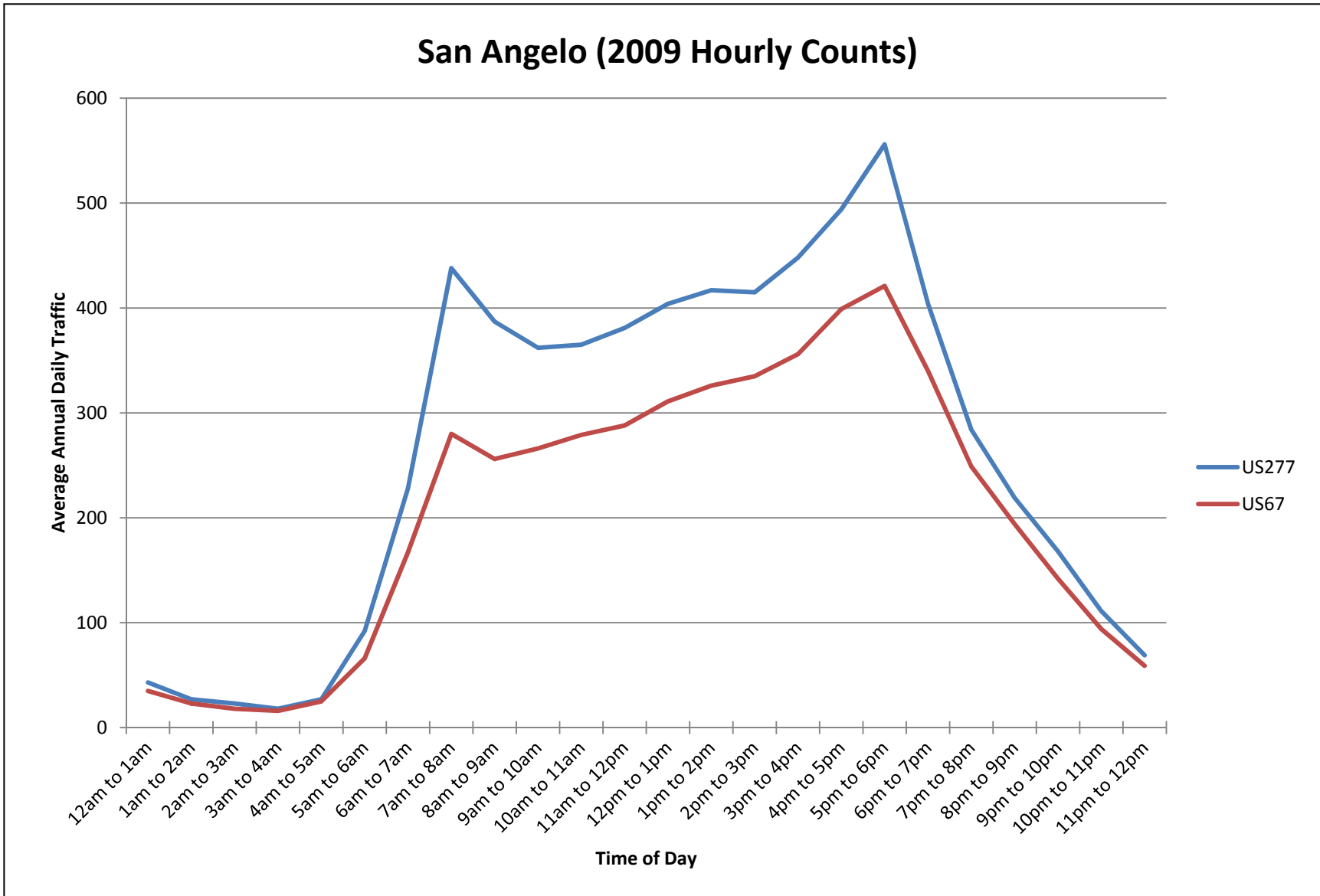
Figure 11. 2009 Hourly Counts (San Angelo).
