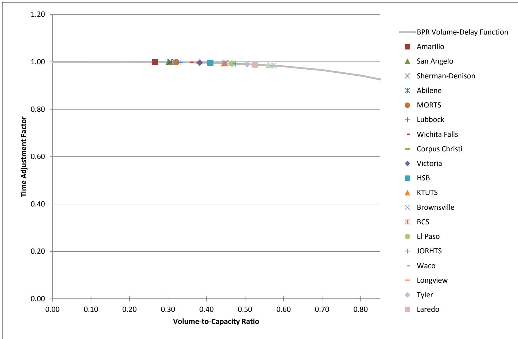
Figure 20. V/C Ratios Relative to BPR Formulation (Magnified).
