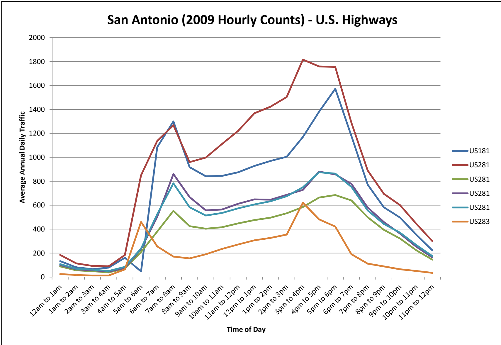
Figure 13. 2009 Hourly Counts (San Antonio)–U.S. Highways Only.
