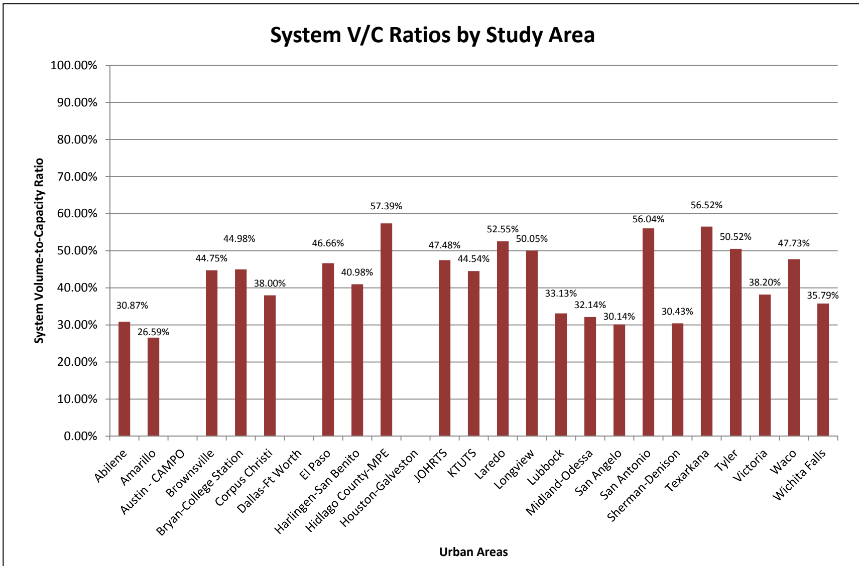
Figure 18. Volume-to-Capacity Ratios by Study Area.
