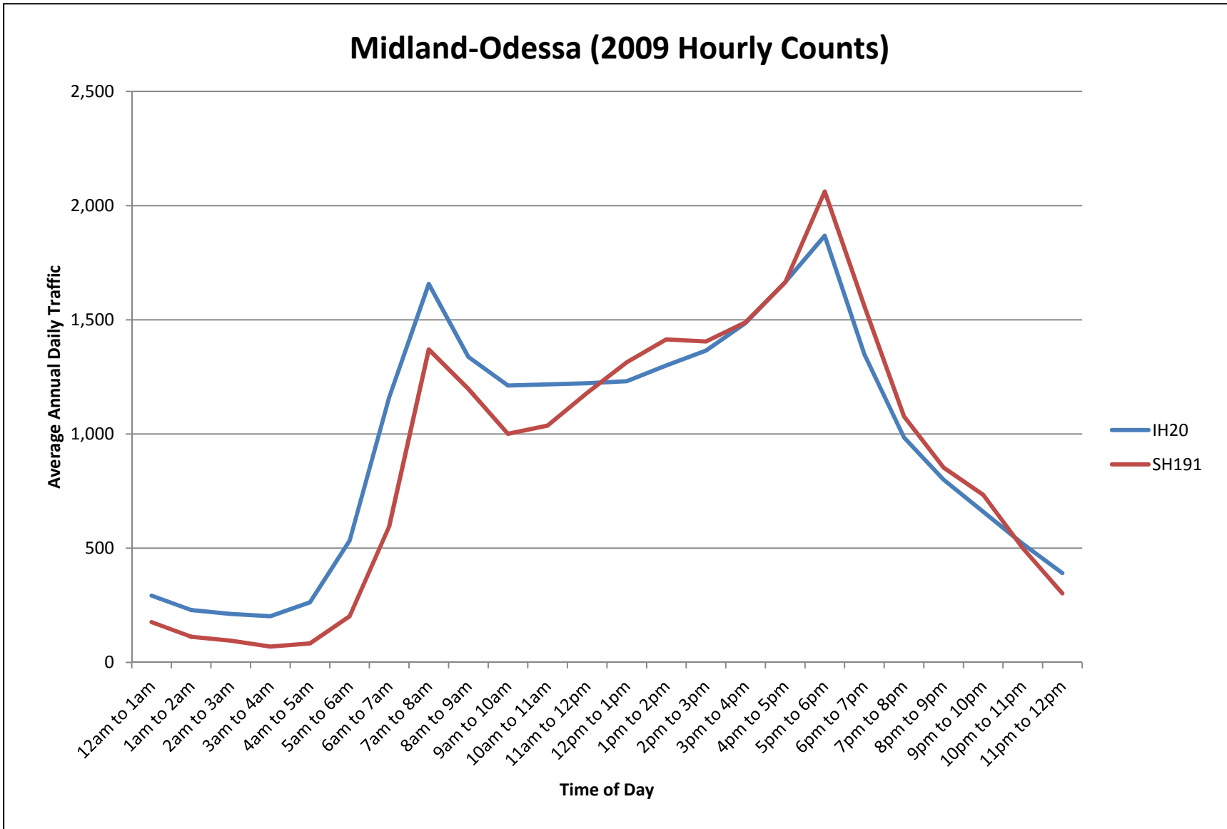
Figure 10. 2009 Hourly Counts (Midland-Odessa).
