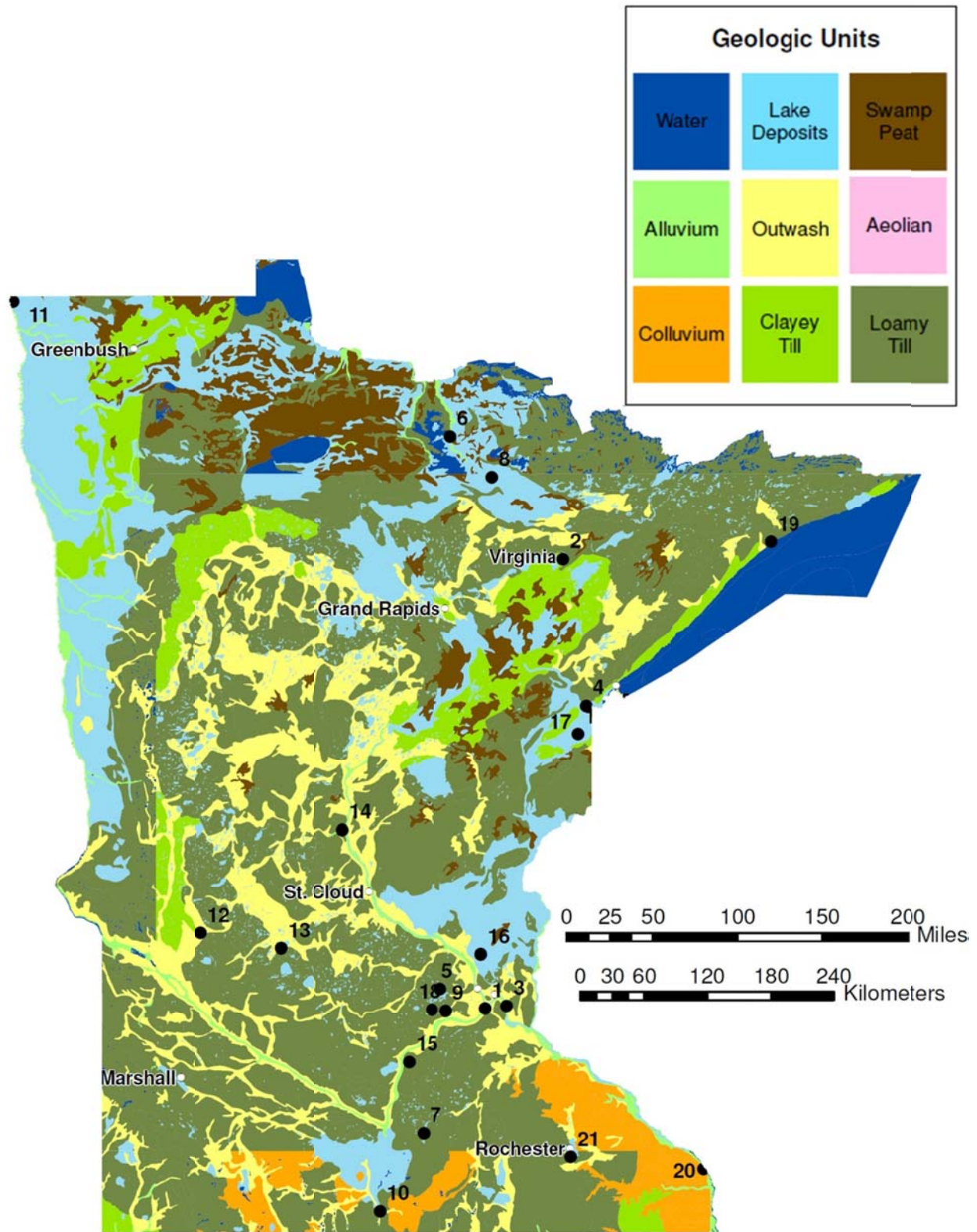
Figure 2.16. Location of Mn/DOT CPT sites with detailed analysis on a map of Minnesota Quaternary geology. Map adapted from data on previously published maps (Goebel et al. 1983, Farrand et al. 1984, Hallberg et al. 1991, Sado et al. 1994, Swinehart et al. 1994, Fullerton et al. 1995, Sado et al. 1995, Fullerton et al. 2000)
