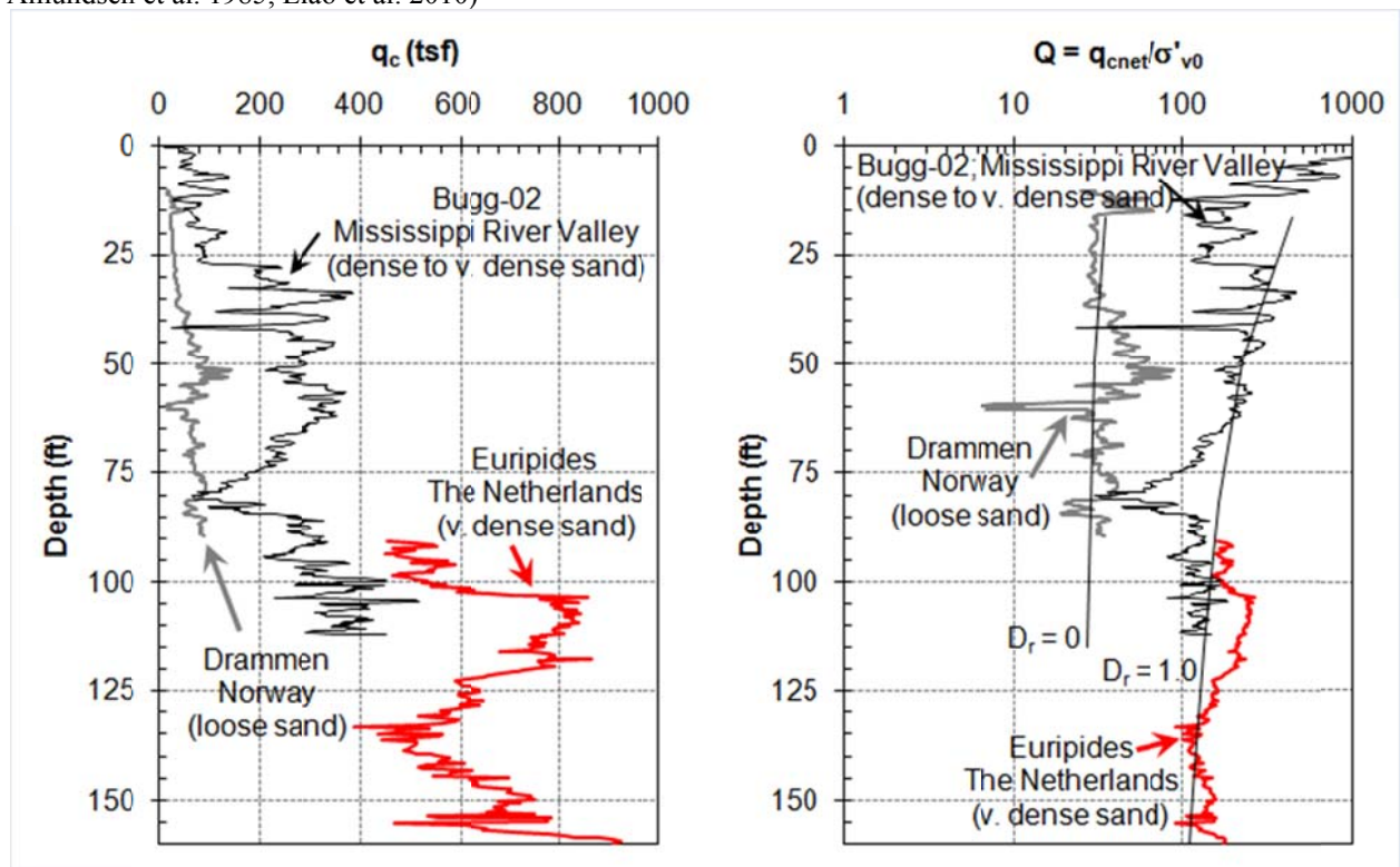
Figure 2.12. Normalized cone tip resistance in loose and very dense sands (after Schneider et al. 2008)
