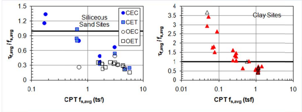
Figure 6.6. Comparison of CPT f_{s,avg} and pile \tau_{f,avg}
