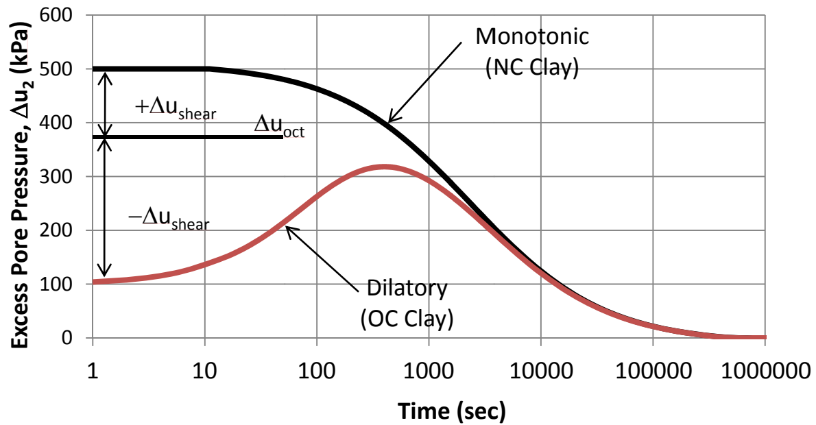
Figure 5.3. Comparison between a monotonic dissipation curve where positive shear pore-water pressures occur during penetration with a dilatory curve where negative pore-water pressures are generated (after Burns and Mayne 1998).
