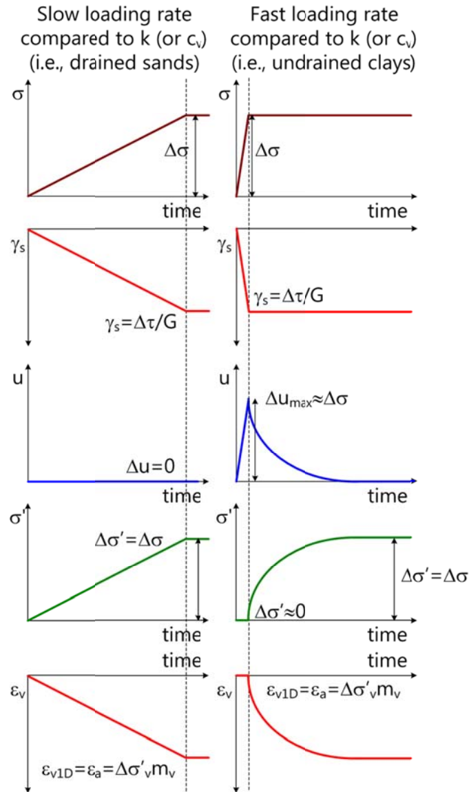
Figure 2.4. Influence of loading rate on changes in effective stress and volume during loading (after Atkinson 2007) \sigma = total stress, \gamma_s = shear strain, u = pore water pressure, \sigma' = effective stress, \epsilon_v = volumetric strain
