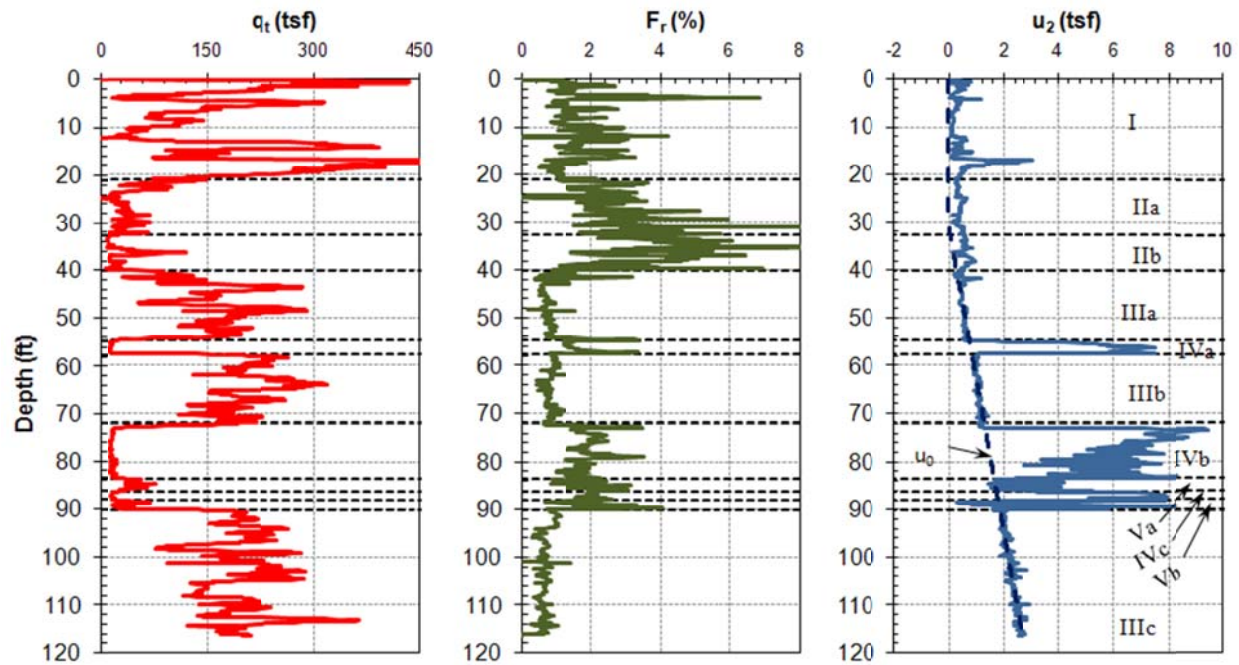
Figure 4.1. Vertical profile of CPT parameters at the sandy Wakota Bridge site, MN
