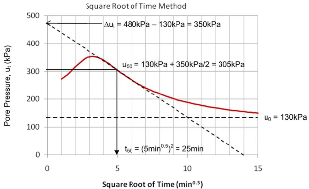
Figure 5.4. Evaluation of dilatory dissipation using square root of time method (after Sully et al. 1999)
