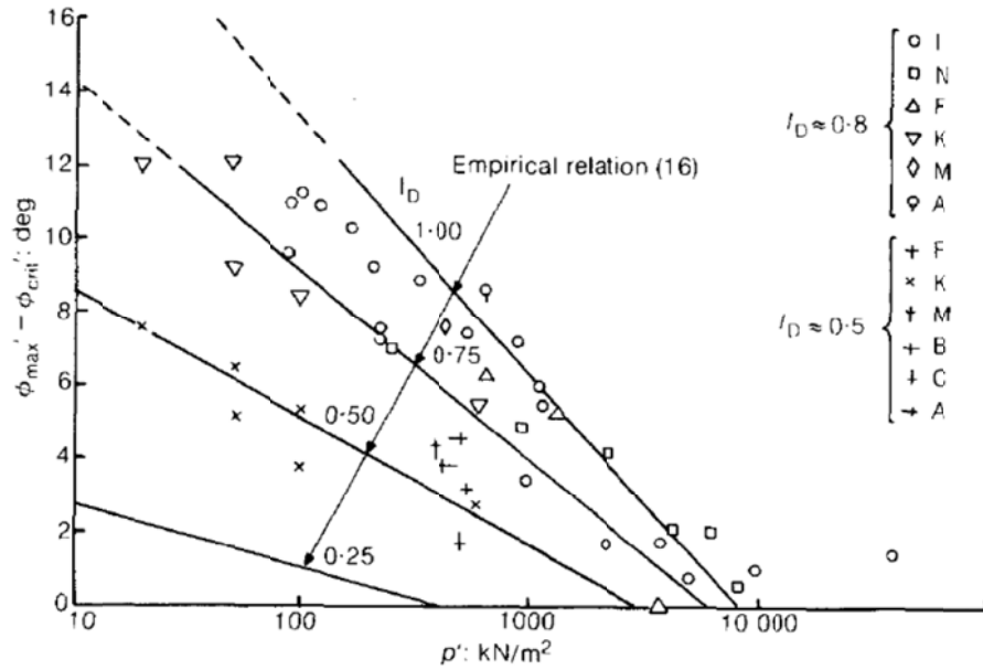
Figure 2.10. Influence of mean stress at failure on the peak friction angle due to dilation (Bolton 1986)
