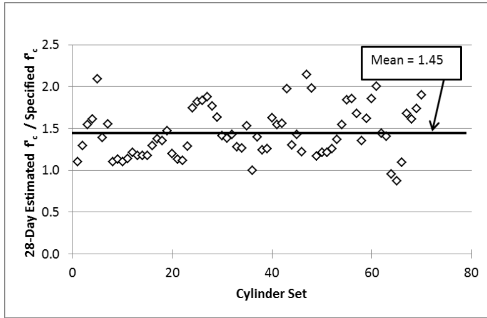
Figure 5-4 The ratio of the estimated actual 28-day strength to the specified 28-day strength for tested concrete cylinders.
