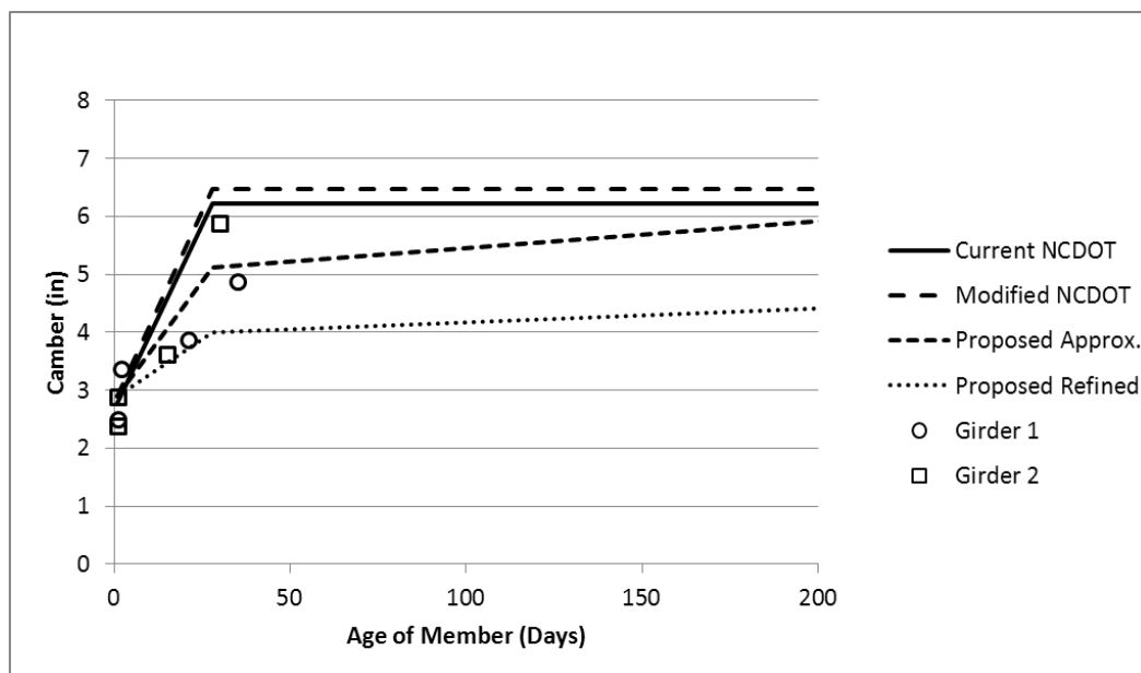
Figure B-1 Predicted and measured camber for two girders.
