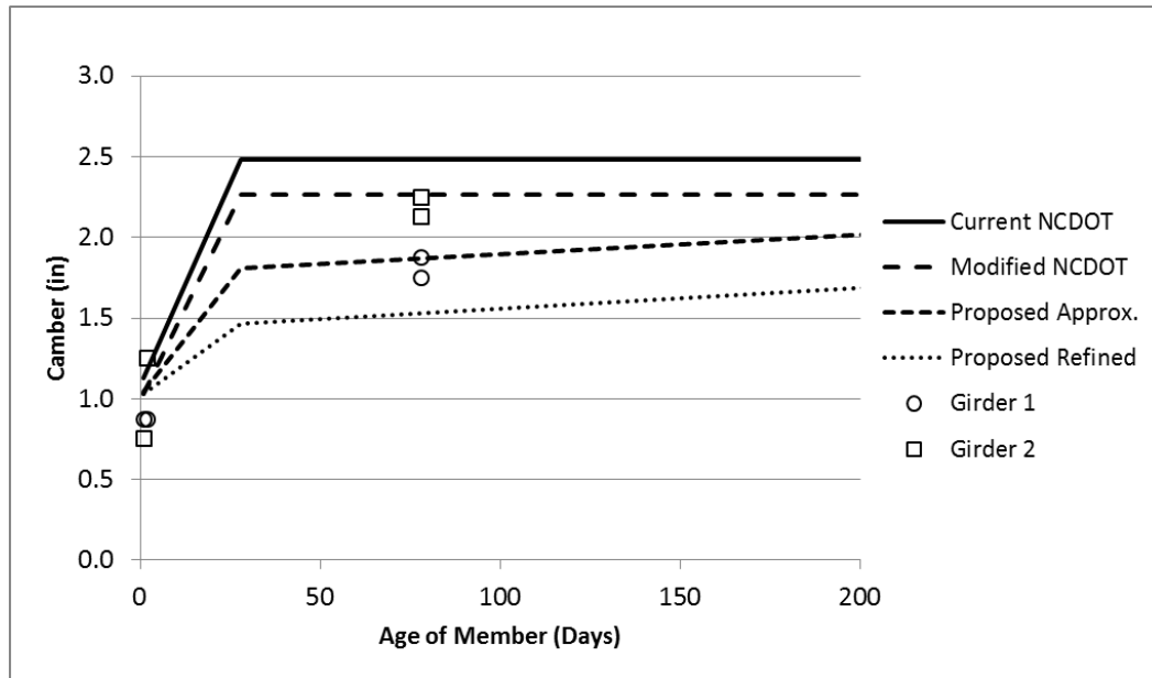
Figure 7-9 Predicted and measured cambers for two identical box beams observed during site visits to Ross Prestress in Bristol, TN. The proposed methods provide improved predictions of camber compared to the current NCDOT method.
