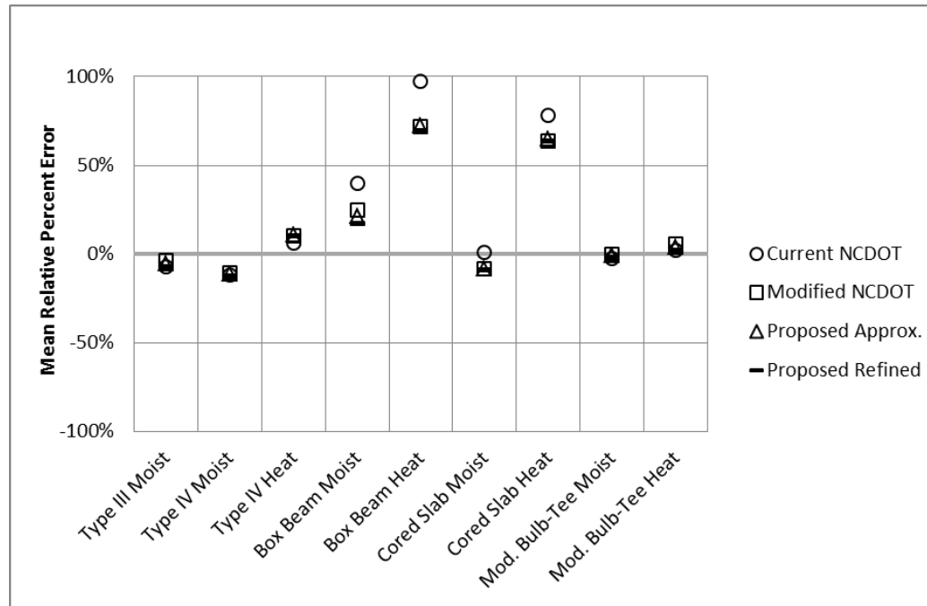
Figure 7-3 Mean relative percent error of the camber predictions for measurements taken at prestress transfer.
