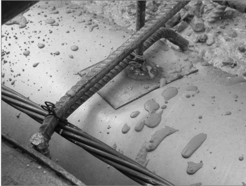
Figure 5-10 A thin metal plate is used to contact the void tube for the hold-down system, resulting in significant local deformation.
