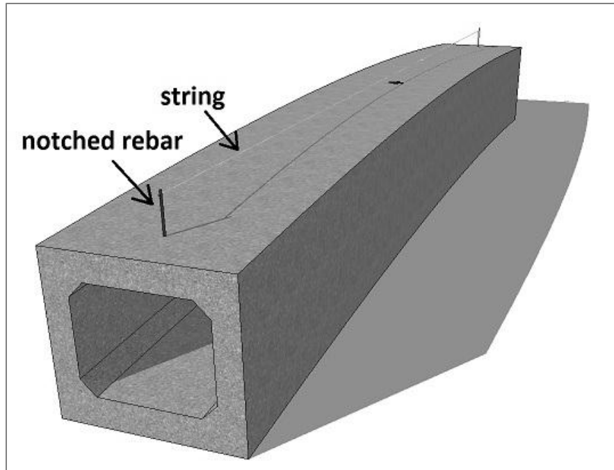
Figure 4-1 Girder with rebar and string in place for camber measurements.
