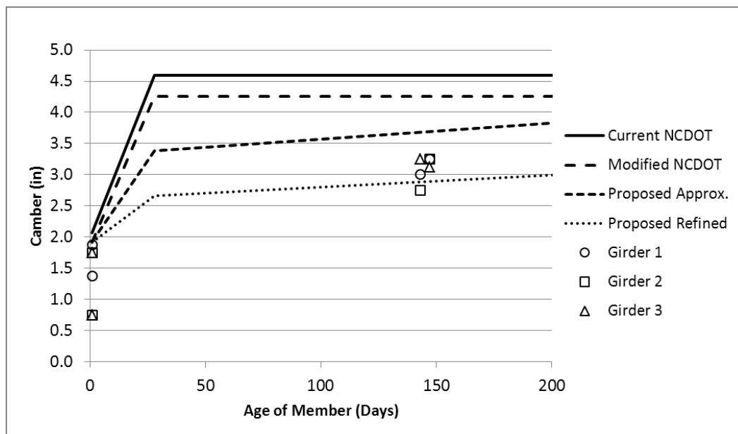
Figure 7-10 Predicted and measured cambers for three identical box beams observed during site visits to Eastern Vault in Princeton, WV. The proposed methods provide improved predictions of camber compared to the current NCDOT method.
