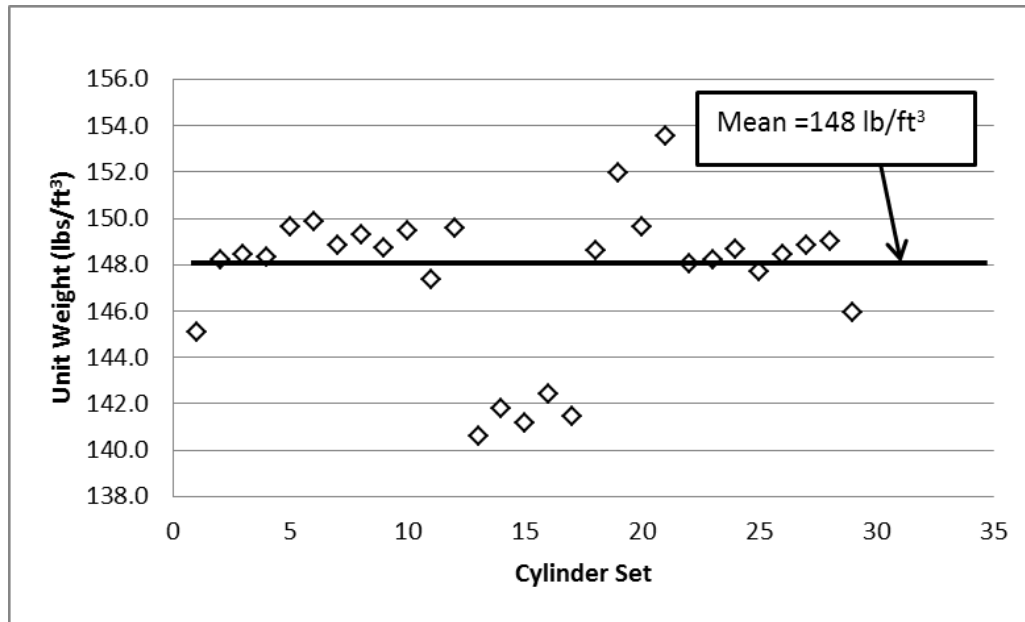
Figure 5-2 Measured unit weight of concrete cylinders.
