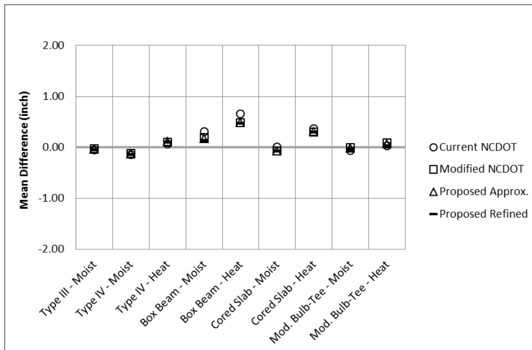
Figure 7-4 Mean difference (predicted camber - measured camber) at prestress transfer.
