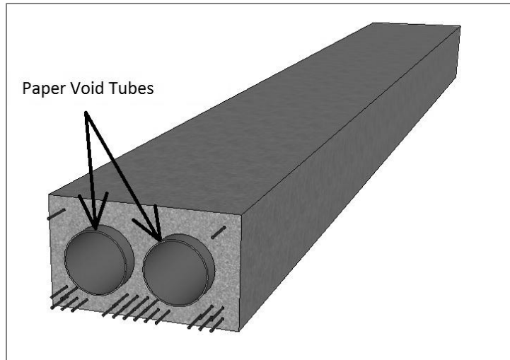
Figure 5-8 Paper tubes are used for the internal voids in cored slabs.
