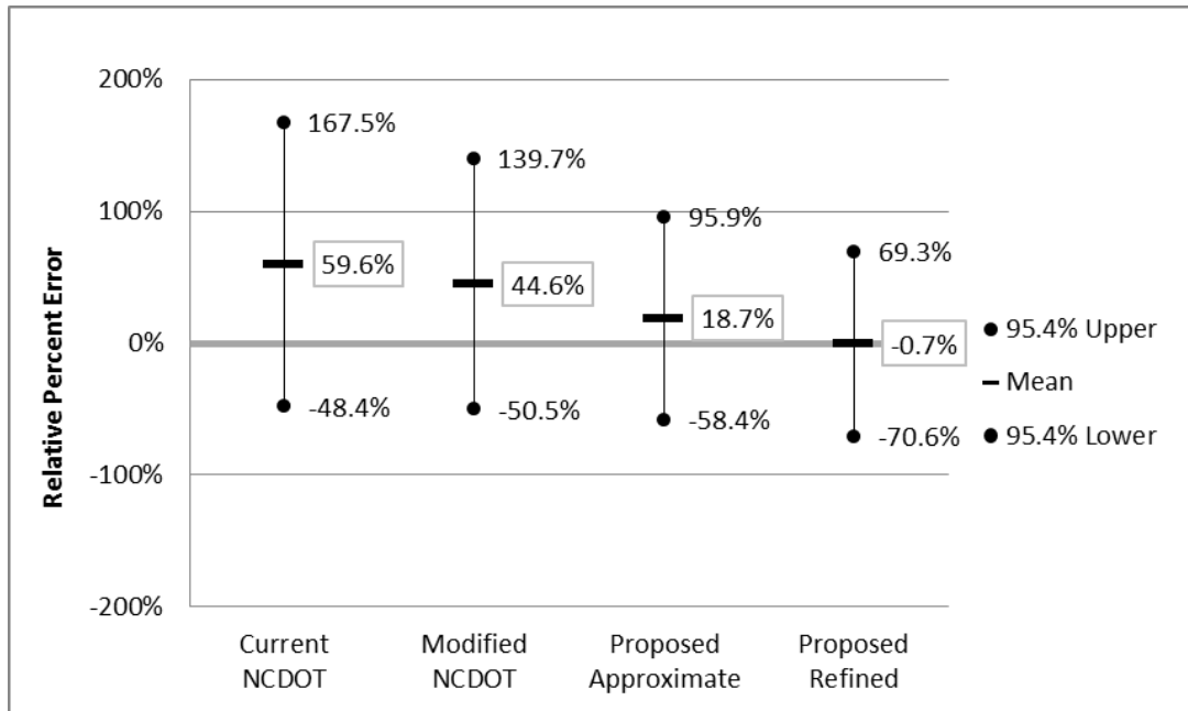
Figure 7-2 Distribution of relative percent error for moist cured cored slabs; includes camber measurements taken at 24 days or greater.
