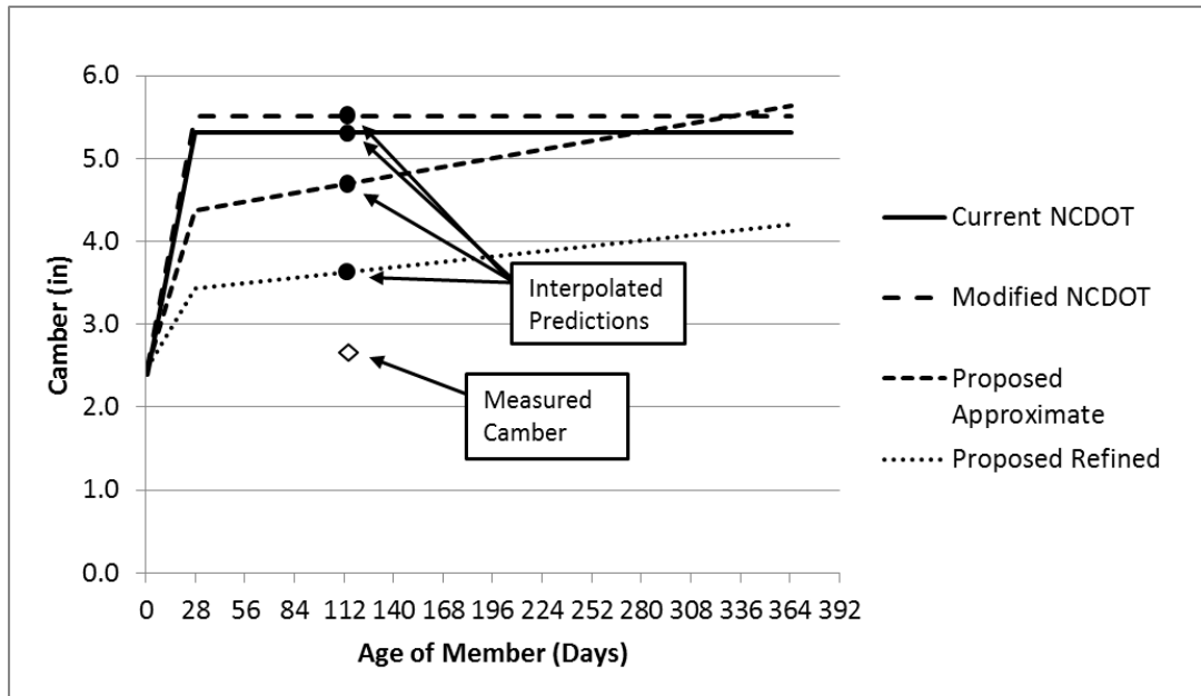
Figure 7-1 Camber is predicted at transfer, at 28 days, and at one year for each prediction method to obtain a bilinear prediction curve. Linear interpolation between these points is performed to determine the predicted value at the time that camber is actually measured.
