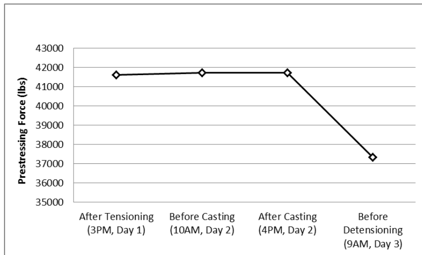
Figure 4-5 Average prestressing force at various stages for box beams cast during the site visit to Eastern Vault in Princeton, WV.
