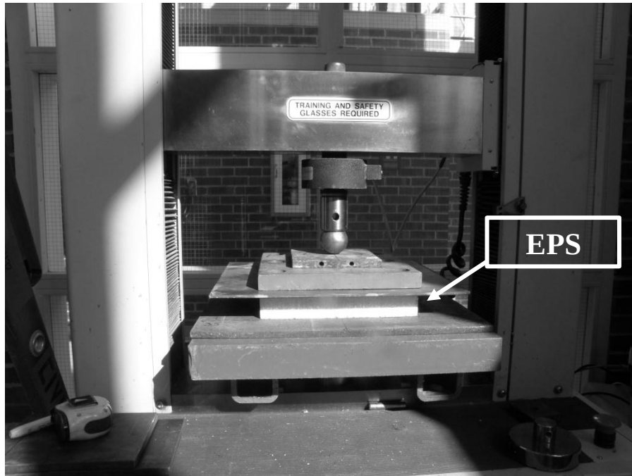
Figure F-1 Testing of EPS void material for elastic modulus and yield stress.
