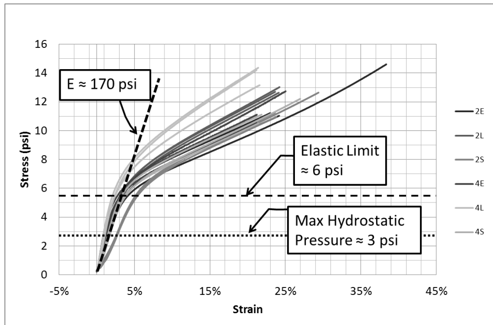
Figure F-2 Compression test results for EPS void material.
