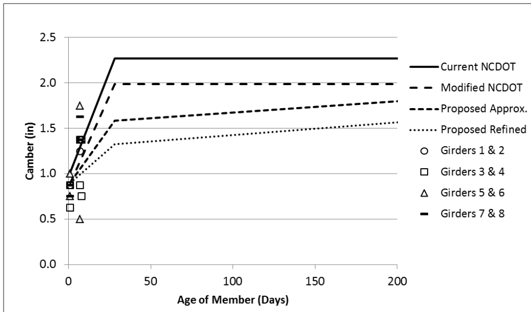
Figure 7-8 Predicted and measured cambers for eight identical cored slabs observed during site visits to S&G Prestress in Wilmington, NC. The camber varies widely at early ages.
