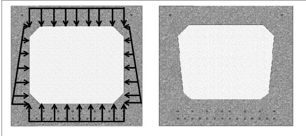
Figure A-1 Distribution of the hydrostatic pressure on the internal foam void of the box beam and the resulting deformed section.
