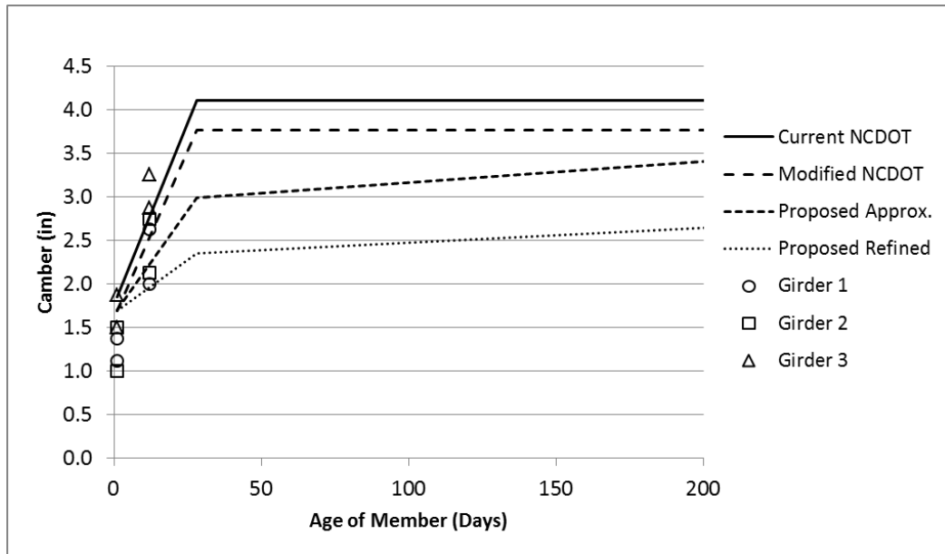
Figure 7-7 Predicted and measured cambers for three identical cored slabs observed during site visits to Utility Precast in Concord, NC. The camber varies widely at early ages.
