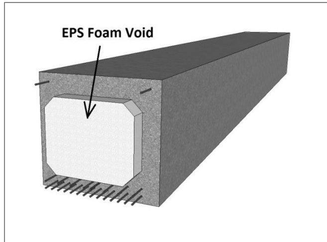
Figure 5-6 Expanded polystyrene blocks are used to form the internal voids in a box beam.
