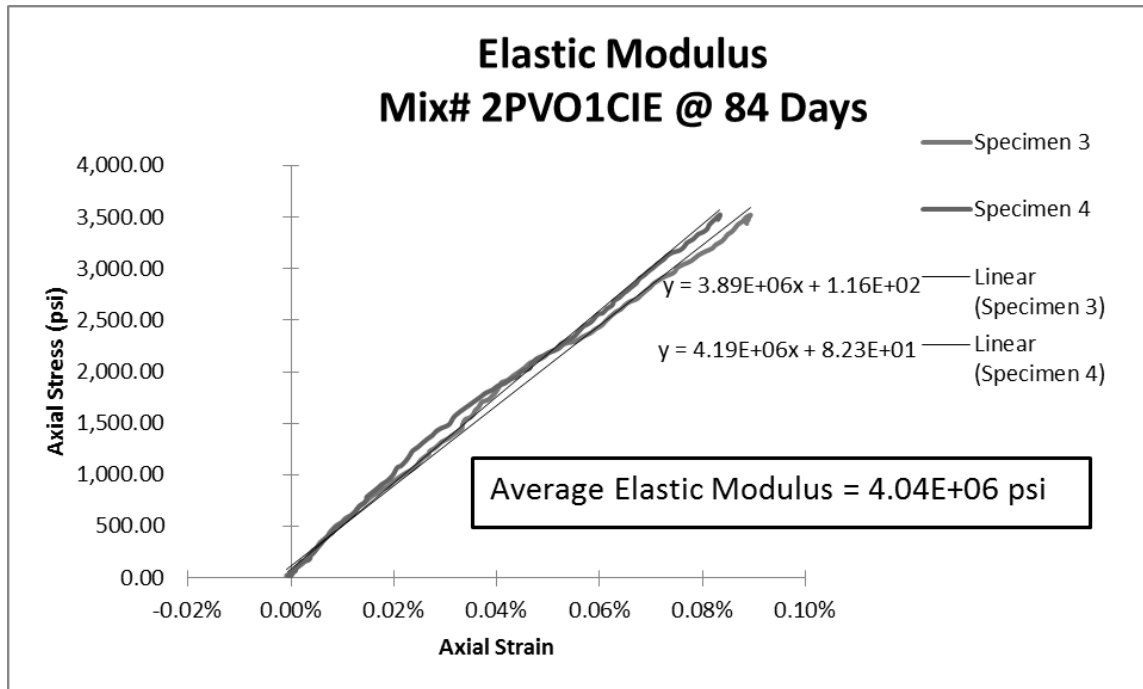
Figure E-2 Sample elastic modulus test results for a set of two concrete cylinders.
