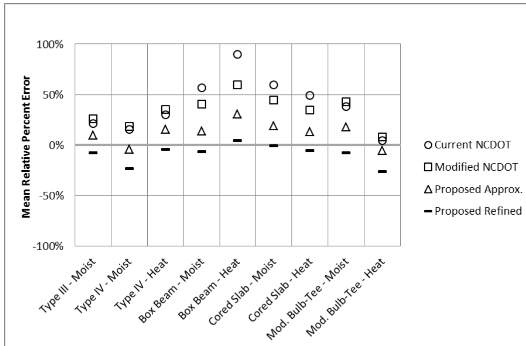
Figure 7-5 Mean relative percent error of the camber predictions for measurements taken at 24 days or later.
