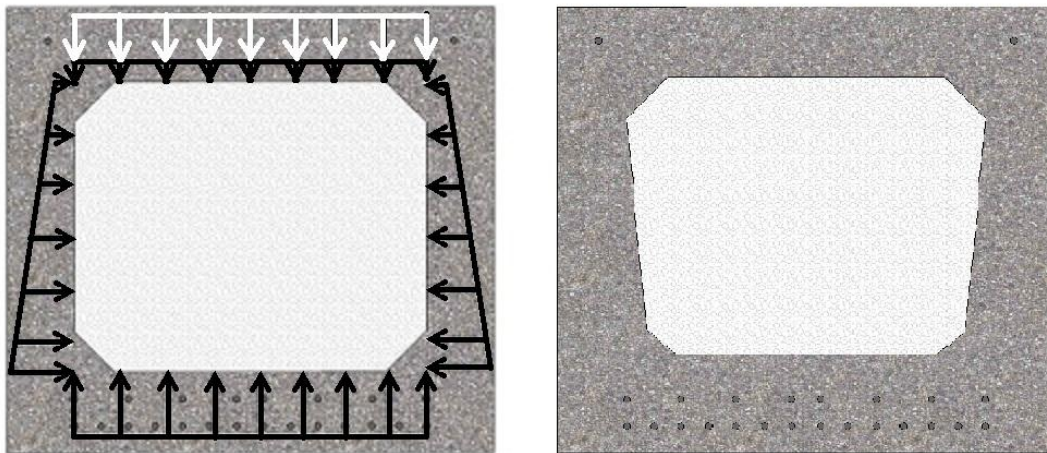
Figure 5-12 Distribution of the assumed pressures acting on the box beam EPS void form and the resulting deformed shape. The black arrows represent the hydrostatic pressure, while the white arrows represent the magnitude of the hold-down support reaction if it were evenly distributed along the entire top surface of the EPS form.
