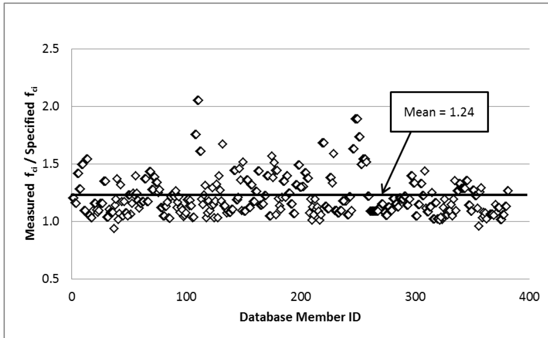
Figure 5-3 Ratio of measured concrete strength to specified strength at the time of prestress transfer.
