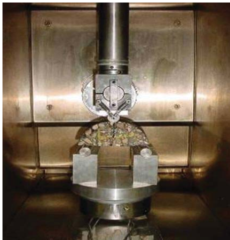
Semi circular bend test set up
