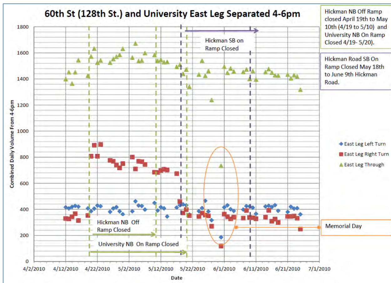
Figure 20. Sample intersection approach counts by movement, 128th Street
