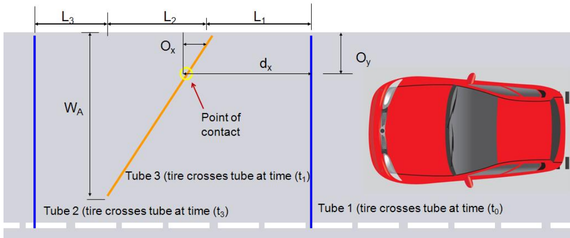
Figure 3.5. Layout configuration of road tubes to measure lateral displacement
