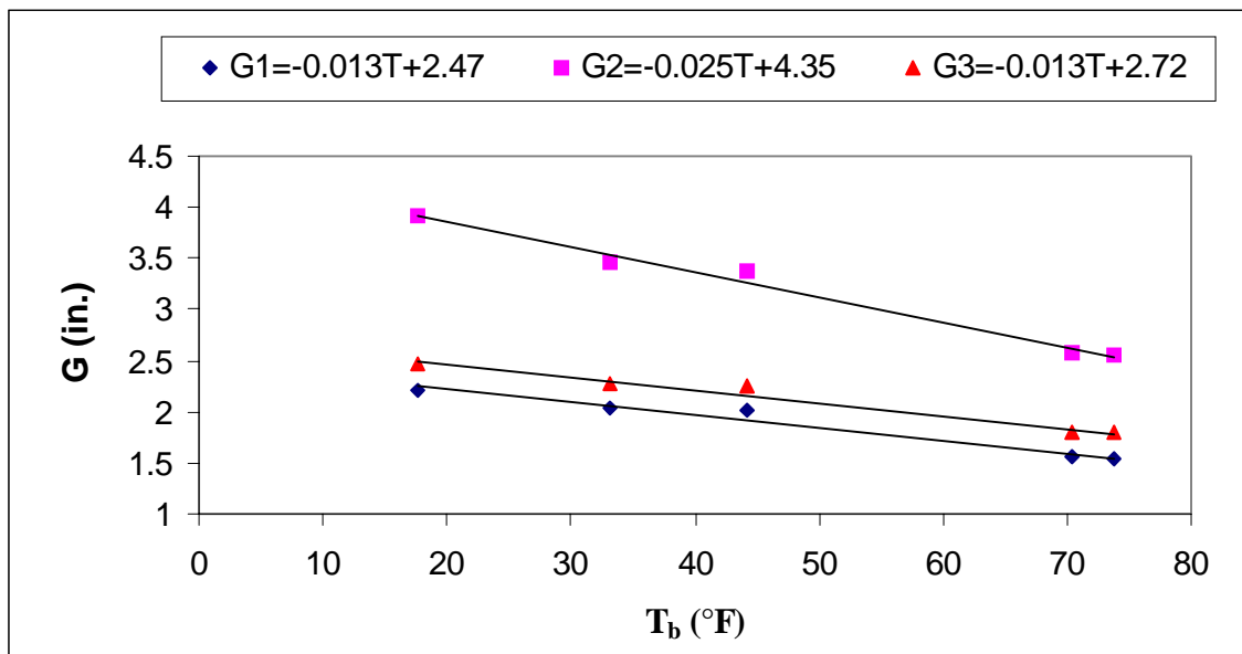
Figure 6.25 Gap openings vs. bridge temperature for Bridge 6 (0784.8S218)
