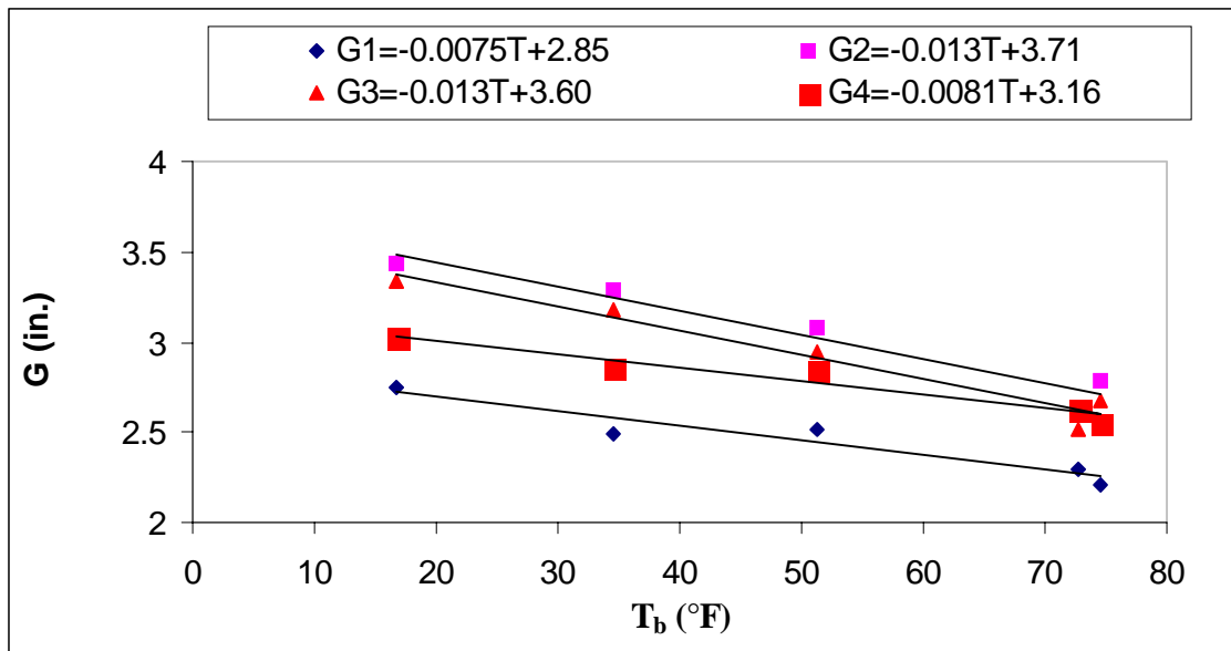
Figure 6.17 Gap openings vs. bridge temperature for Bridge 4 (0996.0L218)
