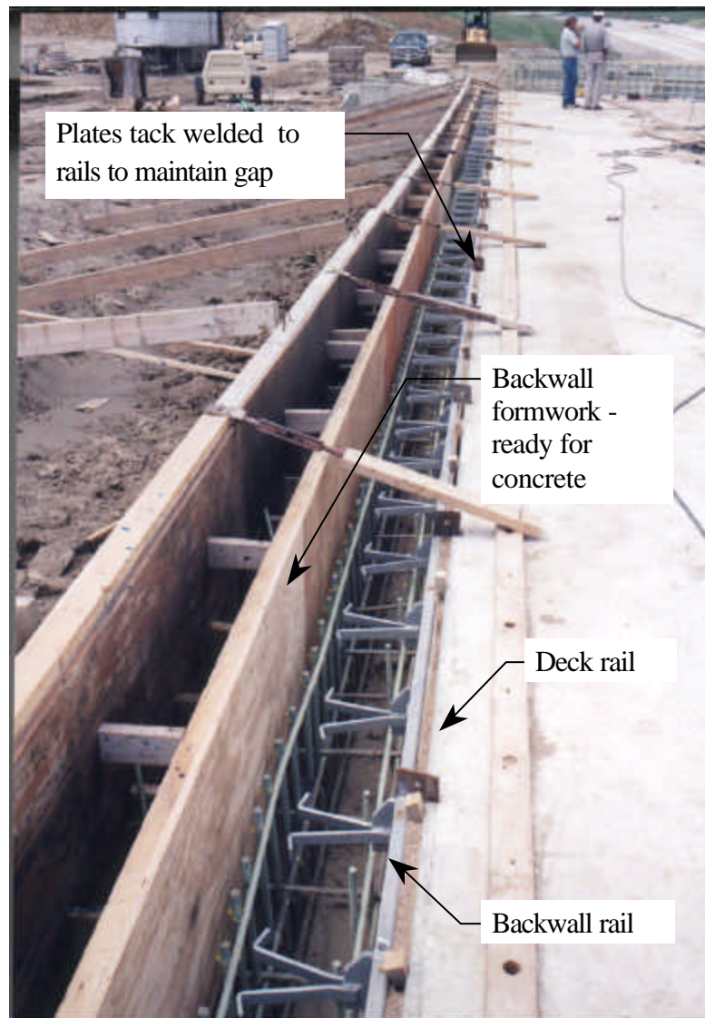
Figure 4.15 West backwall formed and ready for concrete
