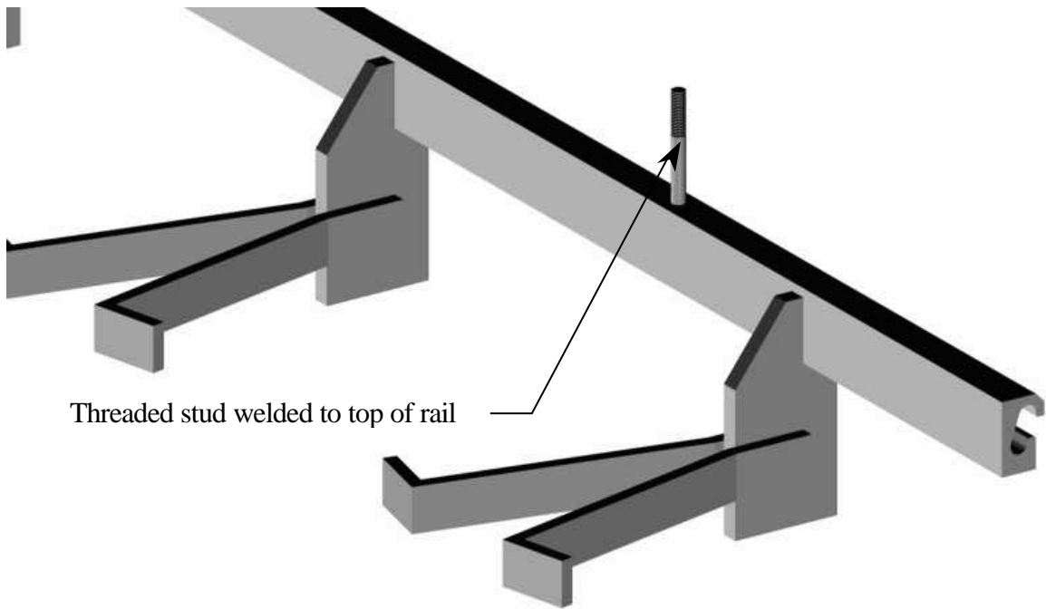
Figure 4.9 Threaded studs are one mechanism used to hold rails in position (see Figure 4.1)
