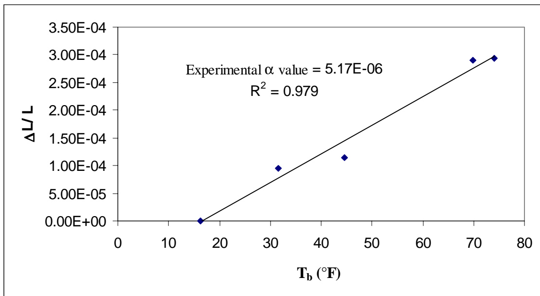
Figure 6.9 The experimental \alpha -value for Bridge 2 (0781.1L218)
