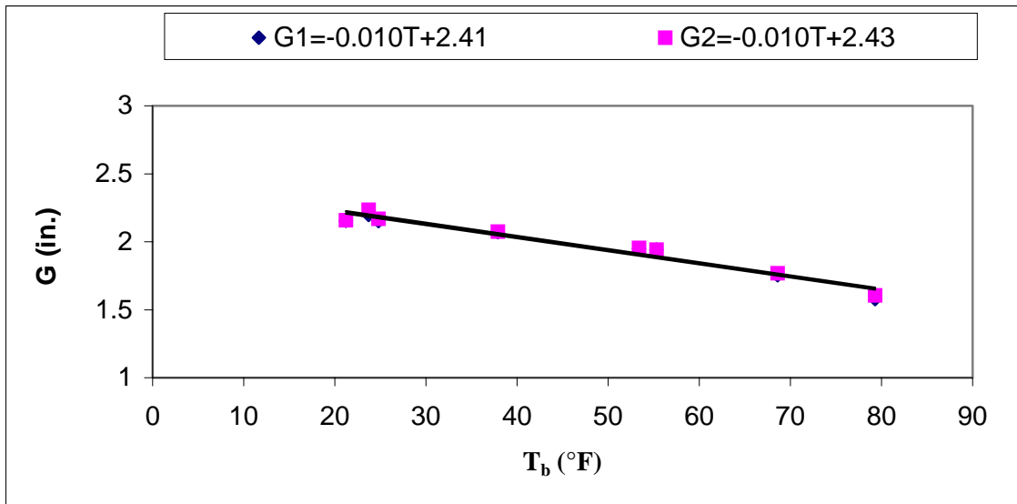
Figure 6.28 Gap opening vs. bridge temperature for Bridge 7 (8561.5L030)
