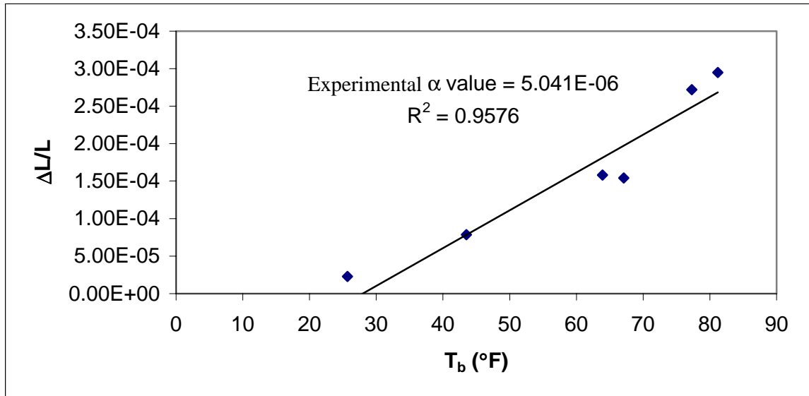
Figure 6.45 The experimental \alpha -value for Bridge 12 (6481.9L030)
