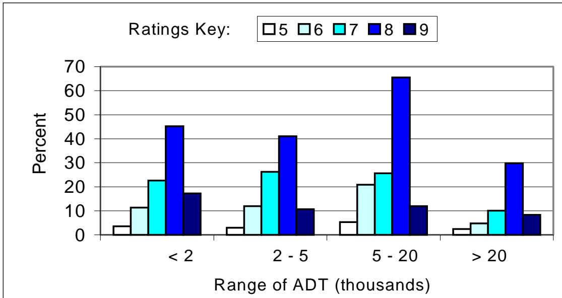
Figure 5.3 End deck joint strip-seal rating versus Average Daily Traffic (ADT)
