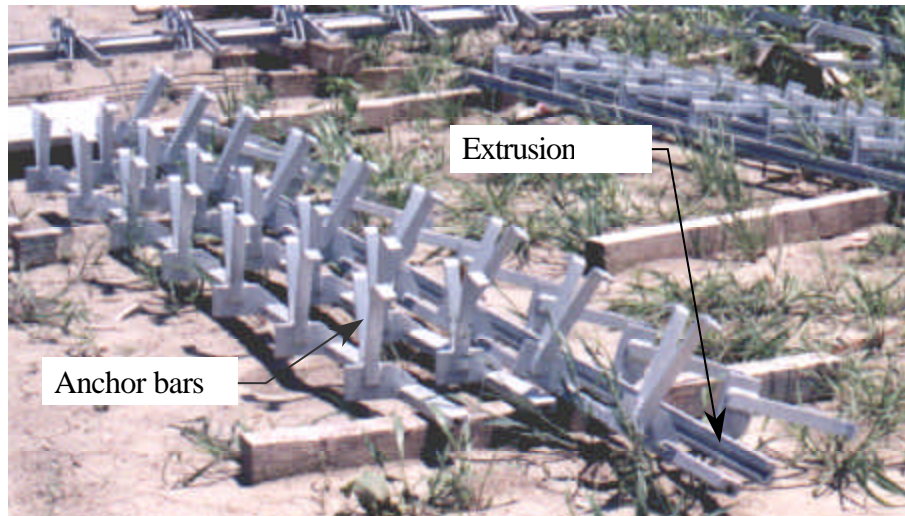
Figure 4. 6 Extrusions with anchorages stacked at construction site
