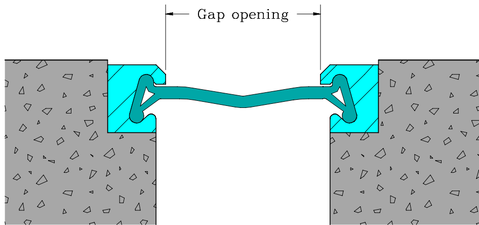
Figure 6.3 Measured expansion joint opening
