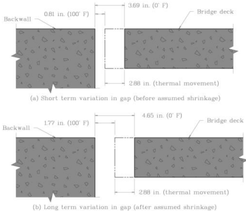
Figure 3.5 Predicted gap variation with and without the effects of shrinkage
