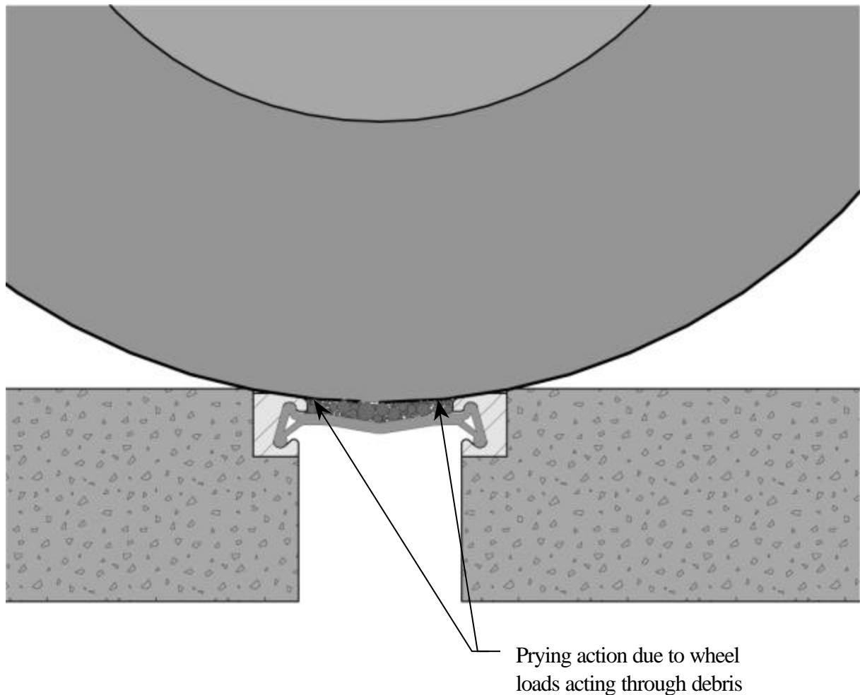
Figure 7.1 Interaction of wheel, seal, and debris when gap is near seal rating
