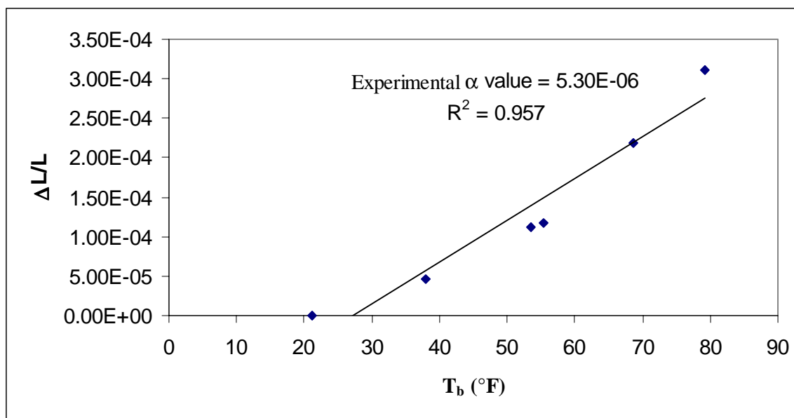
Figure 6.29 The experimental \alpha -value for Bridge 7 (8561.5L030)
