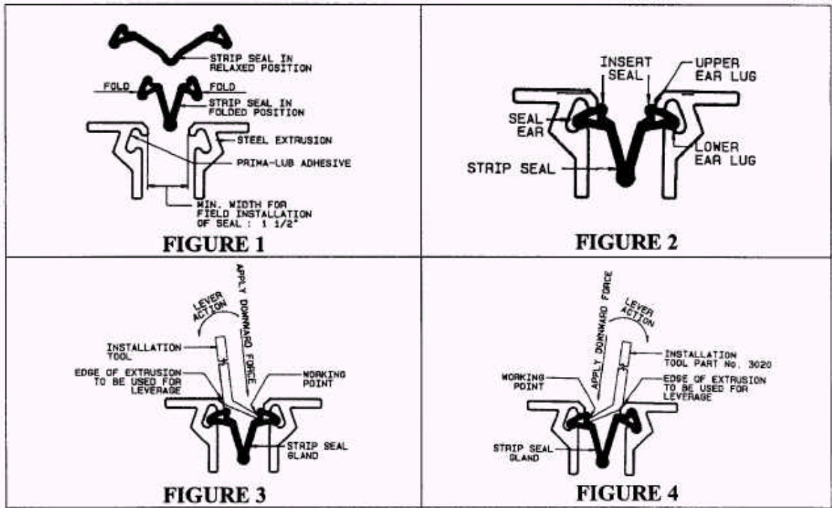
Figure 4. 2 Figures from Watson Bowman Acme to illustrate the seal installation steps
