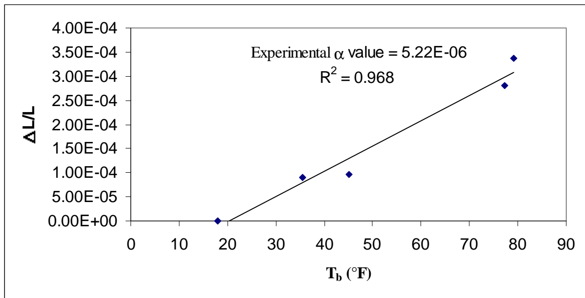
Figure 6.22 The experimental \alpha -value for Bridge 5 (0787.7A218)
