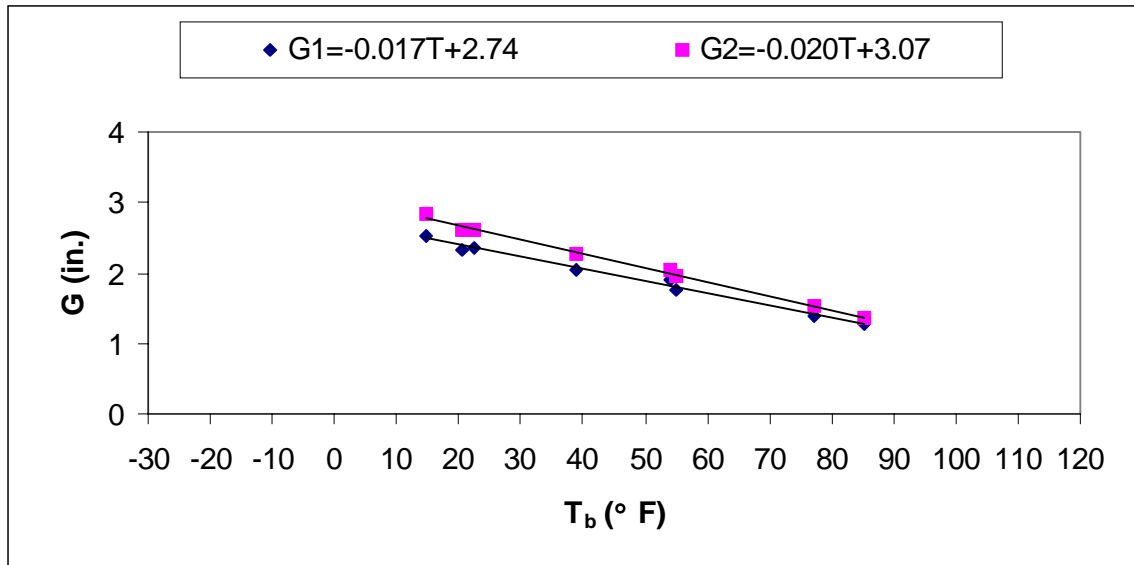
Figure 6.42 Gap opening vs. bridge temperature for Bridge 11 (6403.6L014)
