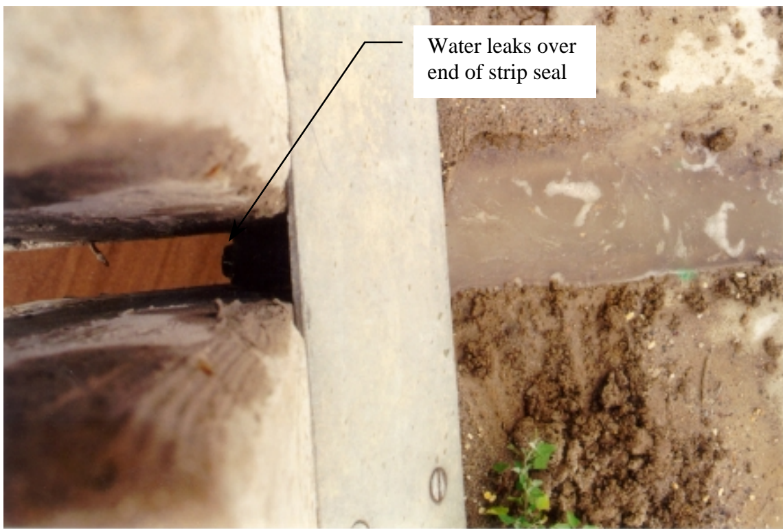
Figure 6.30 Strip seal at G3 for Bridge 8 (7776.8L065)
