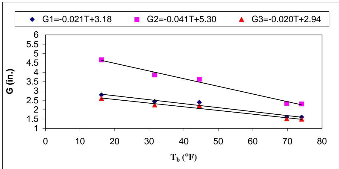
Figure 6.8 Gap openings vs. bridge temperature for Bridge 2 (0781.1L218)
