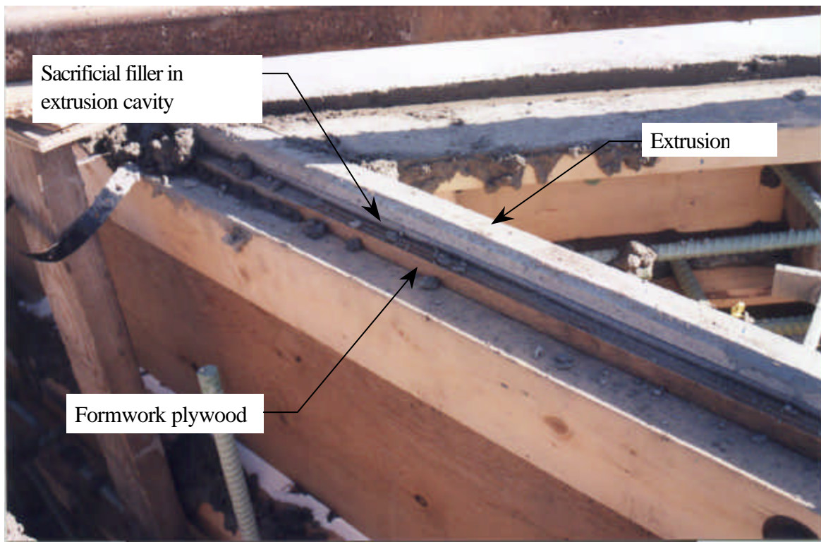
Figure 4.11 Foam backer rod was used to protect the cavity of the west side deck extrusion
