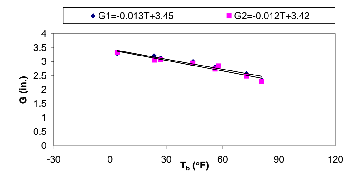
Figure 6.34 Gap opening vs. representative bridge temperature for Bridge 9 (6485.3L030)
