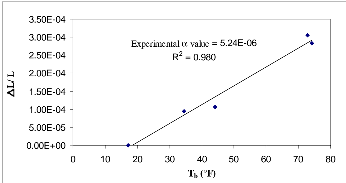
Figure 6.14 The experimental \alpha -value for Bridge 3 (0996.0R218)
