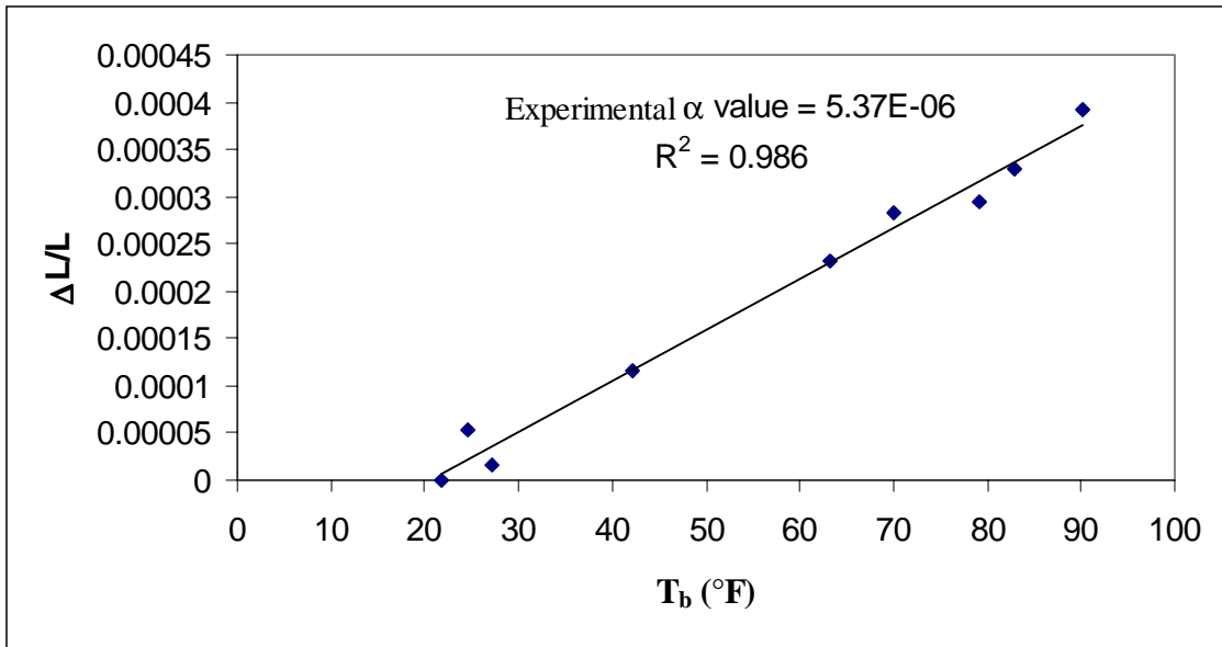
Figure 6.32 The experimental \alpha -value for Bridge 8 (7776.8L065)
