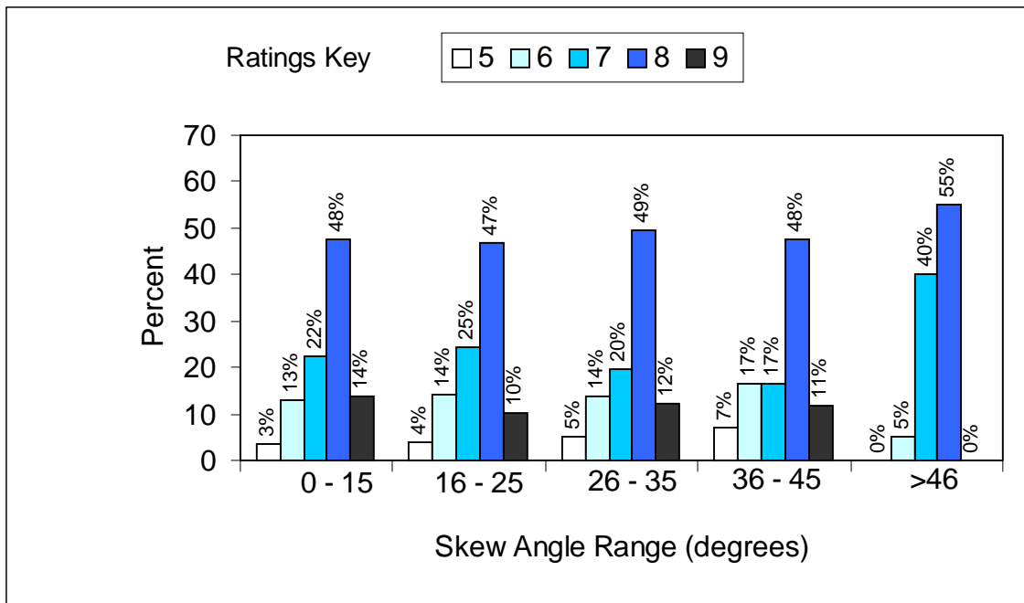
Figure 5.2 End deck joint strip seal rating versus skew angle of bridge
