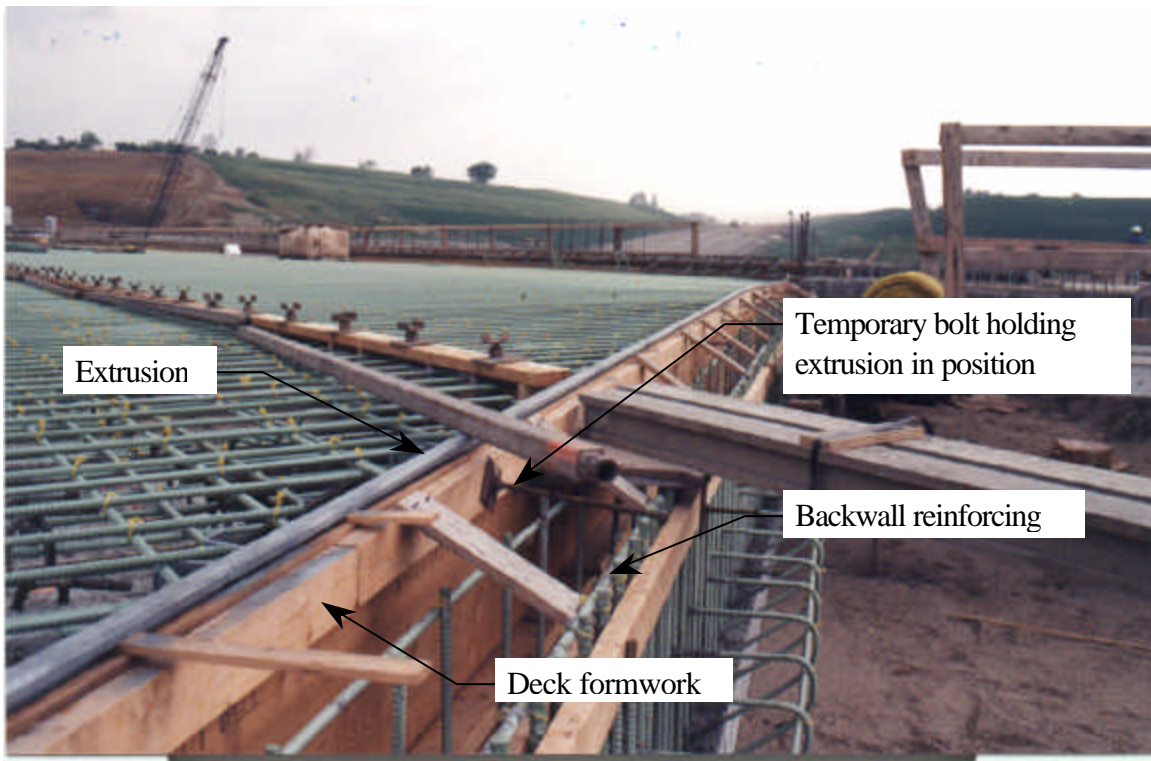
Figure 4.8 Extrusion at one end of deck installed from gutter to gutter
