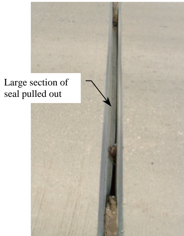
Figure 6.37 Strip seal at G2 for Bridge 10 (6402.0S014)
