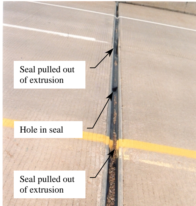
Figure 6.11 Strip seal at G3 for Bridge 3 (0996.0R218)
