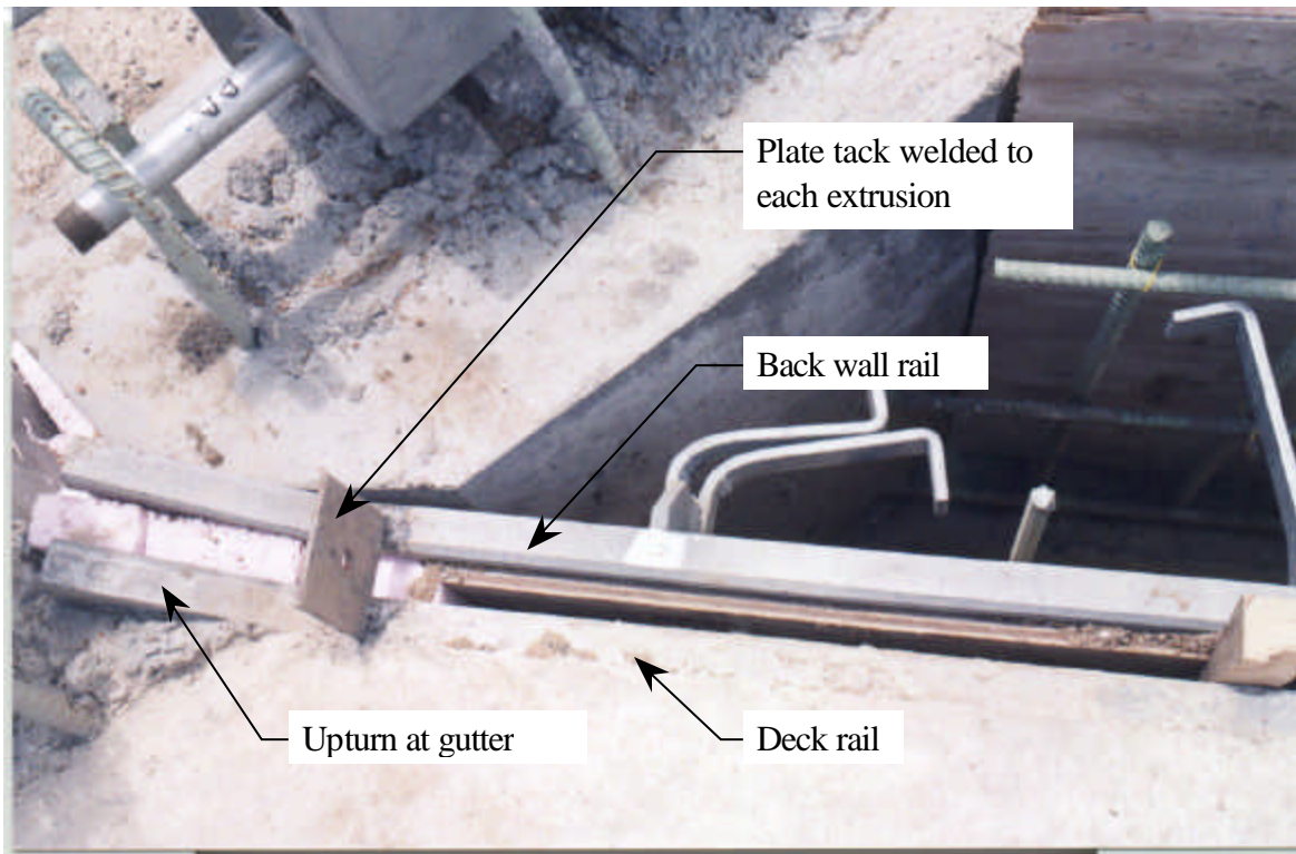
Figure 4.14 Small plates are tack welded to either extrusion to maintain gap
