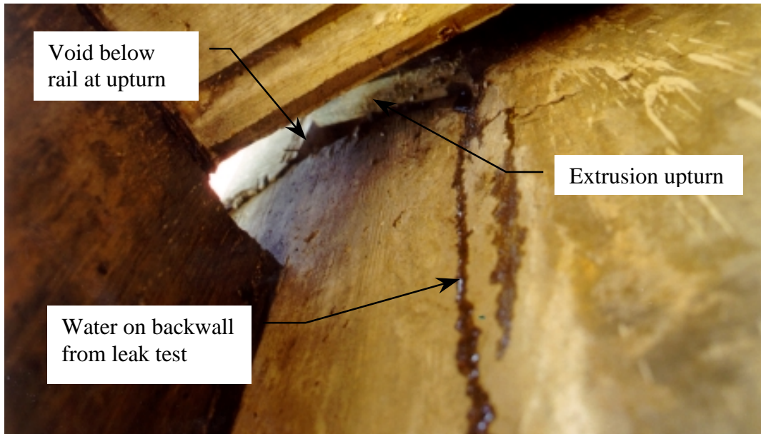
Figure 6.33 Leaking below the right gutter at G1 of Bridge 9 (6485.3L030)
