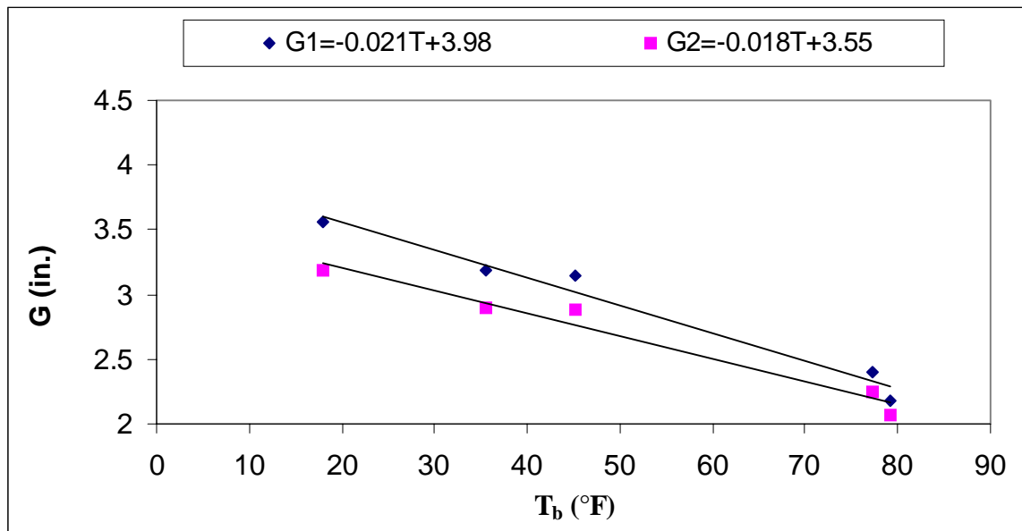
Figure 6.21 Gap opening vs. bridge temperature for Bridge 5 (0787.7A218)
