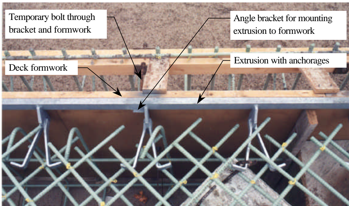
Figure 4.7 Rail section with anchorages positioned and bolted to deck formwork
