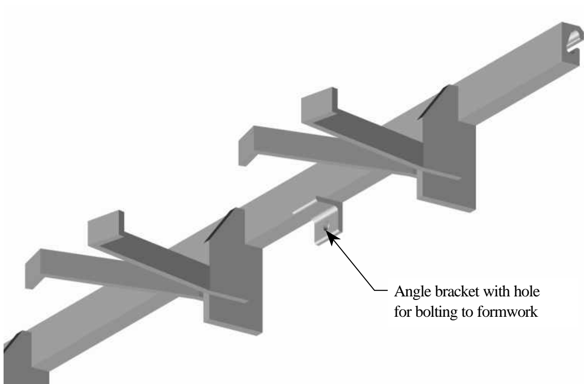
Figure 4.10 Model of extrusion with angle bracket for mounting welded to bottom surface
