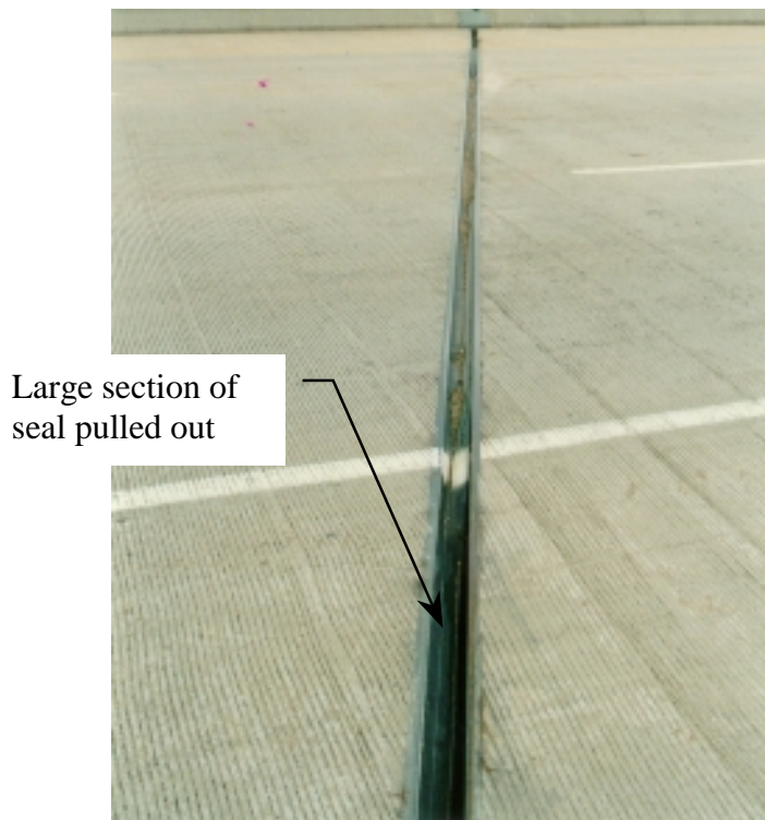
Figure 6.24 Strip seal at G2 of Bridge 6 (0784.8S218)
