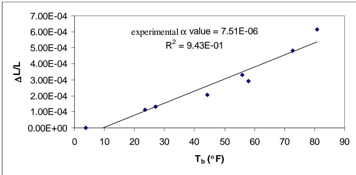
Figure 6.35 The experimental \alpha -value for Bridge 9 (6485.3L030)
