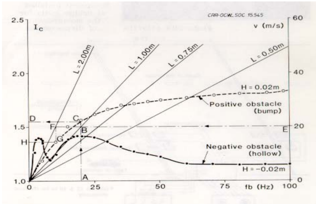
Figure 2.4 Determination of dynamic amplification factor (adapted from [22])
