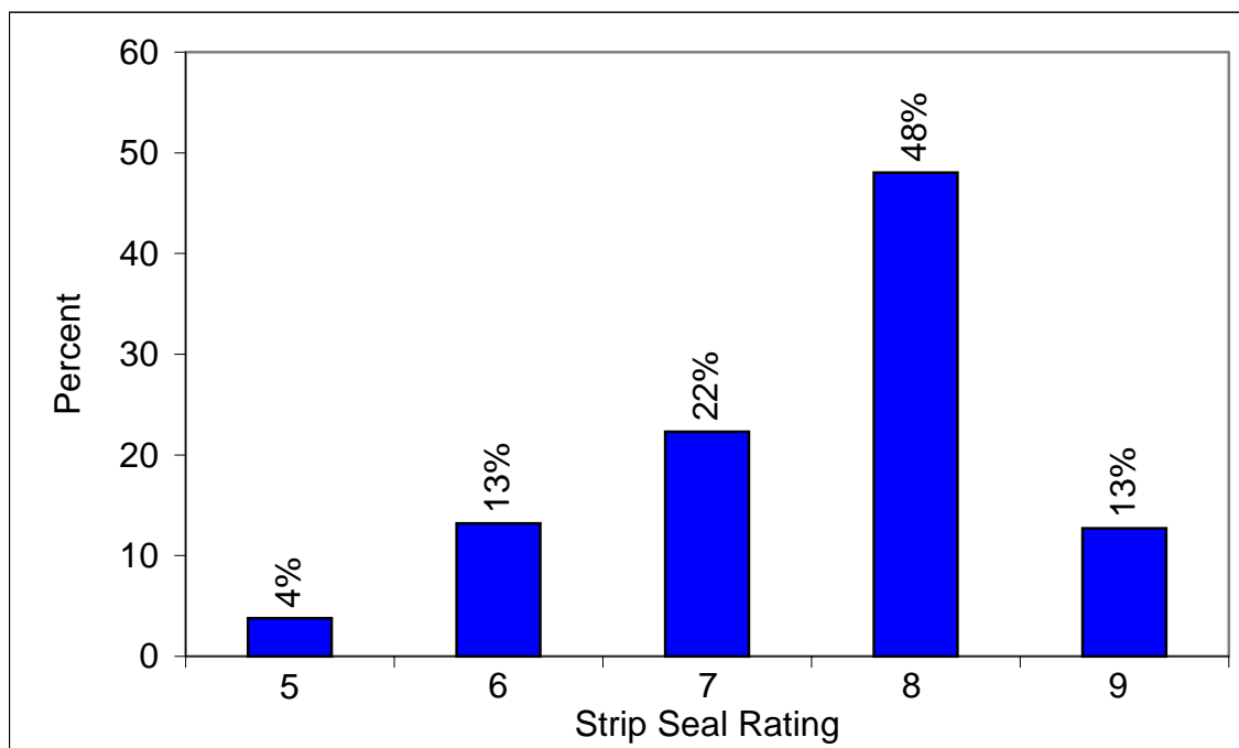
Figure 5.1 – Ratings of the end deck joint strip seals in Iowa bridges
