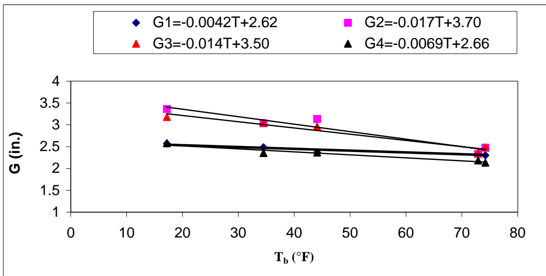
Figure 6.13 Gap openings vs. bridge temperature for Bridge 3 (0996.0R218)
