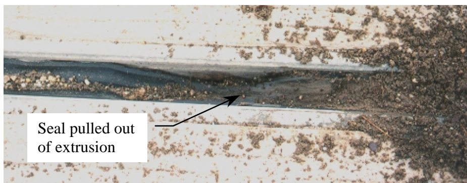
Figure 6.10 Strip seal at G2 for Bridge 3 (0996.0R218)
