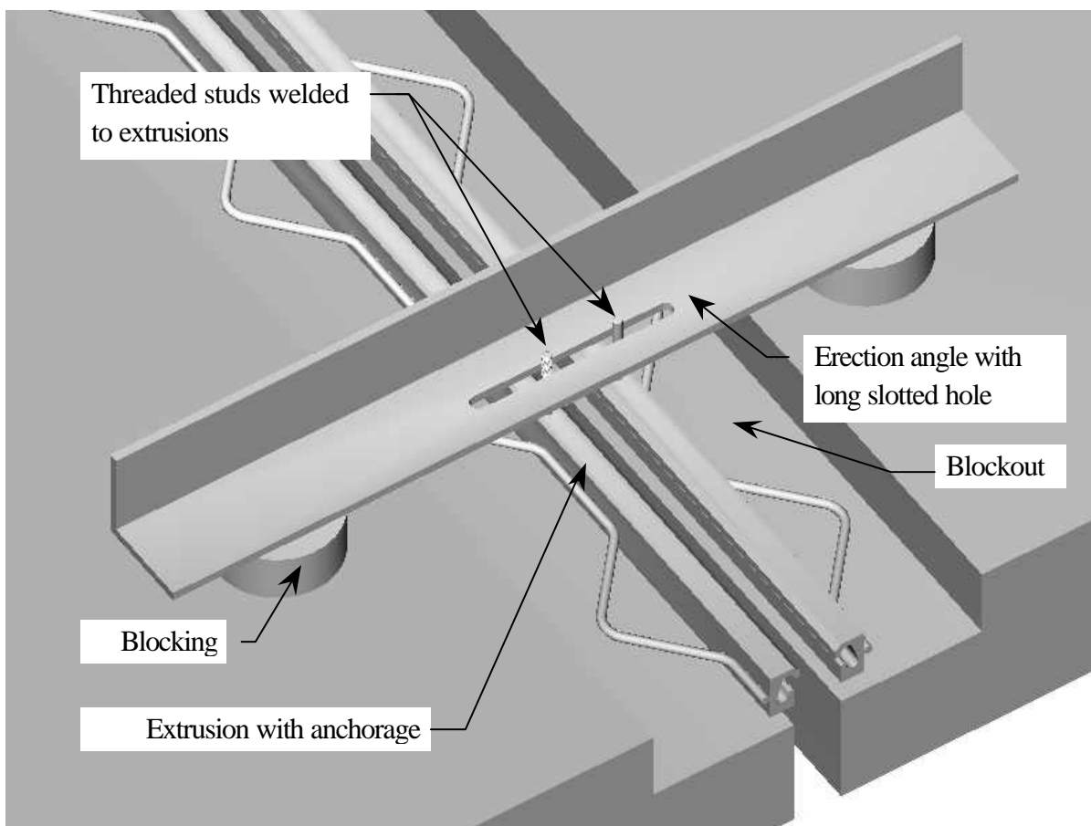
Figure 4.1 Computer model of extrusions positioned in blockouts using an erection angle
