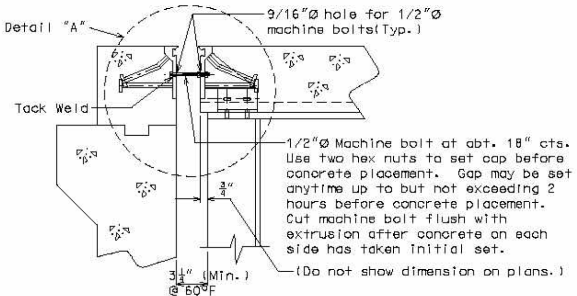
Figure 4.4 Mechanism used in Missouri for setting the gap with P-type extrusions
