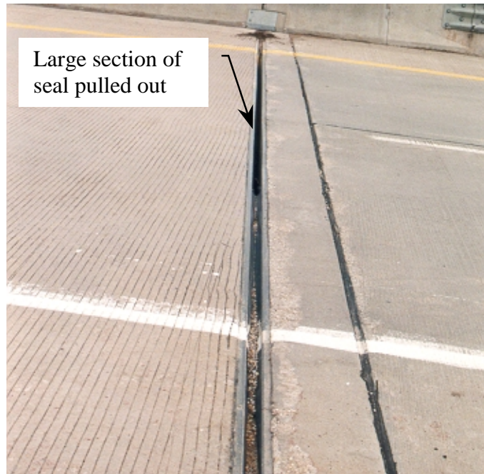
Figure 6.12 Strip seal at G4 for Bridge 3 (0996.0R218)
