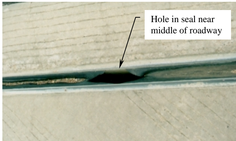
Figure 6.19 Strip seal at G1 for Bridge 5 (0787.7A218)
