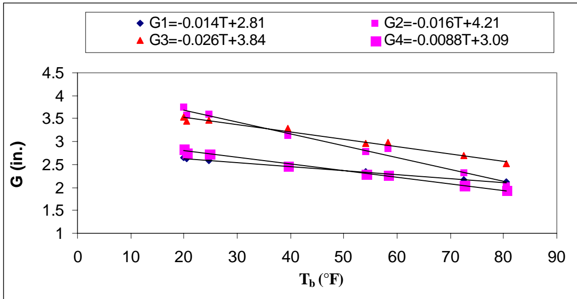
Figure 6.39 Gap openings vs. bridge temperature for Bridge 10 (6402.0S014)
