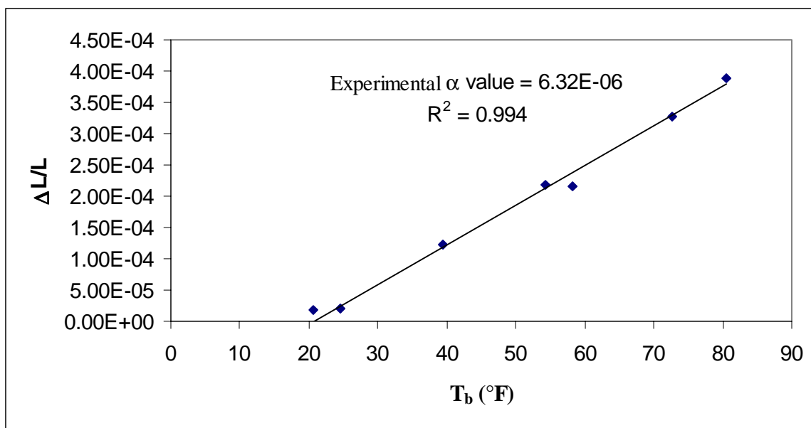
Figure 6.40 The experimental \alpha -value for Bridge 10 (6402.OS014)
