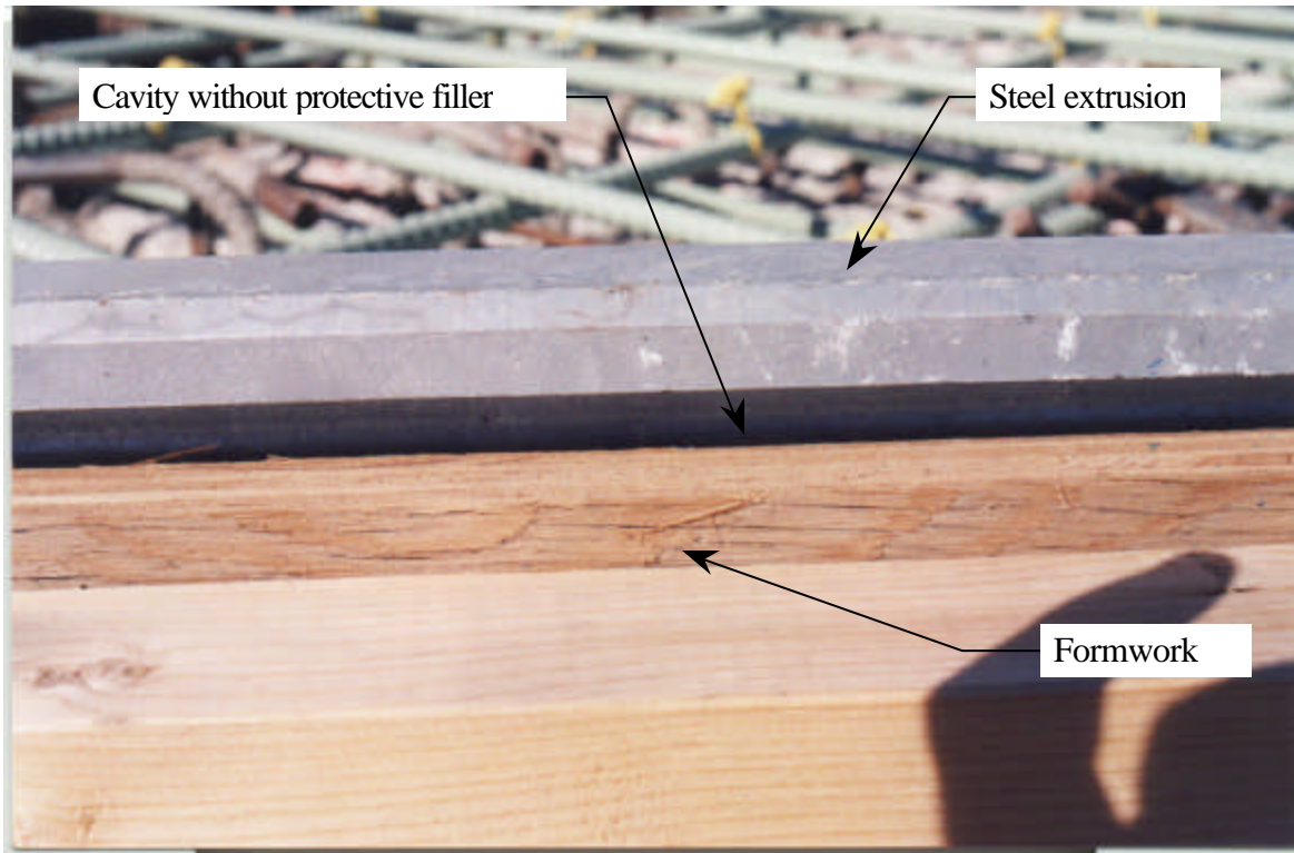
Figure 4.12 No sacrificial filler was present in the cavity on the east end of the deck
