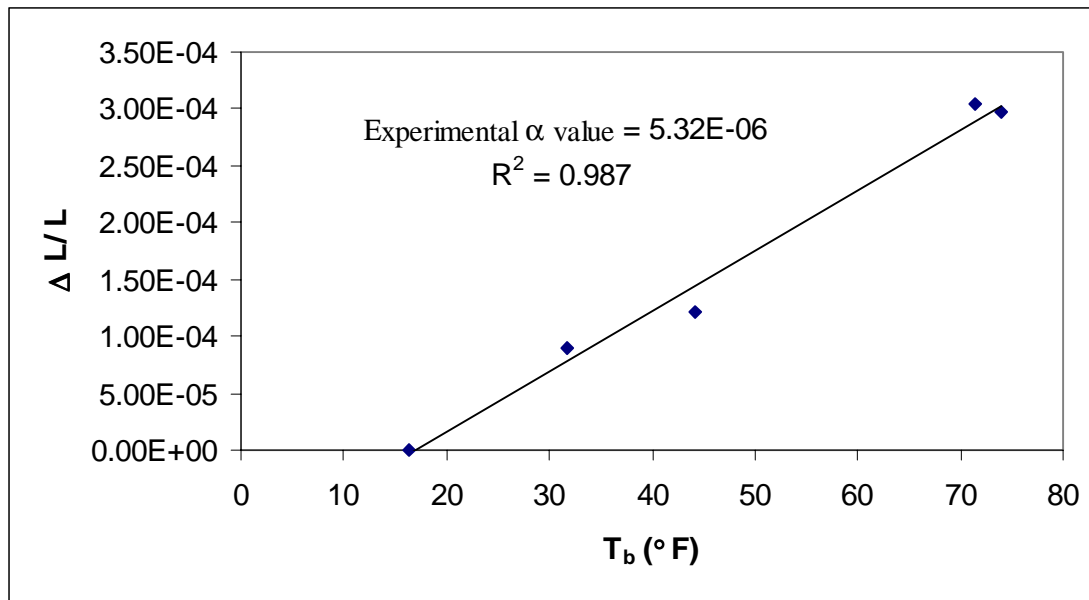
Figure 6.6 The experimental \alpha -value for Bridge 1 (0781.1R218)
