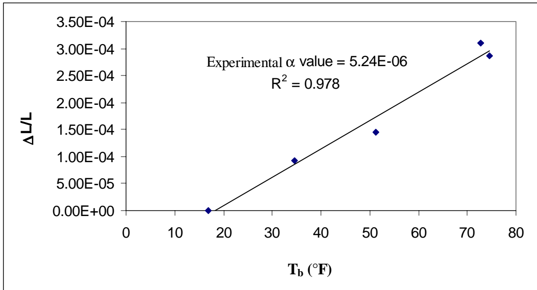
Figure 6.18 The experimental \alpha -value for Bridge 4 (0996.0L218)At a shade
