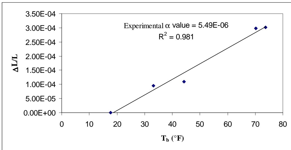
Figure 6.26 The experimental \alpha -value for Bridge 6 (0784.8S218)
