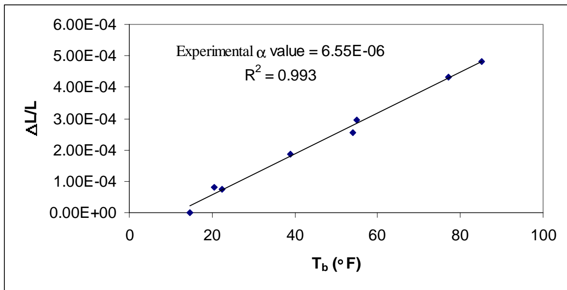
Figure 6.43 The experimental \alpha -value for Bridge 11 (6403.6L014)
