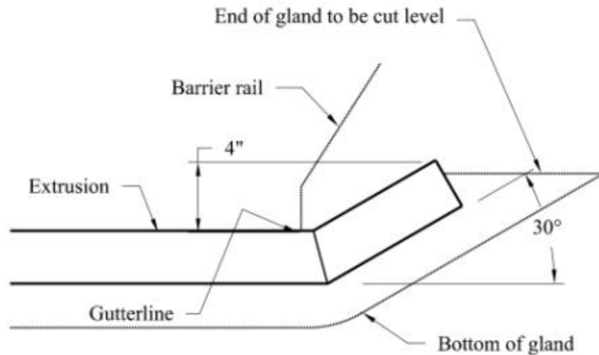
Figure 3.3 The one-step upturn end detail used in Iowa.
