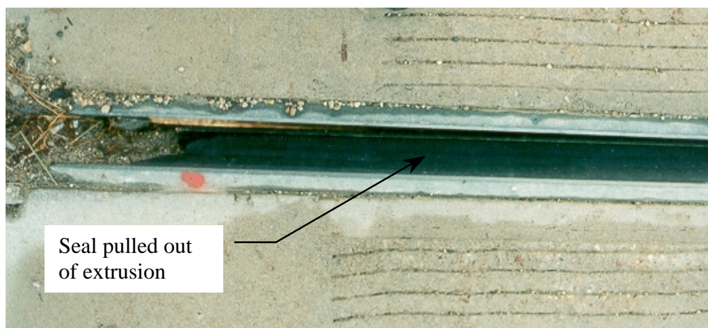
Figure 6.16 Strip seal at G3 for Bridge 4 (0996.0L218)
