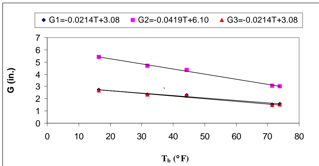
Figure 6.5 Gap openings vs. bridge temperature for Bridge 1 (0781.1R218)
