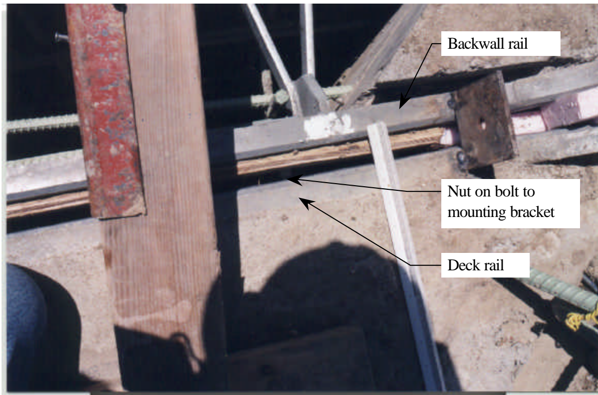
Figure 4.17 There is typically little room to work between the pair of extrusions
