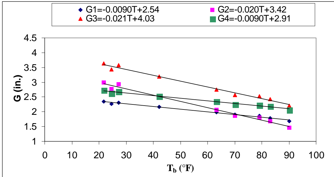
Figure 6.31 Gap opening vs. bridge temperature for Bridge 8 (7776.8L065)
