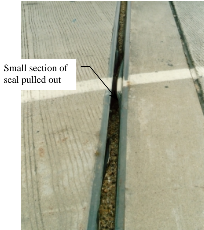
Figure 6.23 Strip seal at G1 of Bridge 6 (0784.8S218)
