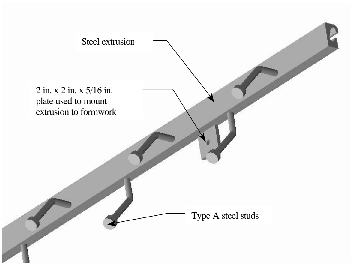
Figure 3.2 Typical configuration of steel extrusions as used in South Dakota.
