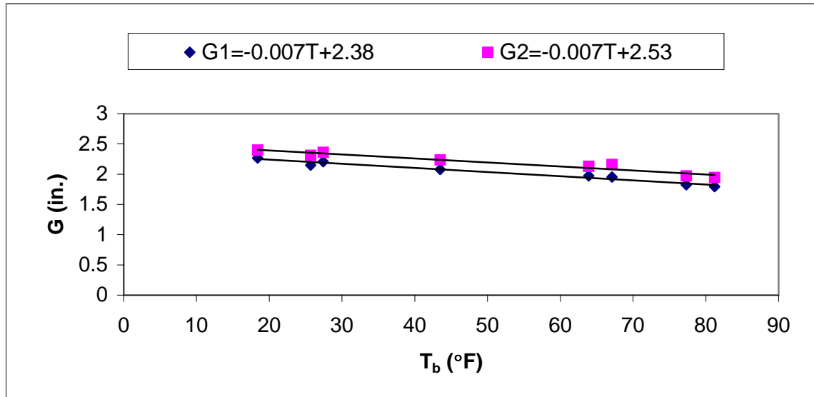
Figure 6.44 Gap opening vs. bridge temperature for Bridge 12 (6481.9L030)
