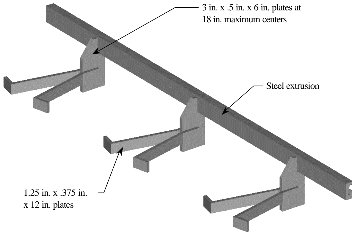
Figure 4.5 Model of the extrusion with anchorages of the type used in Iowa
