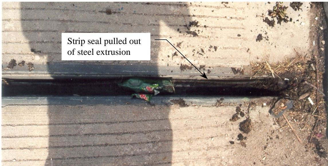
Figure 6.4 Strip seal at G2 for Bridge 1 (0781.1R218)
