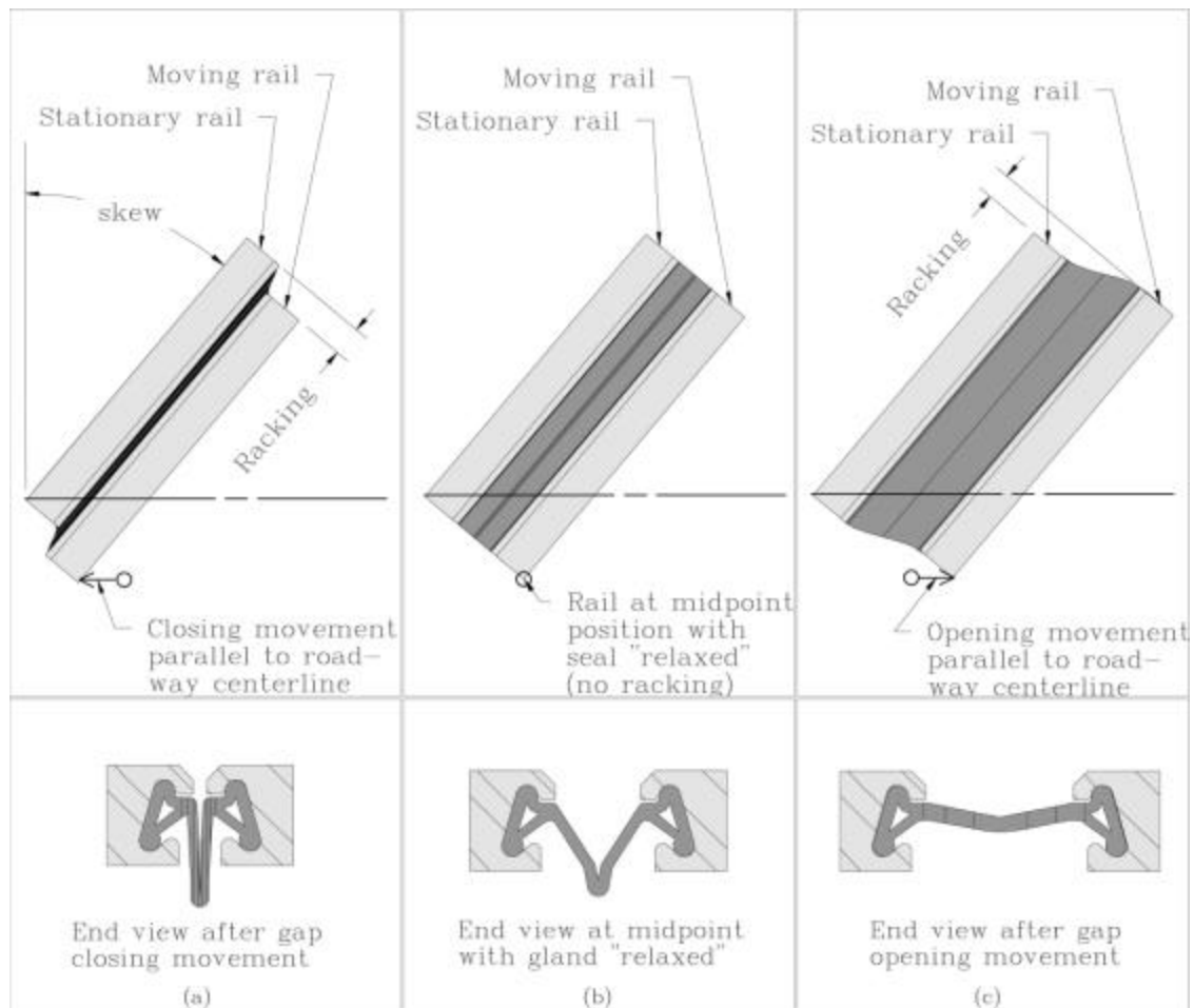
FIGURE 3.4 For large skew angles, movement includes a significant racking component which decreases the effective movement range of the neoprene gland.
