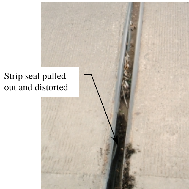
Figure 6.38 Strip seal at G3 for Bridge 10 (6402.0S014)
