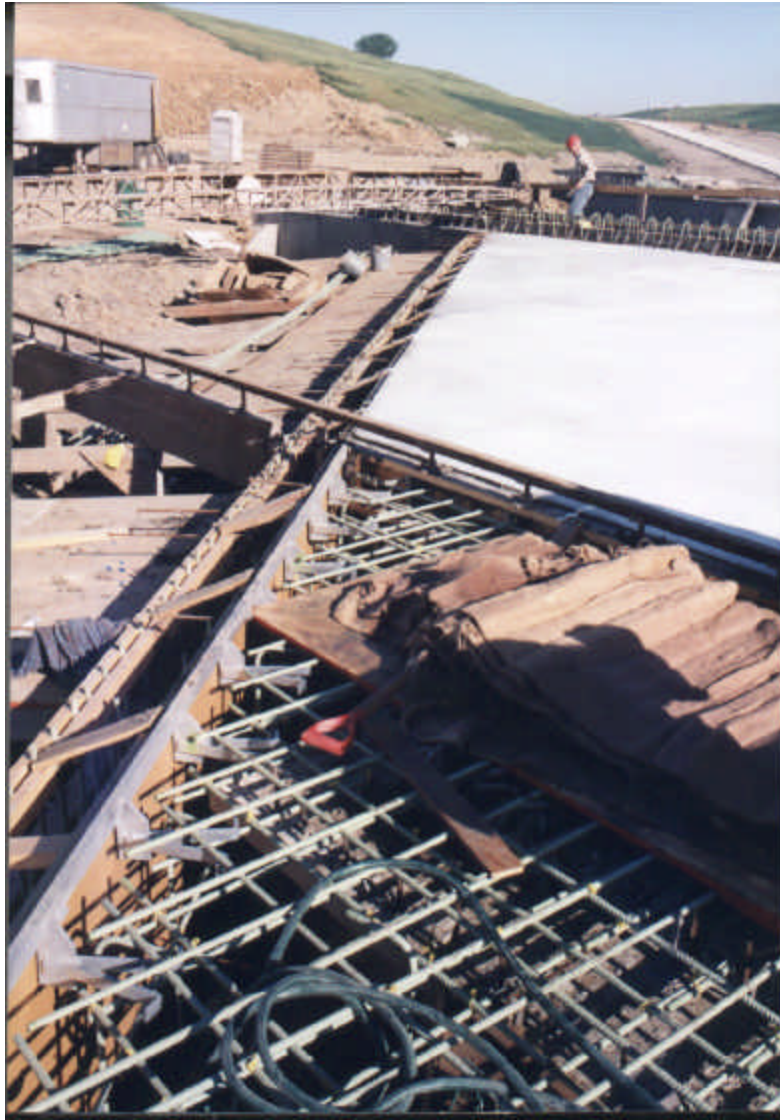
Figure 4.13 North portion of extrusion embedded in concrete
