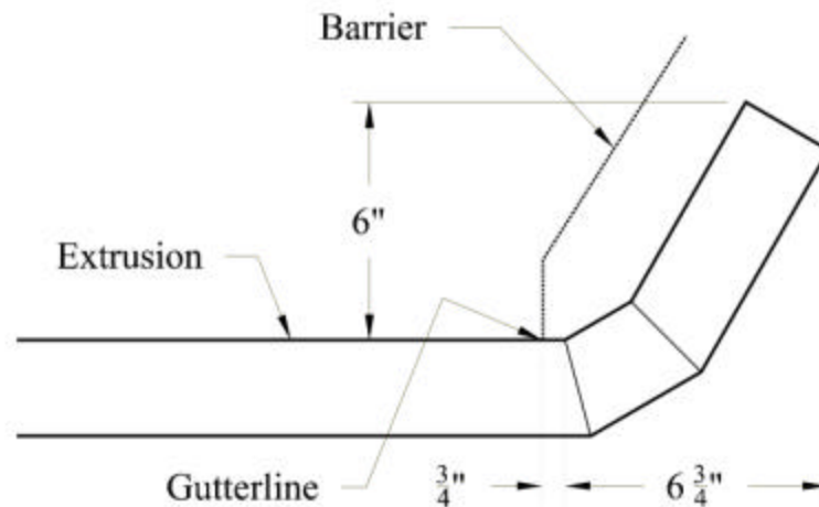
Figure 3.1 A two-step upturn end detail used in Minnesota and Wisconsin. Adopted by Iowa in 2000.
