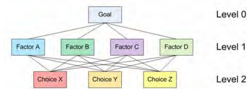
Figure 3.3: A schematic three-level decision making hierarchy
