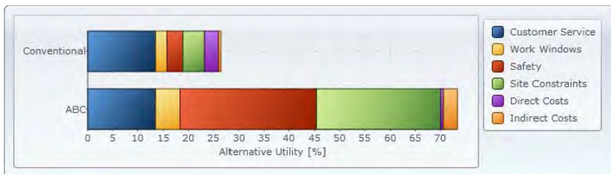
Figure 3.2: Example AHP analysis for Gainesville project
