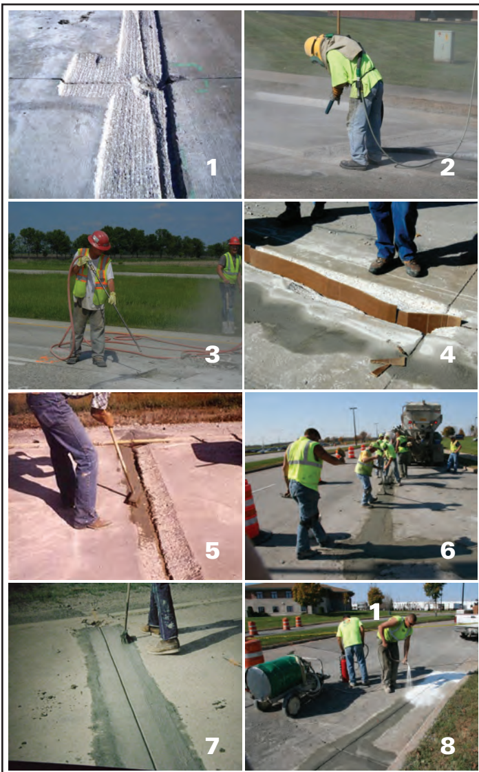
Figure 39. Steps to conducting a proper partial-depth repair (Source: Snyder and Associates)
