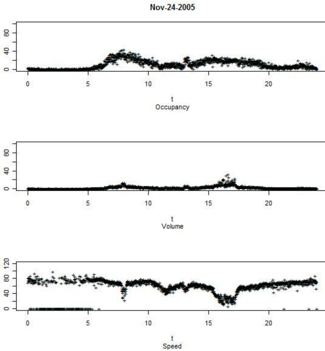
Figure 3. Occupancy, Volume, and Speed Data for Nov. 23, 2005 for the Sensor Northbound from the One in Figure 2.
