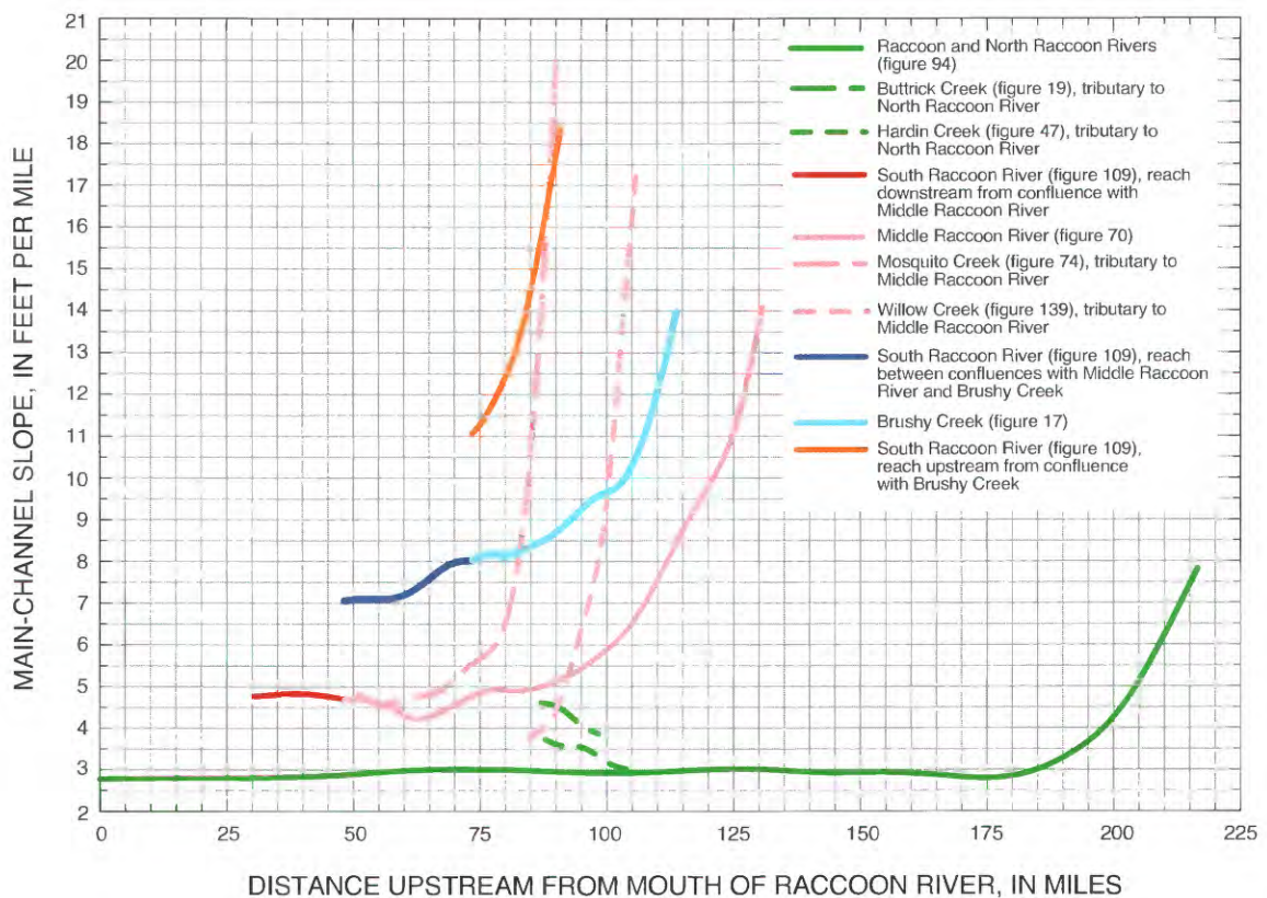
Figure 5. Main-channel-slope curves of selected streams in the Raccoon River Basin.
