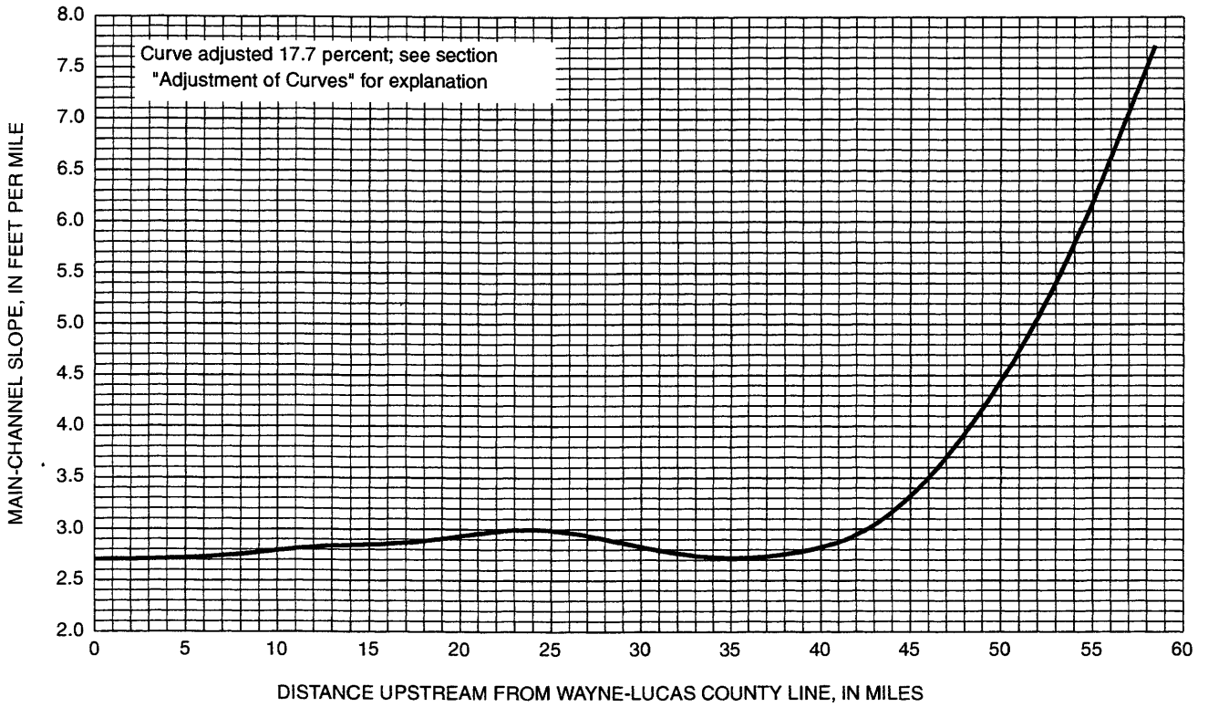
Figure 23. Chariton River, beginning at Wayne-Lucas County line.
