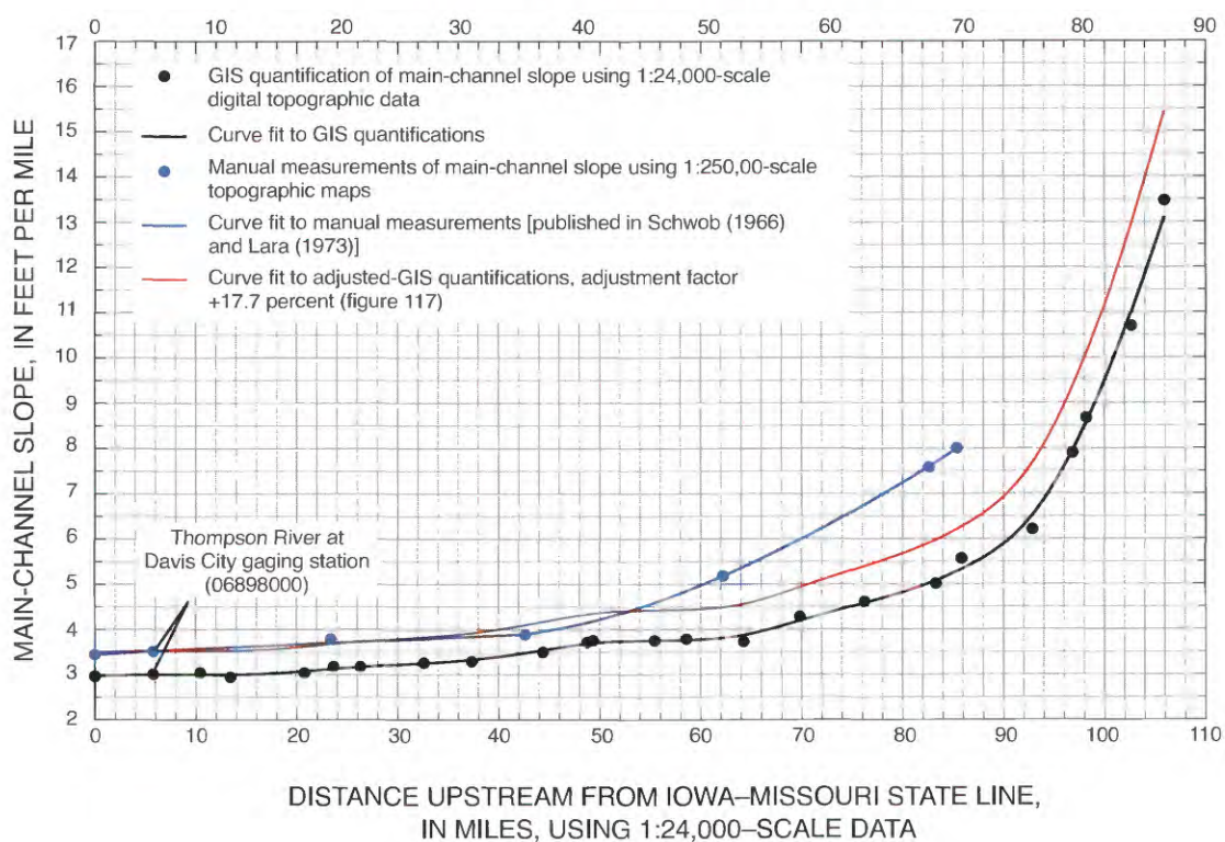
Figure 4. Examples of curves developed using main-channel-slope values determined from manual measurements, GIS quantifications, and adjusted-GIS quantifications.
