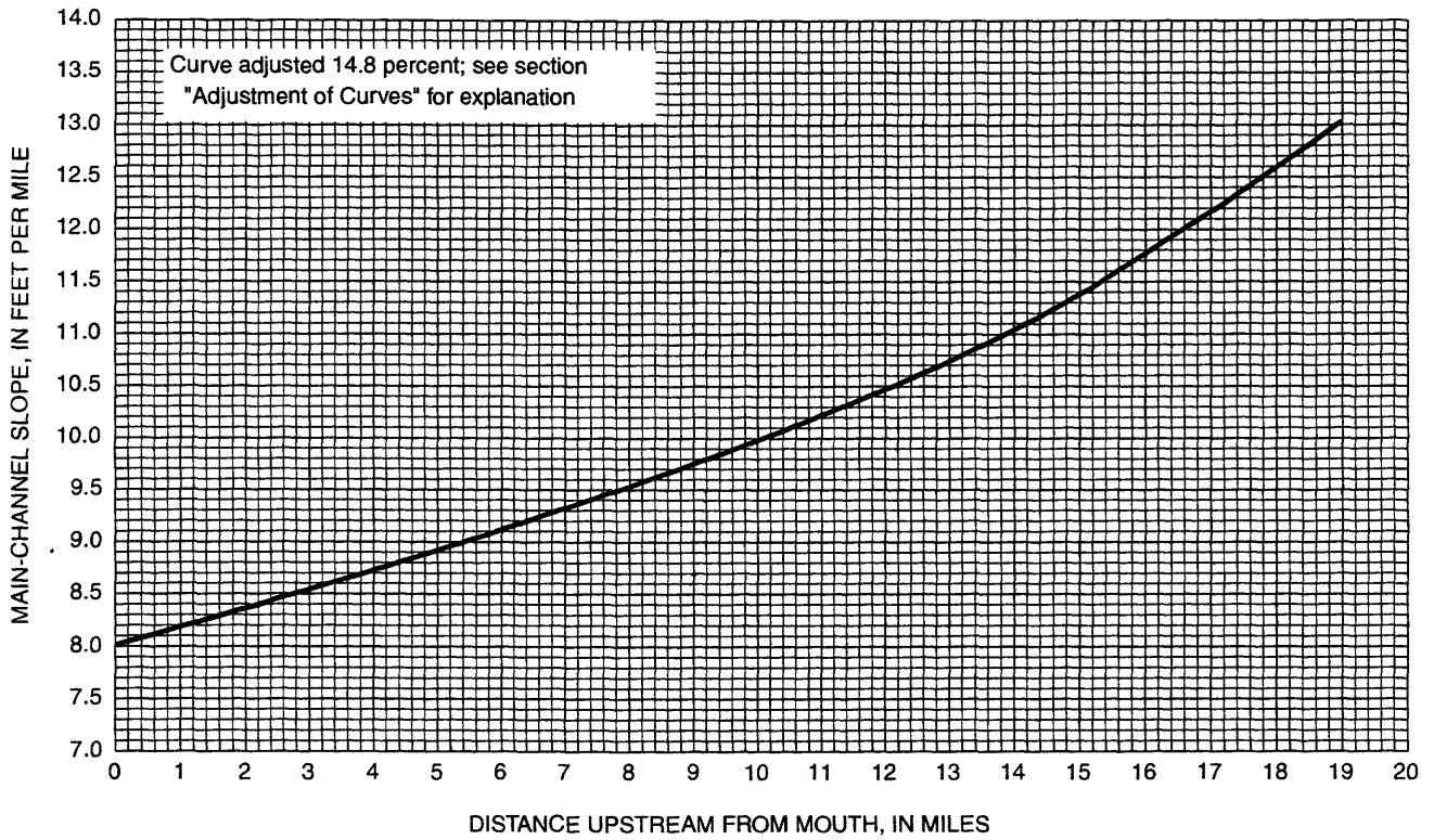
Figure 88. Otter Creek, beginning at mouth in Buchanan County.
