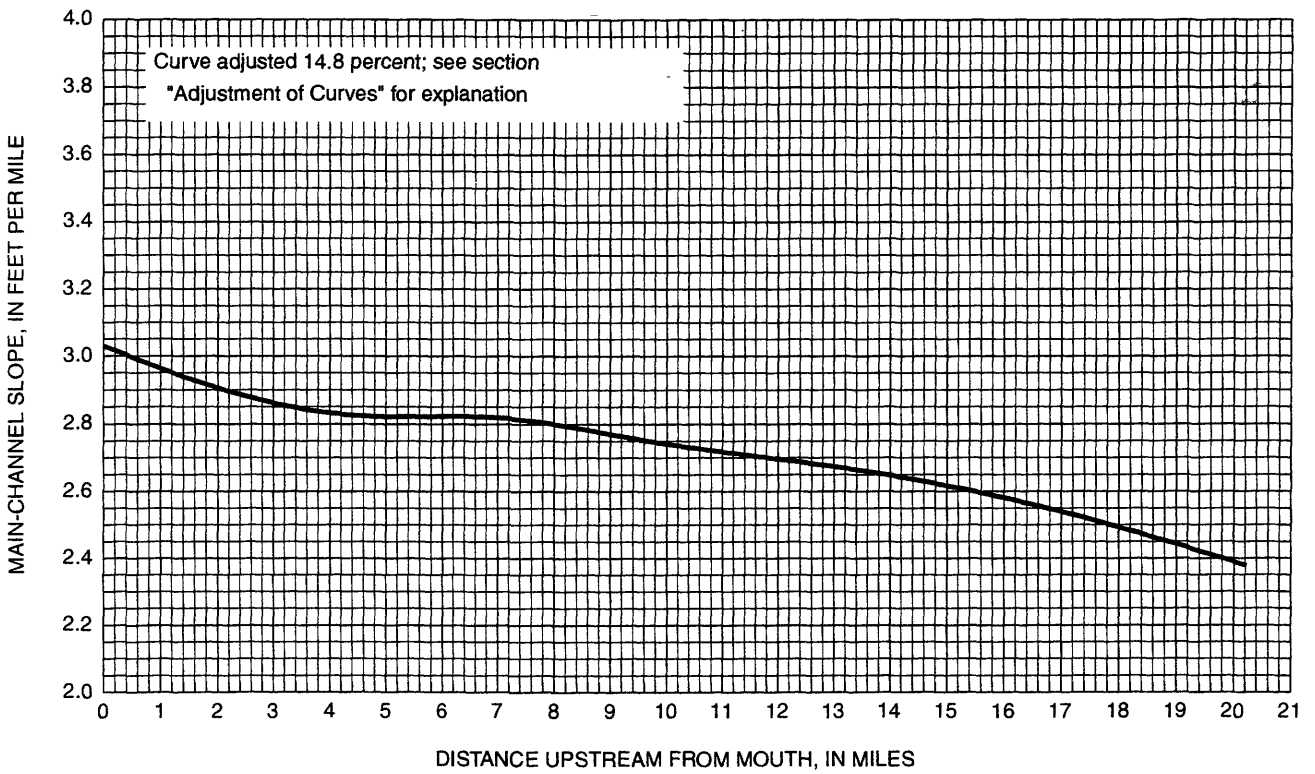
Figure 142. Winnebago River, beginning at mouth in Floyd County.
