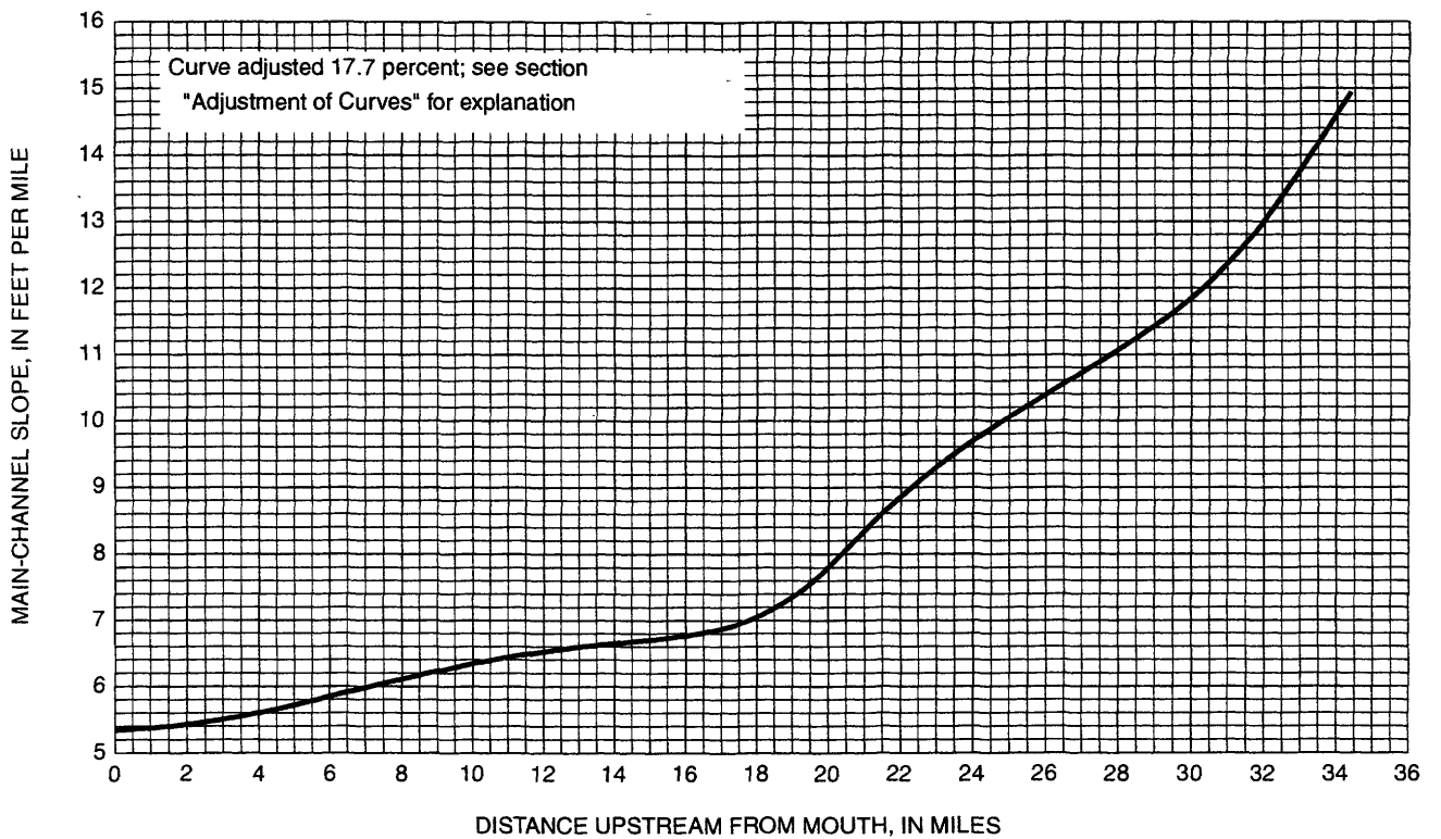
Figure 38. English Creek, beginning at mouth in Marion County.
