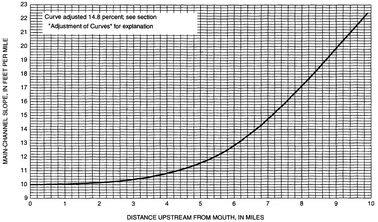
Figure 40. Farm Creek, beginning at mouth in Mills County.
