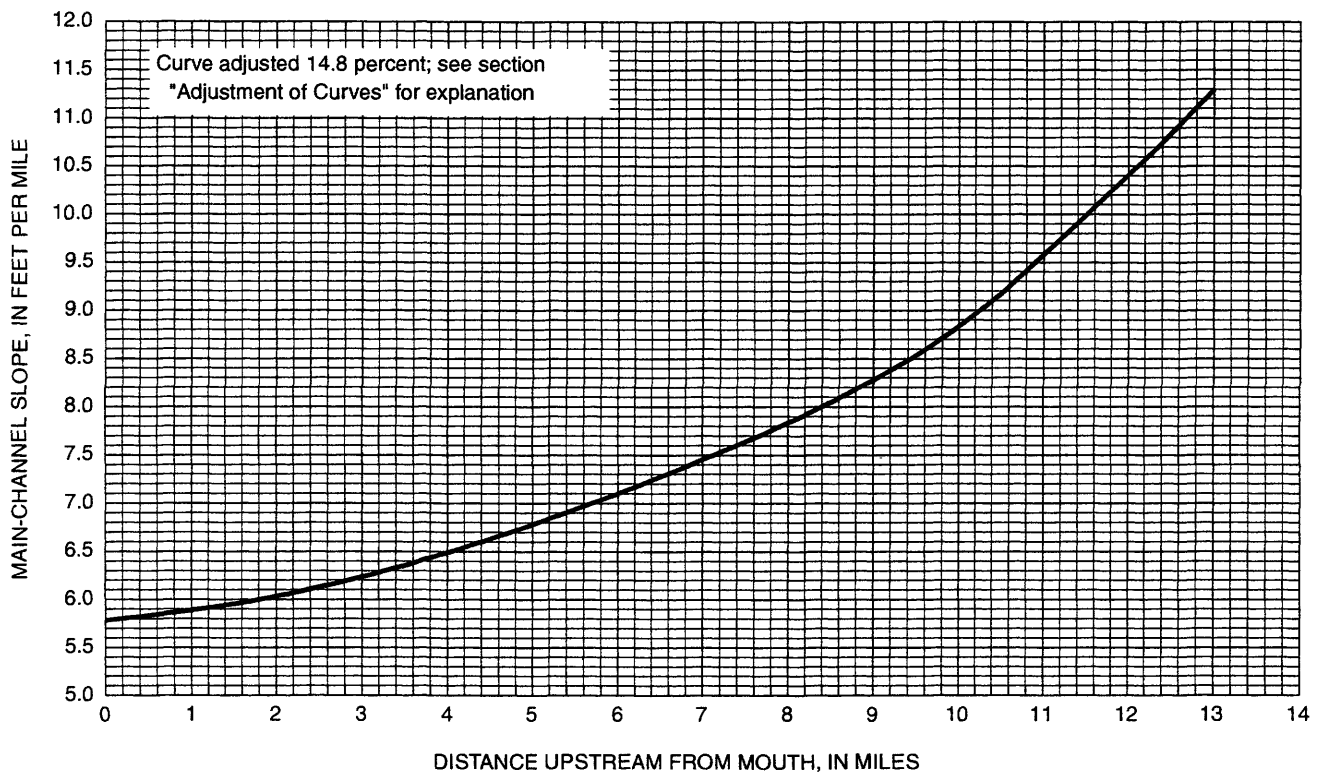
Figure 78. Mud Creek, beginning at mouth in Scott County.
