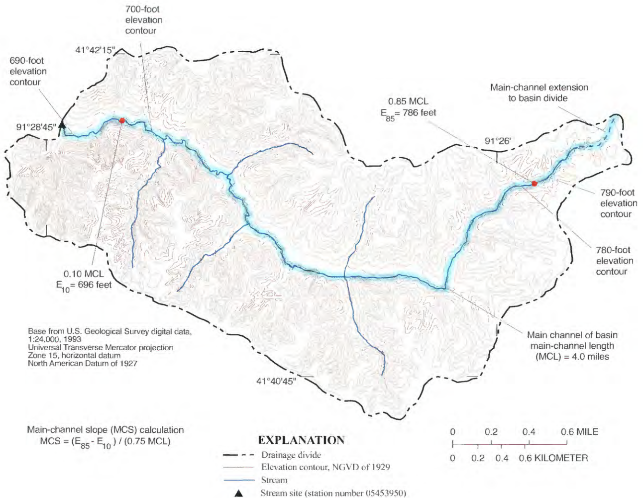
Figure 3. Topographic-map measurements for calculating main-channel slope (from Eash, 2001, figure 17).
