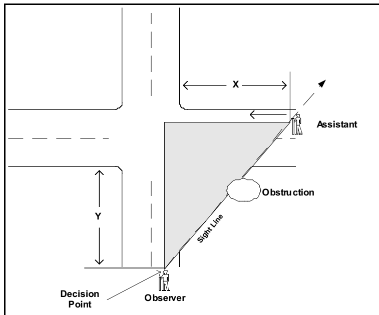
Figure 4.6. Sight Distance Measurement at Uncontrolled Intersection
