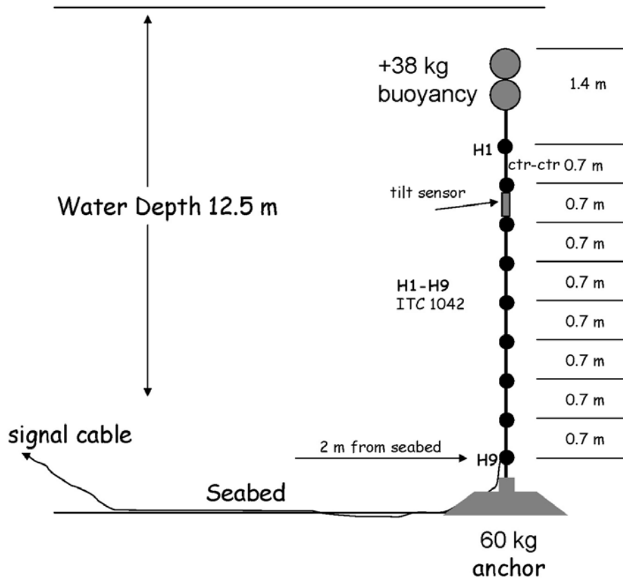
Figure 5. Vertical line array used for measuring underwater acoustic radiation from impact installation pile driving
