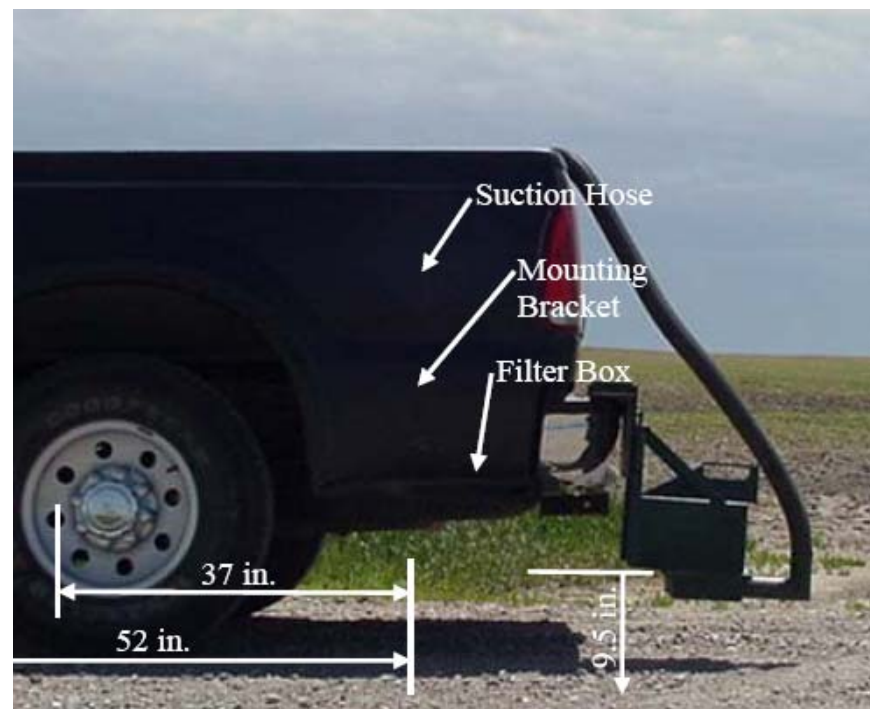
Mounted Dustometer
