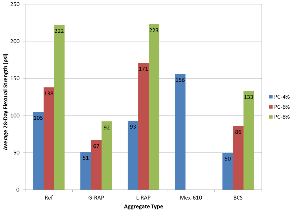
Figure 19 Comparison of the average 28-day flexural strength results for mixtures containing portland cement
