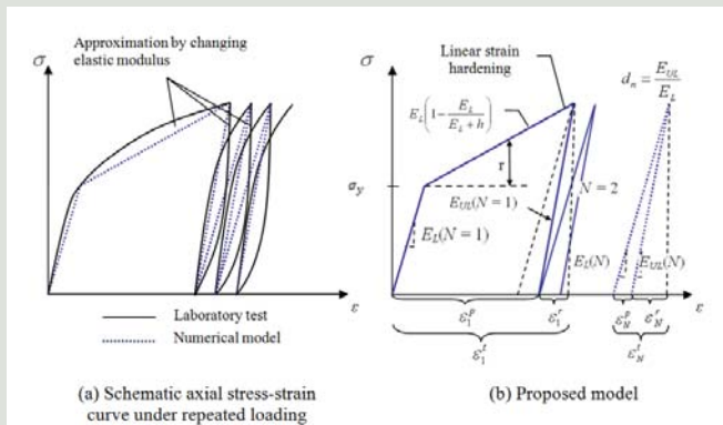
Figure 1. Concept of the proposed P-D model
