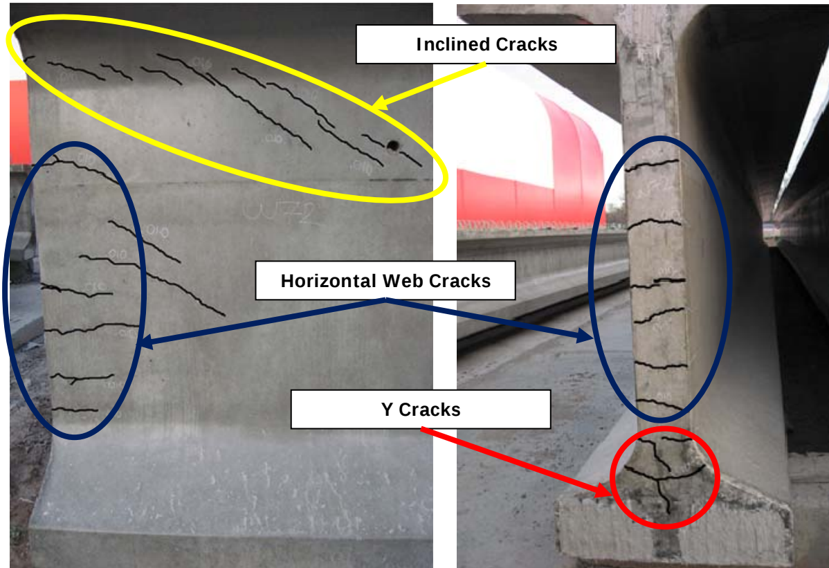
Figure 4 - Typical inclined, web and Y cracks marked on a 72W girder.
