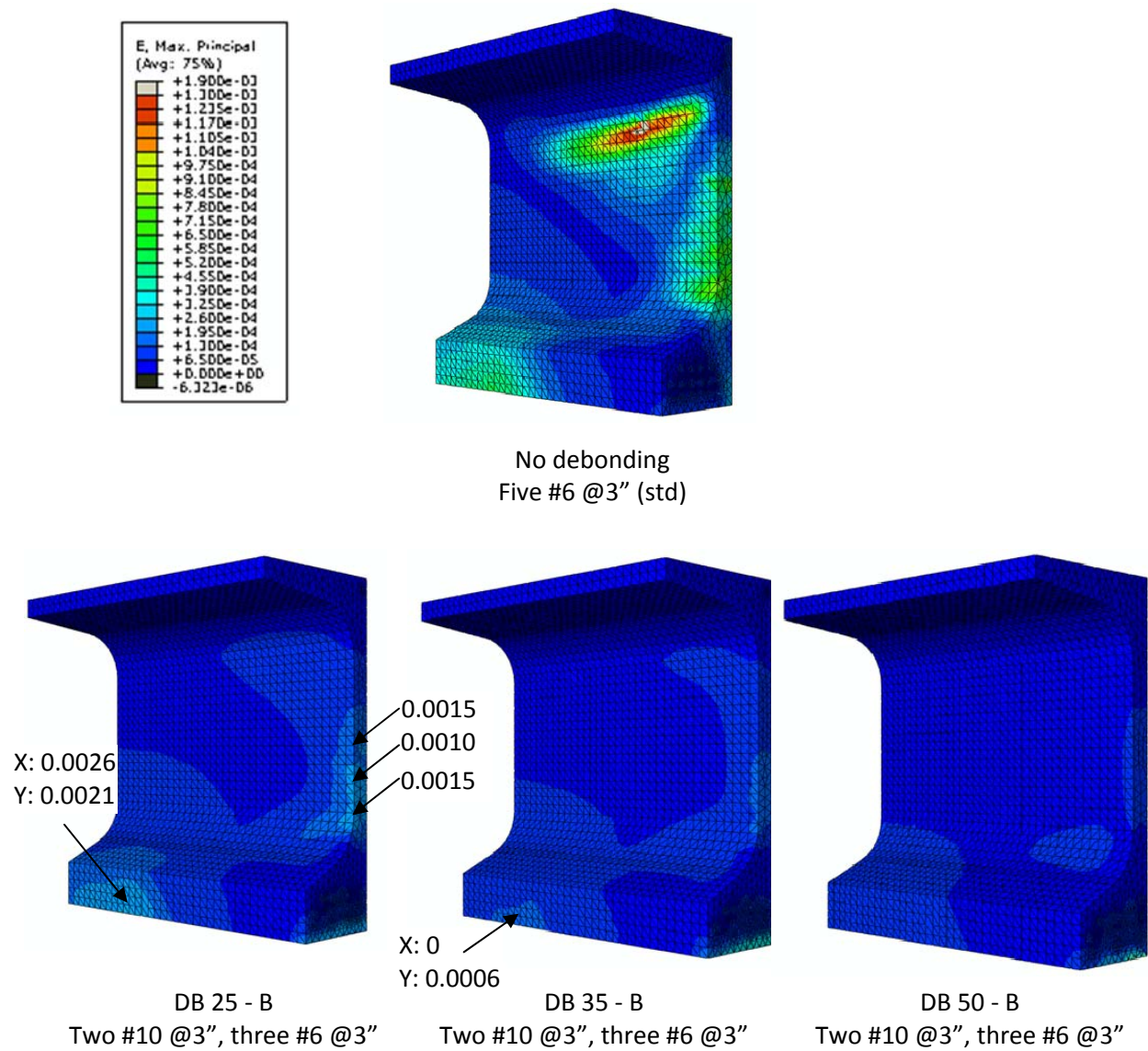
Figure 79 – Principal concrete tension strain contour plots and crack widths for the combination cases as compared to the standard detailed girder.
