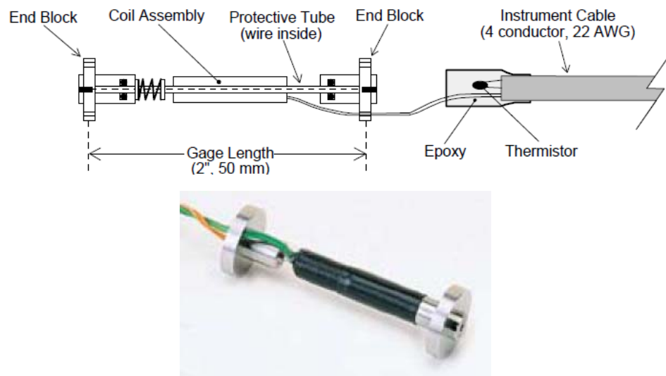
Figure 17 – Vibrating wire strain gages (Geokon 2010).
