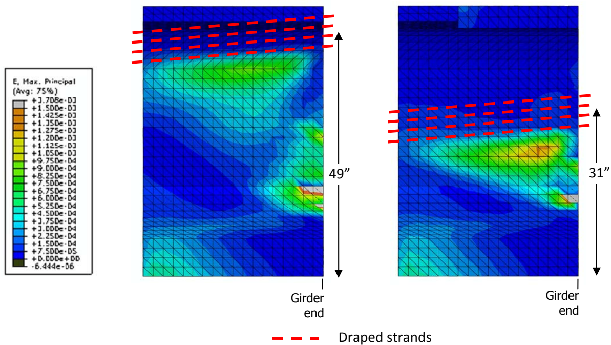
Figure 95 - Principal tensile stress contour plots on the elevation view of the two cases with high (left) and low (right) draped strands. (resultant eccentricities are listed)
