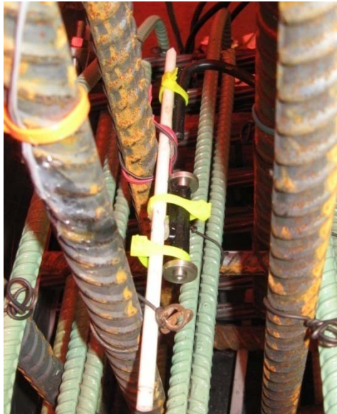
Figure 33 – 2in vibrating wire gage positioned in concrete through nonstructural attachments to rebar.
