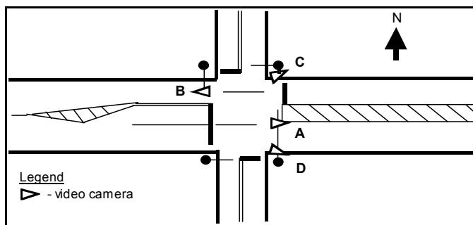
a. Optimal Camera Locations.
