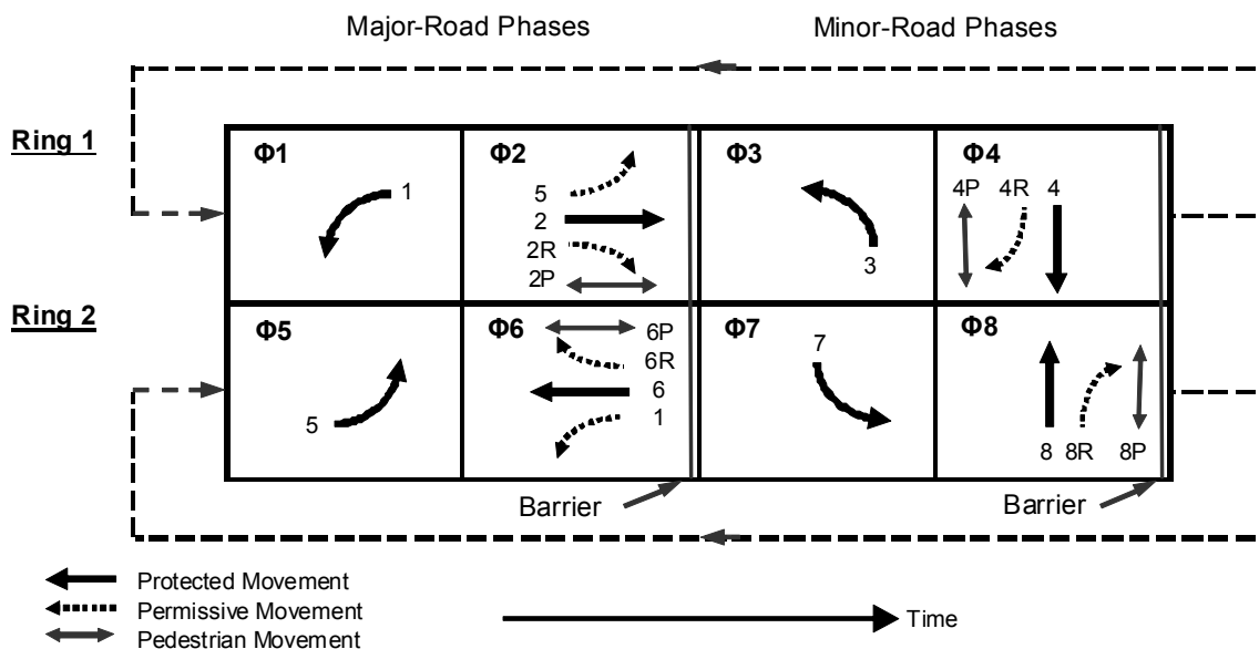
Figure 2-2. Dual-Ring Structure with Illustrative Movement Assignments.
