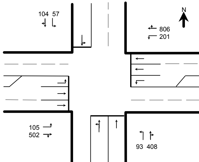
Figure E-1. Example Intersection Used to Illustrate Pedestrian Treatment Evaluation.
