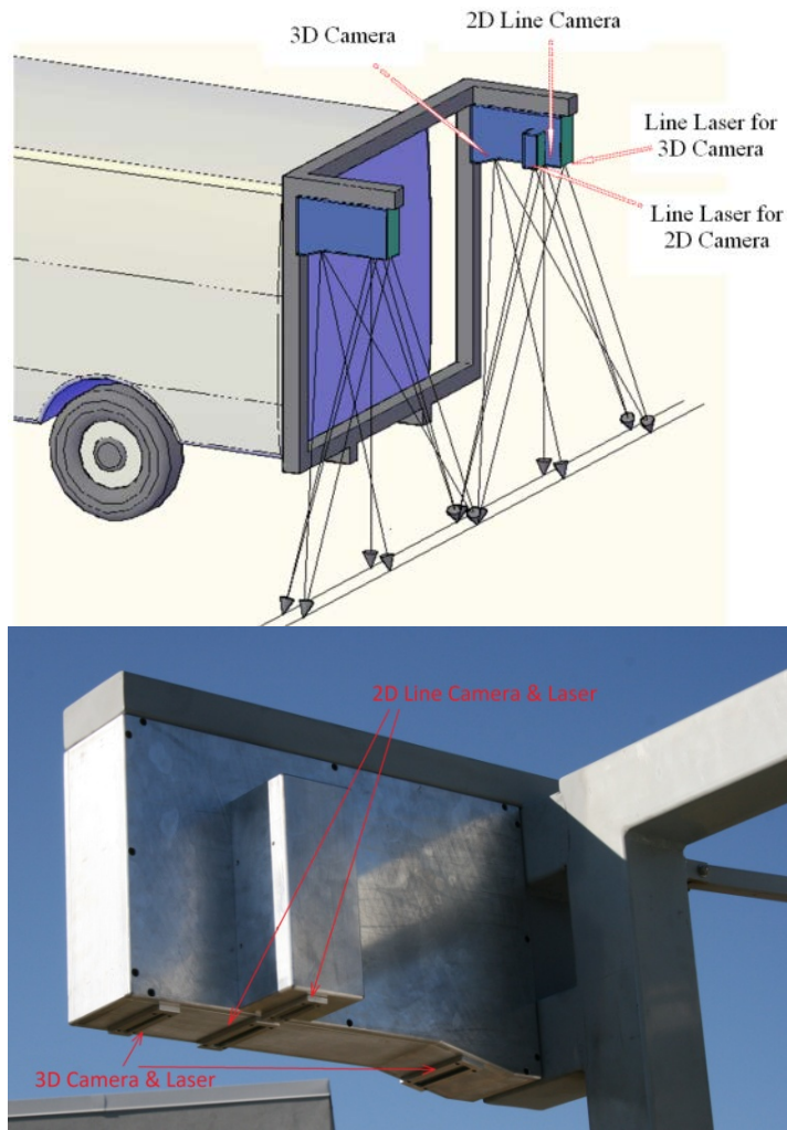
Figure 8. Sensor System Configuration (top) & a Laser Imaging Sensor (bottom)
