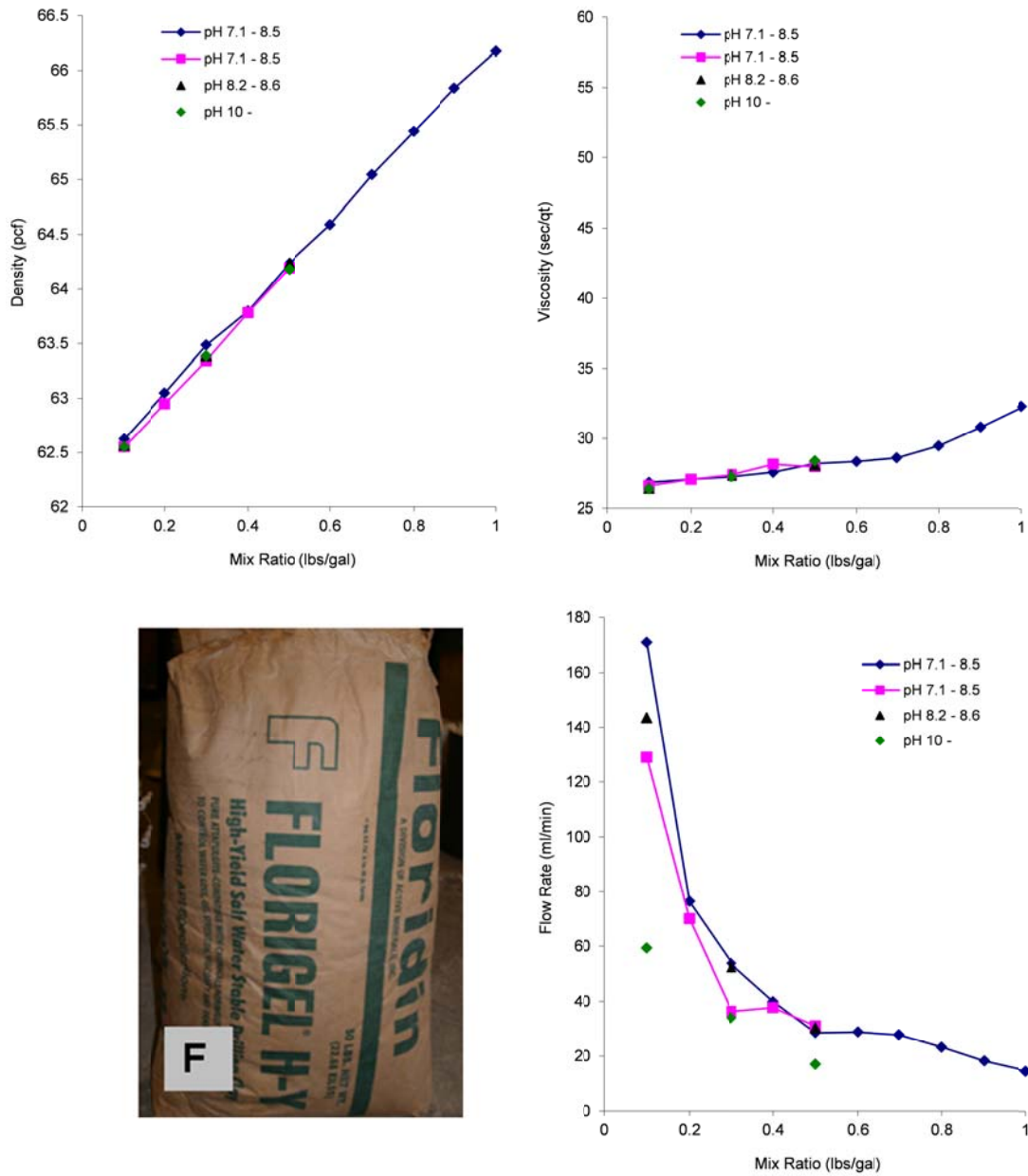
Figure 3.12 Florigel High Yield slurry testing results.
