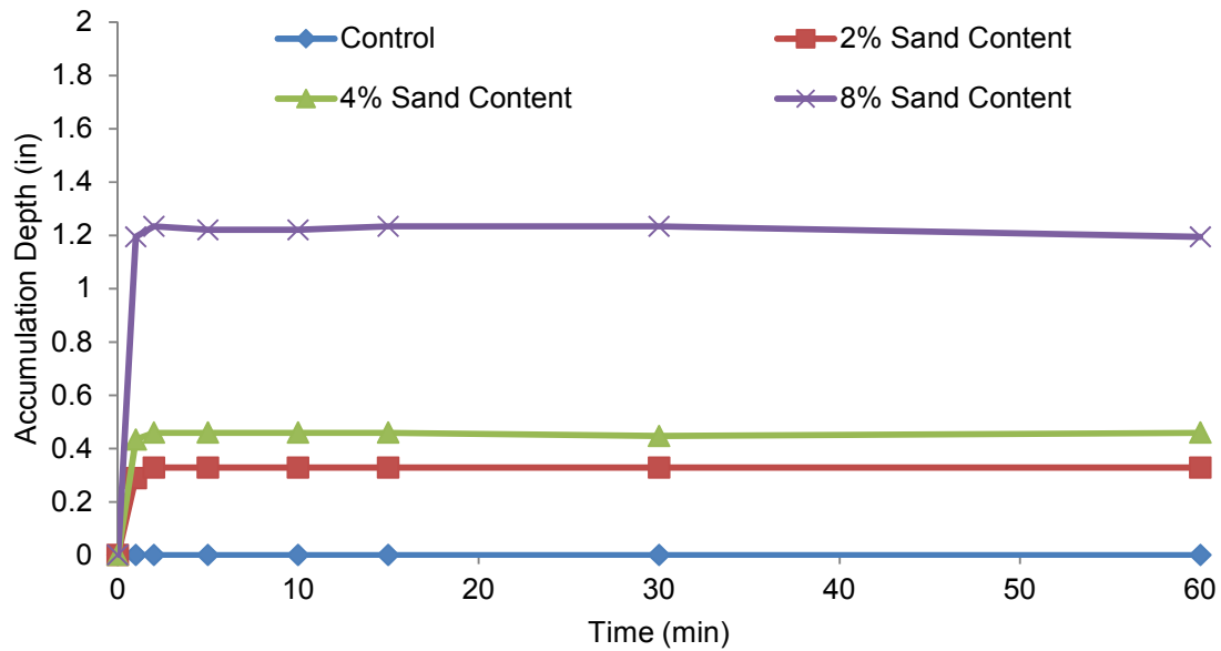
Figure 4.71 Sediment accumulation in 0.25 lb/100 gal Wyo-Vis DP.
