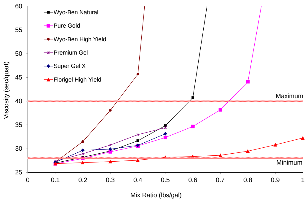
Figure 3.14 Viscosity versus mix ratio comparison of each product.
