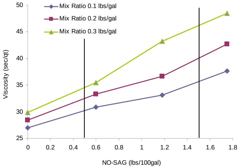
Figure 3.28 Effect of NO-SAG on viscosity for a pure bentonite product.
