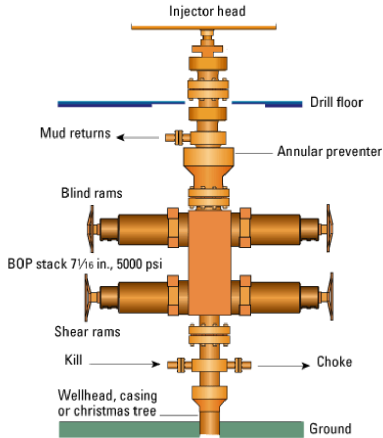
Figure 2.4 Blowout preventer (Schlumberger Limited, 2011).
