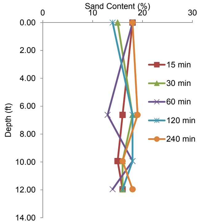
Figure 4.19 Measured sand content versus depth (16.25% overall starting sand content).
