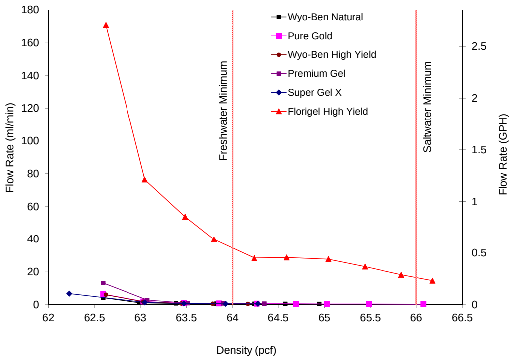
Figure 3.15 Flow rate versus density comparison of each product.
