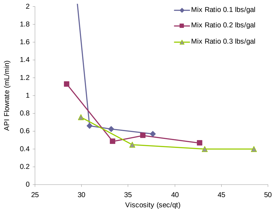
Figure 3.30 API Filter test flow rate versus viscosity for pure bentonite modified with NO-SAG.
