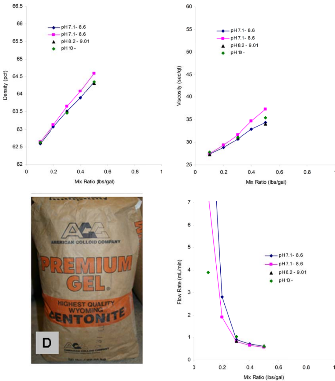
Figure 3.10 Premium Gel slurry testing results.
