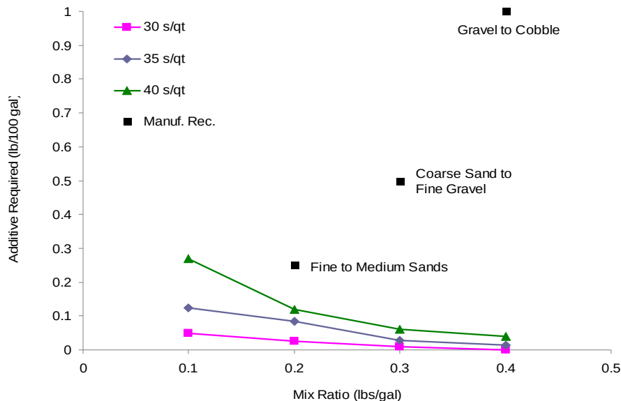
Figure 5.12 Amount of Wyo-Vis “DP” required to produce a desired viscosity for pure bentonite slurry.
