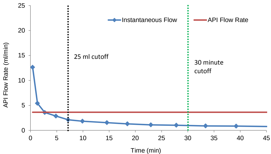
Figure 5.7 Instantaneous and average flow rates for Wyo-Ben NaturalGel (0.1 lb/gal).
