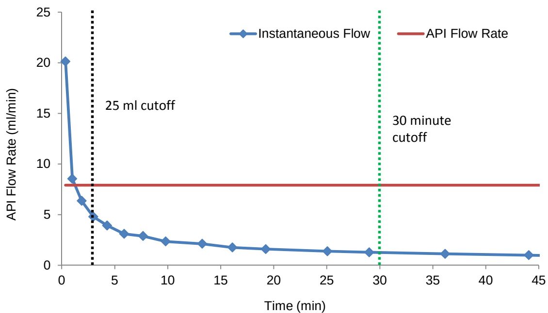
Figure 5.8 Instantaneous and average flow rates for Wyo-Ben Extra High Yield (0.1 lb/gal).
