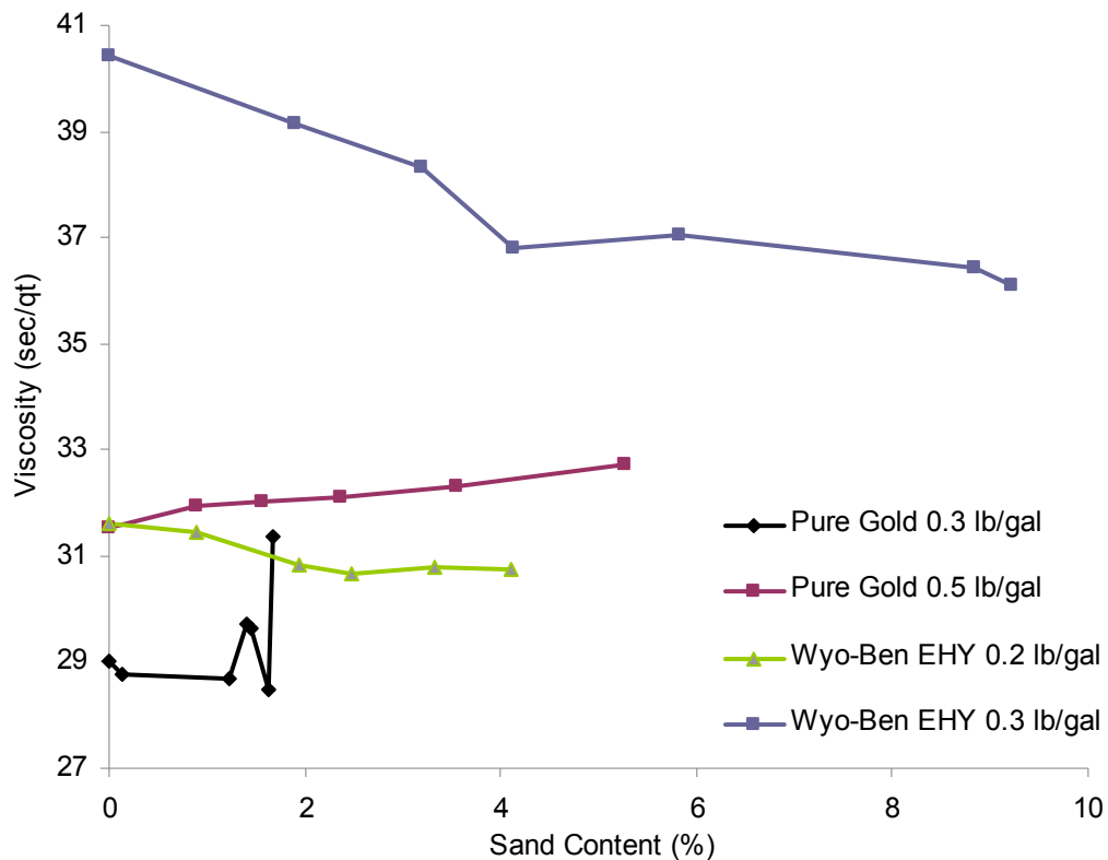
Figure 4.5 Measured sand content versus viscosity.
