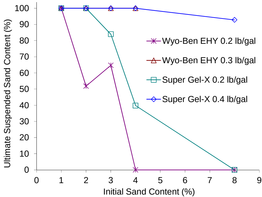
Figure 5.17 Polymer fortified (“High Yield”) slurry sand suspension.
