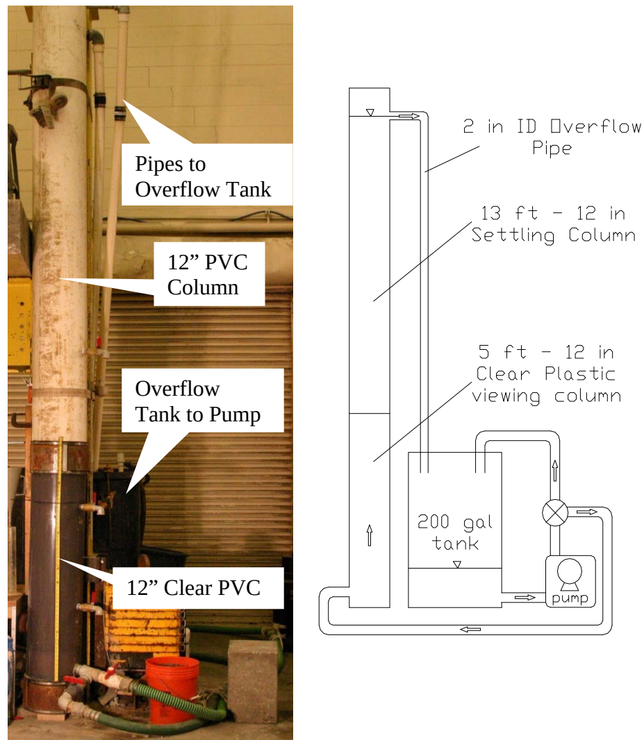
Figure 4.1 Sand settling column.
