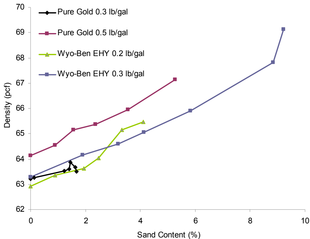
Figure 4.6 Measured sand content versus density.
