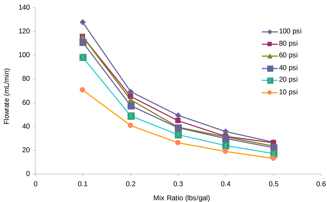
Figure 3.21 API filter press flow rate versus mix ratio at various pressure for attapulgate slurry.
