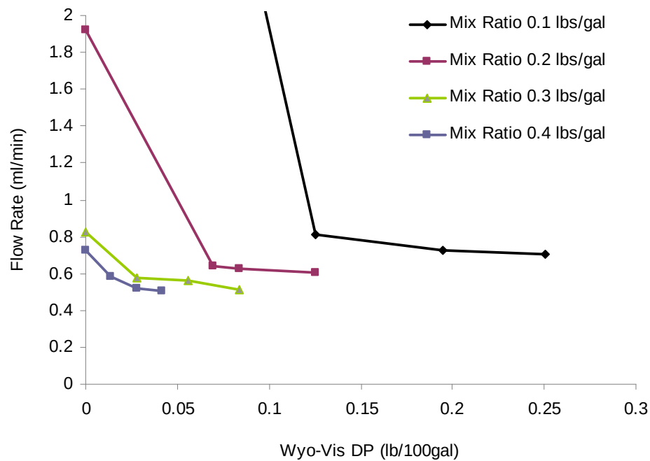
Figure 5.11 Flow rate decrease with increased additive concentrations.
