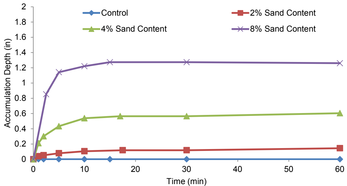
Figure 4.70 Sediment accumulation in 1.77 lb/100 gal NO-SAG
