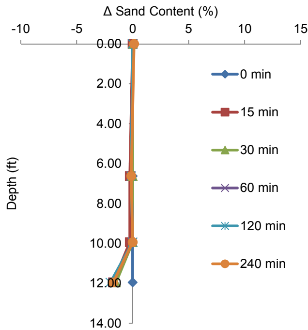
Figure 4.38 Change in sand content (0.9% initial sand content; 0.2 lb/gal; 0.12 lb/100 gal).
