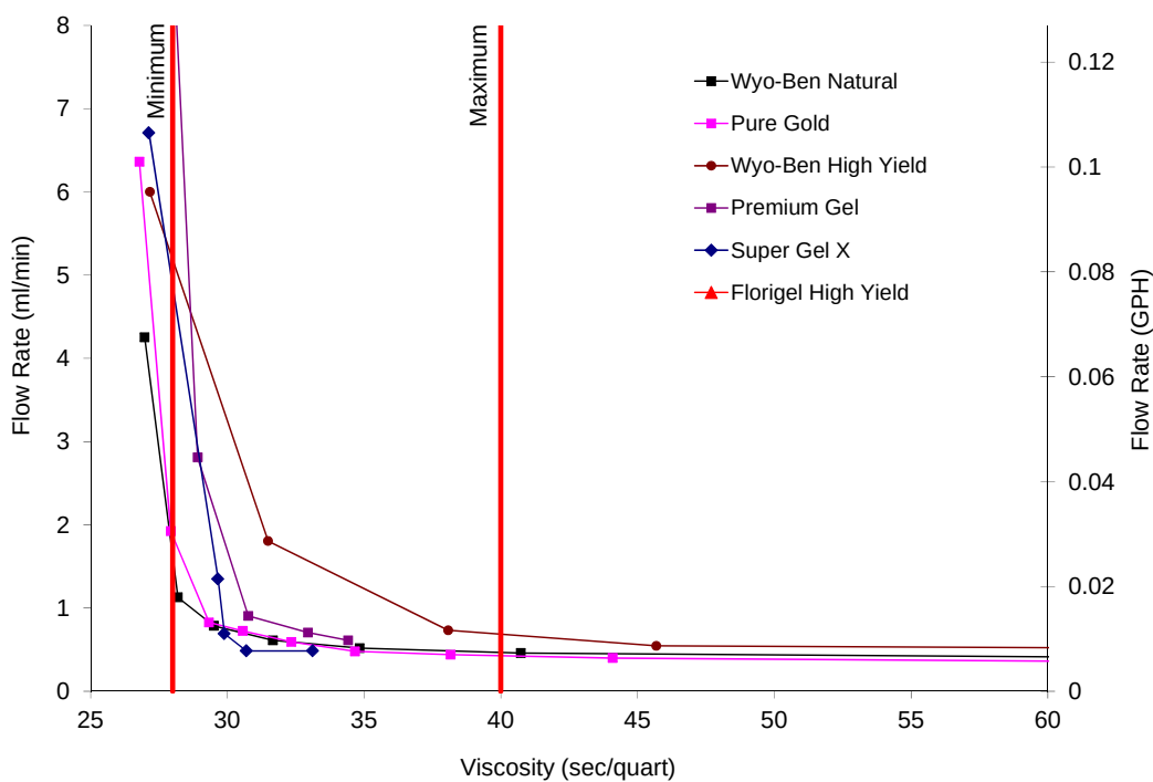
Figure 3.18 Flow rate versus viscosity comparison of each product (excluding attapulgate).
