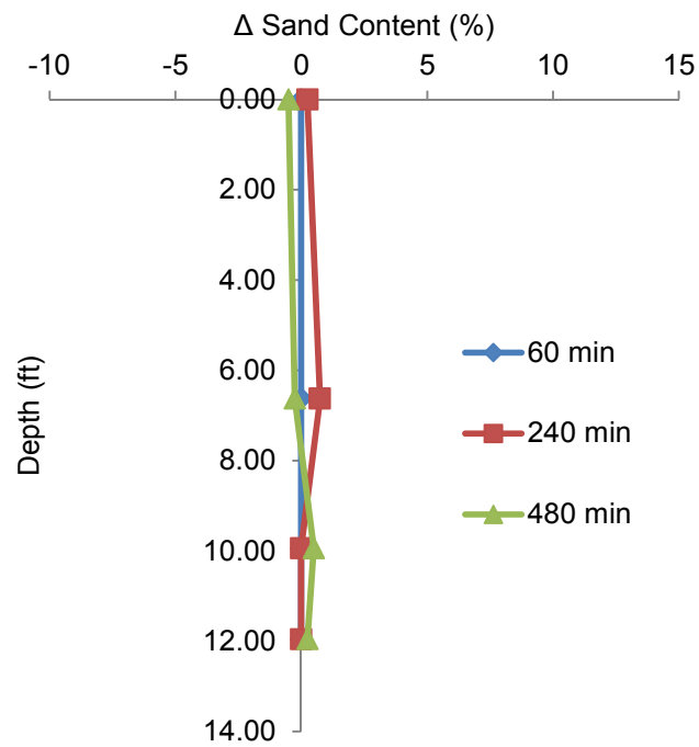
Figure 4.26 Change in sand content (3.1% overall starting sand content).
