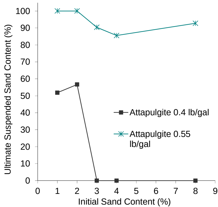
Figure 5.16 Attapulgate slurry sand suspension.
