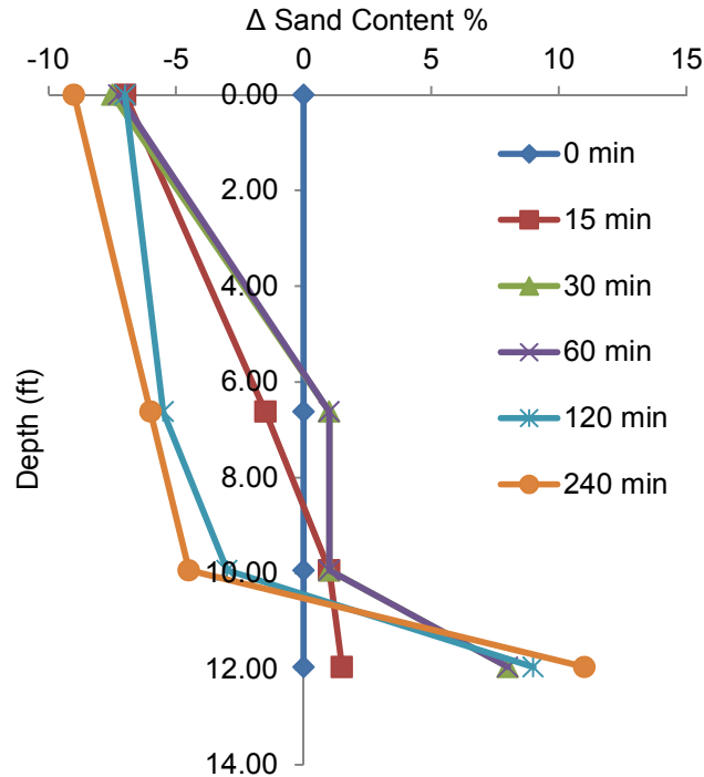
Figure 4.34 Change in sand content (9% overall starting sand content).
