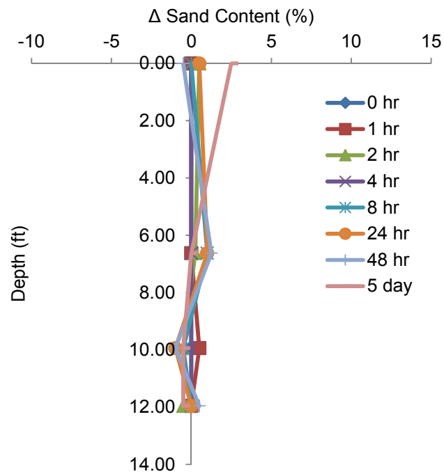
Figure 4.30 Repeated change in sand content (3.1% overall starting sand content).
