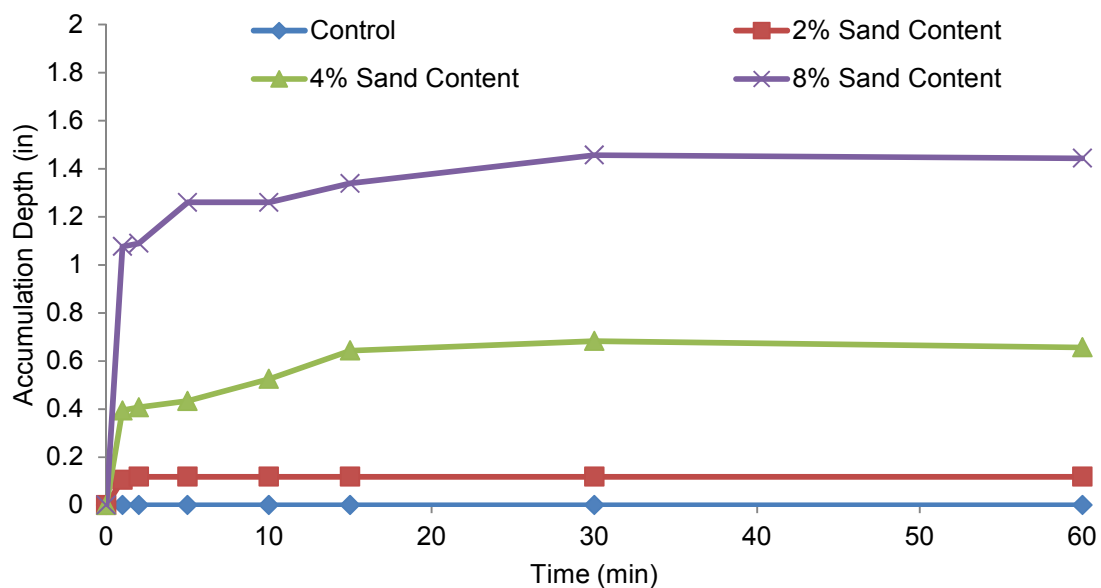
Figure 4.64 Sediment accumulation in 0.4 lb/gal Florigel attapulgite.
