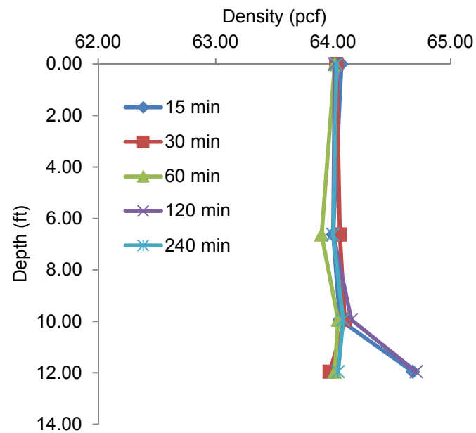
Figure 4.22 Initial density measurements for 0.6 lb/gal
