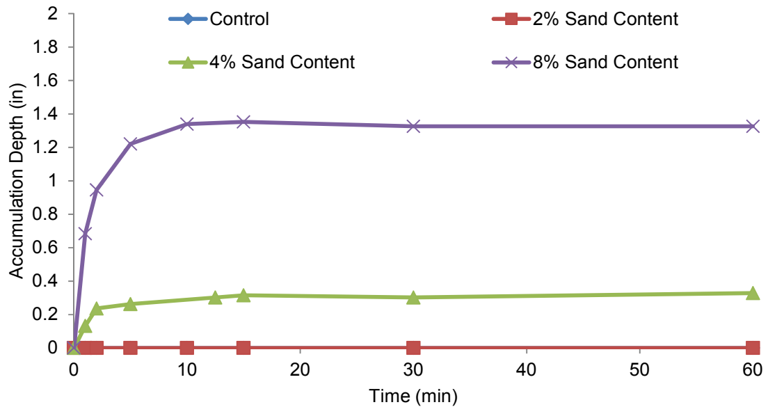
Figure 4.58 Sediment accumulation in 0.3 lb/gal Super Gel-X.
