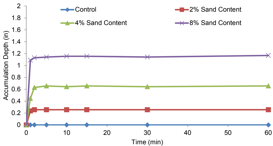
Figure 4.61 Sediment accumulation in 0.62 lb/100 gal SlurryPro CDP.
