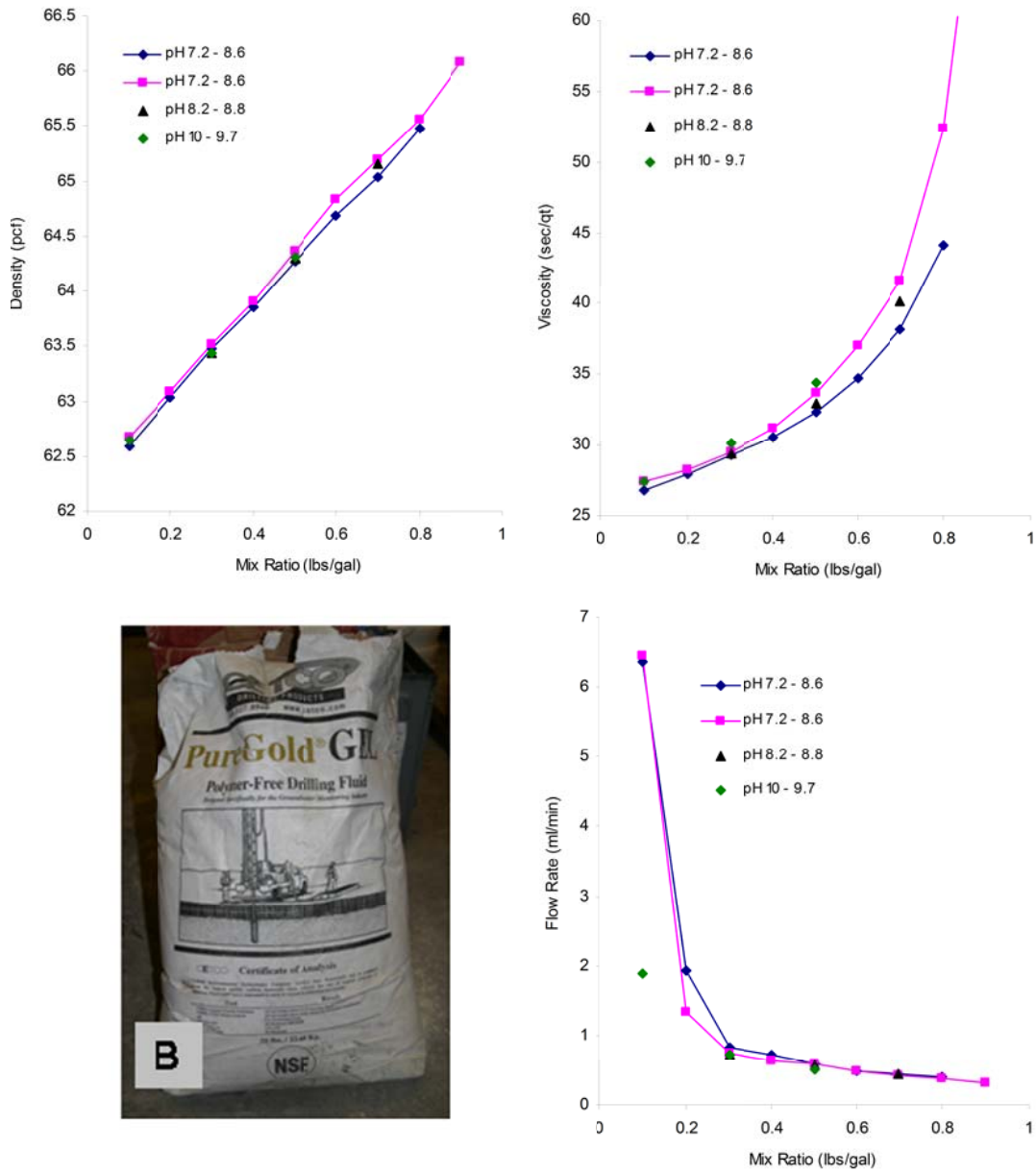
Figure 3.8 Pure Gold slurry testing results.
