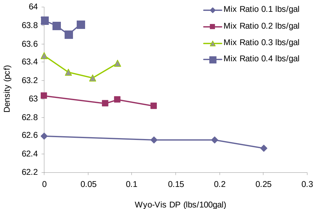
Figure 3.23 Effect of Wyo-Vis “DP” on density for a pure bentonite product.
