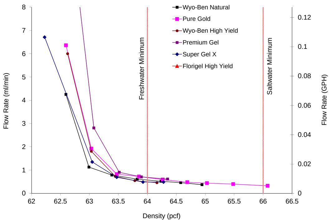
Figure 3.16 Flow rate versus density comparison of each product (excluding attapulgite).
