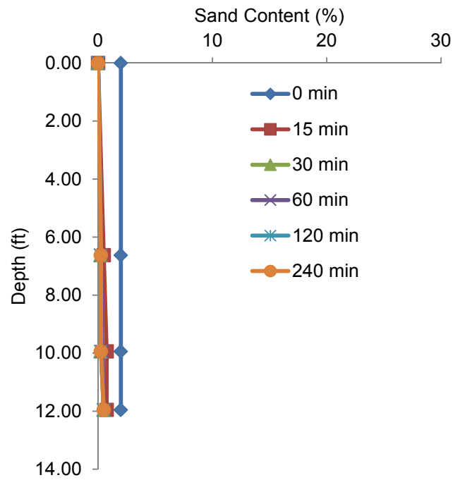
Figure 4.41 Measured sand content (2% initial sand content; 0.2 lb/gal; 0.12 lb/100 gal).
