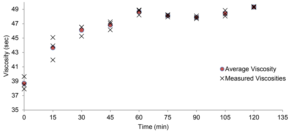
Figure 4.11 Polymer viscosity recovery following high shear mixing.
