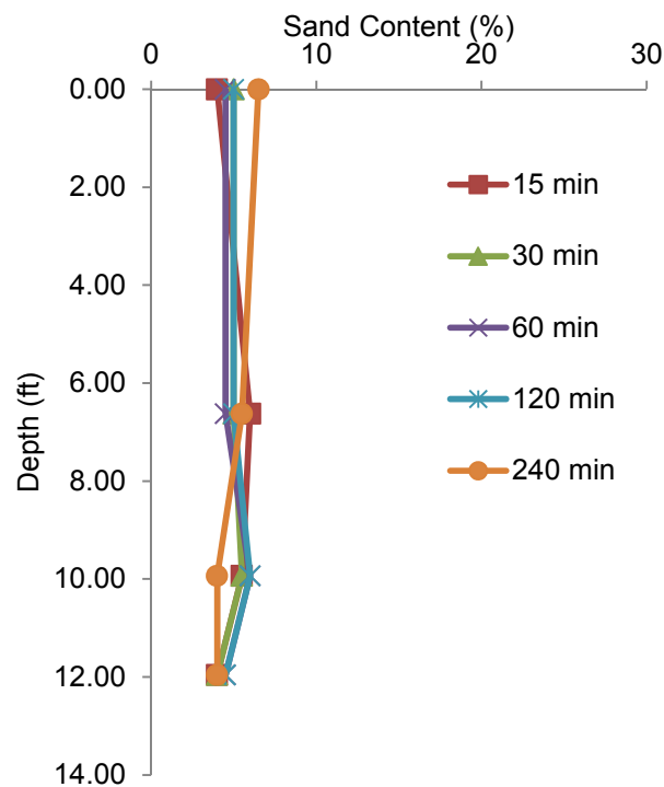
Figure 4.15 Measured sand content versus depth (4.9% overall starting sand content).
