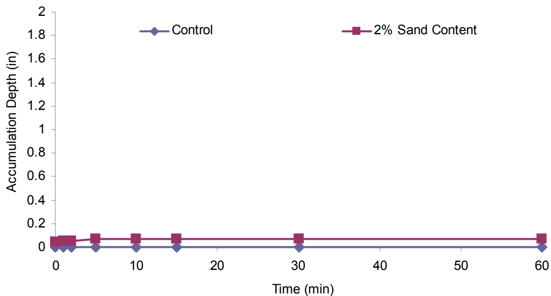
Figure 4.67 Sediment accumulation in 0.3 lb/gal CETCO PureGold with Wyo-Vis DP.
