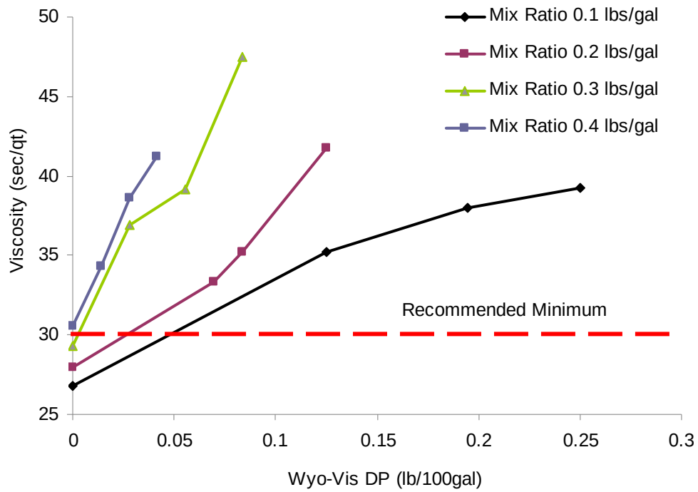
Figure 5.10 Viscosity increase as a function of additive concentration.
