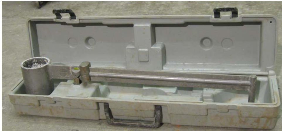
Figure 2.12 Mud balance with case
