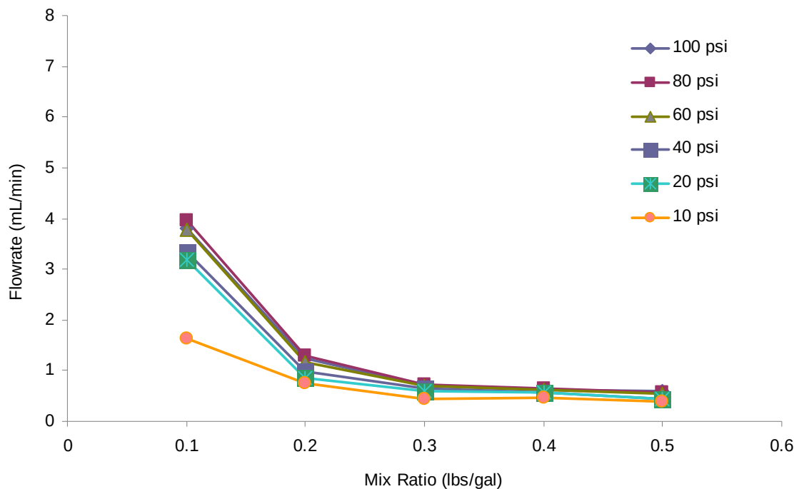
Figure 3.19 API filter press flow rate versus mix ratio at various pressure for pure bentonite slurry.
