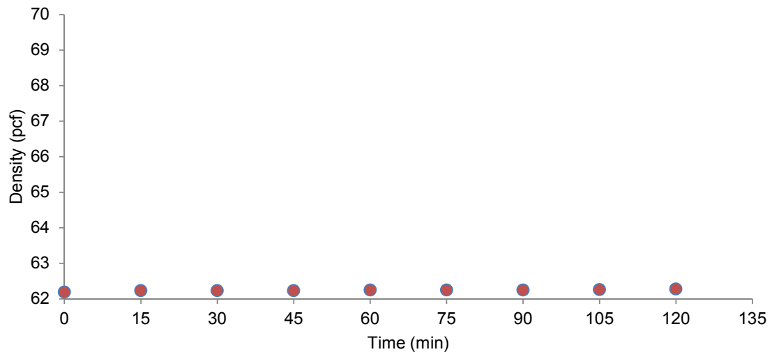
Figure 4.12 Polymer density recovery following high shear mixing.
