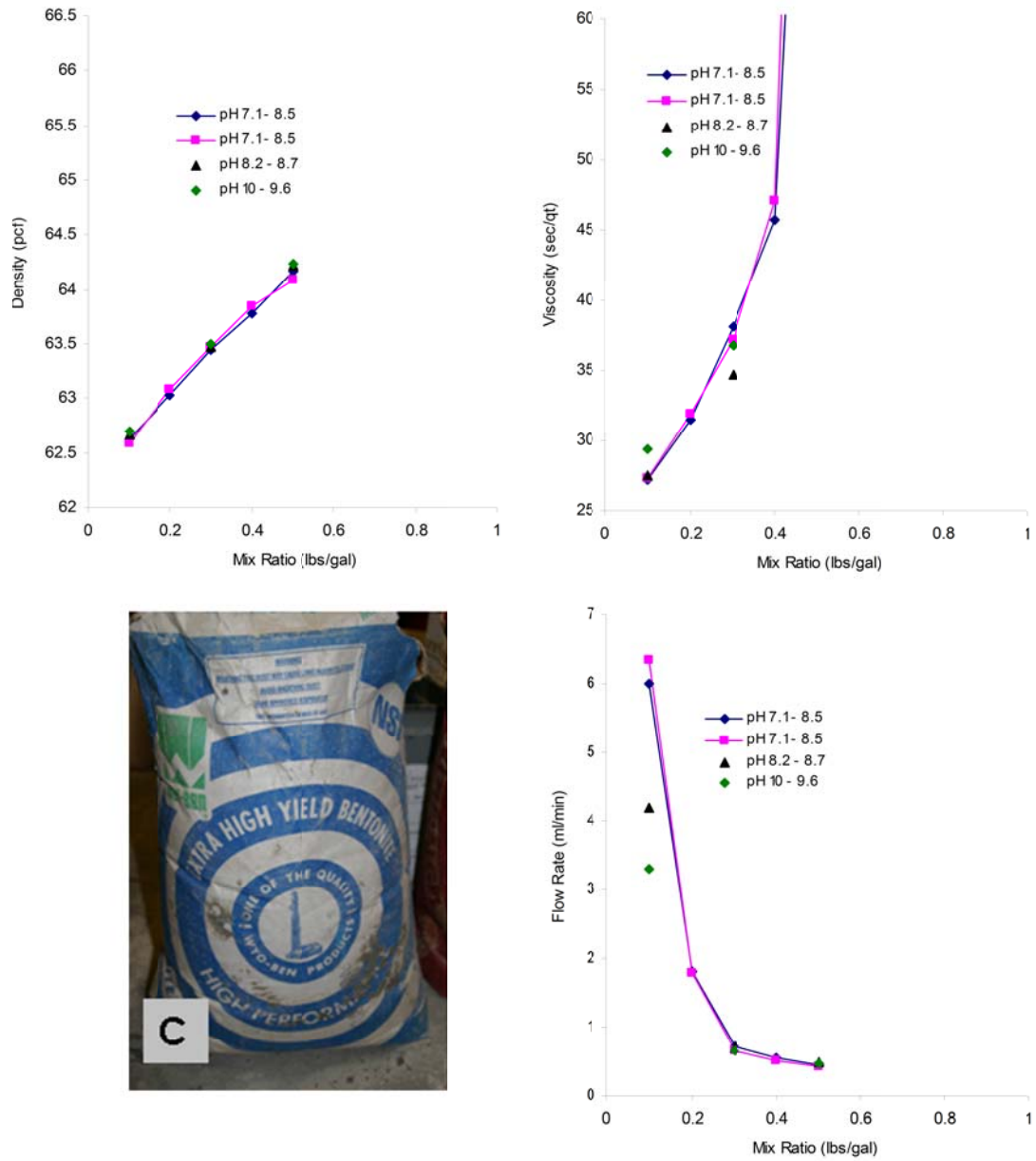
Figure 3.9 Wyo-Ben Extra High Yield slurry testing results.
