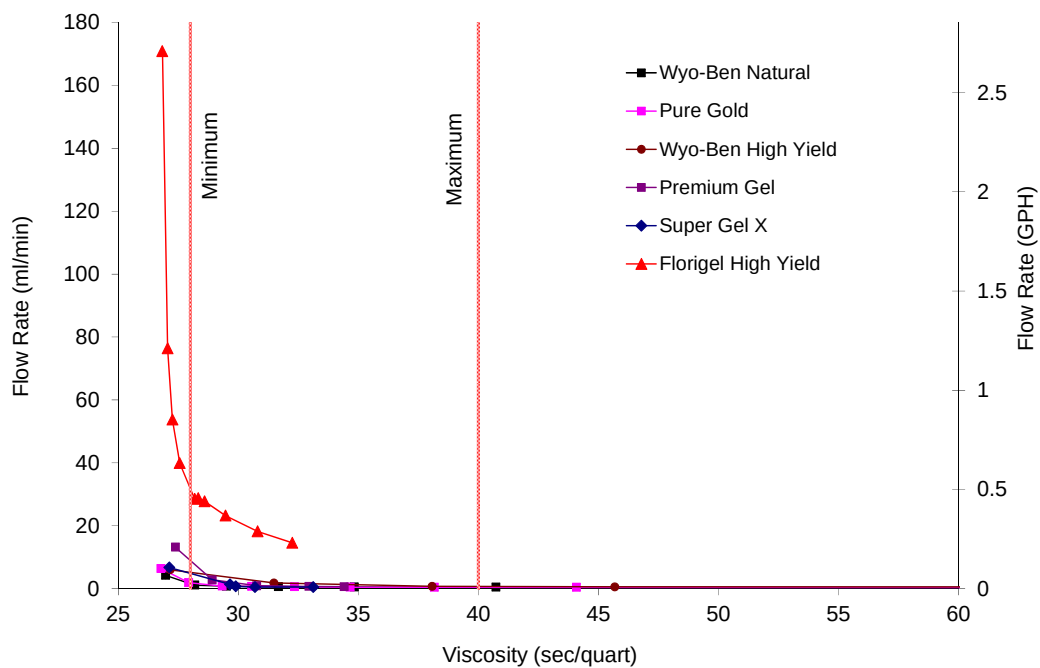
Figure 3.17 Flow rate versus viscosity comparison of each product.
