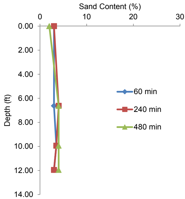
Figure 4.27 Repeated measured sand content (3.1% overall starting sand content).
