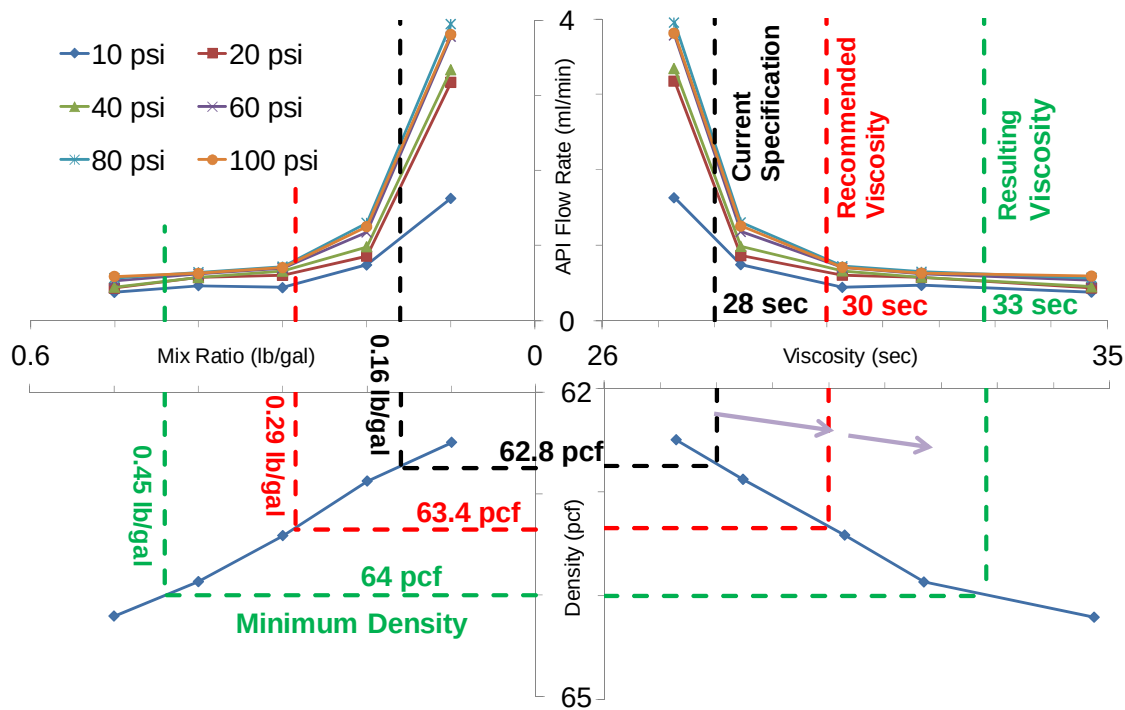
Figure 5.20 Mix ratio selection plots for bentonite.
