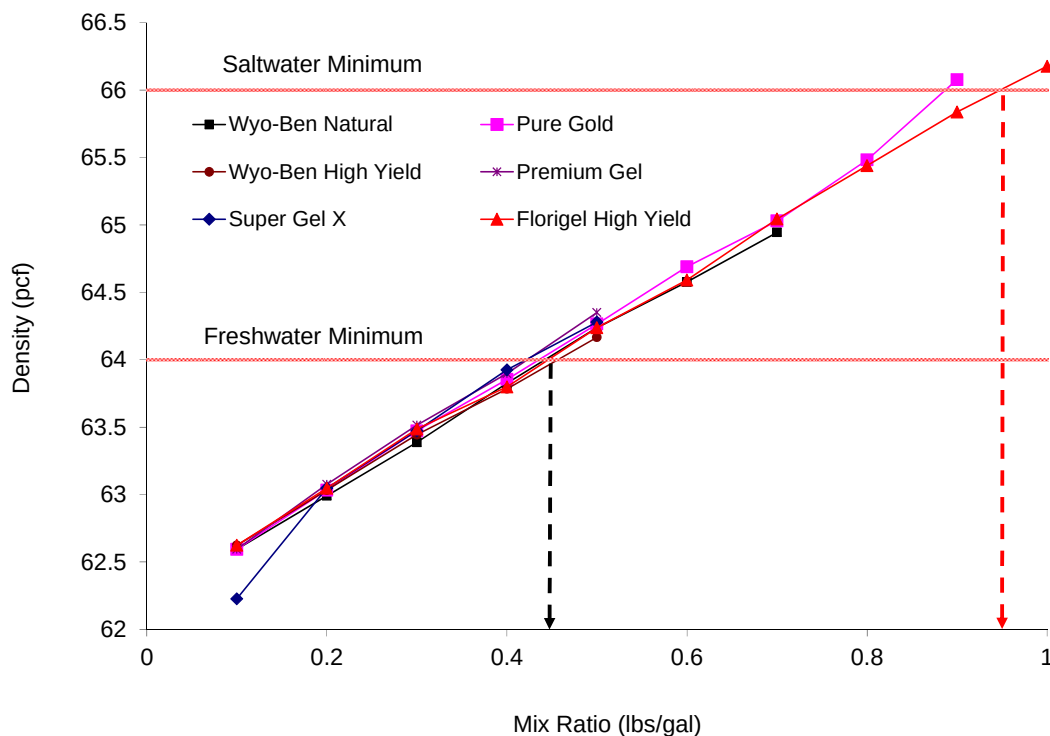
Figure 5.1 Density as a function of mix ratio for all the mineral slurries tested.
