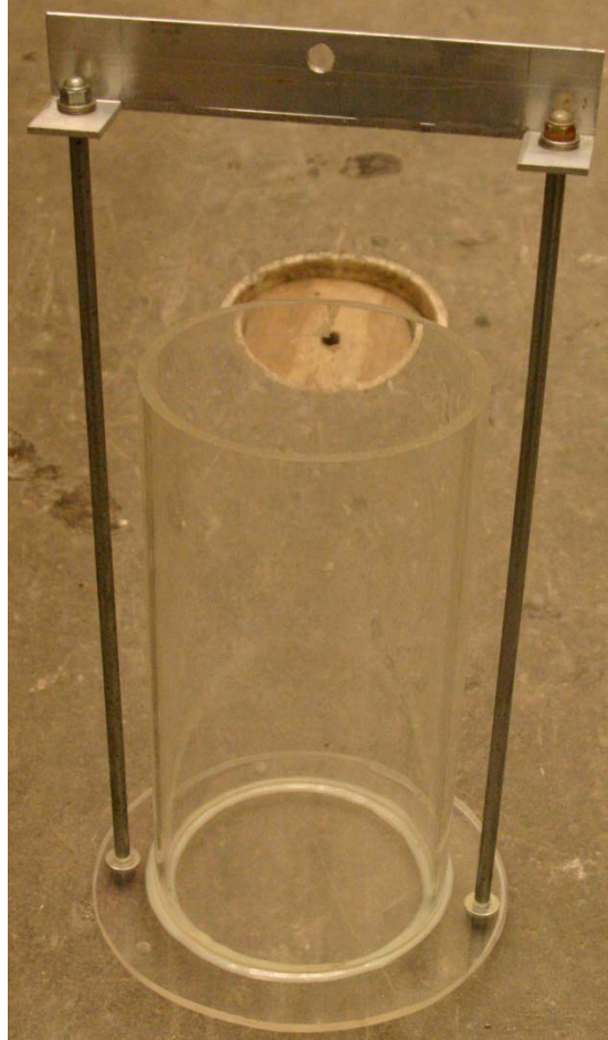
Figure 4.45 Lexan accumulation sampler
