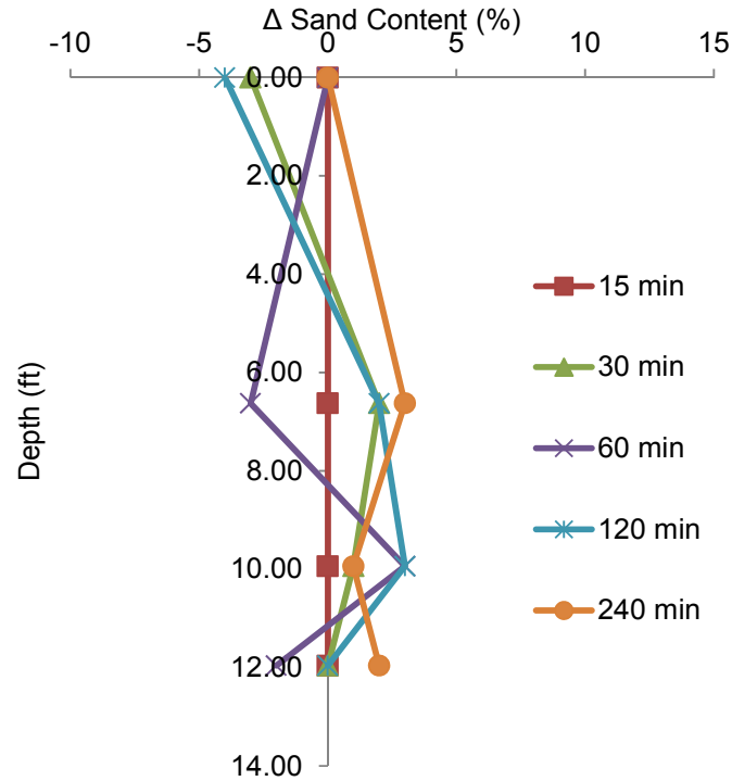
Figure 4.20 Change in sand content (16.25% overall starting sand content).
