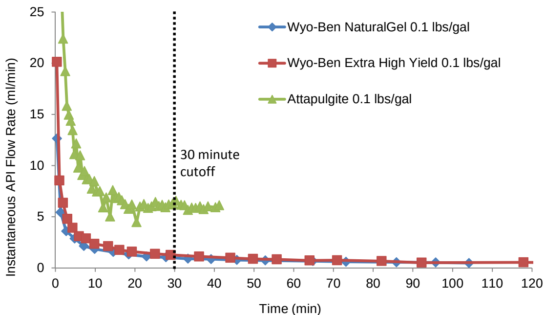
Figure 5.5 Extended filter press results versus elapsed time.
