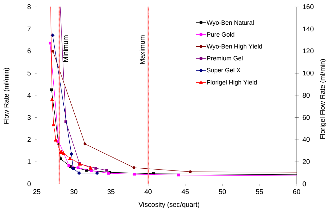
Figure 5.3 Stable infiltration flow rates at viscosity values above 30 to 32 sec/qt.
