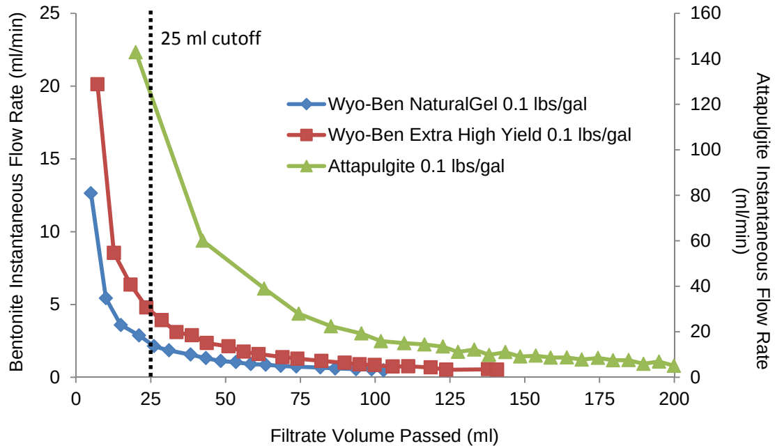
Figure 5.6 Extended filter press results versus filtrate volume.
