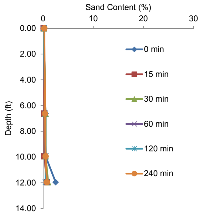
Figure 4.37 Measured sand content (0.9% initial sand content; 0.2 lb/gal; 0.12 lb/100 gal).
