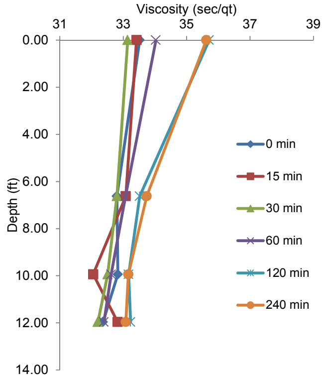
Figure 4.35 Initial hybrid slurry viscosity testing (bentonite 0.2 lb/gal; Wyo-Vis “DP” 0.12 lb/100 gal).
