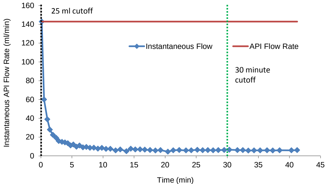
Figure 5.9 Instantaneous and average flow rates for Florigel Attapulgite (0.1 lb/gal).
