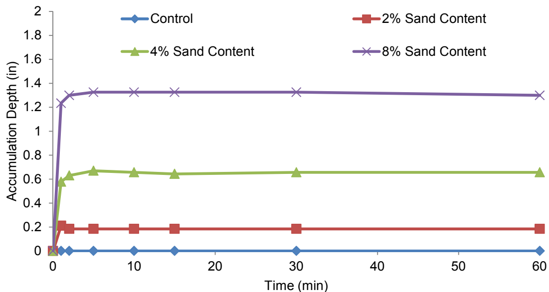
Figure 4.62 Sediment accumulation in 1.26 lb/100 gal SlurryPro CDP.
