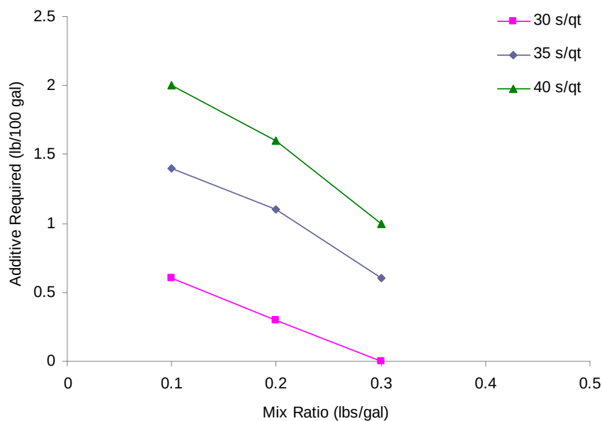
Figure 5.13 Amount of NO-SAG to produce a desired viscosity for a pure bentonite product.
