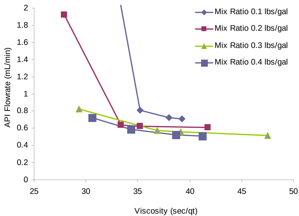
Figure 3.26 Viscosity versus API Filter test flow rate for a pure bentonite product modified with Wyo-Vis “DP”.
