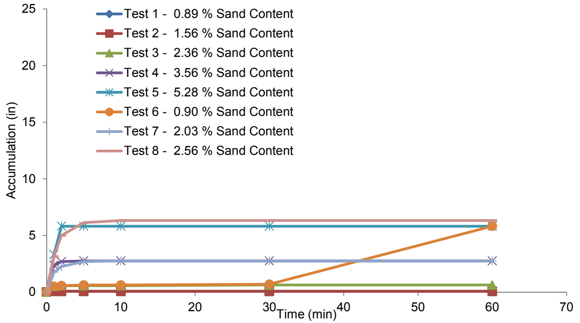
Figure 4.8 Measured accumulation for 0.5 lb/gal PureGold.
