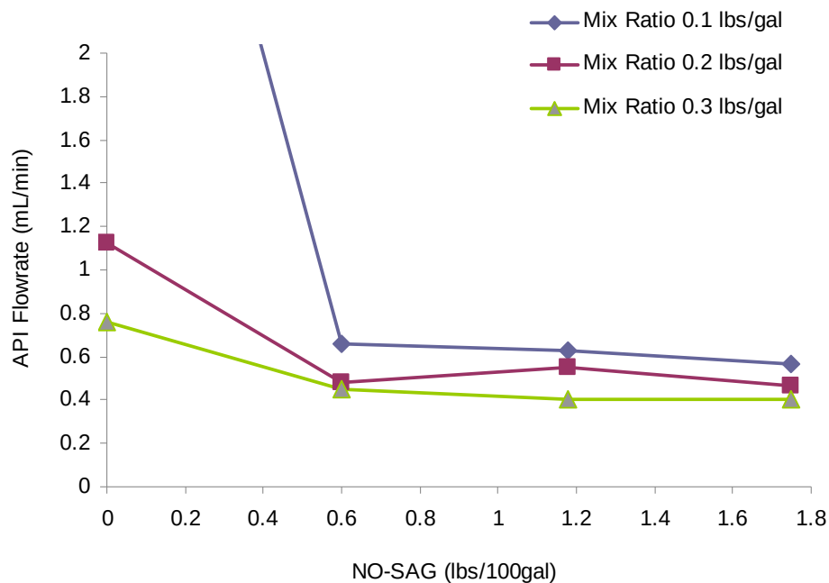
Figure 3.29 Effect of NO-SAG on API Filter test flow rate for a pure bentonite product.
