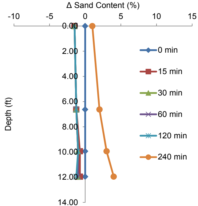
Figure 4.40 Change in sand content (1.5% initial sand content; 0.2 lb/gal; 0.12 lb/100 gal).
