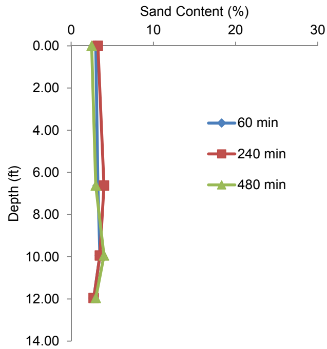
Figure 4.25 Measured sand content (3.1% overall starting sand content).
