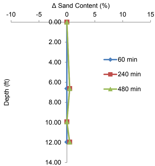
Figure 4.24 Change in sand content (2.25% overall starting sand content).
