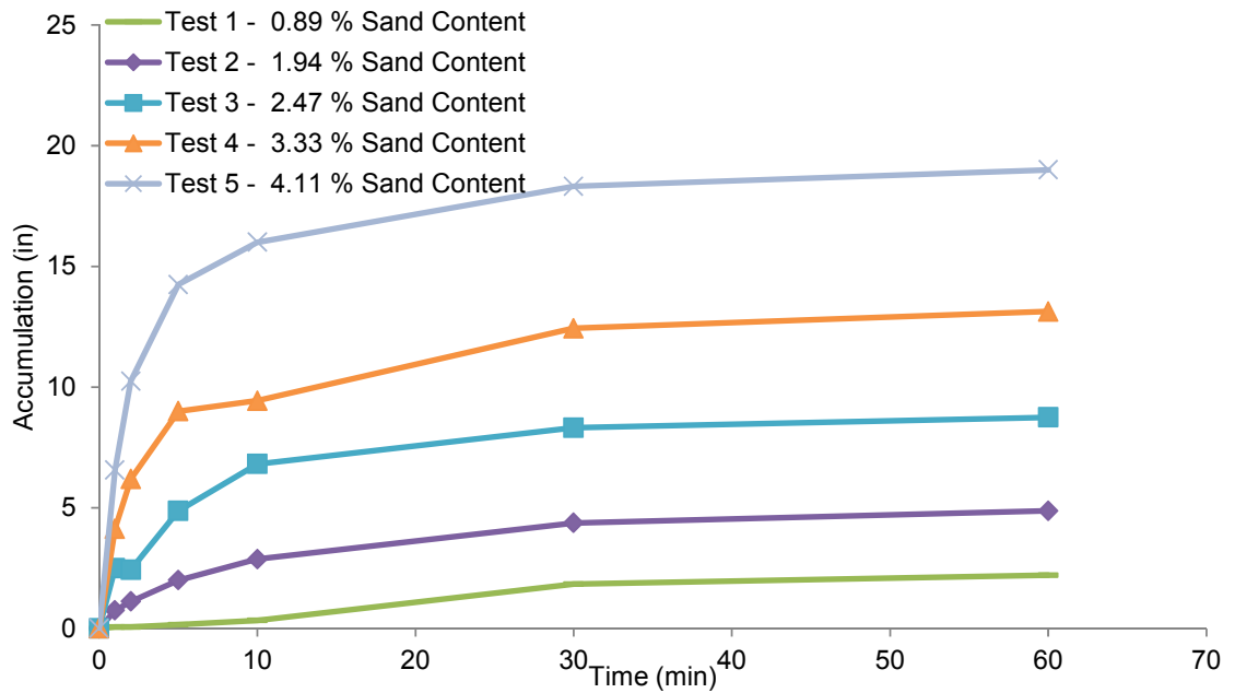
Figure 4.9 Measured accumulation for 0.2 lb/gal Wyo-Ben High Yield.
