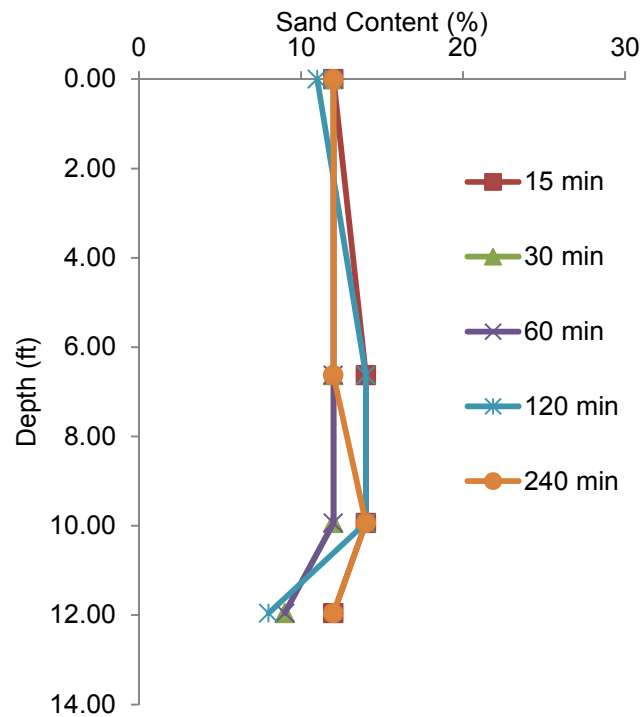
Figure 4.17 Measured sand content versus depth (13% overall starting sand content).
