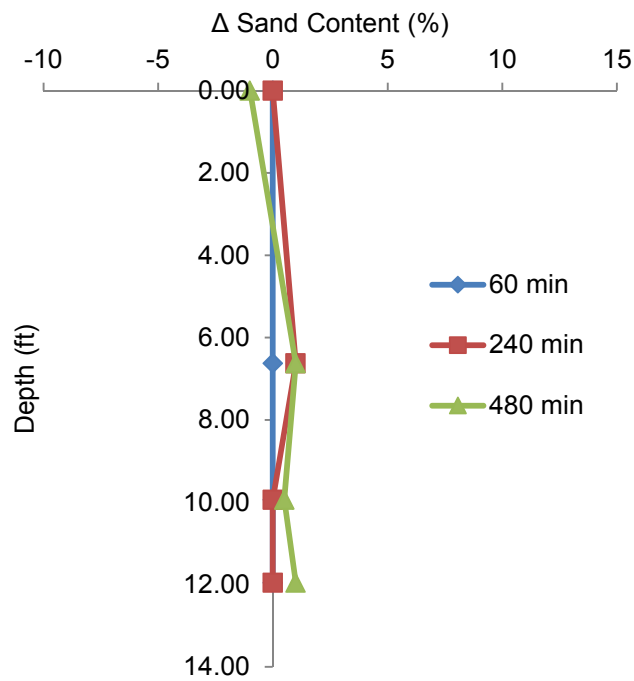
Figure 4.28 Repeated change in sand content (3.1% overall starting sand content).
