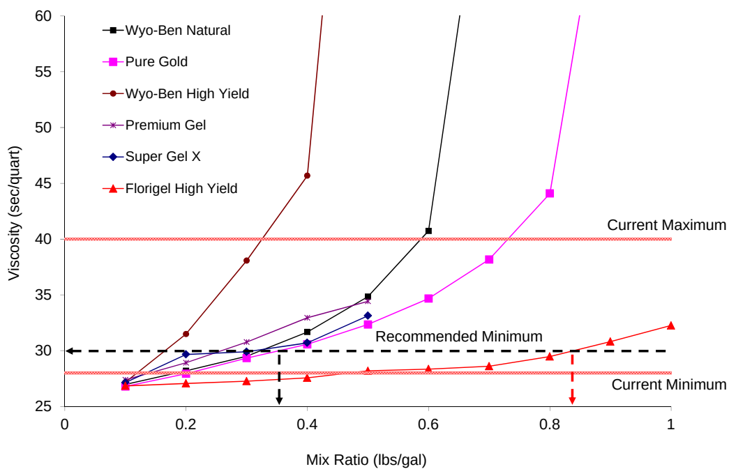
Figure 5.2 Viscosity as a function of mix ratio with recommended changes to the minimum state viscosity specification.
