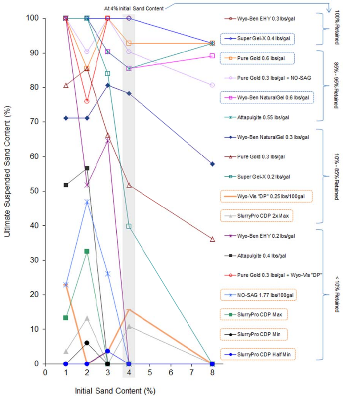
Figure 5.14 Retained sand in suspension for all tested slurries (boxed mineral (blue) and polymer (orange) meet FDOT slurry specifications).
