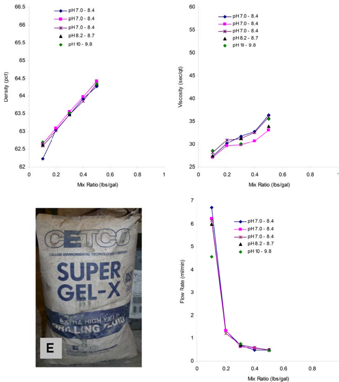
Figure 3.11 Super Gel-X slurry testing results.
