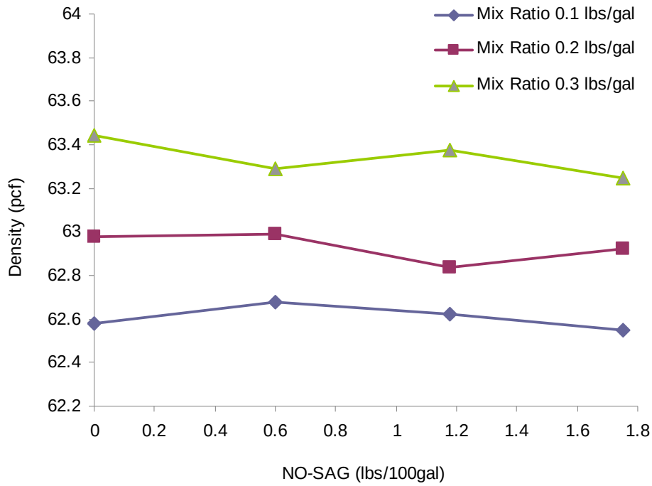
Figure 3.27 Effect of NO-SAG on density for a pure bentonite product.
