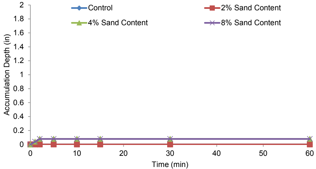
Figure 4.65 Sediment accumulation in 0.55 lb/gal Florigel attapulgite.
