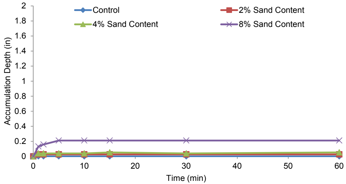
Figure 4.66 Sediment accumulation in 0.3 lb/gal CETCO PureGold with NO-SAG.
