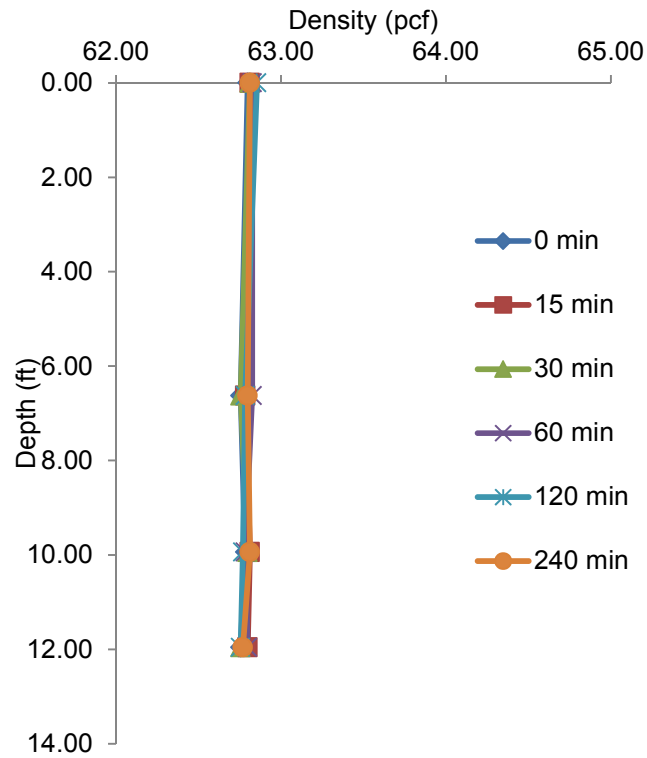
Figure 4.36 Initial hybrid slurry density testing (bentonite 0.2 lb/gal; Wyo-Vis “DP” 0.12 lb/100 gal).
