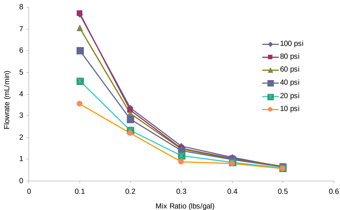
Figure 3.20 API filter press flow rate versus mix ratio at various pressure for high yield slurry.
