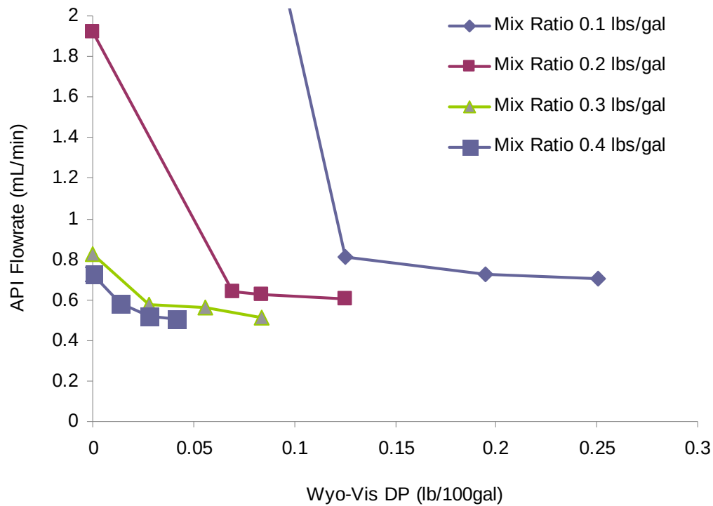
Figure 3.25 Effect of Wyo-Vis “DP” on API Filter test flow rate for a pure bentonite product.
