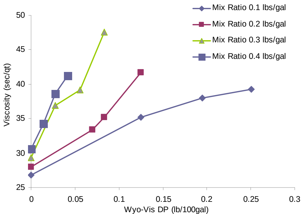
Figure 3.24 Effect of Wyo-Vis “DP” on viscosity for a pure bentonite product.
