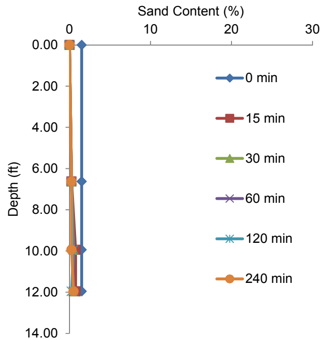
Figure 4.39 Measured sand content (1.5% initial sand content; 0.2 lb/gal; 0.12 lb/100 gal).
