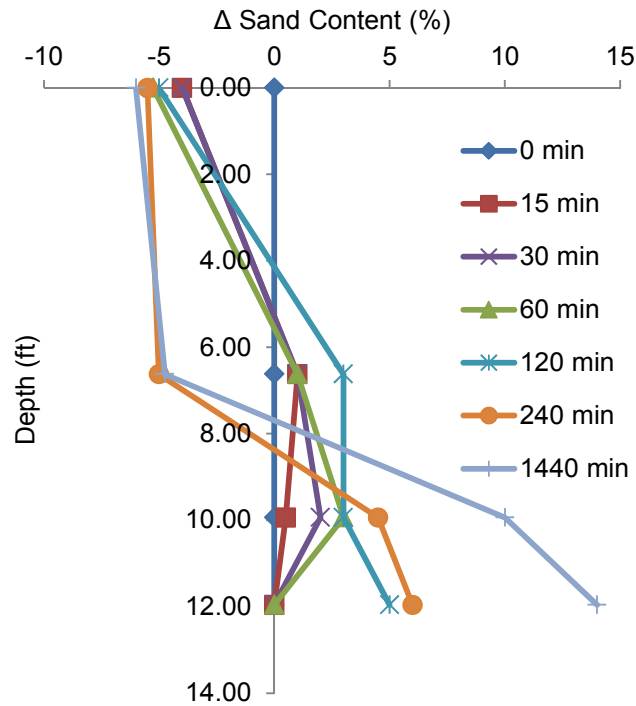
Figure 4.32 Change in sand content (6% overall starting sand content).
