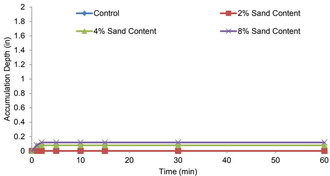
Figure 4.51 Sediment accumulation in 0.6 lb/gal Wyo-Ben NaturalGel.
