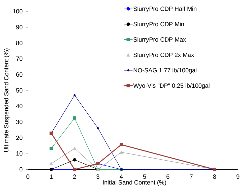
Figure 5.19 Polymer slurry sand suspension.
