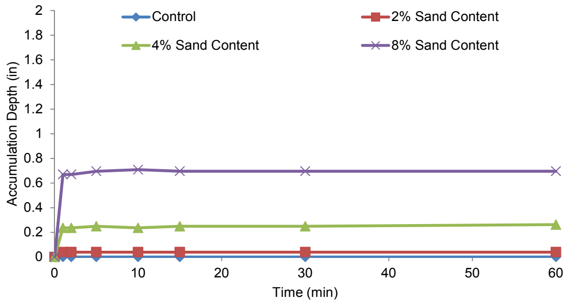
Figure 4.52 Sediment accumulation in 0.3 lb/gal PureGold.
