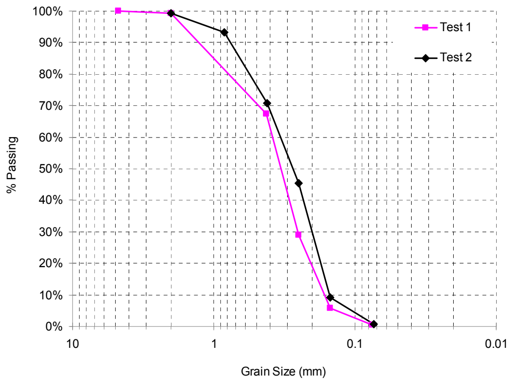
Figure 4.4 Grain size distribution for the sand used in the testing.
