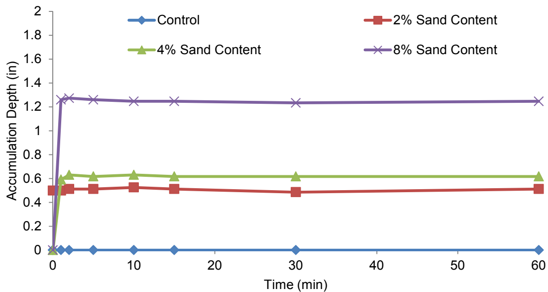
Figure 4.60 Sediment accumulation in 0.31 lb/100 gal SlurryPro CDP.
