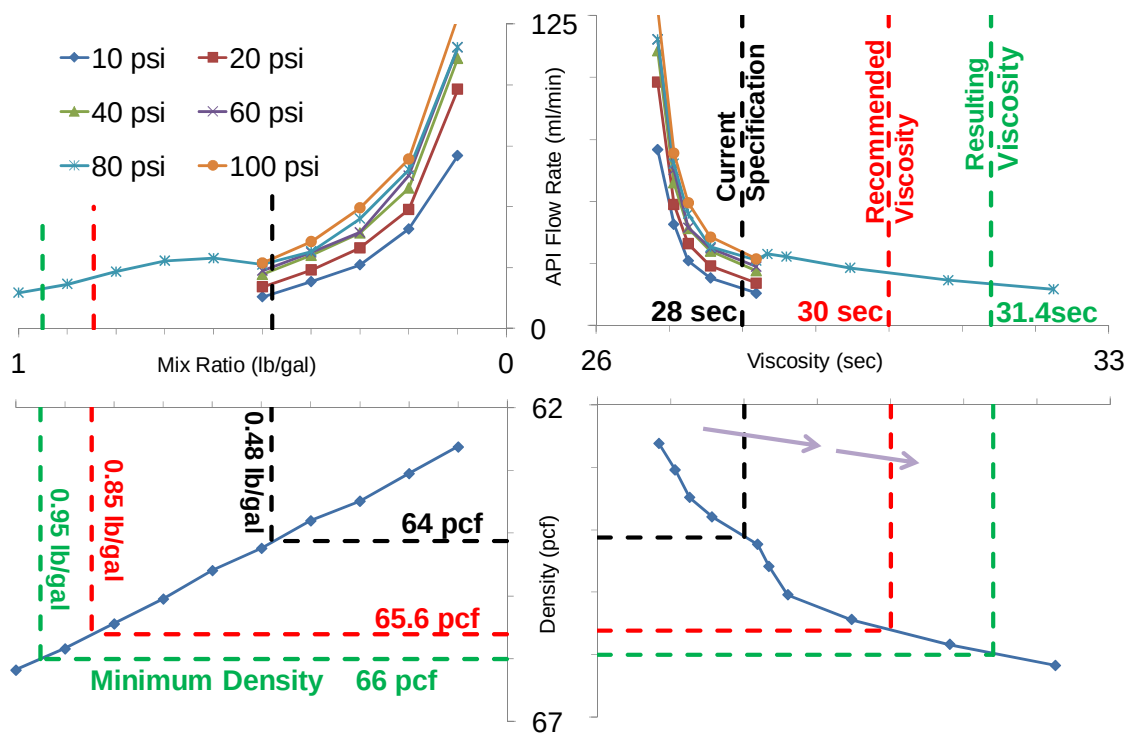
Figure 5.21 Mix ratio selection plots for attapulgite.
