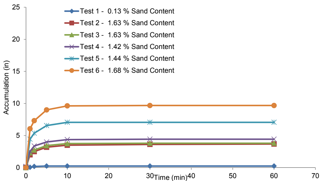
Figure 4.7 Measured accumulation for 0.3 lb/gal PureGold.
