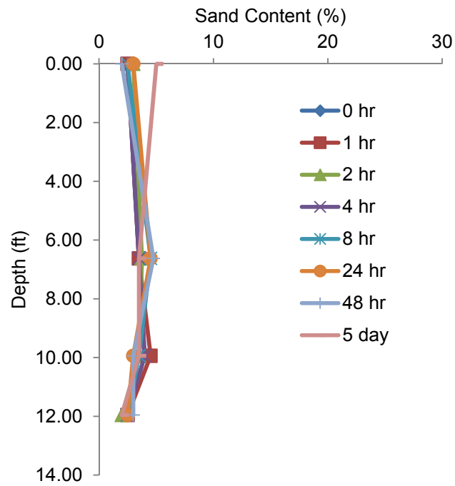
Figure 4.29 Repeated measured sand content (3.1% overall starting sand content).
