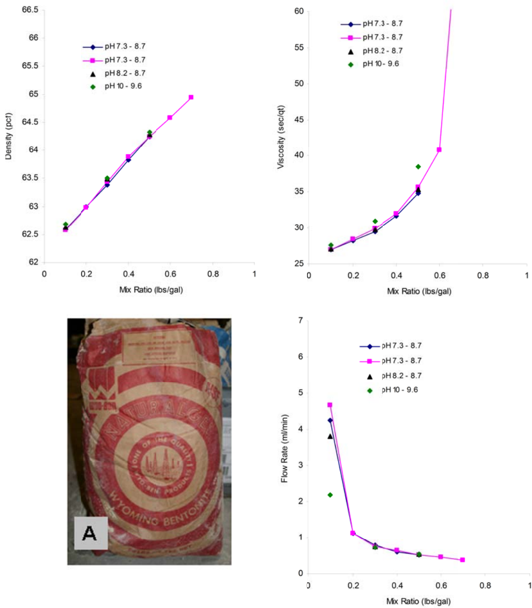
Figure 3.7 Wyo-Ben Natural slurry testing results.
