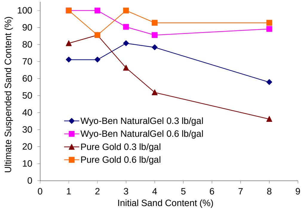
Figure 5.15 Pure bentonite slurry sand suspension.
