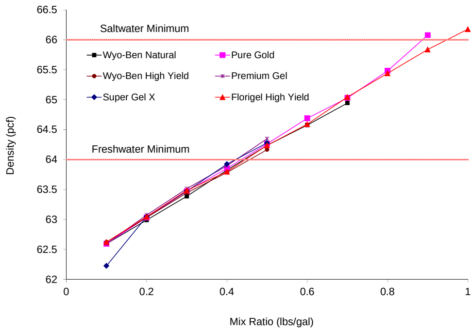
Figure 3.13 Density versus mix ratio comparison of each product.
