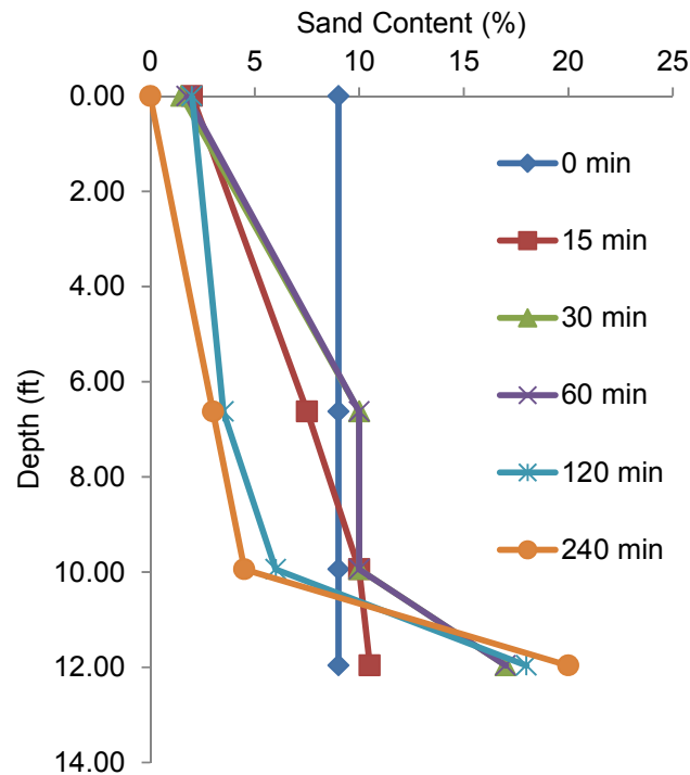
Figure 4.33 Measured sand content (9% overall starting sand content).
