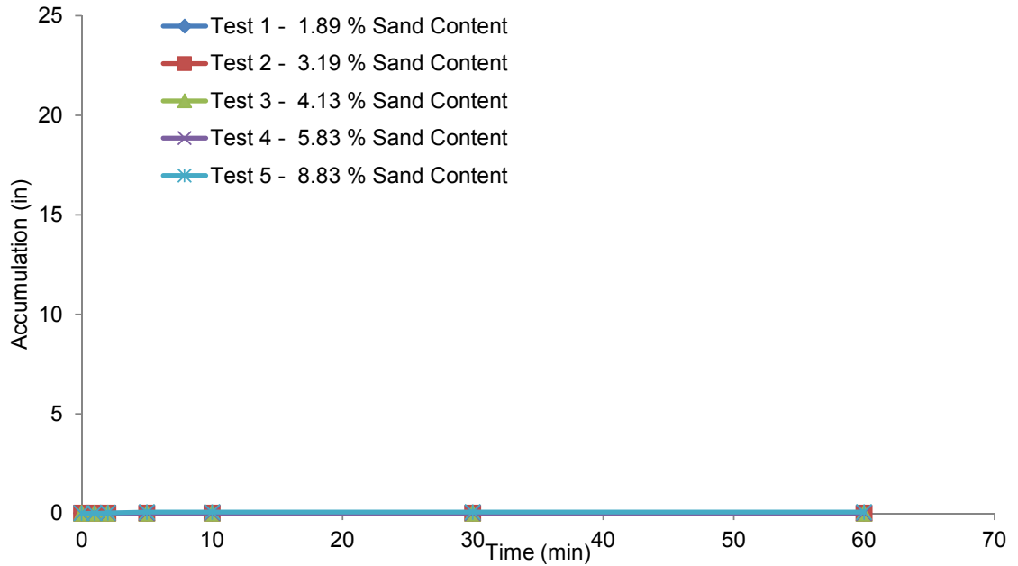
Figure 4.10 Measured accumulation for 0.3 lb/gal Wyo-Ben High Yield.
