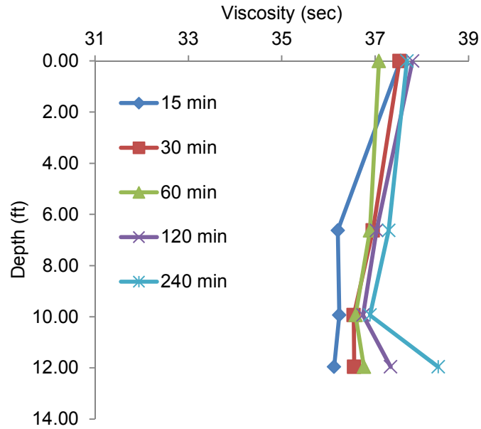
Figure 4.21 Initial viscosity measurements for 0.6 lb/gal
