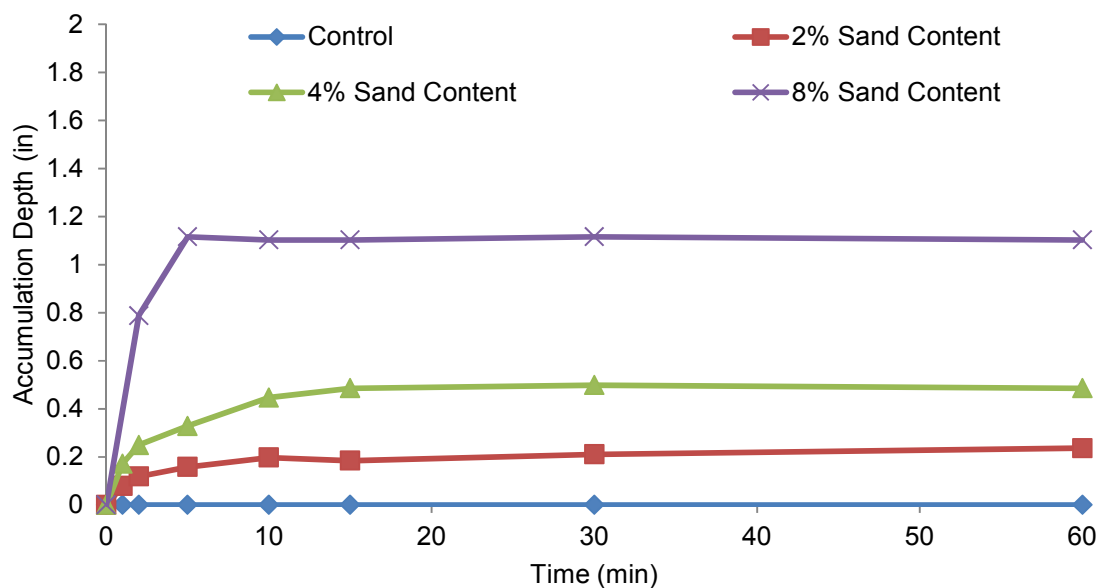
Figure 4.63 Sediment accumulation in 2.52 lb/100 gal SlurryPro CDP.
