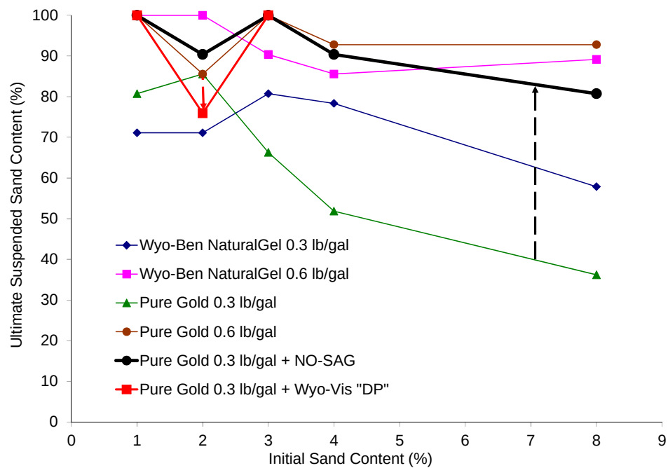
Figure 5.18 Effect of WyoVis and NO-SAG on suspension performance.
