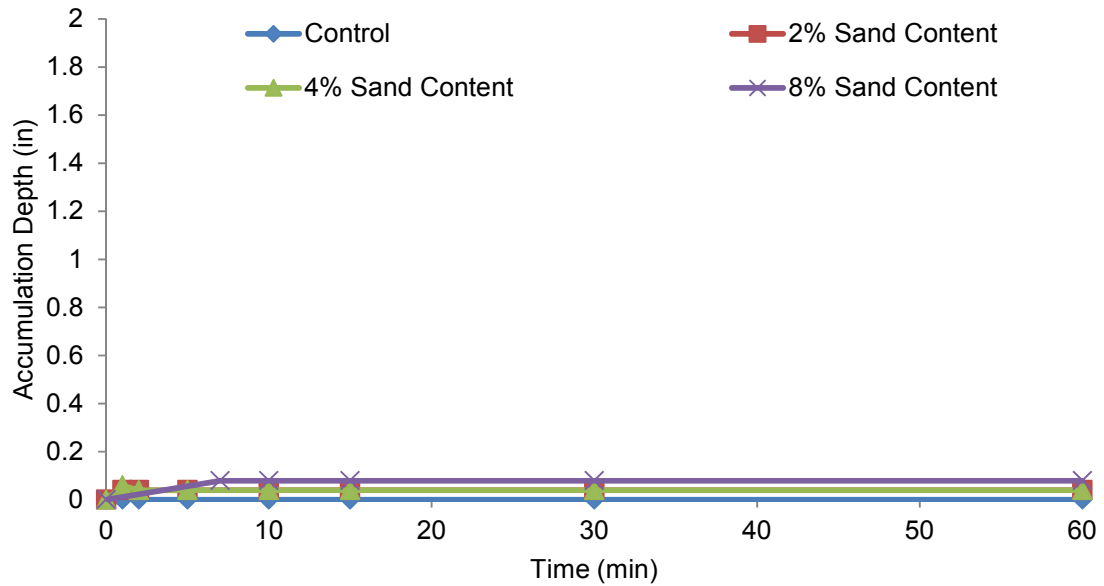
Figure 4.53 Sediment accumulation in 0.6 lb/gal PureGold
