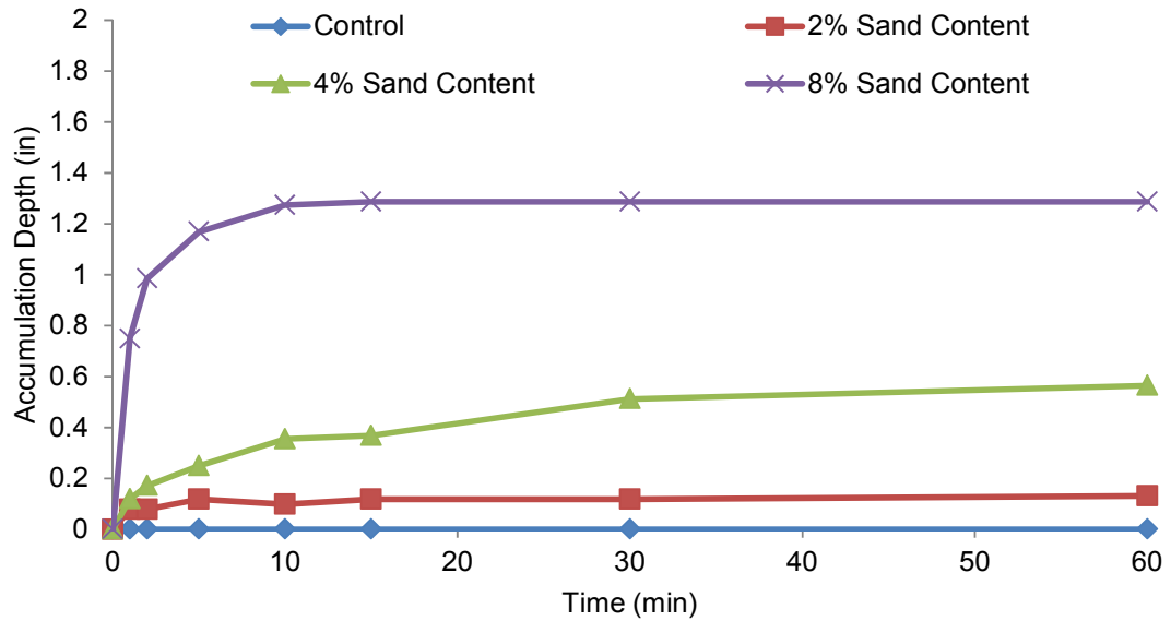
Figure 4.54 Sediment accumulation in 0.2 lb/gal Wyo-Ben Extra High Yield.
