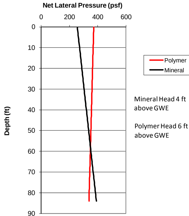
Figure 2.11 Net lateral pressure on excavation walls from mineral and polymer slurry.
