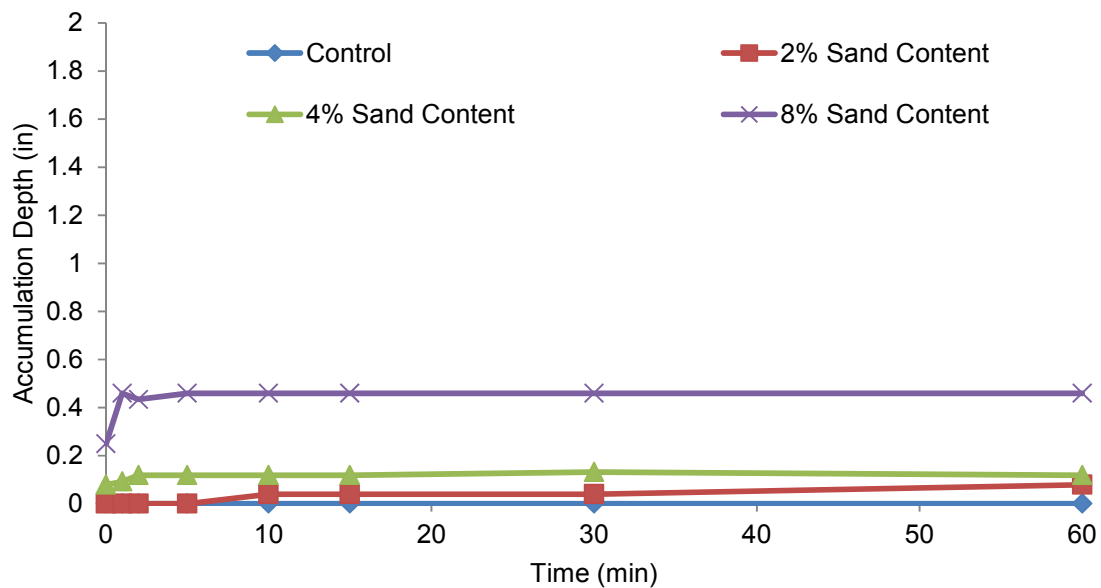
Figure 4.50 Sediment accumulation in 0.3 lb/gal Wyo-Ben NaturalGel.
