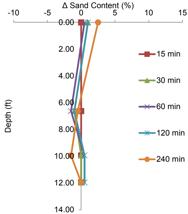
Figure 4.16 Change in sand content versus depth (4.9% overall starting sand content).
