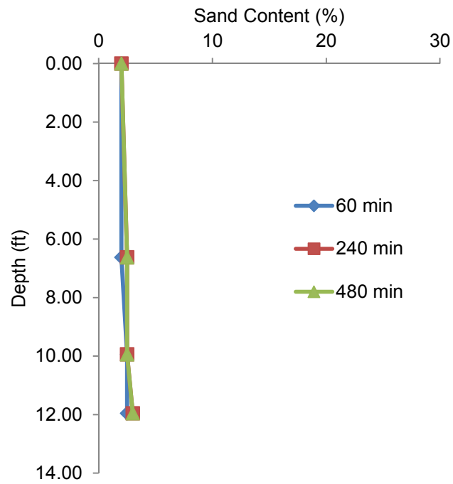
Figure 4.23 Measured sand content (2.25% overall starting sand content).
