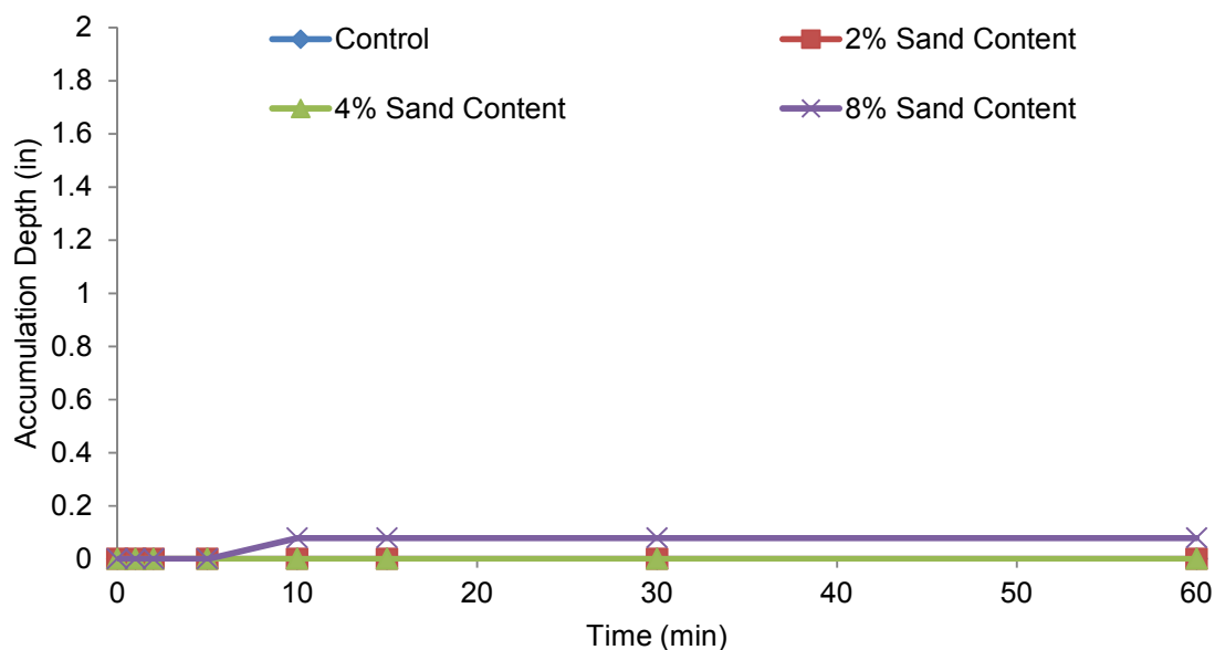
Figure 4.59 Sediment accumulation in 0.4 lb/gal Super Gel-X.
