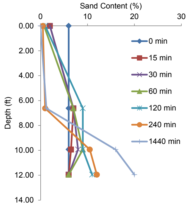
Figure 4.31 Measured sand content (6% overall starting sand content).
