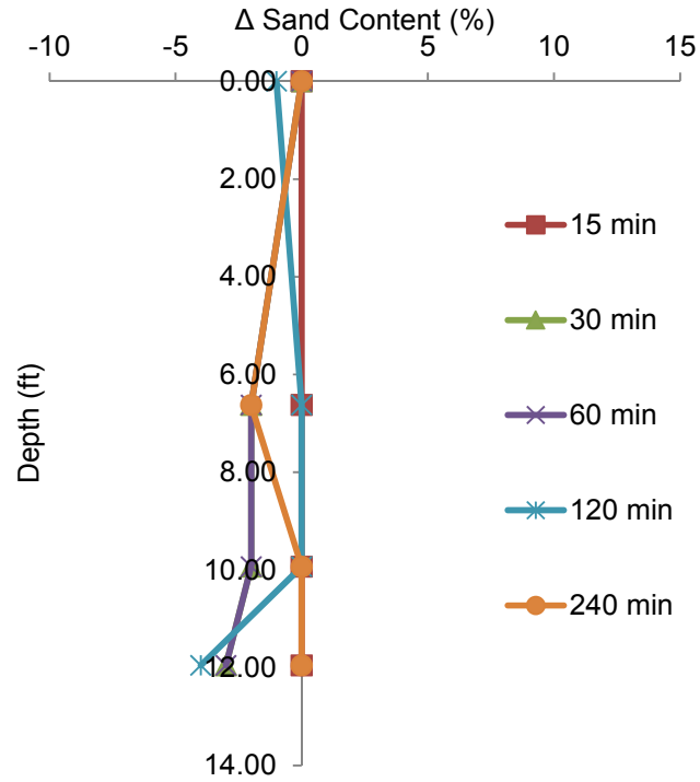
Figure 4.18 Change in sand content versus depth (13% overall starting sand content).
