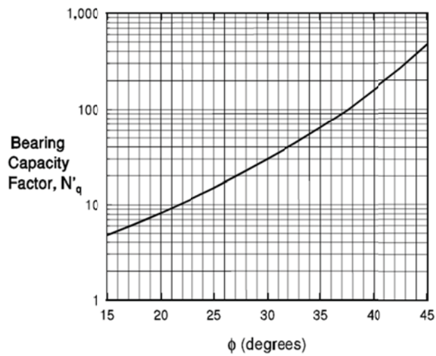
Figure 3.10 Bearing capacity factor N'_q (FHWA--DRIVEN, 1998)
