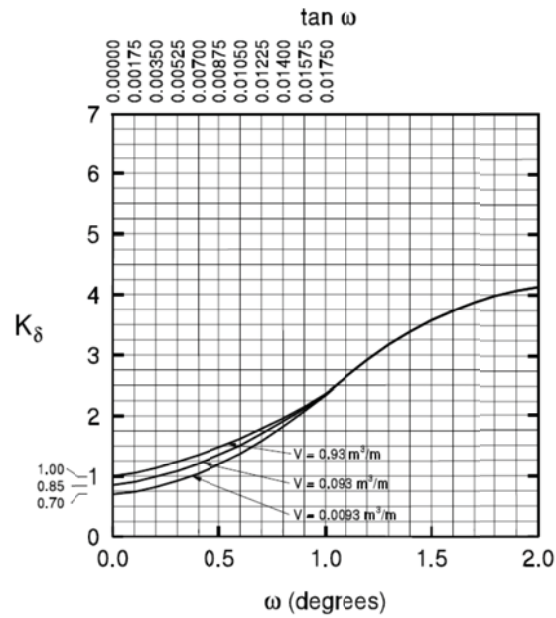
Figure 3.3 Design curve for evaluating K_\delta when \phi = 25^\circ (after Nordlund, 1979)
