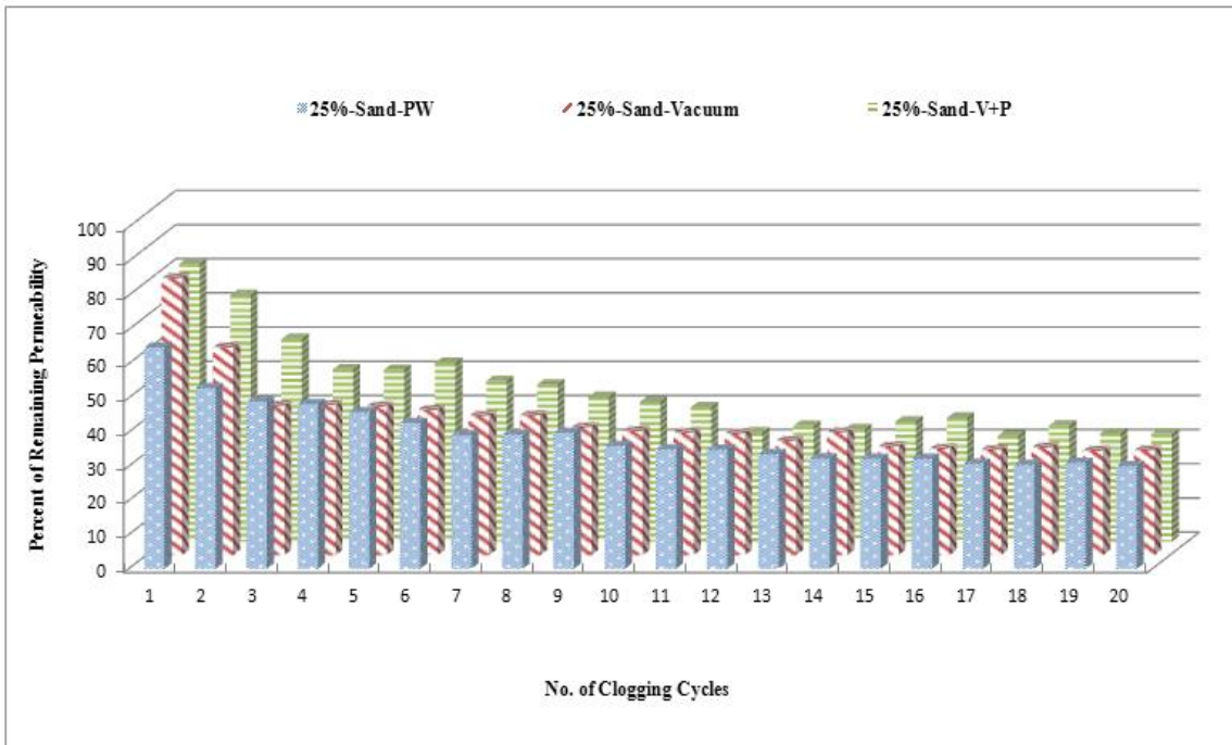
Figure 52. Sand specimens, 25% porosity, cleaned by three rehabilitation methods
