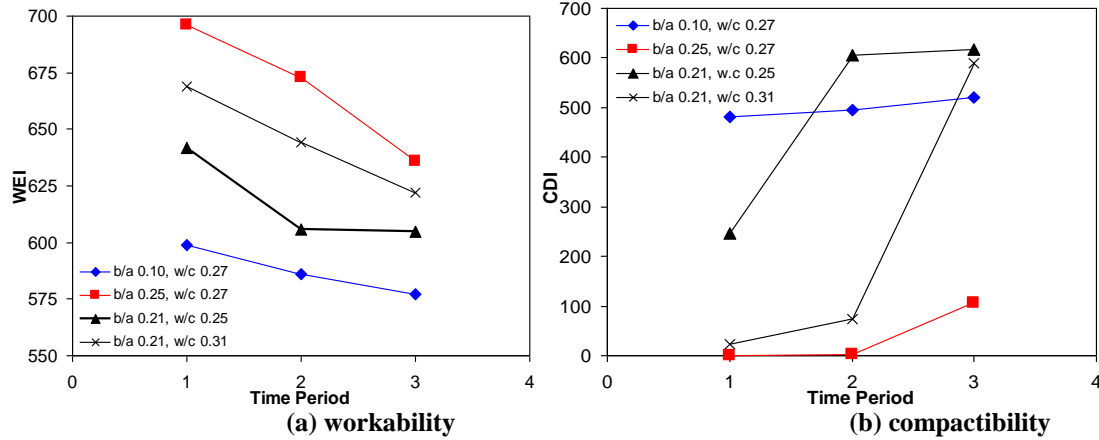
Figure 21. Effect on placeability of mixing time
