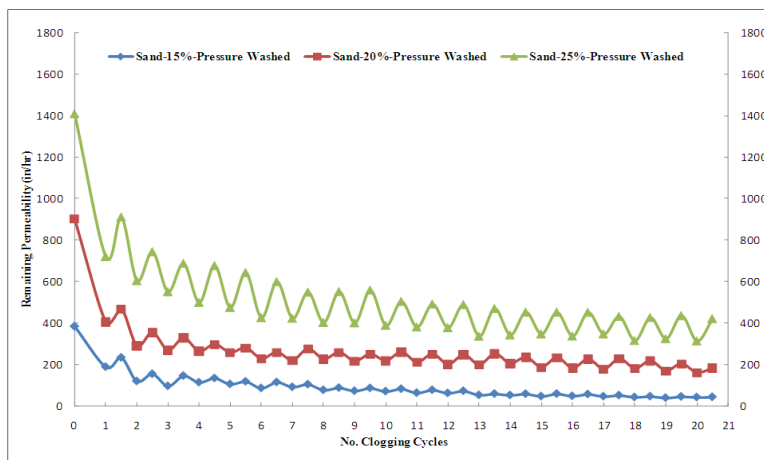
Figure 49. Permeability of specimens subjected to sand sediments and cleaned by pressure washing
