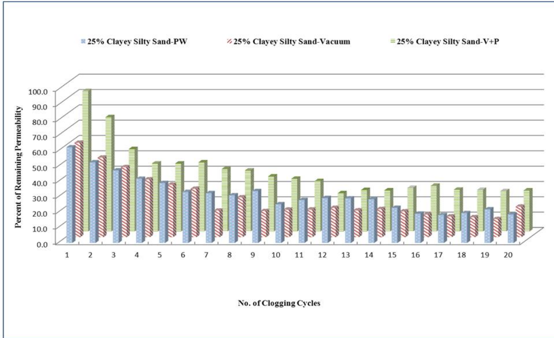
Figure 55. Silty clay sand specimens, 25% porosity, cleaned by three rehabilitation methods
