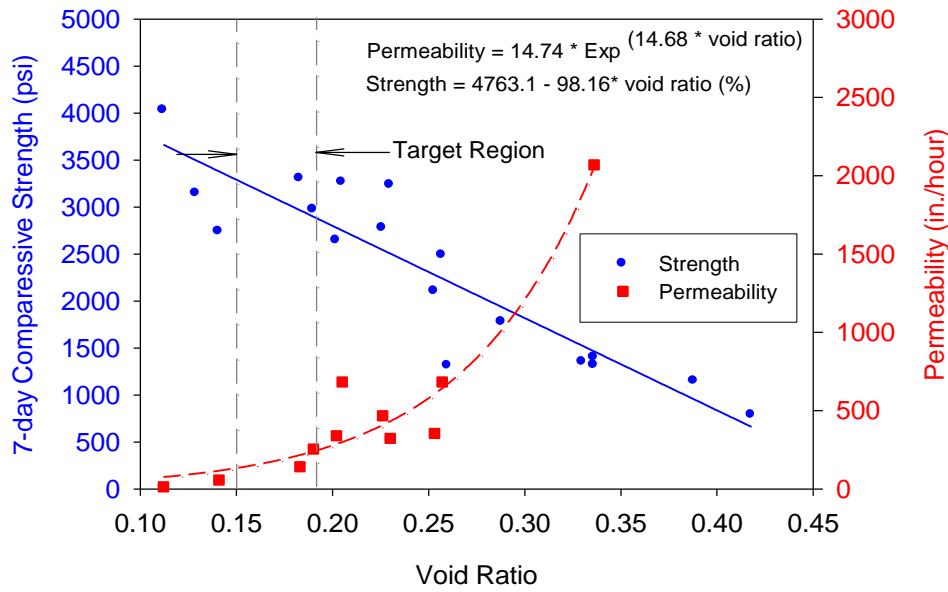
Figure 1. Relationship between pervious concrete void ratio, permeability, and 7-day compressive strength for all mixes placed using regular compaction energy
