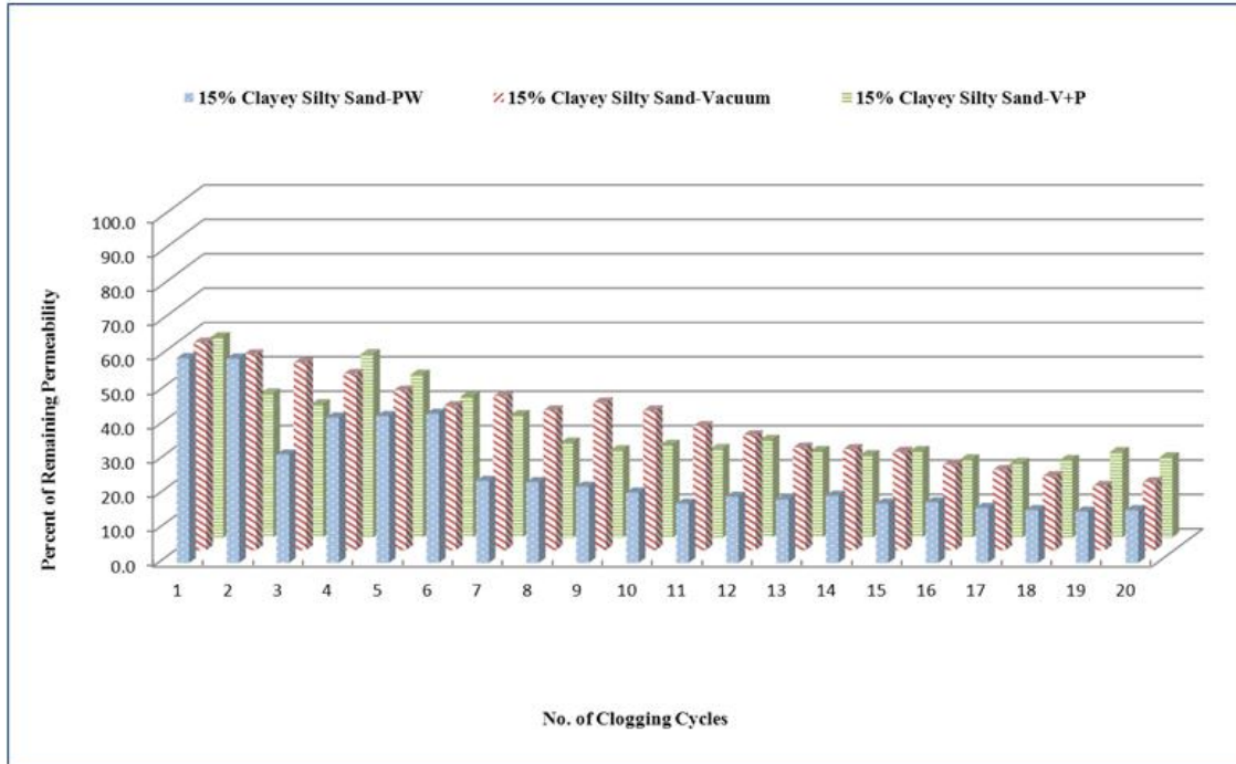
Figure 53. Silty clay sand specimens, 15% porosity, cleaned by three rehabilitation methods
