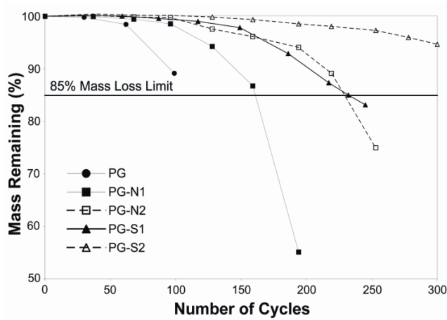
Figure 12. Freeze-thaw durability of the pea gravel mixtures
