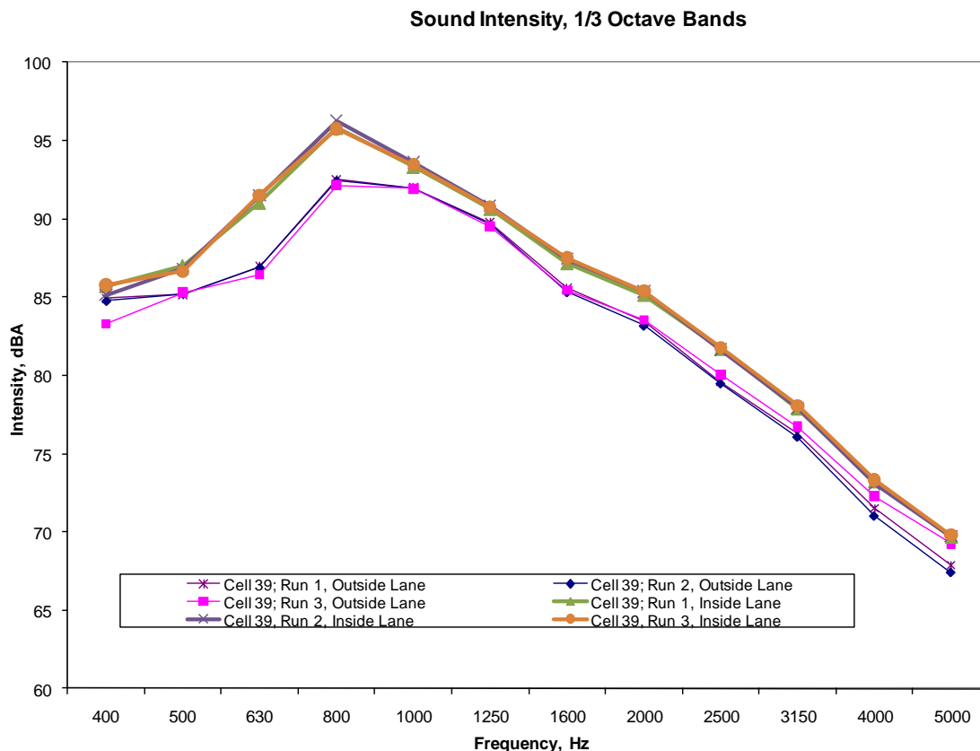
Figure 79. Frequency versus intensity for Cell 39, outside environmental lane and inside traffic lane, July 22, 2009
