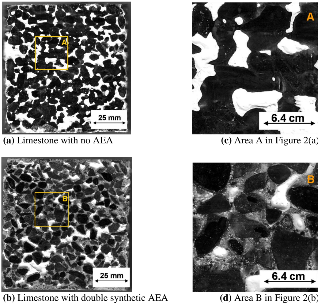
Figure 5. Images of typical pervious concrete samples
