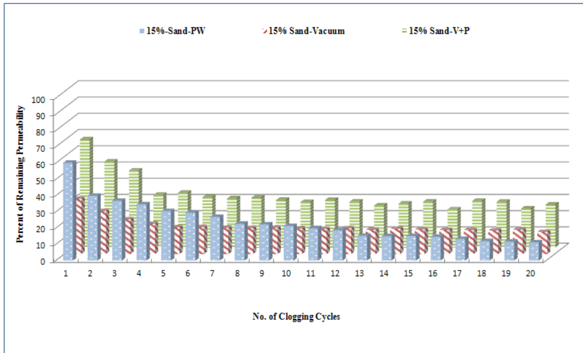
Figure 50. Sand specimens, 15% porosity, cleaned by three rehabilitation methods
