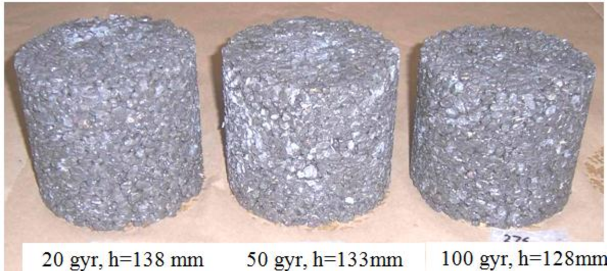
Figure 14. Samples compacted at different gyrations (gyr)
