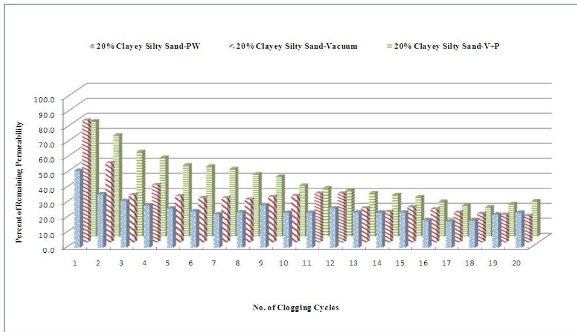
Figure 54. Silty clay sand specimens, 20% porosity, cleaned by three rehabilitation methods
