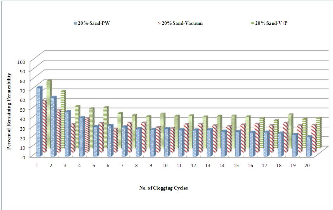
Figure 51. Sand specimens, 20% porosity, cleaned by three rehabilitation methods
