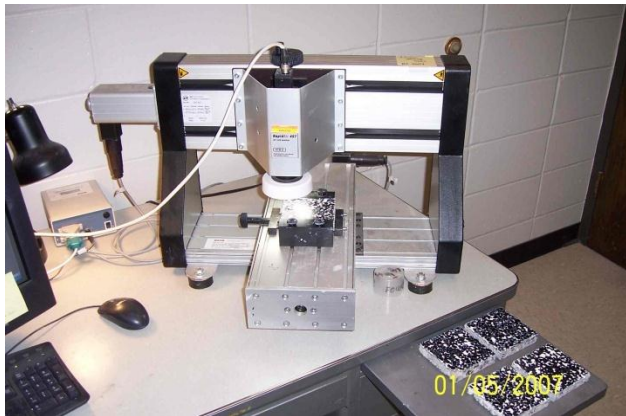
Figure 4. RapidAir device
