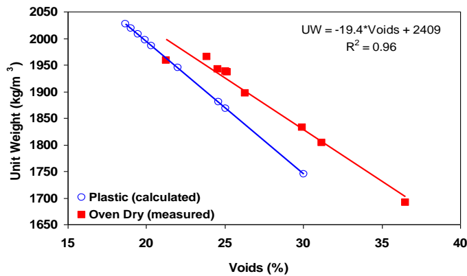
Figure 16. Relationship between voids and unit weight of pervious concrete samples made with gyrotory compaction
