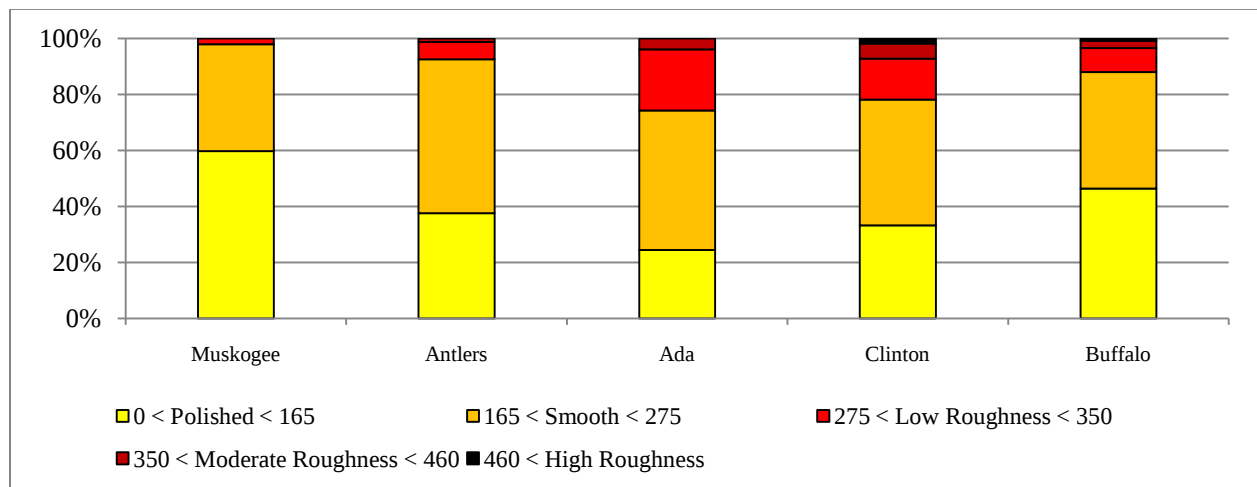
Figure 25. Details of Texture Index of Division Aggregates
