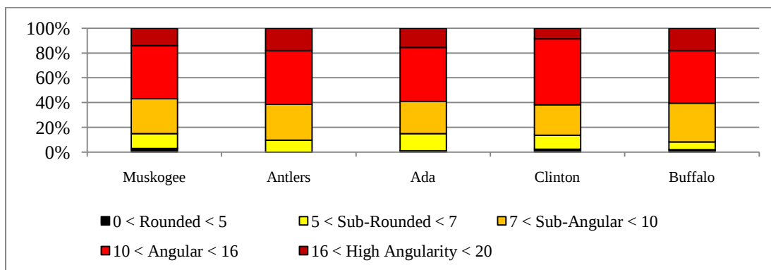
Figure 23. Details of Radius Angularity Index of Division Aggregates
