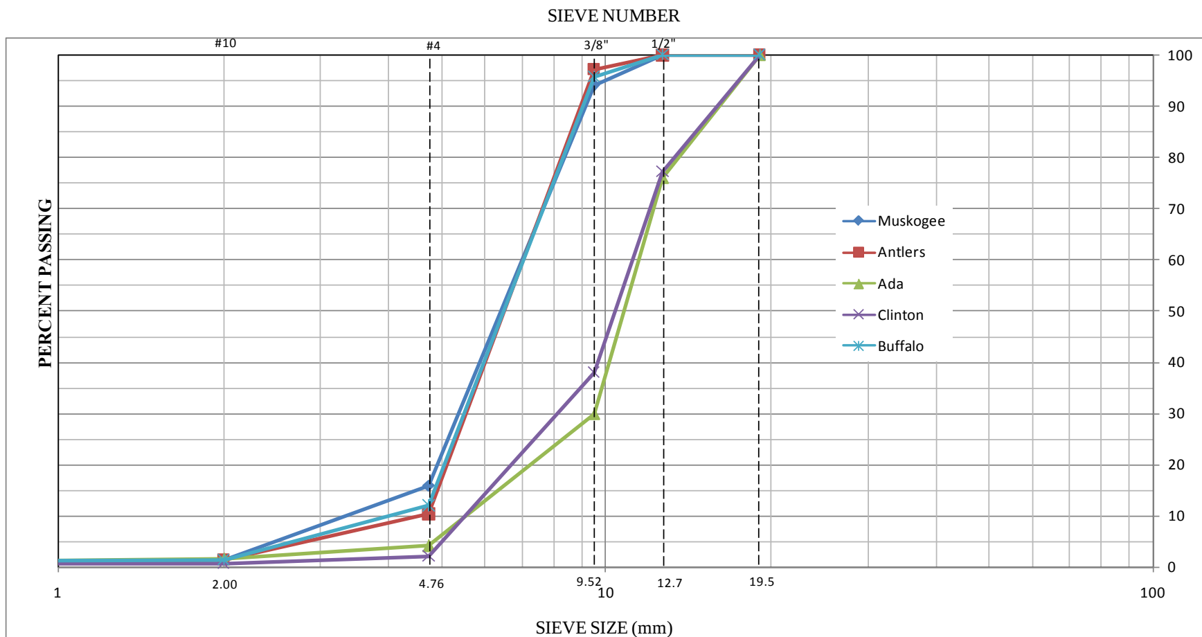
Figure 12 Gradation Curves of Division Aggregates
