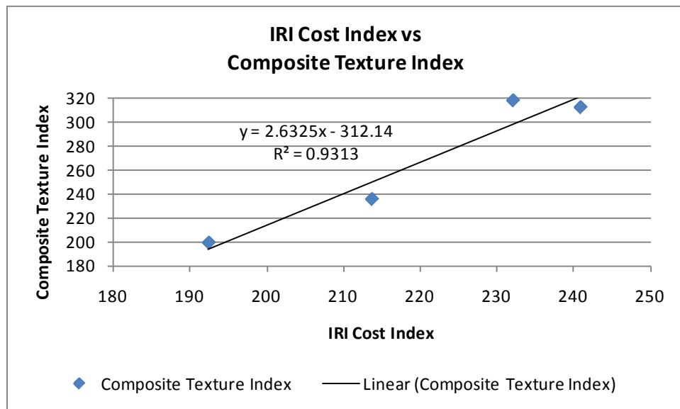
Figure 26. IRI Cost Index Regressed with Composite Texture Index.
