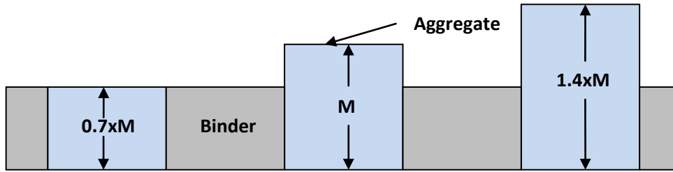
Figure 2: Schematic of McLeod's Failure Criteria (after Lee and Kim 2009).
