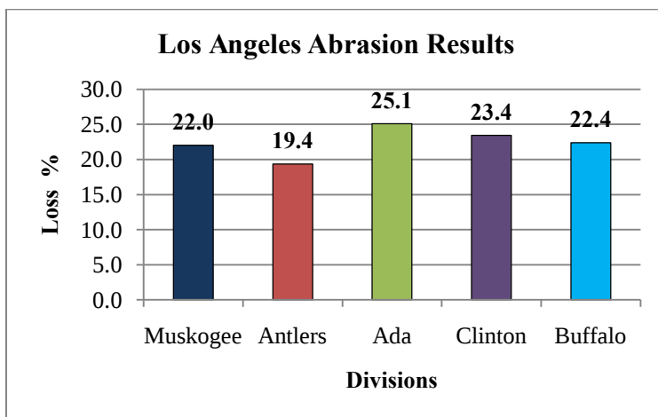
Figure 13. LA Abrasion Test Results
