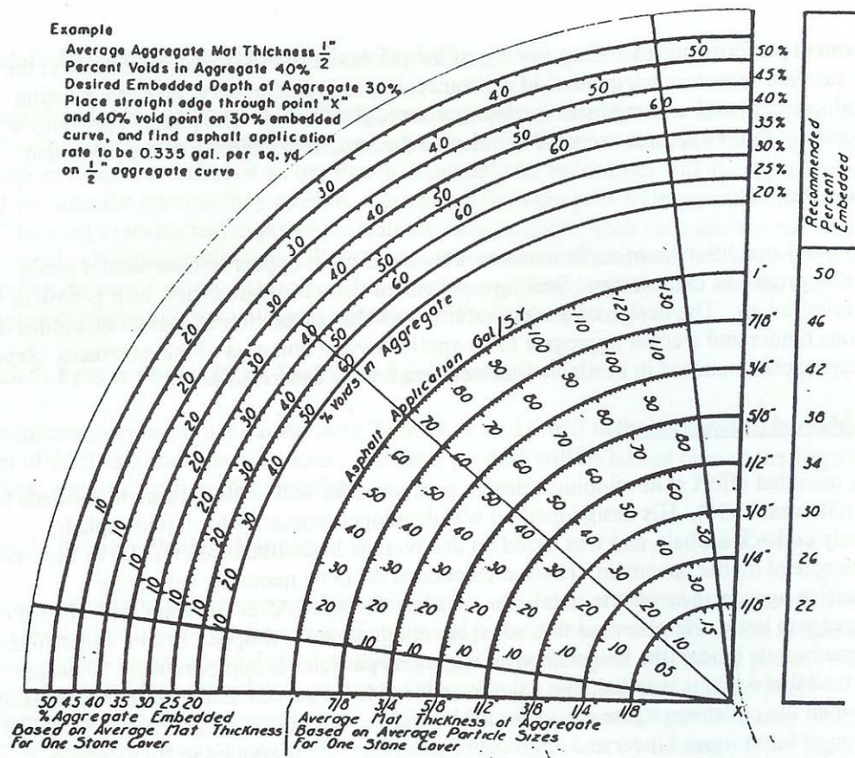
Figure 1: Nomograph to determine asphalt cement application rate in seal coats and one course surface treatments (Kearby 1953).
