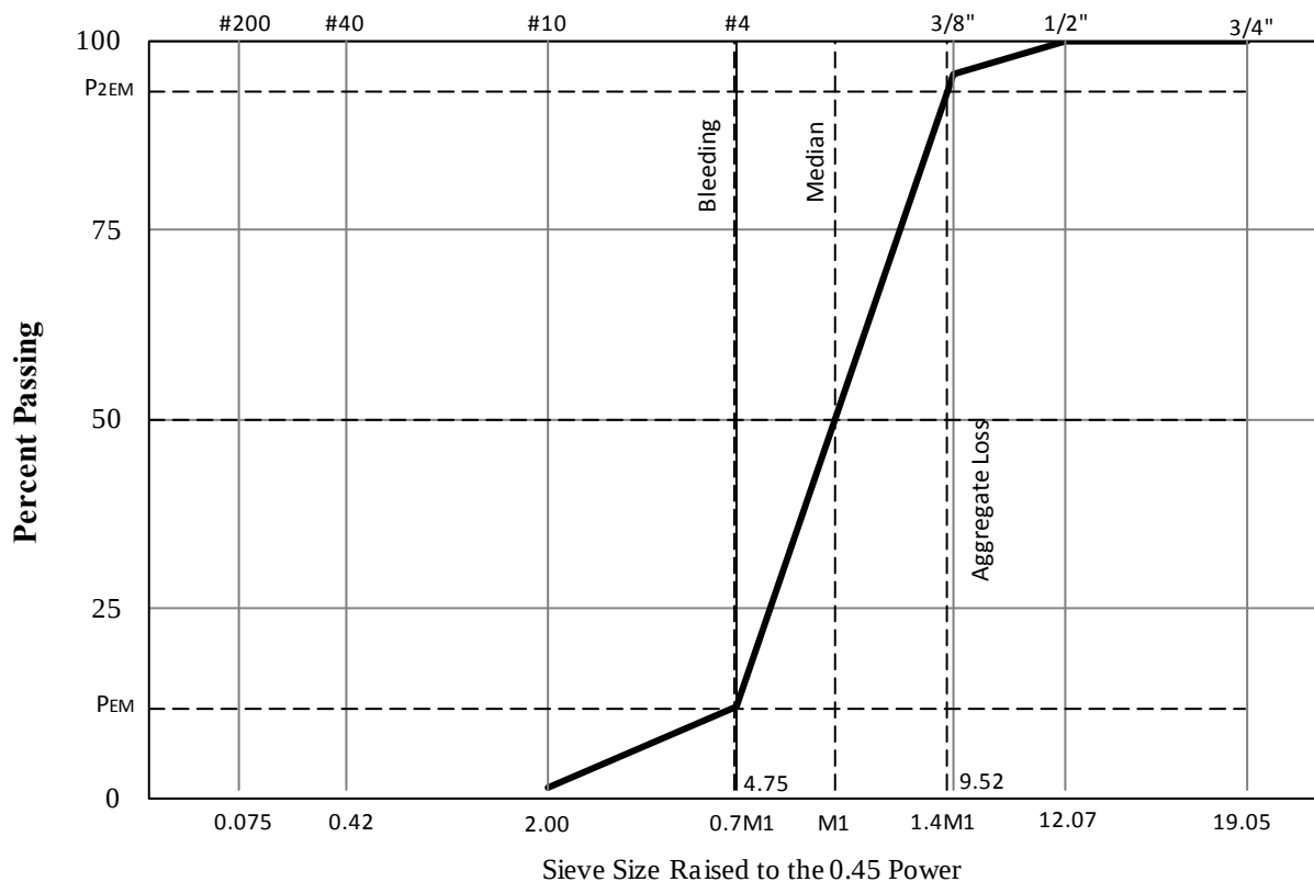
Figure 3: Gradation Range to Maximize Performance (after Lee and Kim 2009)
