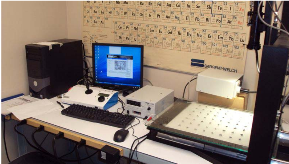
Figure 4: Aggregate Imaging System in OU Lab
