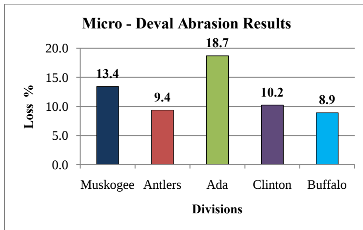
Figure 14. Micro-Deval Abrasion Test Results
