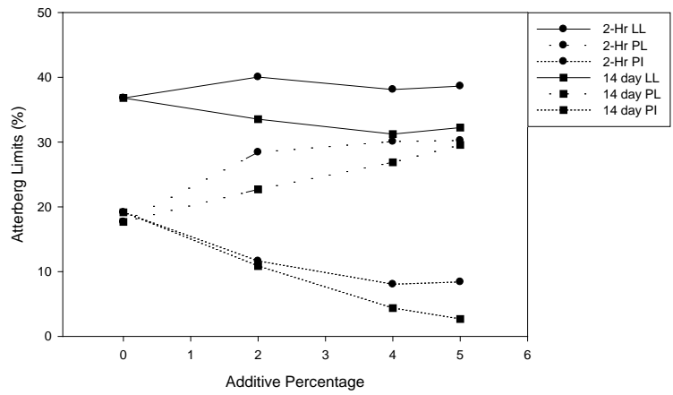
Figure A.38: Ashport-Grainola (A-6) Atterberg Limits with Lime
