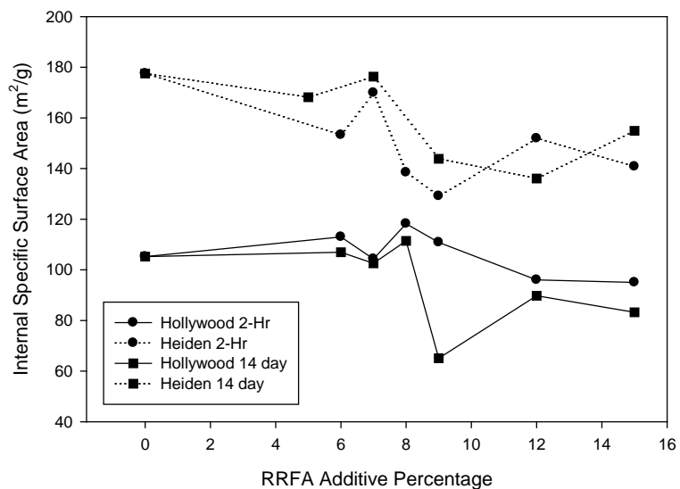
Figure A.135: Internal SSA Curves for A-7-6 Soils with Red Rock FA
