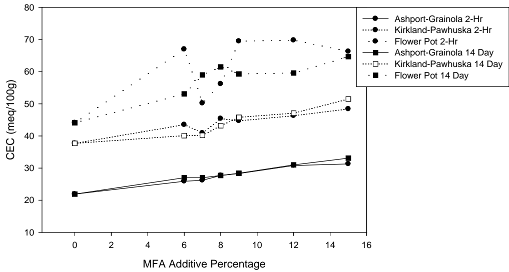
Figure A.104: Cation Exchange Capacity Curves for A-6 Soils with Muskogee FA
