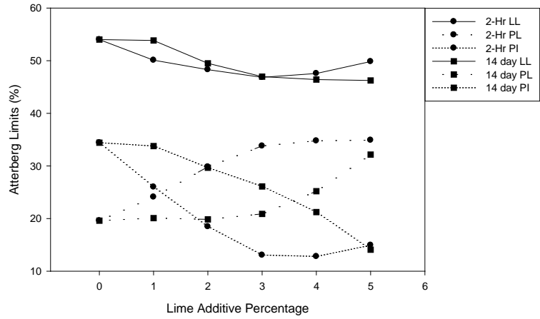
Figure A.50: Hollywood (A-7-6) Atterberg Limits with Lime
