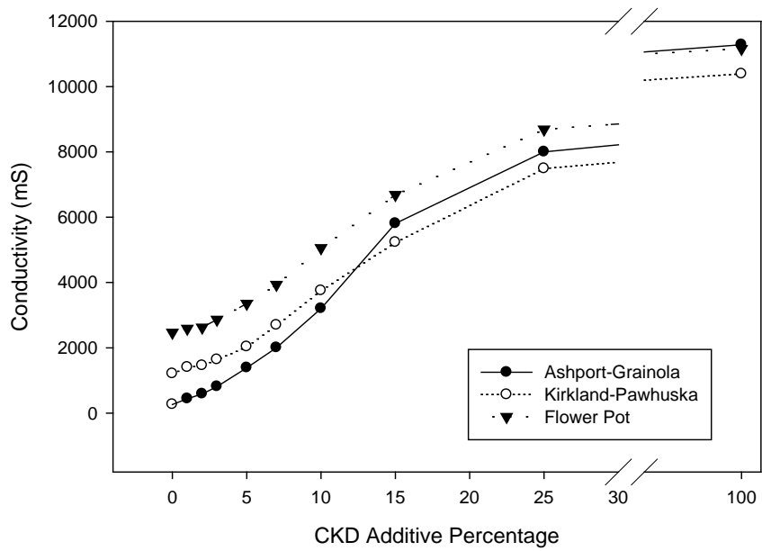
Figure A.87: Conductivity Curves for A-6 Soils with CKD
