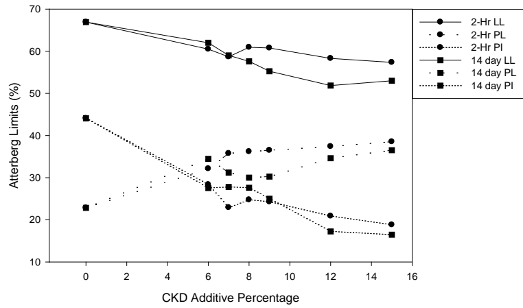
Figure A.53: Heiden (A-7-6) Atterberg Limits with CKD
