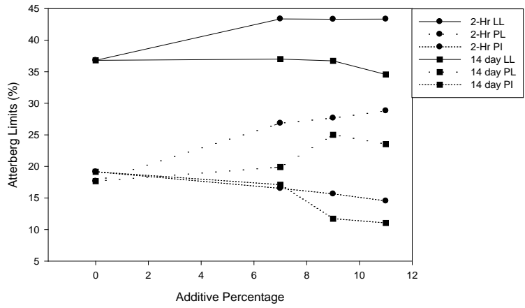
Figure A.37: Ashport-Grainola (A-6) Atterberg Limits with CKD
