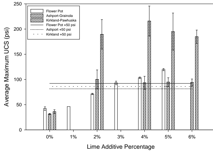
Figure 22: UCS Plots for A-6 Soils with Lime
