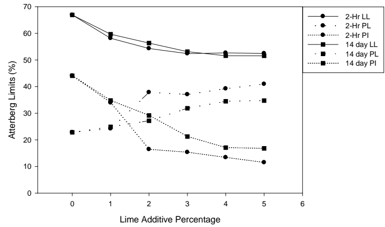
Figure A.54: Heiden (A-7-6) Atterberg Limits with Lime
