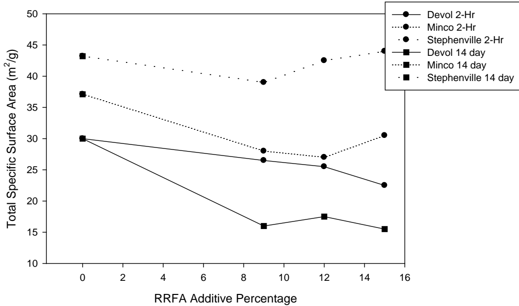
Figure A.112: Total SSA Curves for A-4 Soils with Red Rock FA
