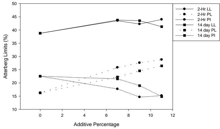
Figure A.41: Kirkland-Pawhuska (A-6) Atterberg Limits with CKD
