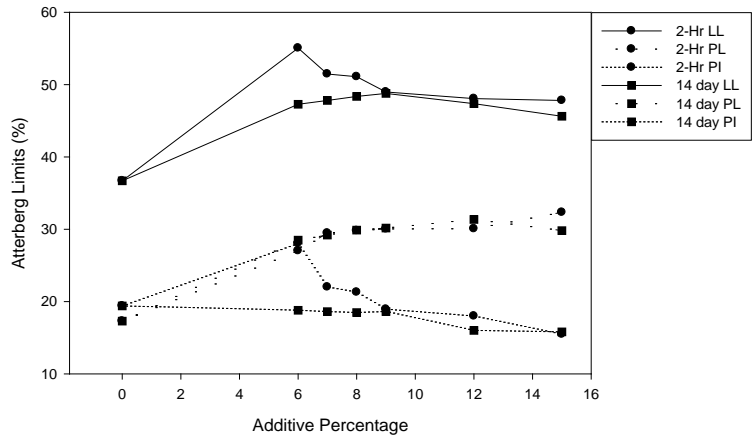
Figure A.45: Flower Pot (A-6) Atterberg Limits with CKD
