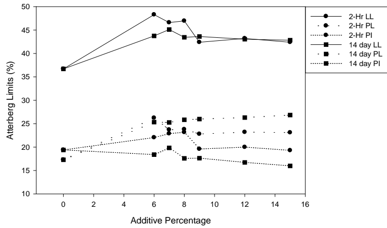
Figure A.47: Flower Pot (A-6) Atterberg Limits with Red Rock FA
