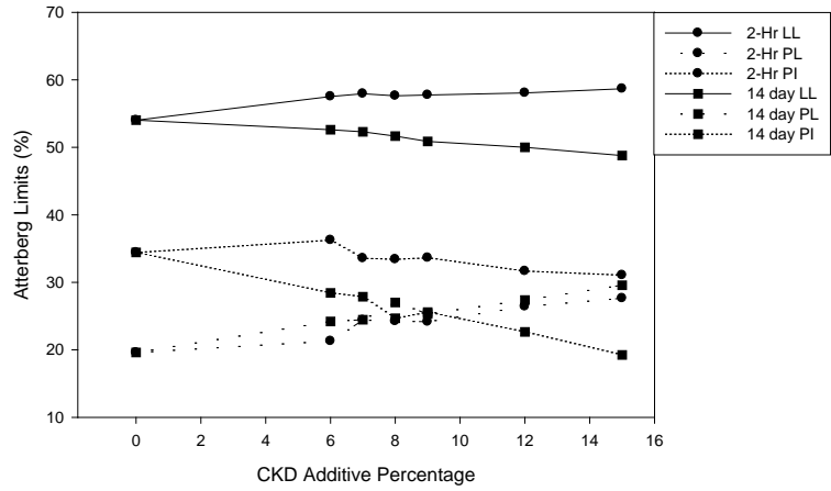
Figure A.49: Hollywood (A-7-6) Atterberg Limits with CKD
