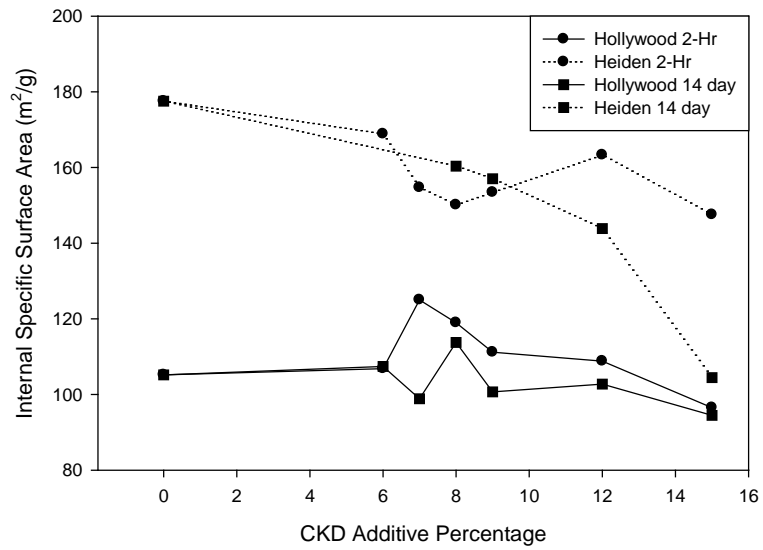
Figure A.129: Internal SSA Curves for A-7-6 Soils with CKD
