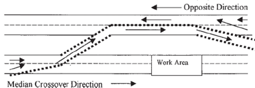
Exhibit 16: Crossover Work Zone. (27)
