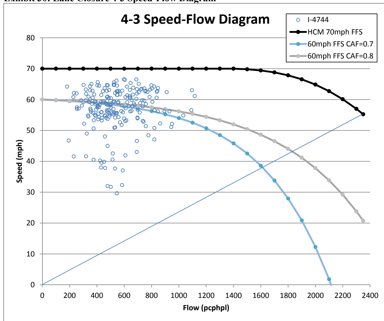
Exhibit 30: Lane Closure 4-3 Speed-Flow Diagram
