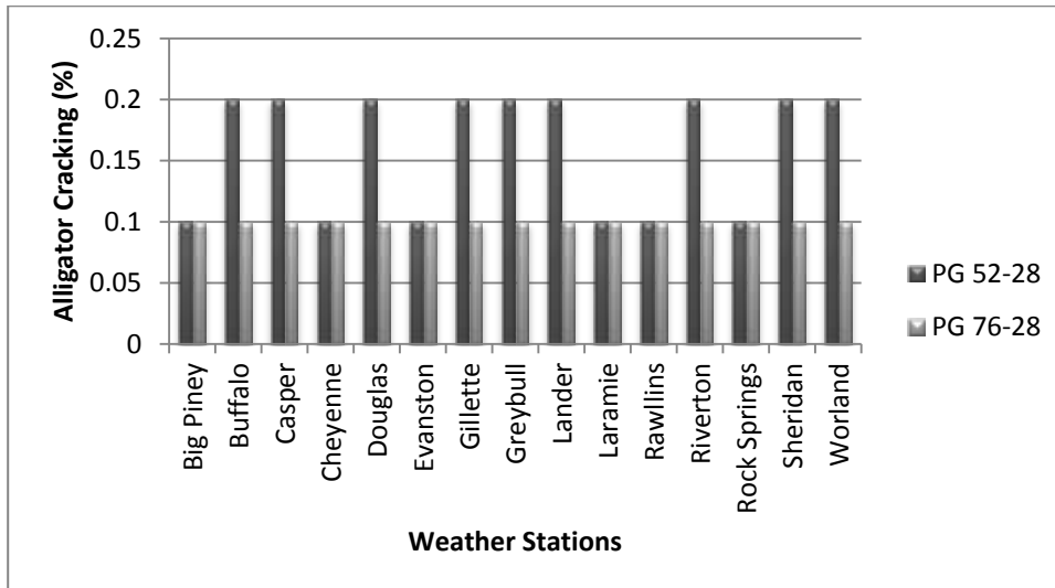
Figure 5.14 Alligator cracking values for various weather stations.
