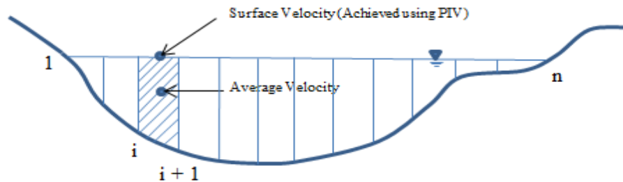
Figure 3.9 Depiction of subareas associated with interrogation points used for discharge calculations
