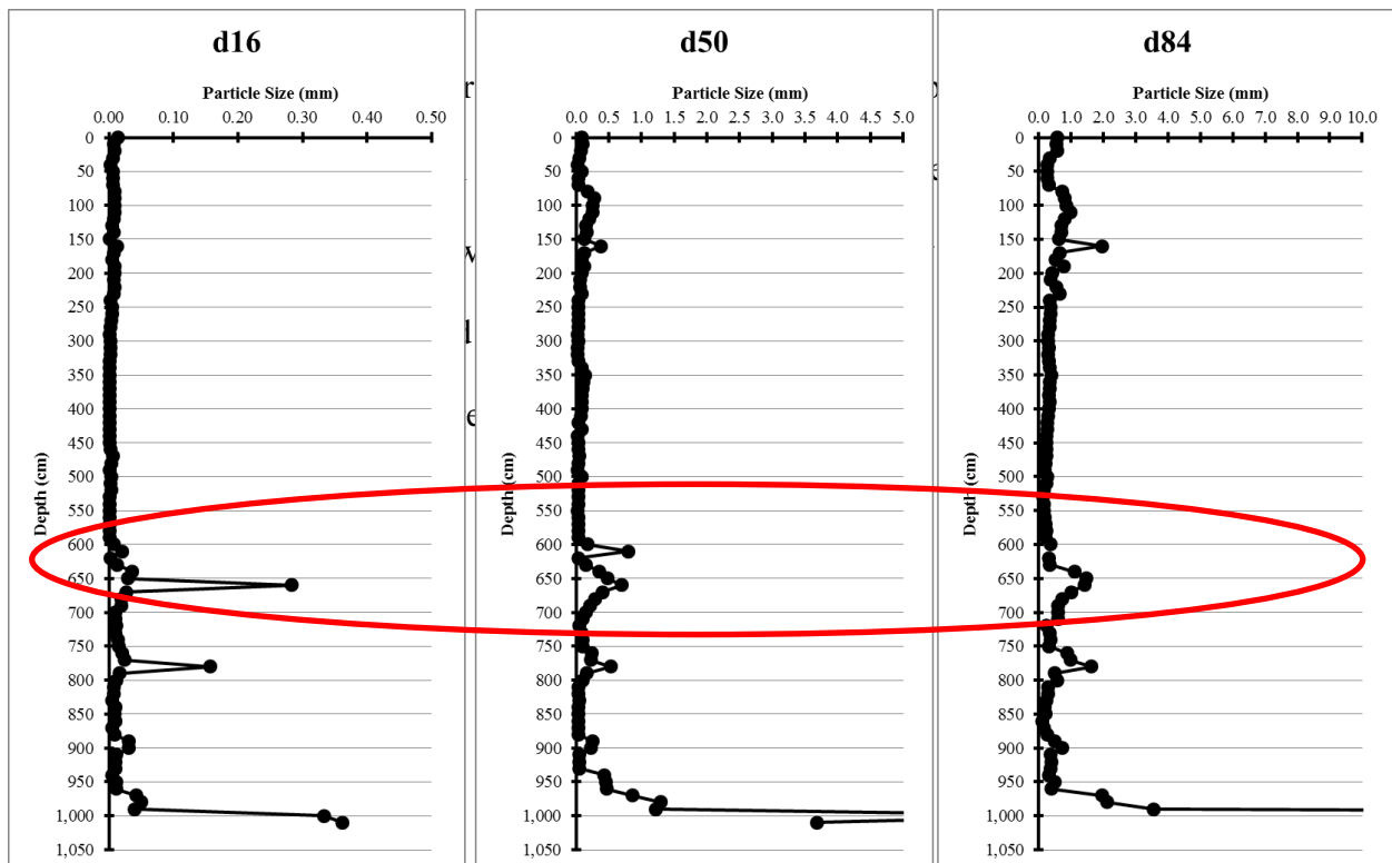
Figure 4.2 Particle size distribution. These graphs show key particle size diameters of the sampled depth intervals in a stream bank core from the study site. The d16, d50, and d84 for each interval are plotted relative to depth. The red circle highlighting the 600–650 cm depth interval corresponds to a coarsening of the overall particle size distribution, as there are increases in the d50 and d84. This elevation corresponds to the top elevation of the knickpoint face.
