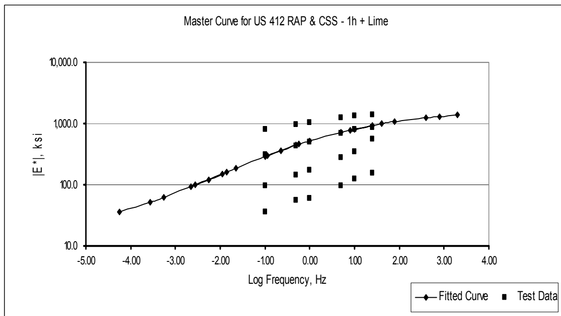
FIGURE 31 Master curve for US 412 RAP and CSS-1h+Lime emulsion.
