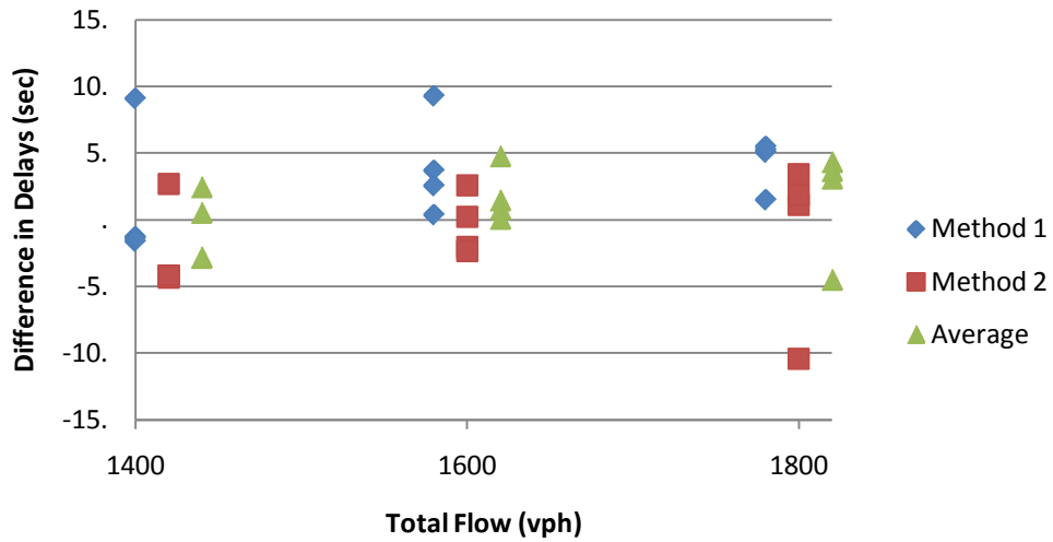
Double Lane (50 In, 50 Out)
