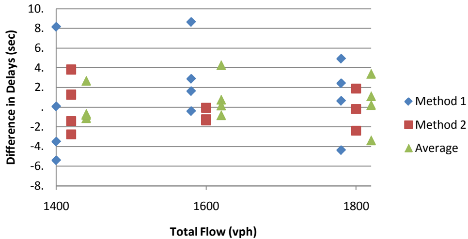
Double Lane (0 In, 100 Out)
