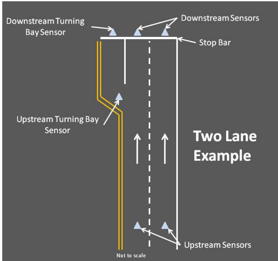
Figure 3-4: Two Lane Example of Left Turning Bay.
