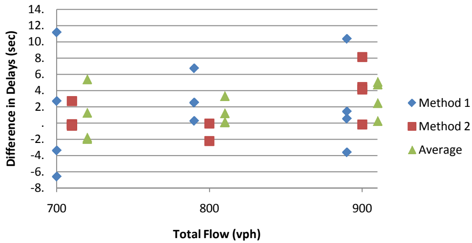
Single Lane (100 In, 100 Out)
