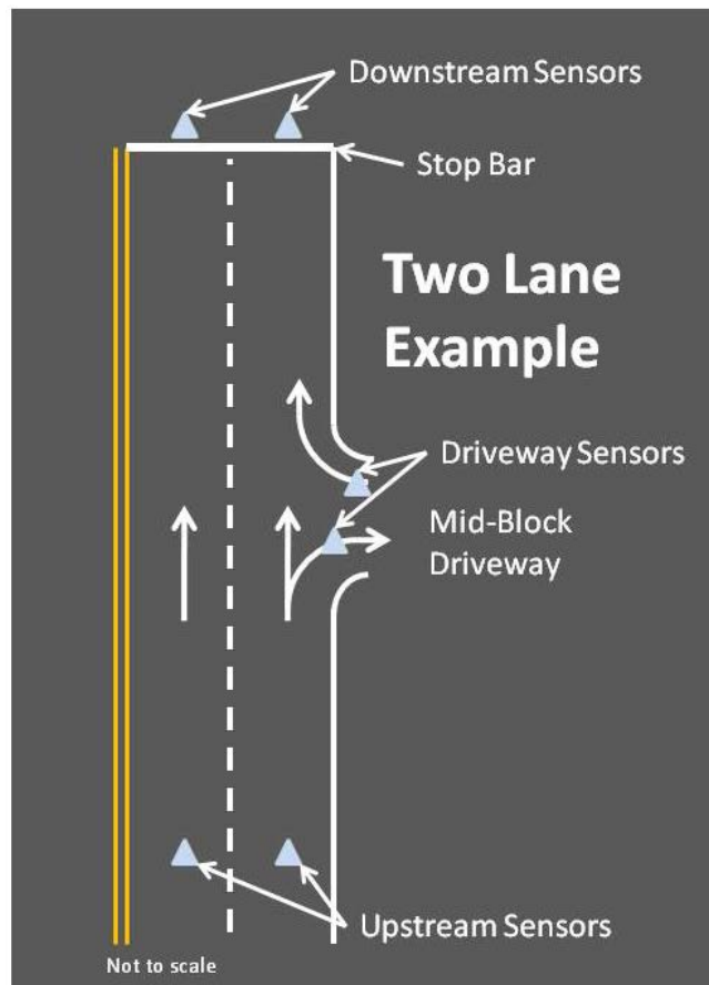
Figure 3-3: Two Lane Example of Mid-block Driveway with Driveway Sensors.
