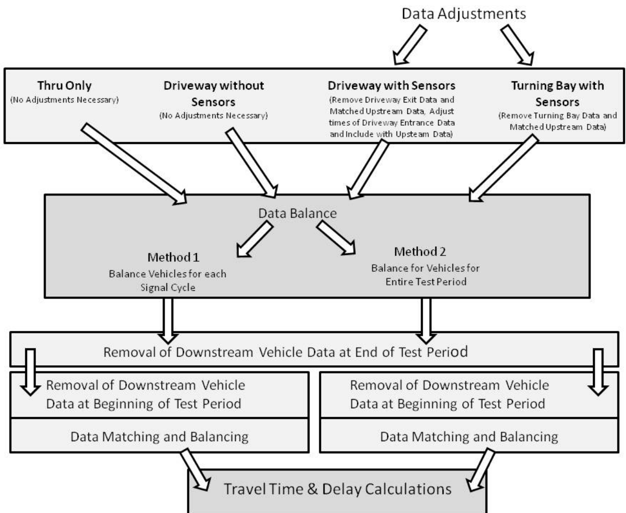
4-5. Flow Chart of Algorithm Processes.
