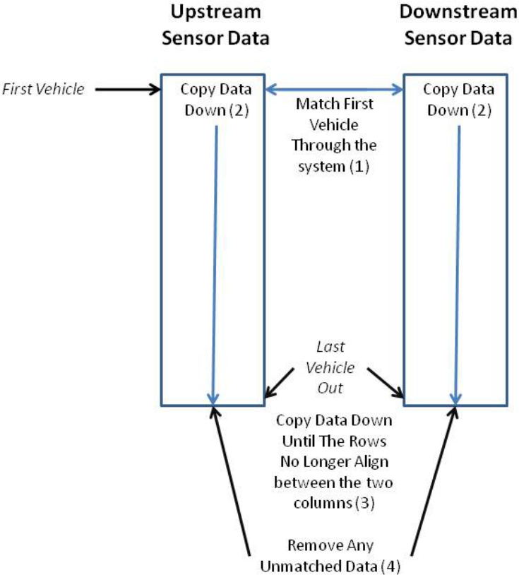
Figure 4-4: Method 2 Final Vehicle Data Balancing.
