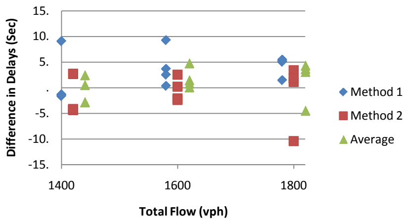
Figure 5-8: Double Driveway without Sensors (50 In, 50 Out).
