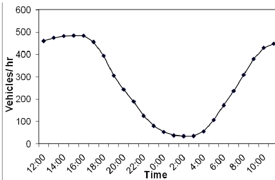
Figure 4. Hourly traffic volume (vehicles/hr) by hour along US 89, Arizona from 2007 to 2008, determined by an automatic traffic recorder installed in 2007.
