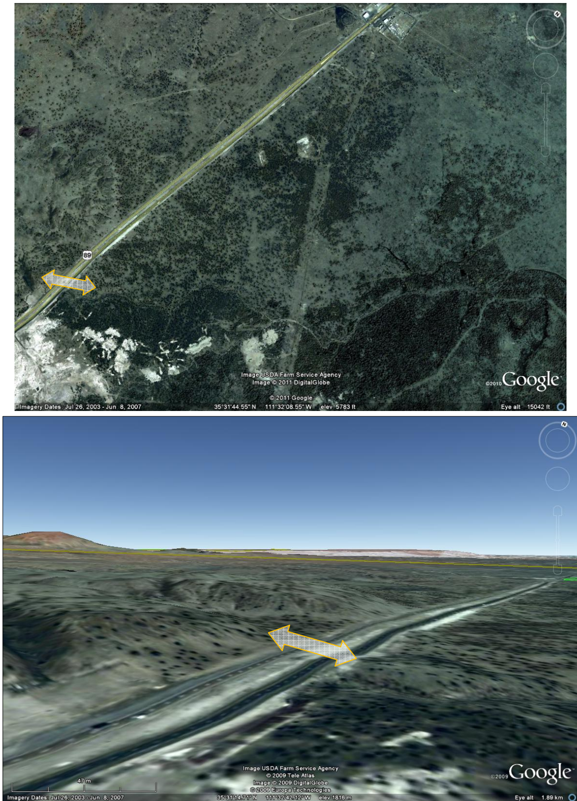
Figure 13. Aerial view (top) and enlarged oblique view (bottom) from GoogleEarth© depicting the proposed Coconino NF - Antelope Hills pronghorn passage structure site on US 89 between MP 440.6 and 441.1.
