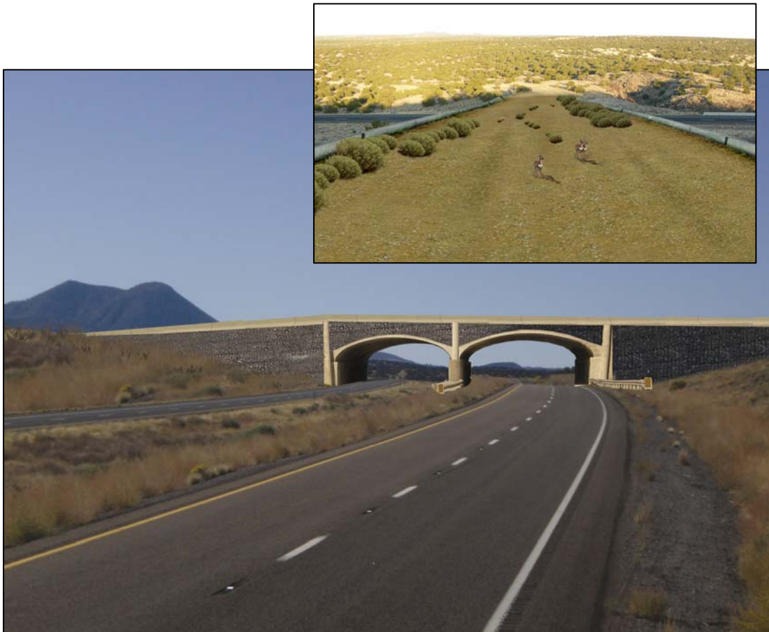
Figure 17. Rendering of a CON/SPAN ® pre-cast concrete arch application for a wildlife overpass at MP 440.9 along US 89. The bottom rendering depicts separate 32-ft spans (21 ft high) over each set of lanes, looking south, and the inset depicts the top of the overpass, looking east (note: fencing would need to be erected atop the walls).
