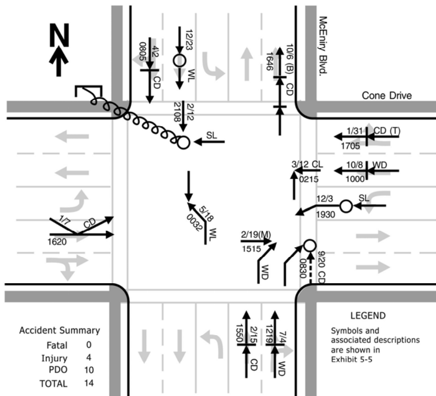
Figure 3-4. Example collision diagram (AASHTO 2010).
