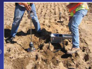
Light Weight Deflectometer (Model: Zorn ZFG2000)
