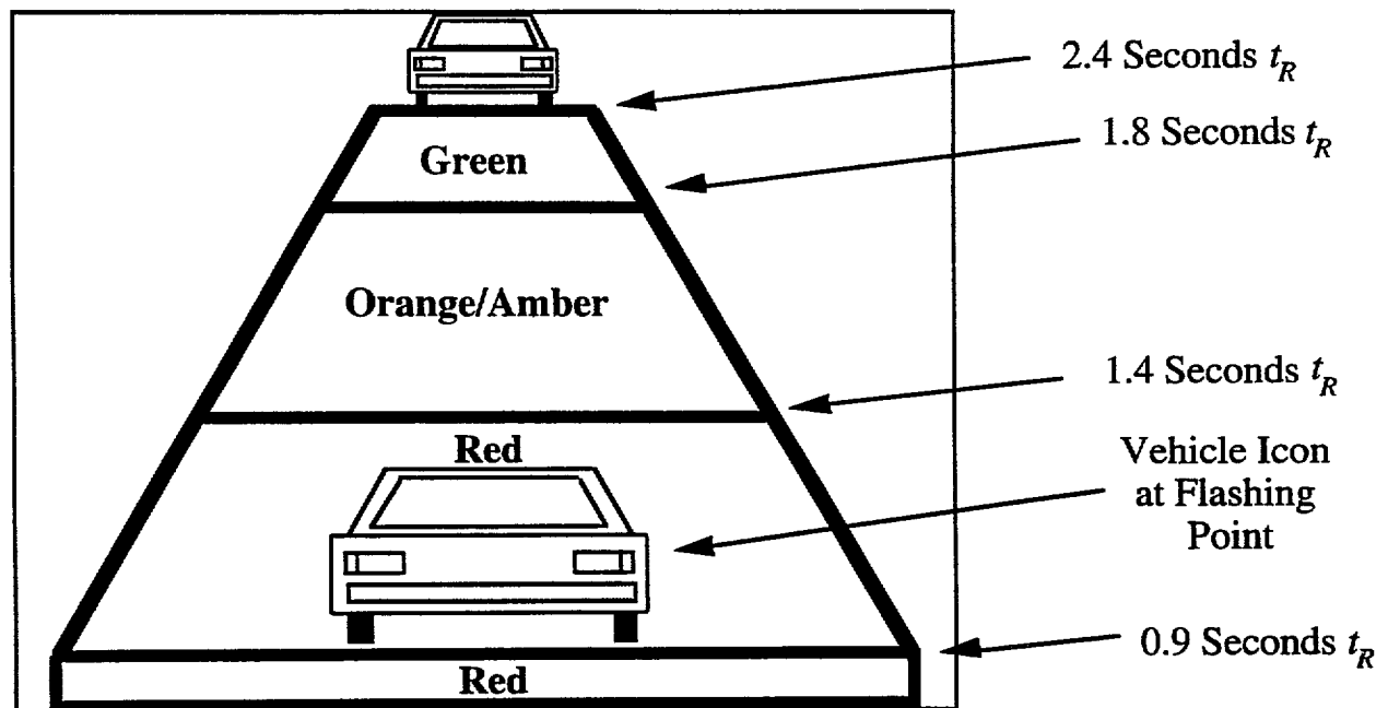
Figure 3.1-1 McGehee et al. (1992) Perspective Car Icon Display
