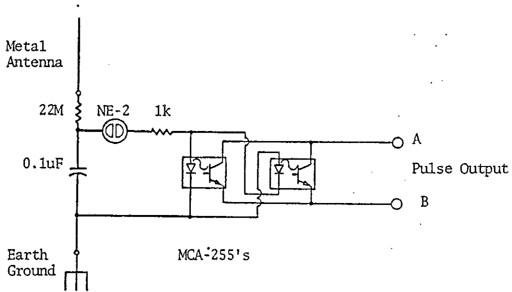
Figure 4. Experimental Electrostatic Blowing Dust Sensor
