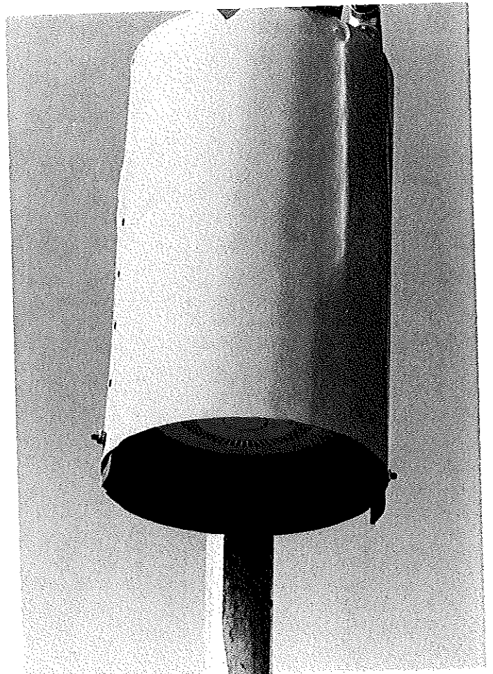
Figure 8. Recessed Smoke Alarm Chamber
