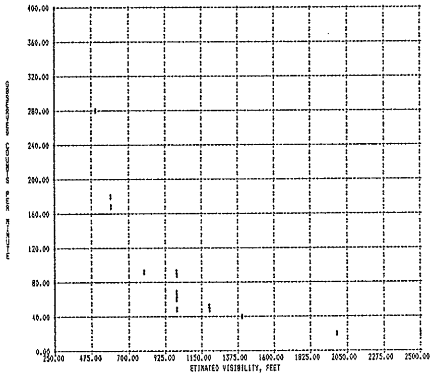
Figure 5. Electrostatic Sensor Response
