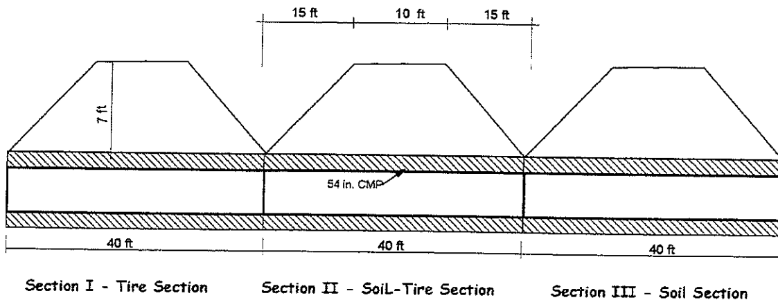
Figure 8. Longitudinal cross section of the test embankment
