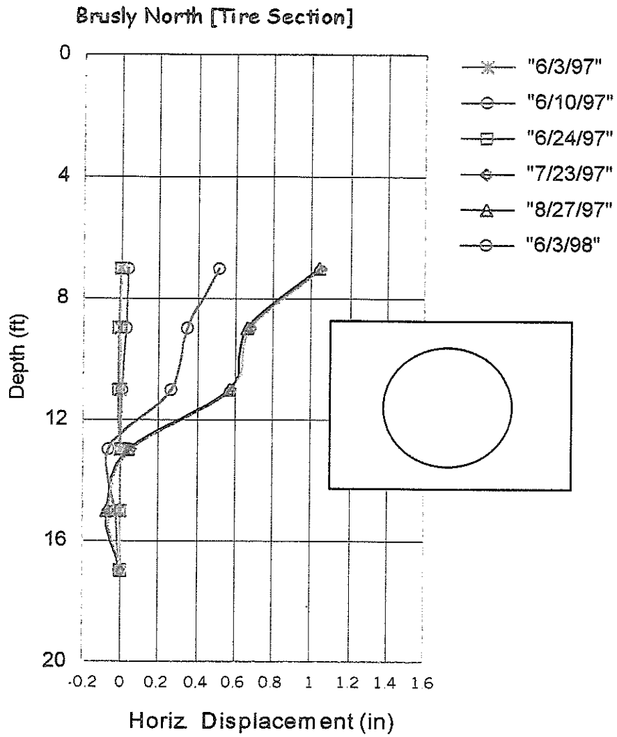
Figure 18. Horizontal soil displacement near the pipe in the tire section
