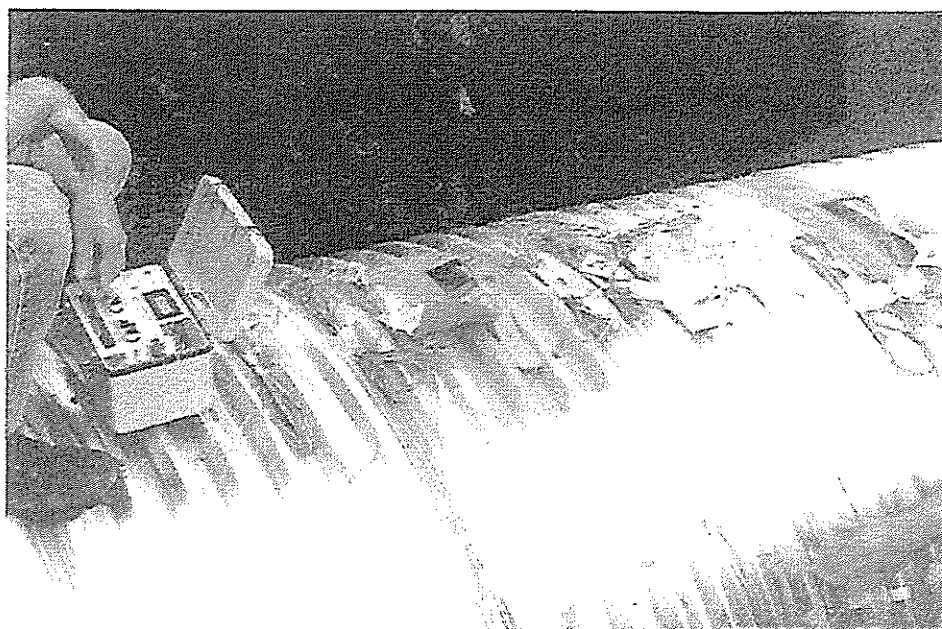
Figure 17. Initial reading of the strain gages in the field
