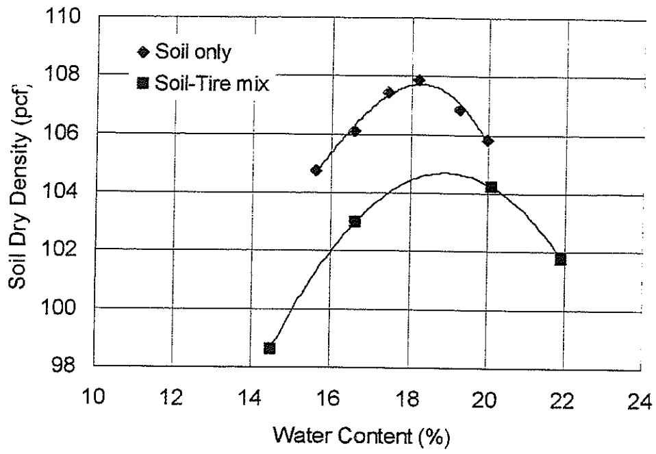
Figure 6. Moisture-Density relationship of the soil and the soil-tire mix
