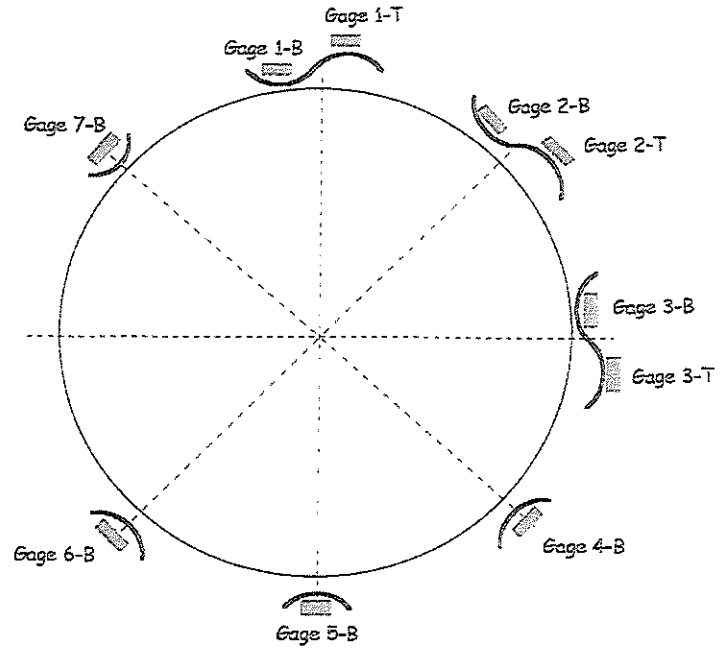
Figure 14. Schematic of the locations of strain gages in the Field
