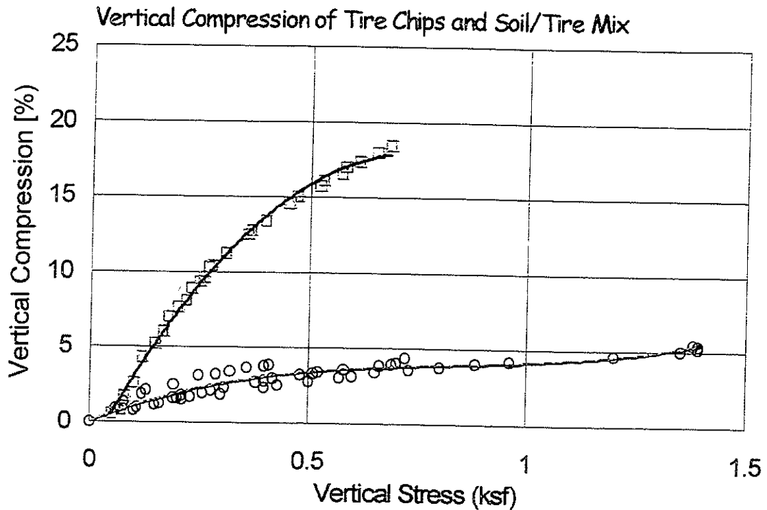
Figure 3. Compressibility of tire chips and soil-tire mix
