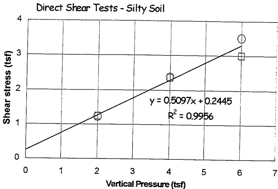
Figure 4. Direct shear test results on the silty-clay soil
