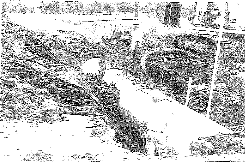
Figure 9. Placement of tire chips around the pipe
