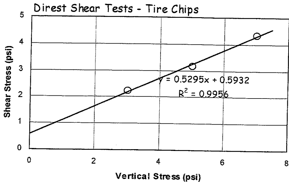
Figure 2. Direct shear test results on the tire chips
