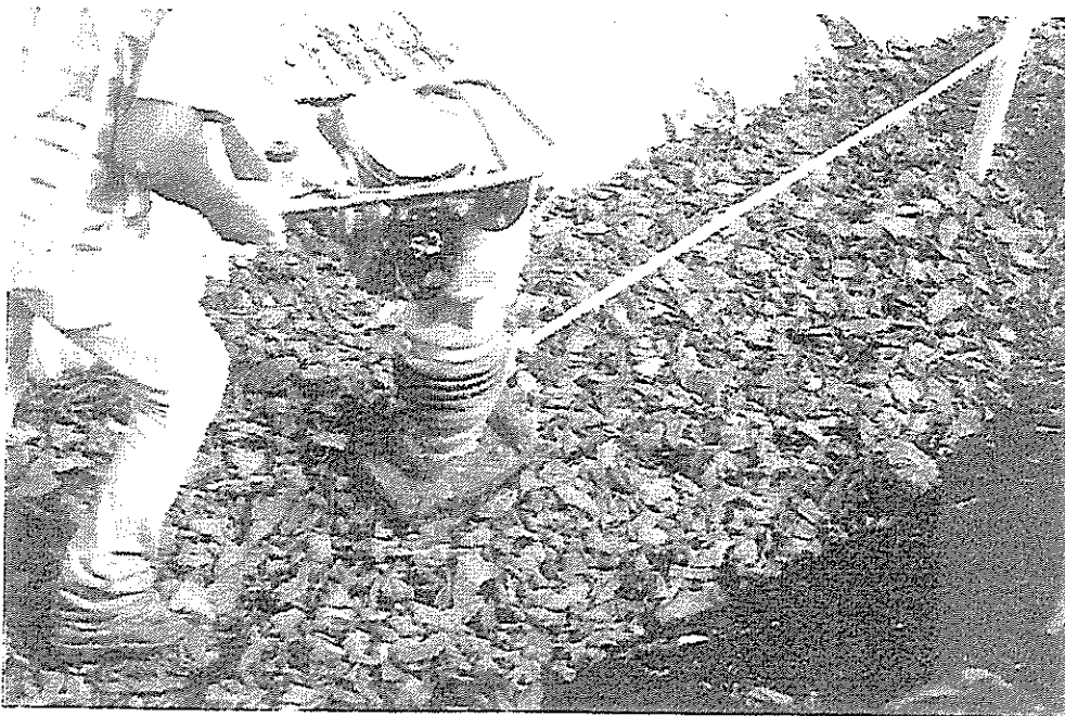
Figure 10. Compaction of the tire chips around the pipe
