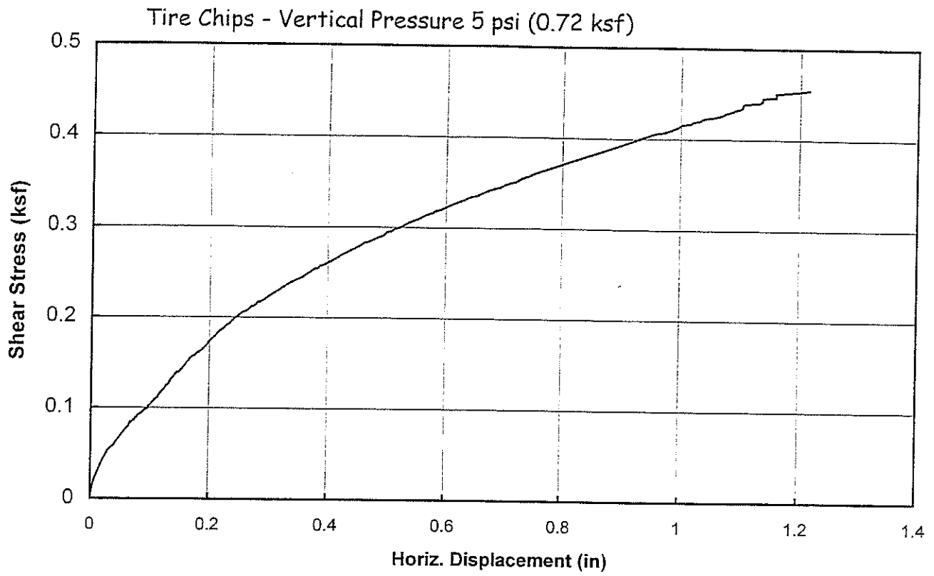
Figure A-2 Direct shear tests on tire chips
