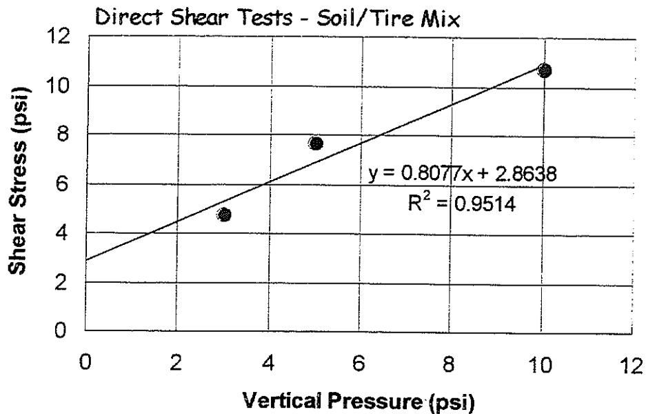
Figure 5. Direct shear test results on the soil-tire mix
