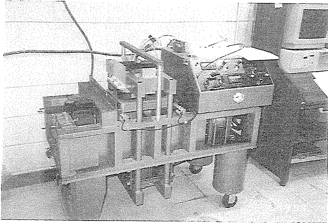
Figure 1. View of the large direct shear testing apparatus
