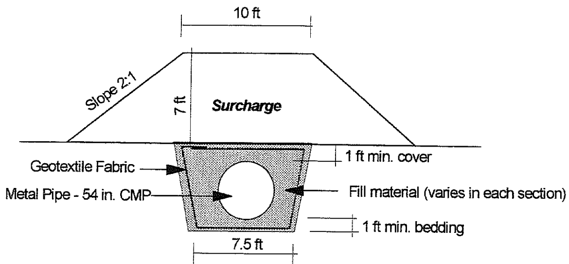
Figure 7. Typical cross section of the test embankment
