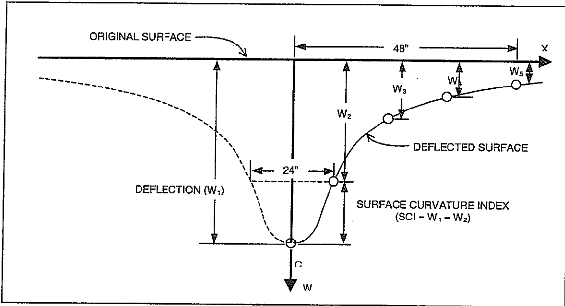
Figure 2 Typical DYNAFLECT Deflection Bowl
