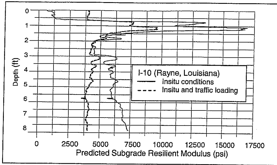
Figure 4 Resilient Modulus Predicted by CPT Model for Cohesive Soil
