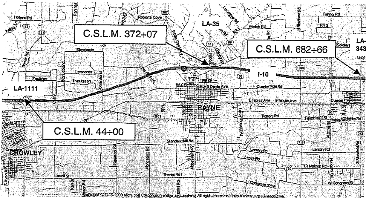
Figure 1 Site Plan
