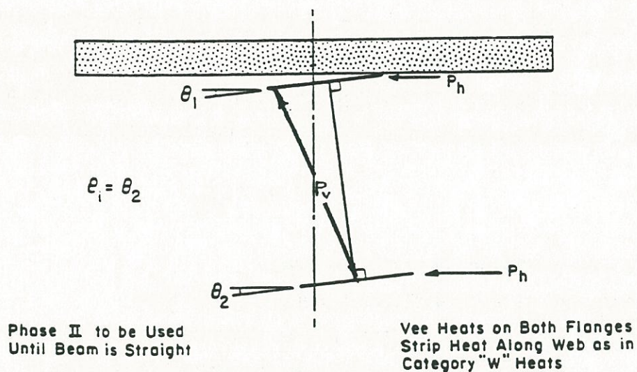
(b) SET-UP FOR PHASE II
