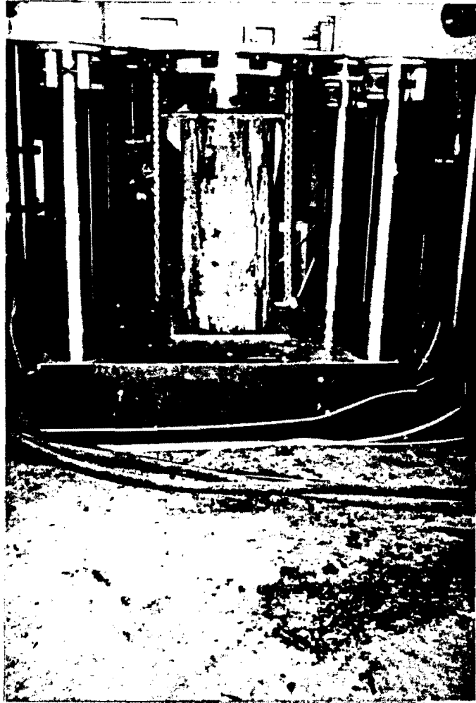
Figure 7 Example of crushing failure in Pile 8B
