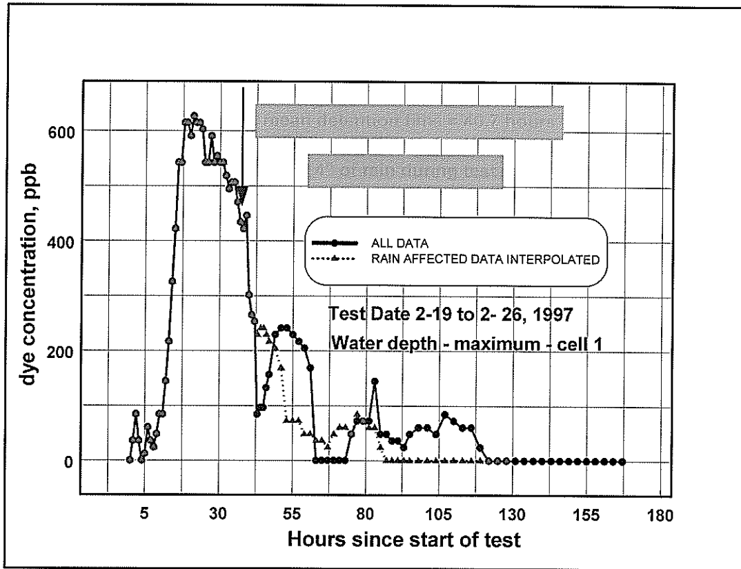
Figure 12 Tracer test - cell 3 - maximum water depth
