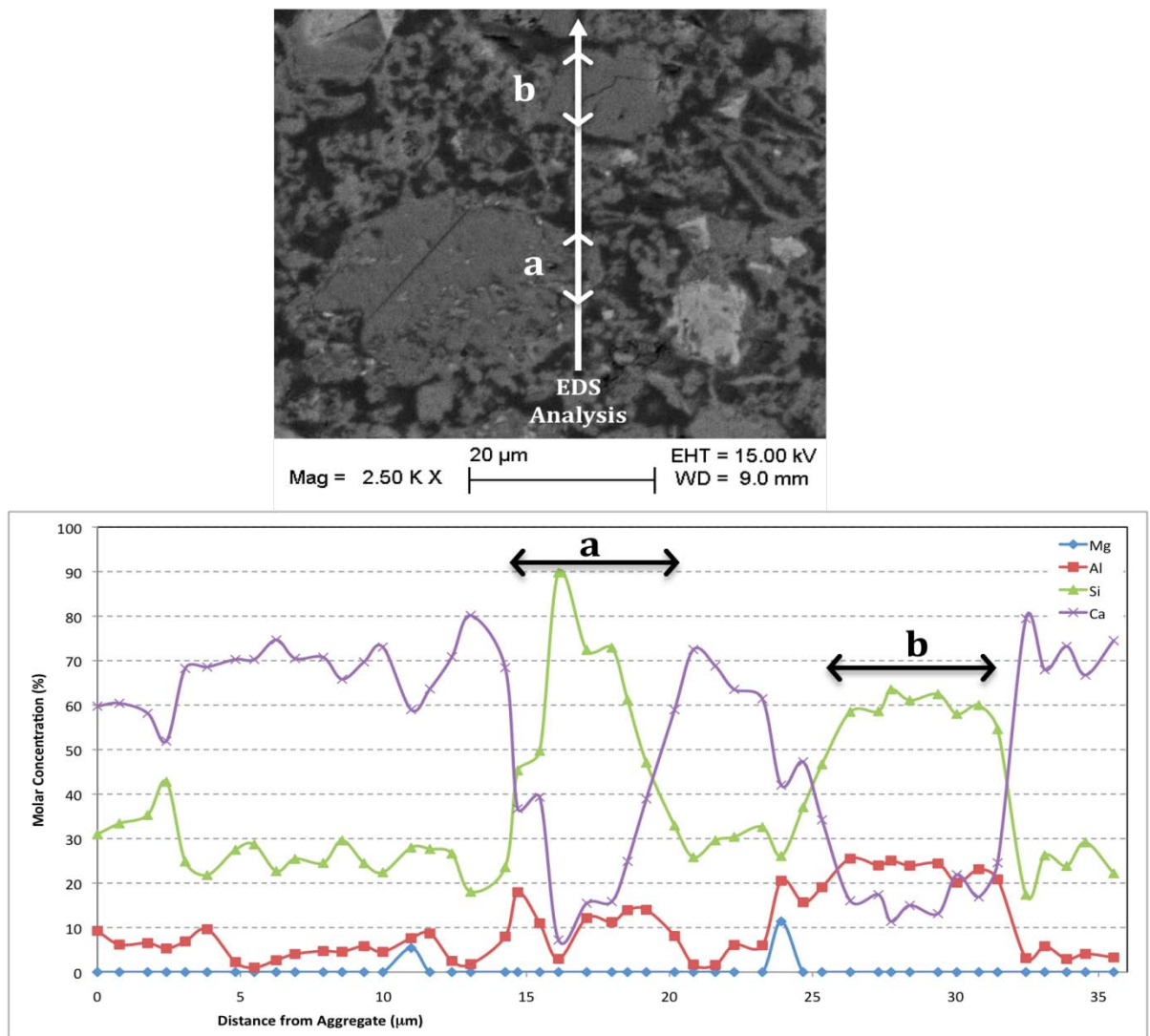
Figure 10.4.6: BSE Image and EDS Analysis of Quartz (a) and Feldspar (b).
