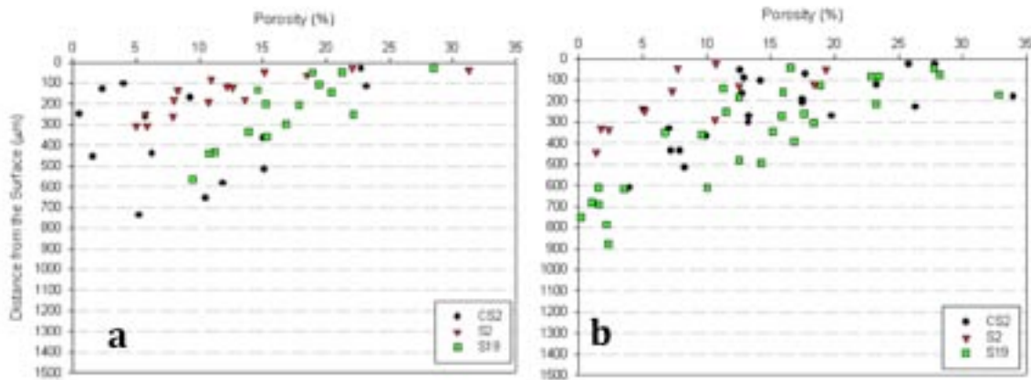
Figure 16: Porosity Profiles of Samples made with Microfines From Siliceous Aggregates Under Wet Curing Process (a) and Dry Curing Process (b).
