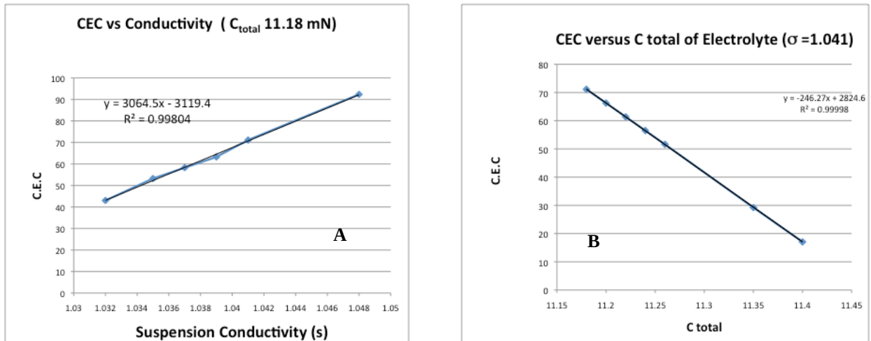
Figure 19: Sensitivity of the CEC Values to Changes in Either Conductivity or Initial Concentration of Electrolyte
