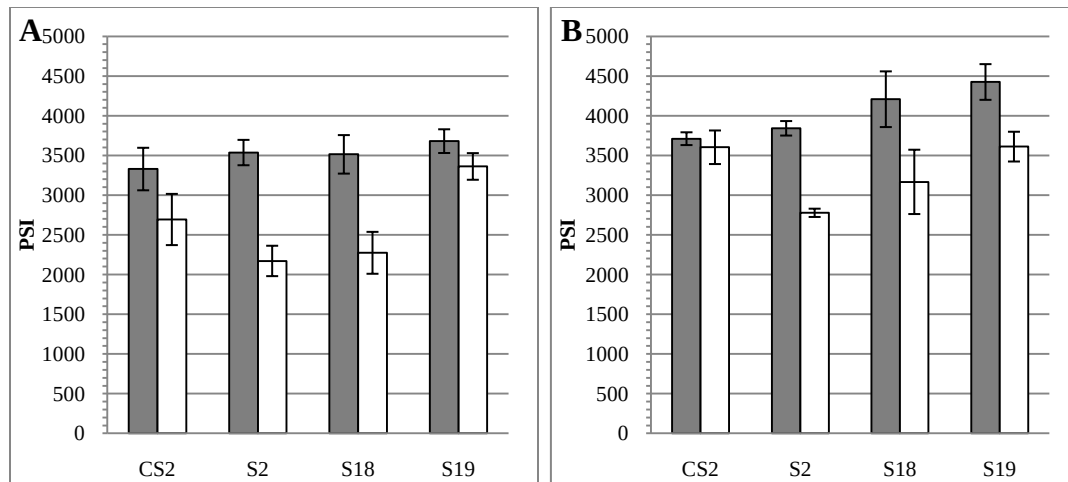
Figure 5: Values of Compressive Strength at 7 (A) and 28 (B) Days of Curing Under WC (Dark Grey Column) and DC (Light Column) for Concrete Batches of Group B
