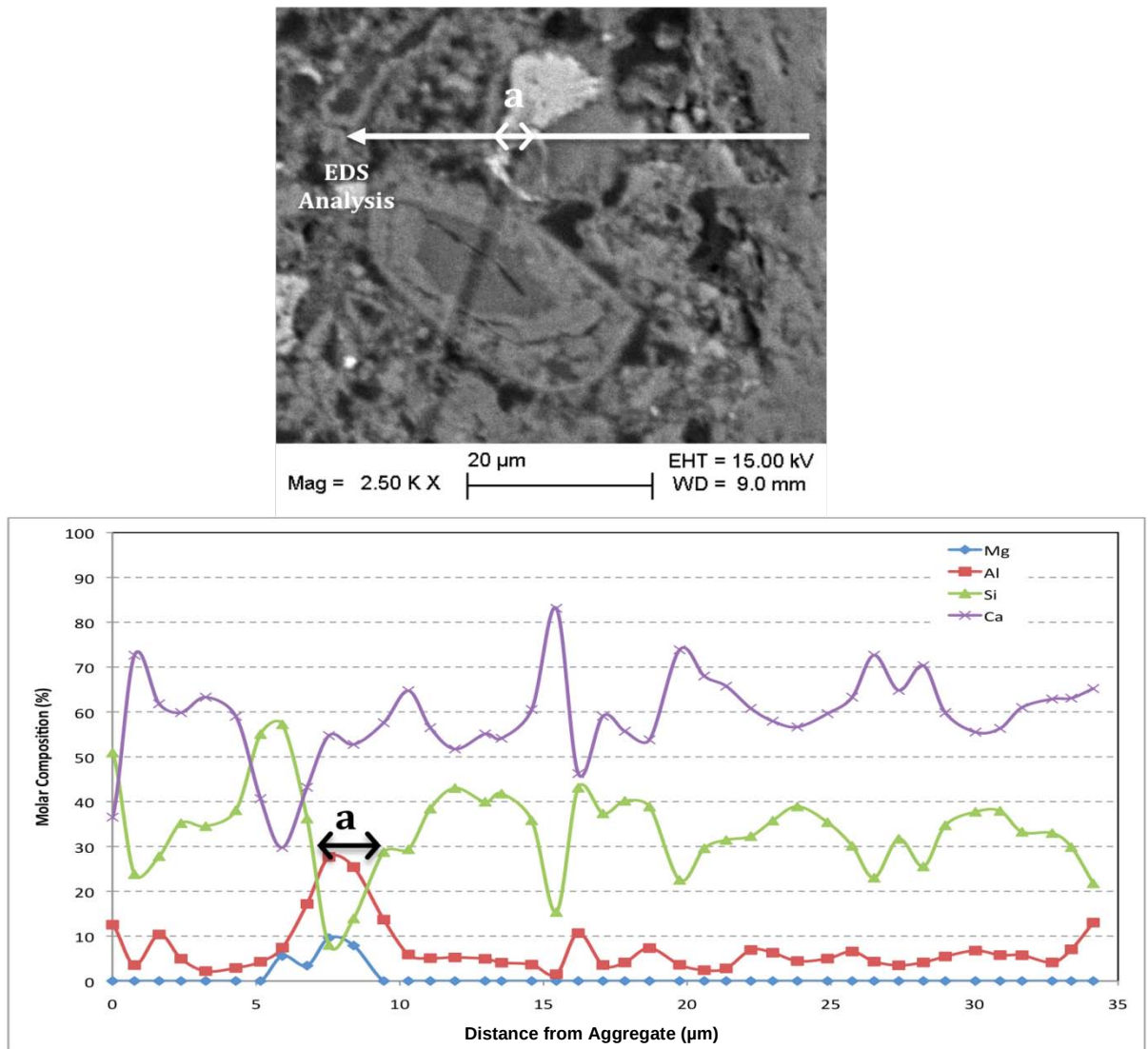
Figure 10.4.4: BSE Image and EDS Analysis of C4AFe (a).
