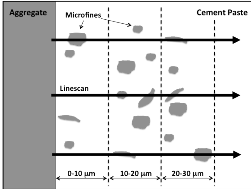
Figure 1: Schematic Representation of EDS Analysis
