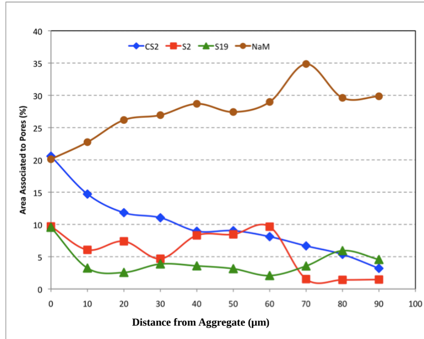
Figure 14: Average Distribution of Porosity in the Interfacial Transition Zone of Concrete Samples Made with Microfines From Siliceous Aggregates.
