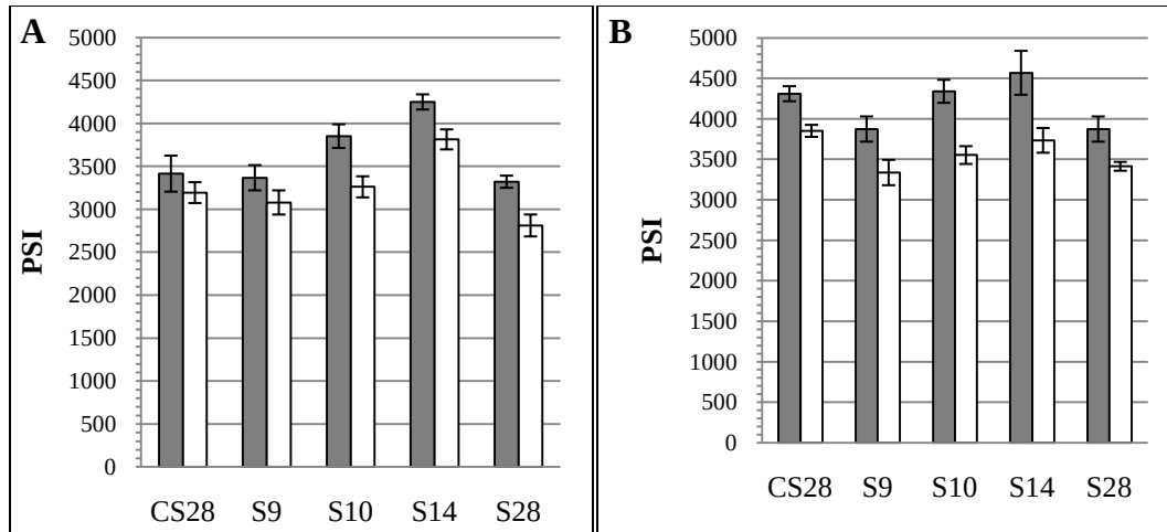
Figure 4: Values of Compressive Strength at 7 (A) and 28 (B) Days of Curing Under WC (Dark Grey Column) and DC (Light Column) for Concrete Batches of Group A
