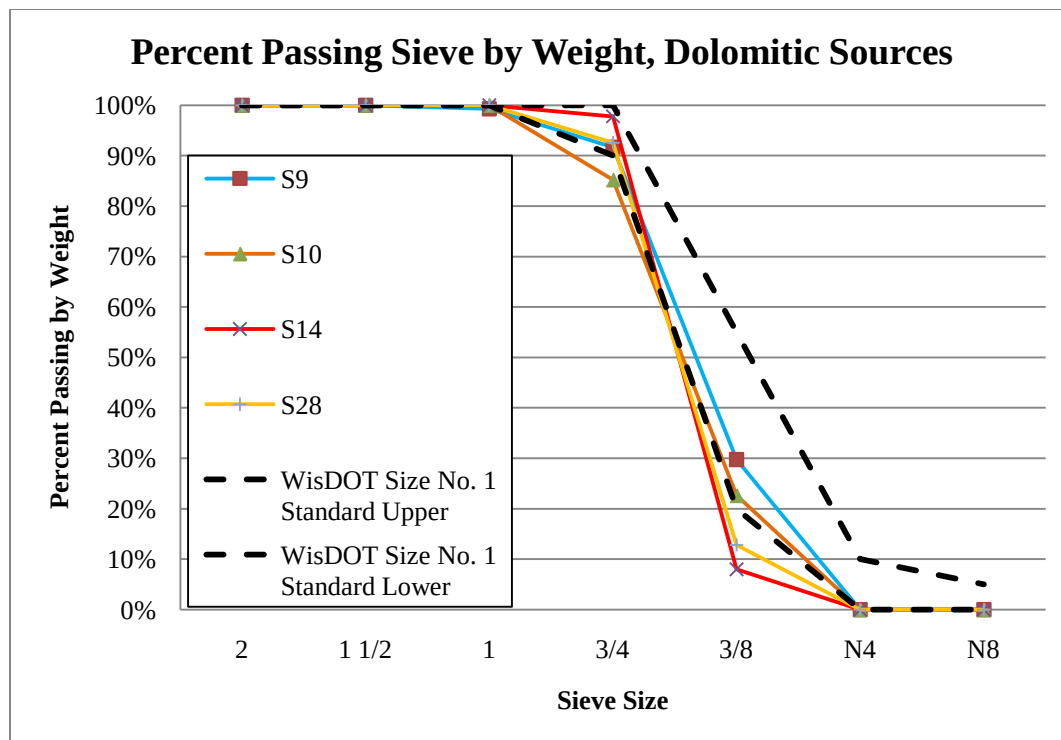
Figure 10.2.3: Sieve Analysis Results for Coarse Aggregates From Dolomitic Sources
