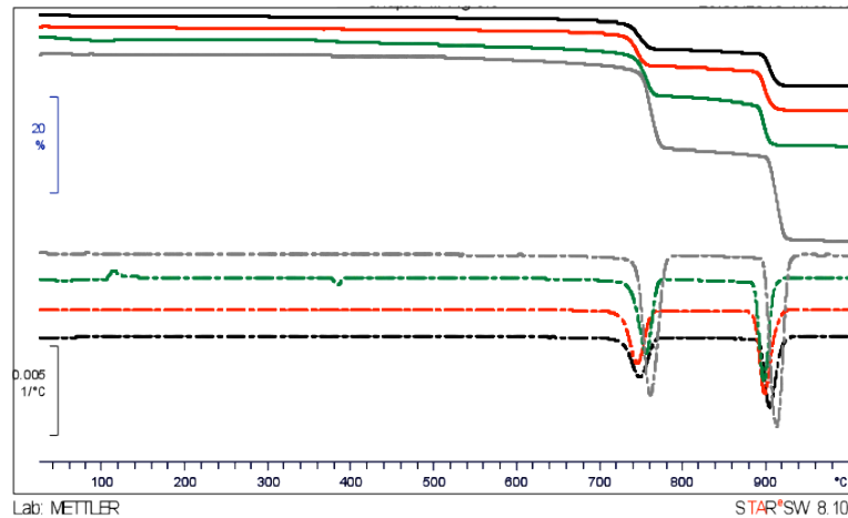
Figure 3: TG (Top) and DTG (Bottom) Curves for Group A Microfines: S28 (Grey), S9 (Green), S10 (Black), and S14 (Red)
