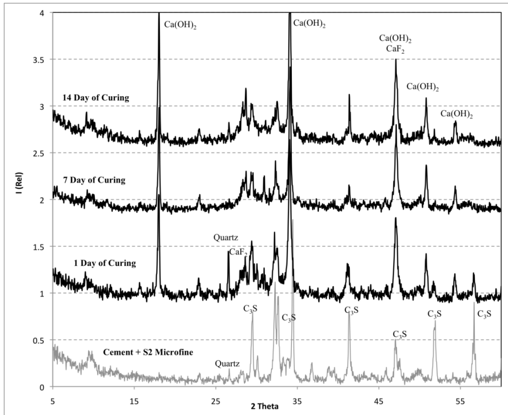
Figure 10.3.3: X-ray Diffraction Patterns of Cement Paste Containing a Siliceous Microfine (S2) at Different Aging Times
