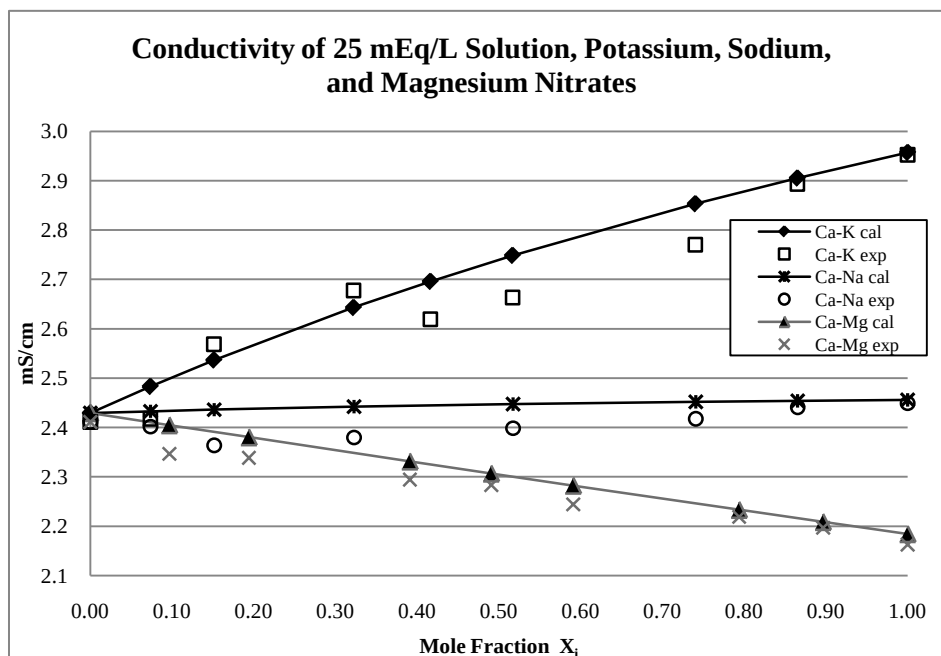
Figure 17: Comparison Between Calculated (full markers) and Measured Conductivity (empty markers) for Binary Electrolytes Solutions.
