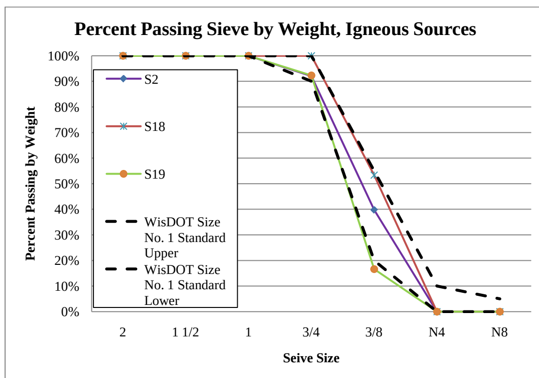
Figure 10.2.4: Sieve Analysis Results for Coarse Aggregates From Igneous Sources
