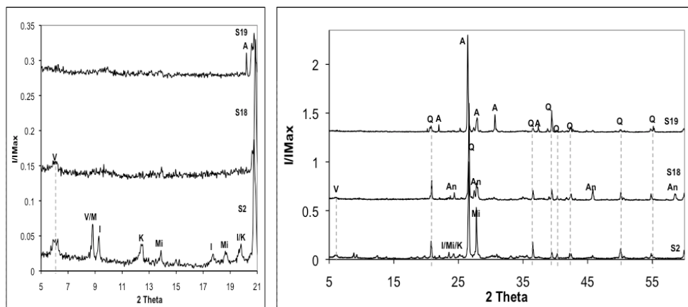
Figure 2: X-ray Diffractograms of the Group B of Microfine Samples. A: albite, An: anorthite, I: illite, K: kaolinite, M: muscovite, Mi: microcline, Q: quartz, and V: vermiculite
