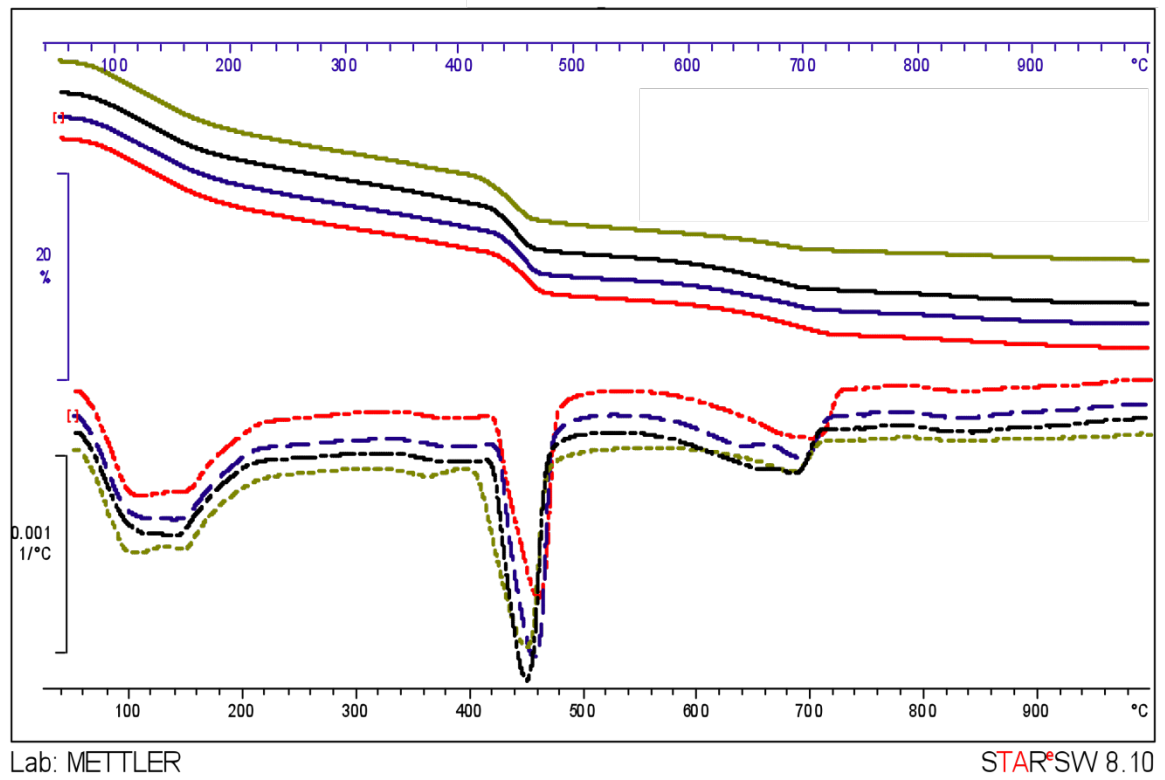
Figure 10.3.5: TG (Top) and DTA (Bottom) Curves for Cement Paste Samples Containing Kaolin (Green), S14 Microfines (Dark Blue), S2 Microfines (Red), and the Control (black).
