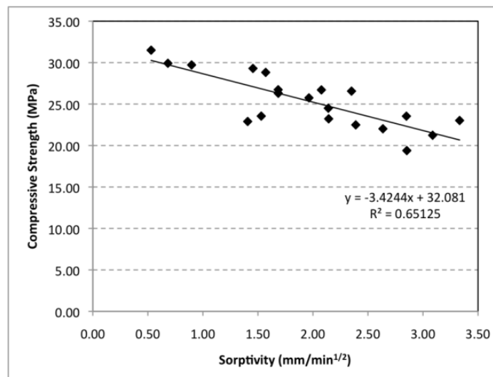
Figure 8: Correlation Between Sorptivity and Compressive Strength for the Entire Sample Population at 7 and 28 Days of Curing.
