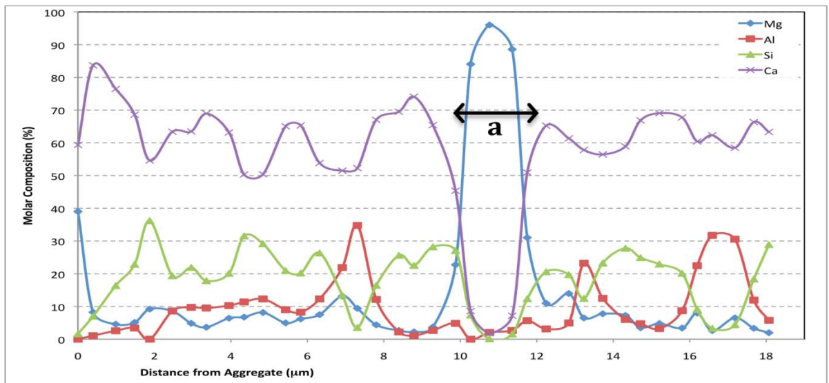
Figure 10.4.10: BSE Image and EDS Analysis of Brucite (a).
