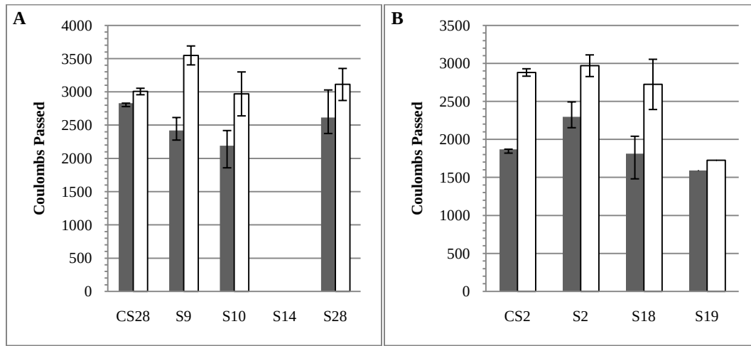
Figure 11: Rapid Chloride Penetration Test Results at 7 (A) and 28 (B) Days. Wet Cured Samples in Gray and Dry Cured Samples in White.
