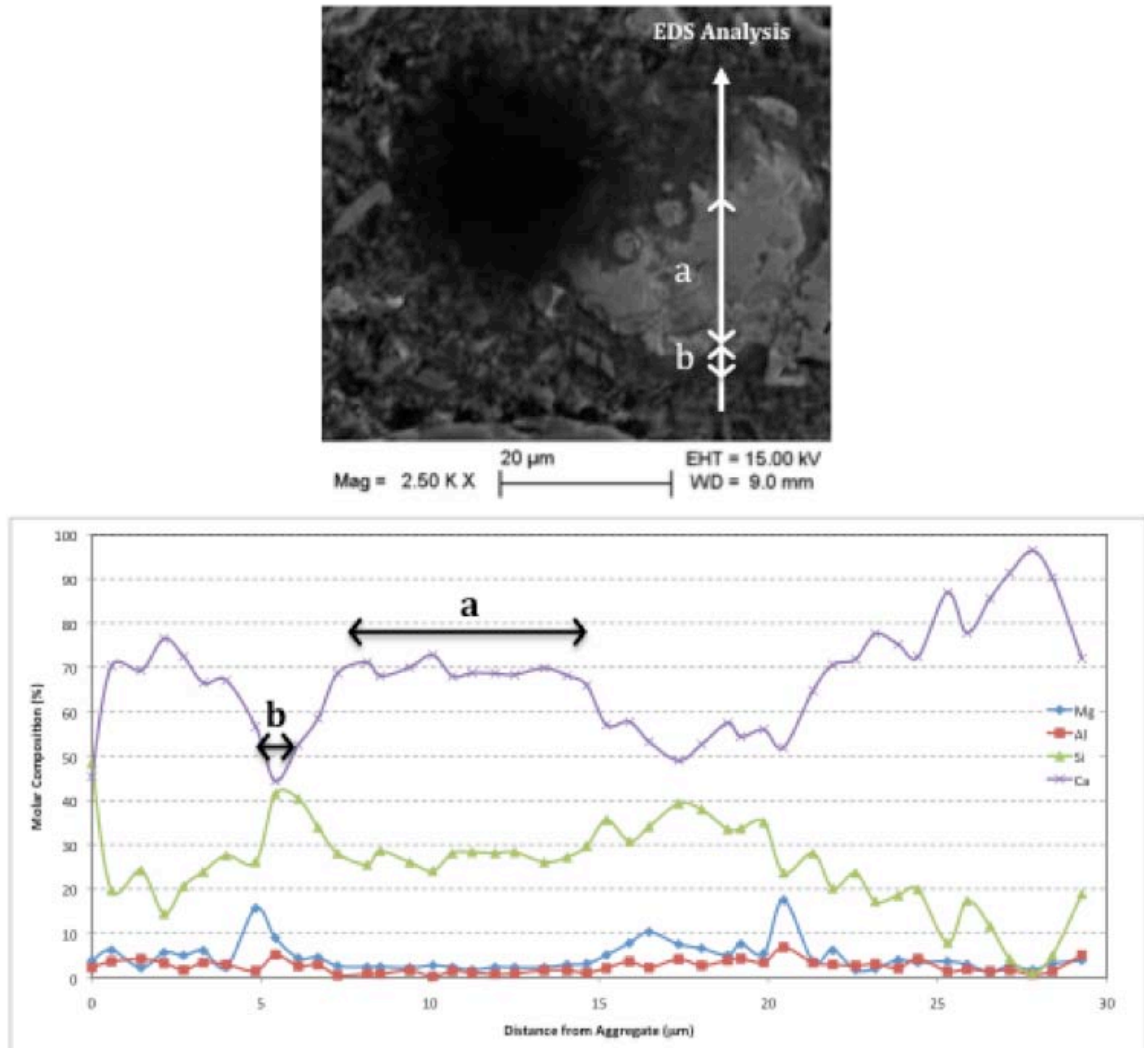
Figure 10.4.1: BSE Image and EDS Analysis of C3S (a) and C-S-H (b).
