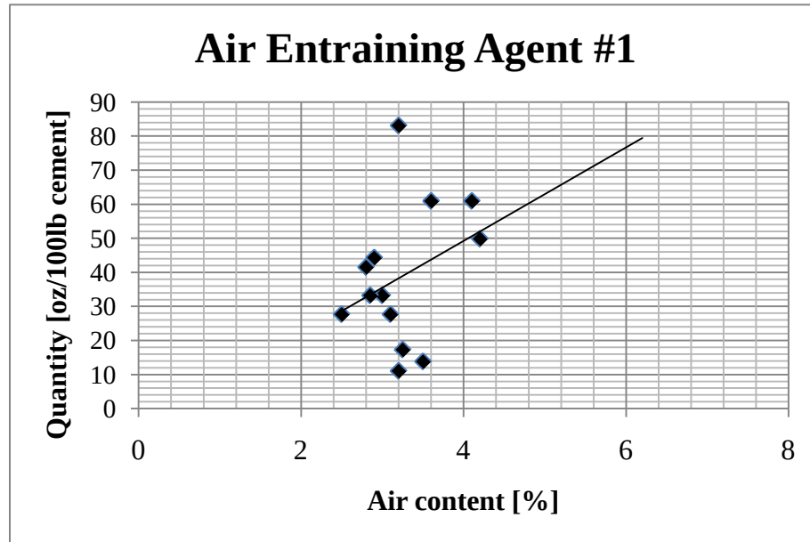
Figure 20: Effectiveness of An Air Entraining Agent (AEA) in a Concrete Mixture Containing 5 Percent Microfines by Coarse Aggregate Weight (Aggregates from Wisconsin and Microfines from Wyoming). The Recommended AEA dosage was 1 to 3 fl. oz. per 100 lbs of Cement.
