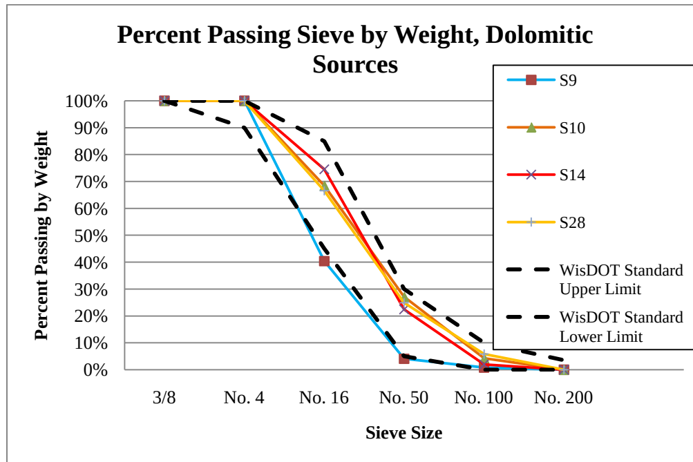
Figure 10.2.1: Sieve Analysis Results for Fine Aggregates From Dolomitic Sources
