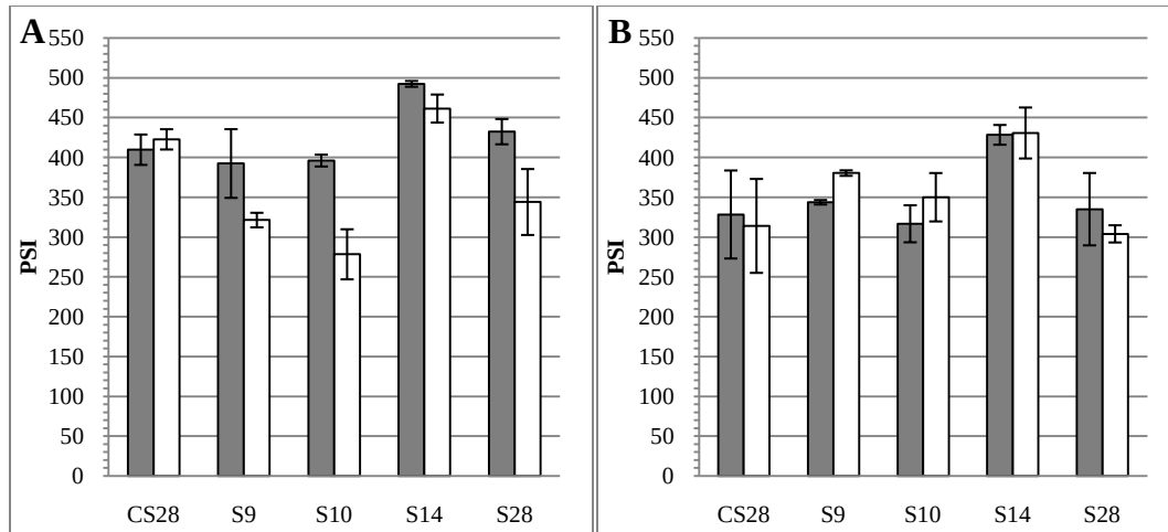
Figure 6: Values of Tensile Strength at 7 (A) and 28 (B) Days of Curing Under WC (Dark Grey Column) and DC (Light Column) for Concrete Batches of Group A
