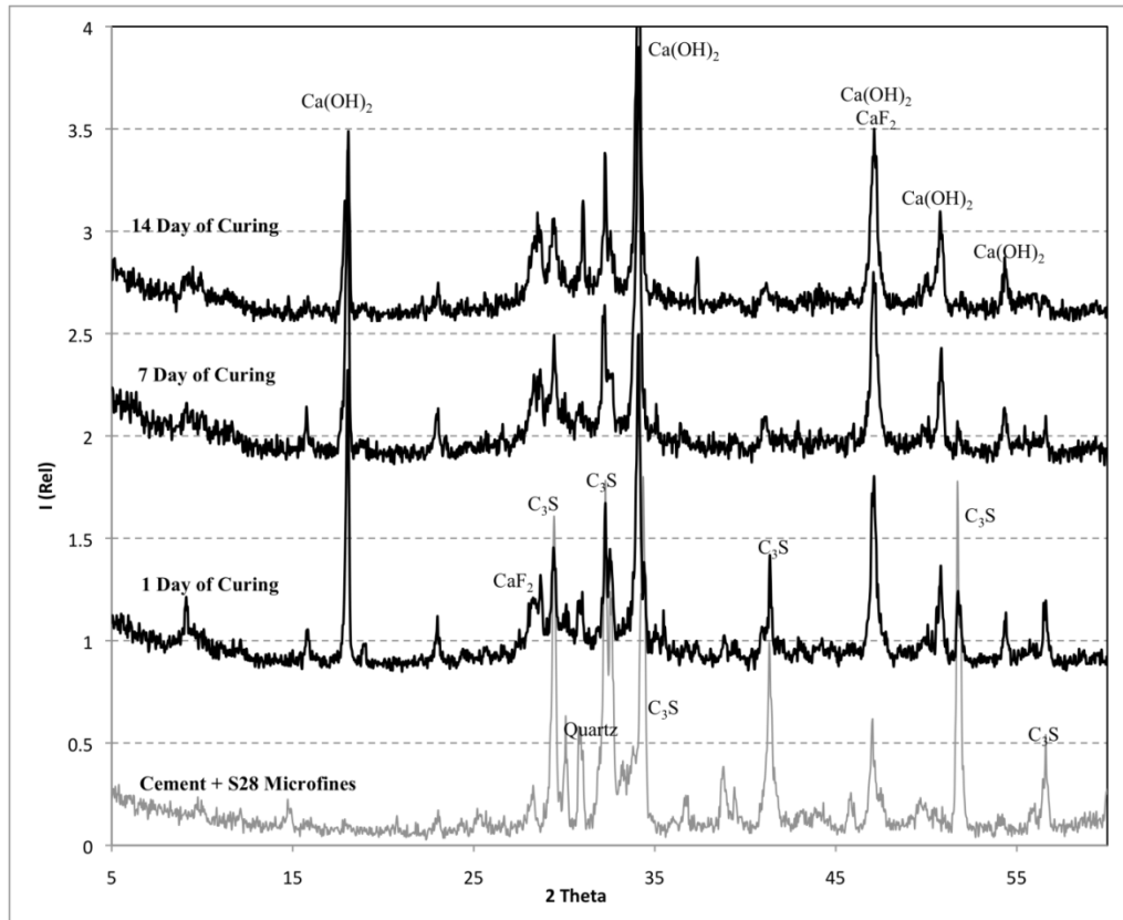
Figure 10.3.2: X-ray Diffraction Patterns of Cement Paste Containing a Carbonate Microfine (S28) at Different Aging Times.
