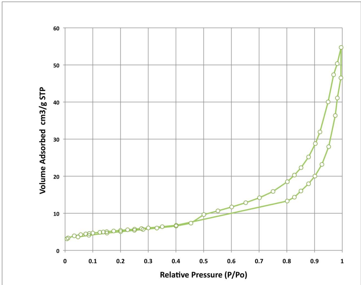
Figure 10.3.6: Adsorption / Desorption Isotherm for the Cement Paste Control.
