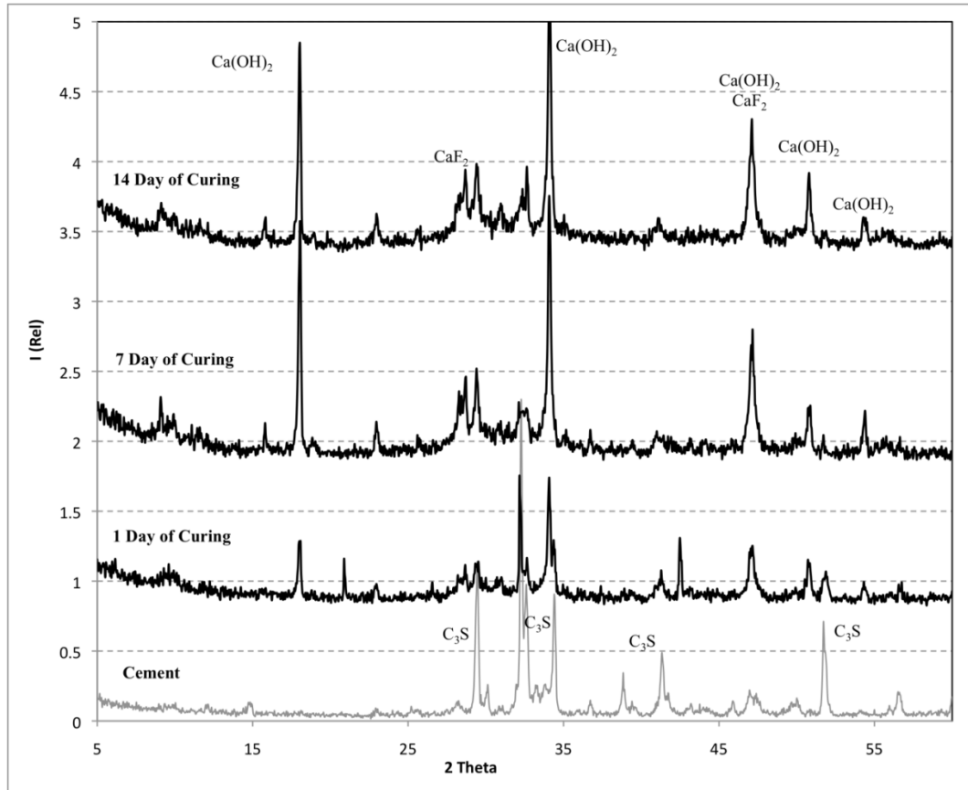
Figure 10.3.1: X-ray Diffraction Patterns for the Cement Paste Control at Different Aging Times.
