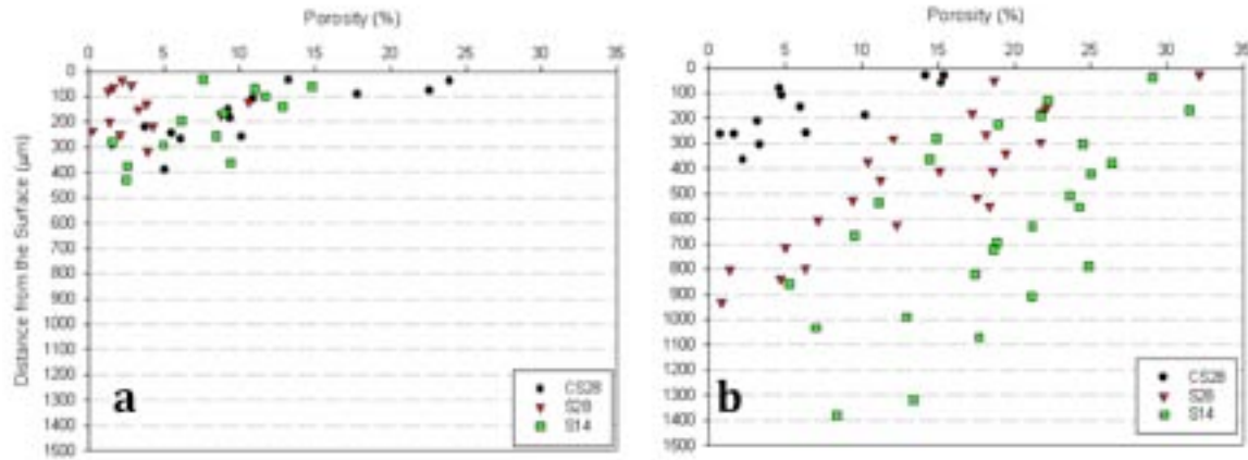
Figure 15: Porosity Profiles of Samples Made with Microfines From Dolomitic Limestone Aggregates Under Wet Curing Process (a) and Dry Curing Process (b).
