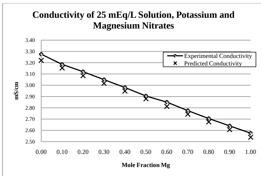
Figure 18: Comparison Between Calculated (full markers) and Measured Conductivity (empty markers) for a K-Mg Binary Electrolyte Solution
