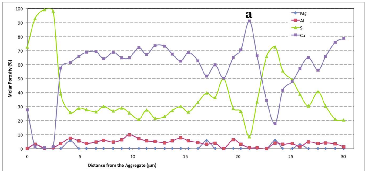
Figure 10.4.5: BSE Image and EDS Analysis of \text{Ca}(\text{OH})_2 (a).
