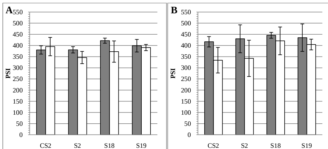
Figure 7: Values of Tensile Strength at 7 (A) and 28 (B) Days of Curing Under WC (Dark Grey Column) and DC (Light Column) for Concrete Batches of Group B
