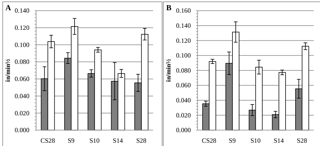
Figure 9: Sorptivity Values for WC (A) and DC (B) Concrete Specimens Made with Microfines from Group A at 7 Days (Gray Column) and 28 Days (White Column) of Curing
