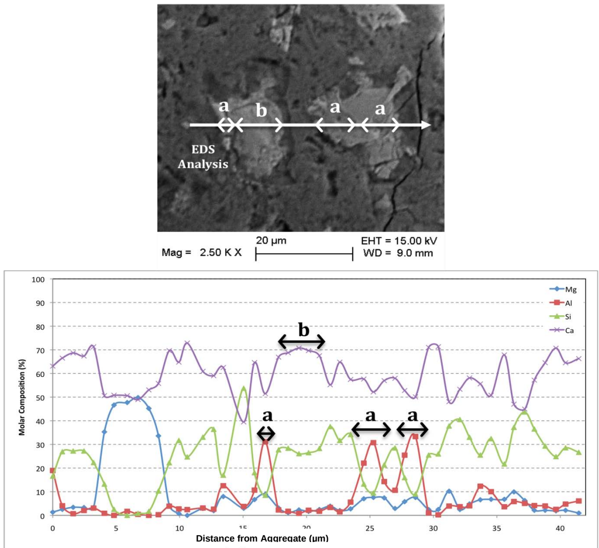
Figure 10.4.3: BSE Image and EDS Analysis of C3A (a) and C3S (b).
