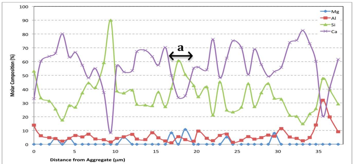
Figure 10.4.8: BSE Image and EDS Analysis of Calcium Silicate (a).
