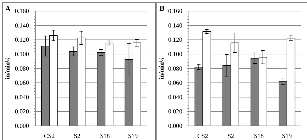
Figure 10: Sorptivity Values for WC (A) and DC (B) Concrete Specimens Made with Microfines from Group B at 7 Days (Gray Column) and 28 Days (White Column) of Curing
