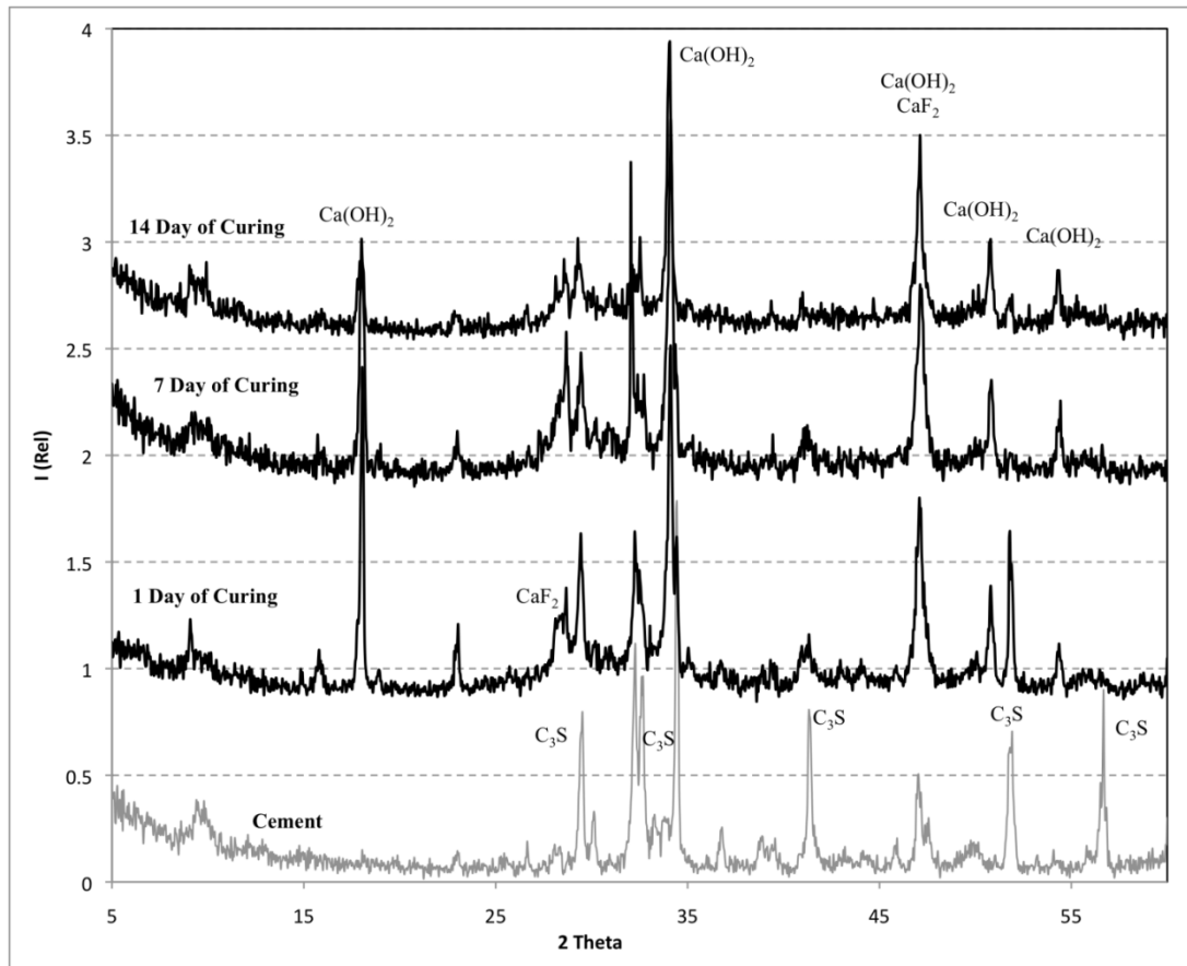
Figure 10.3.4: X-ray Diffraction Patterns for the Cement Paste Containing Microfines of CaM at Different Aging Times.
