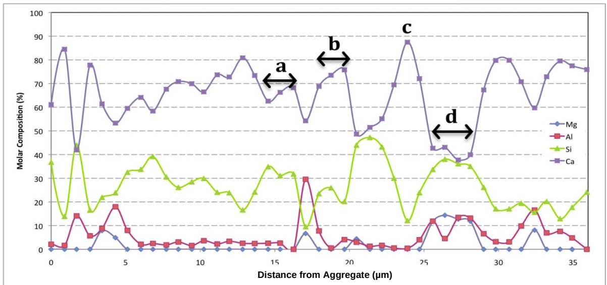
Figure 10.4.2: BSE Image and EDS Analysis of C2S (a), C3S (b), Pore Rich in \text{Ca(OH)}_2 (c), and Dolomite (d).
