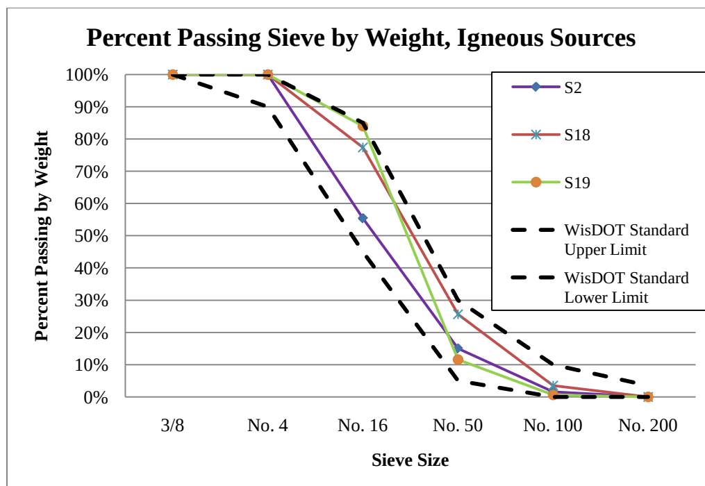
Figure 10.2.2: Sieve Analysis Results for Fine Aggregates From Igneous Sources
