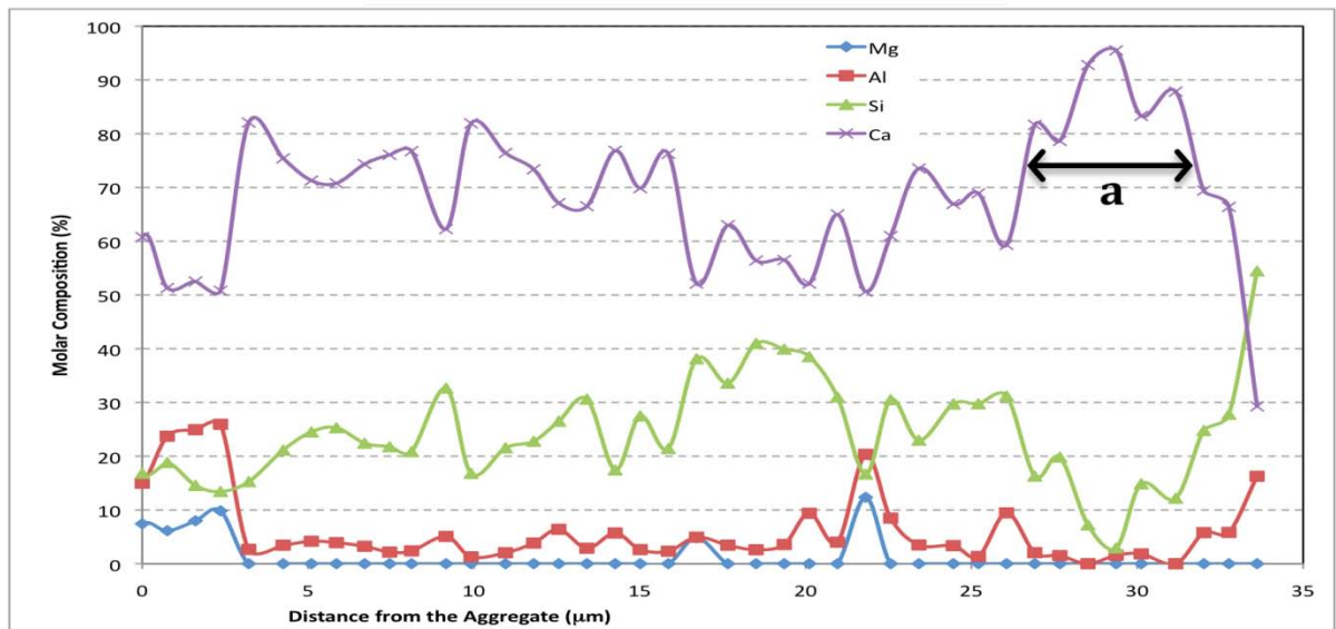
Figure 10.4.7: BSE Image and EDS Analysis of Calcite (a).
