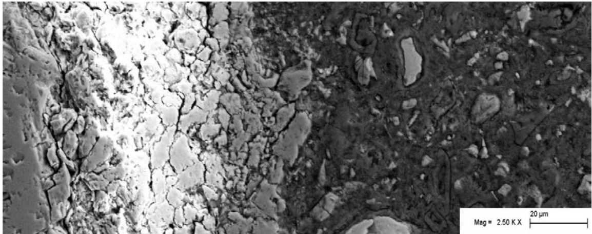
Figure 10.5.1: BSE Image of a Sodium Montmorillonite Coating Over a Coarse Aggregate.
