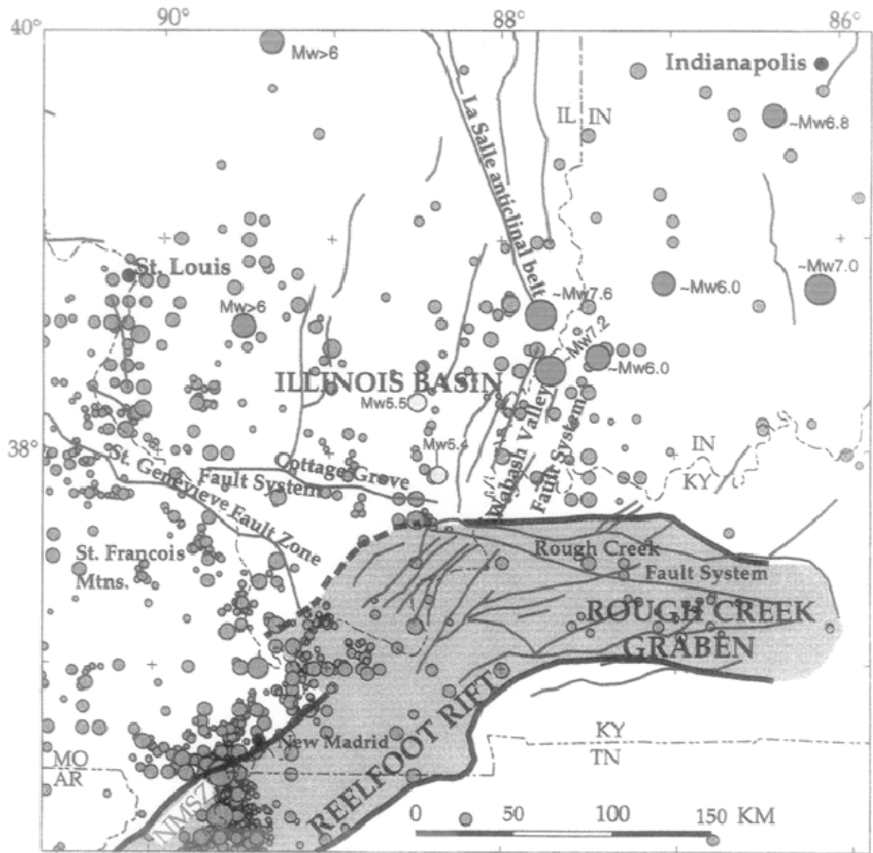
Figure 4-14. The Rough Creek Graben.
