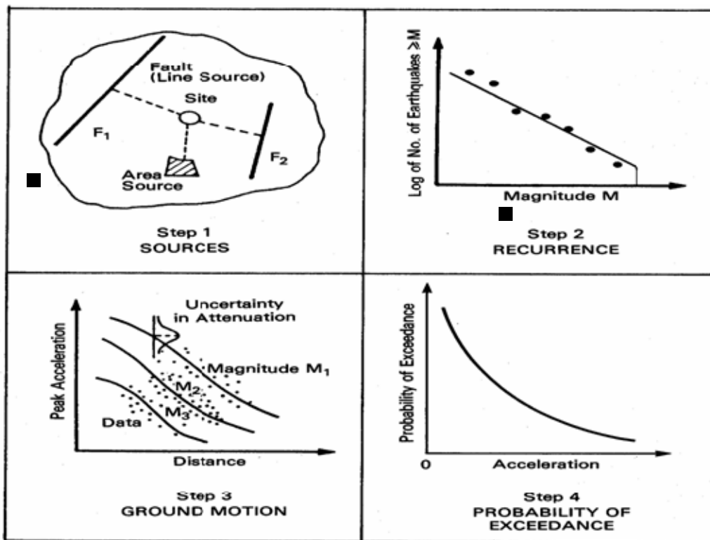
Figure 3-2. Steps involved in PSHA (Reiter, 1990).
