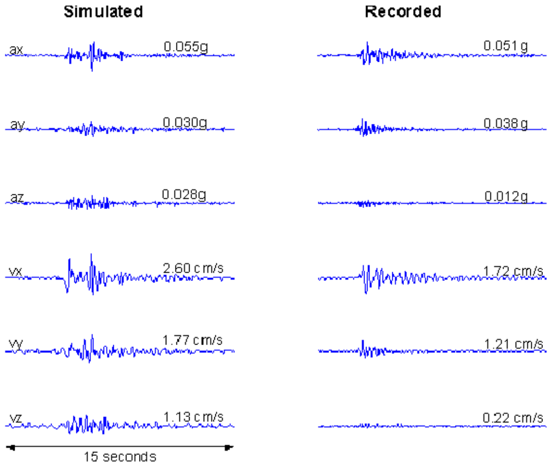
Figure 6-4. Comparison of observed and synthetic ground motion at Newburgh Lock and Dam. Observed acceleration and velocity are in the right column. The horizontal components a_x and a_y refer to instrument orientations, and the vertical component is denoted by a_z .
