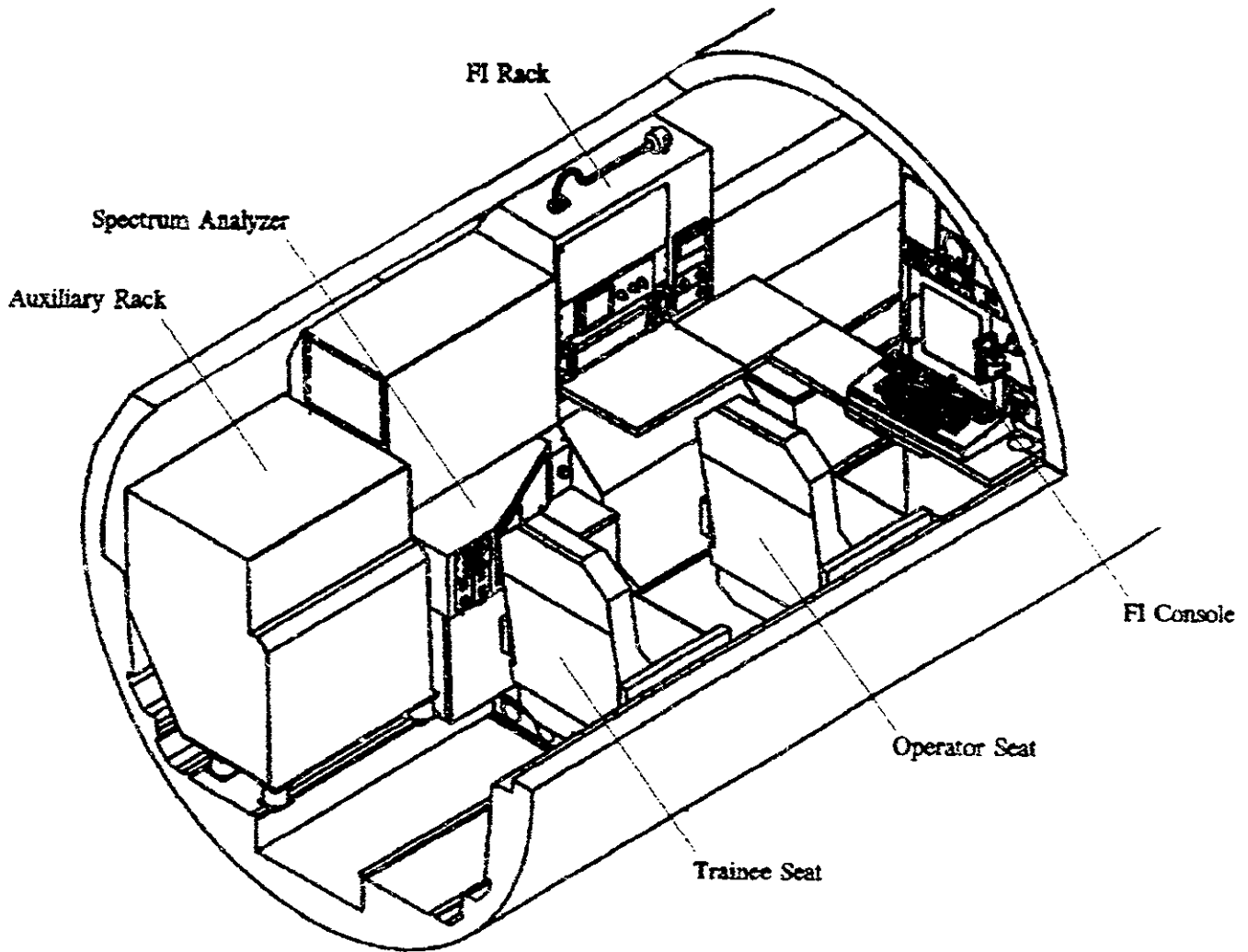
FIGURE 9 Proposed Workstation Layout
