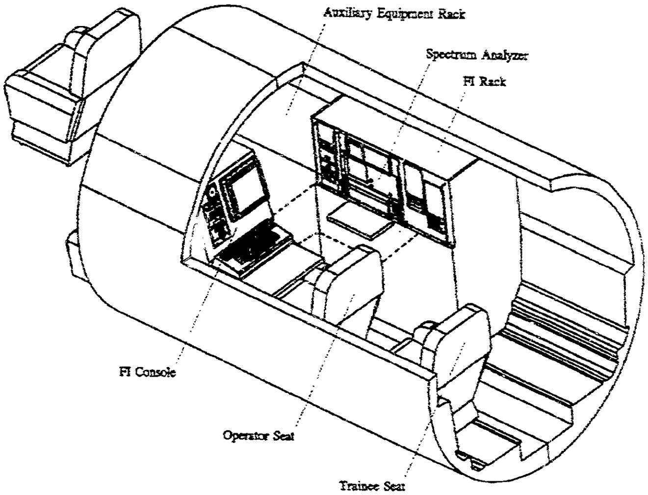
FIGURE 11 Accepted Workstation Layout
