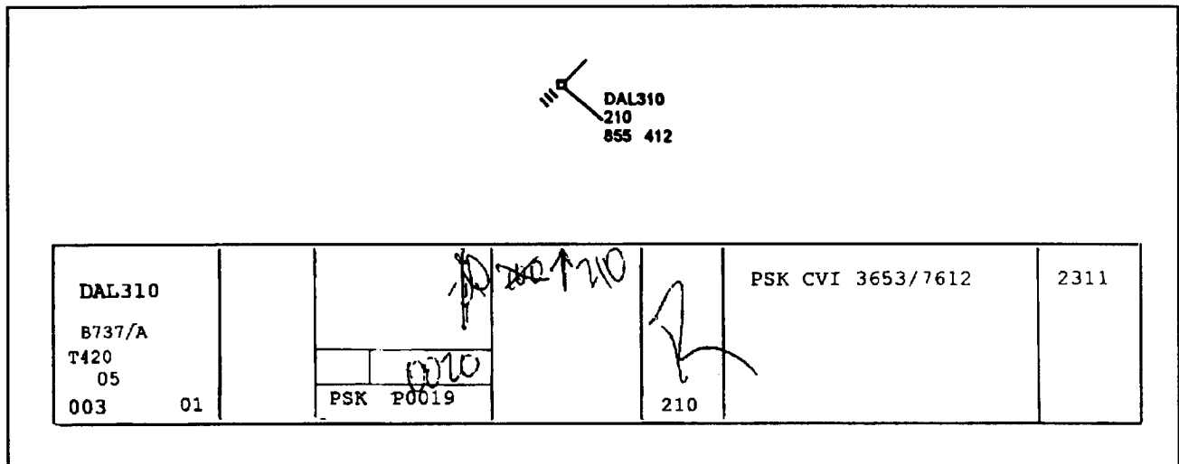
Figure 1. An aircraft's representation on the PVD and on a Flight Progress Strip.
