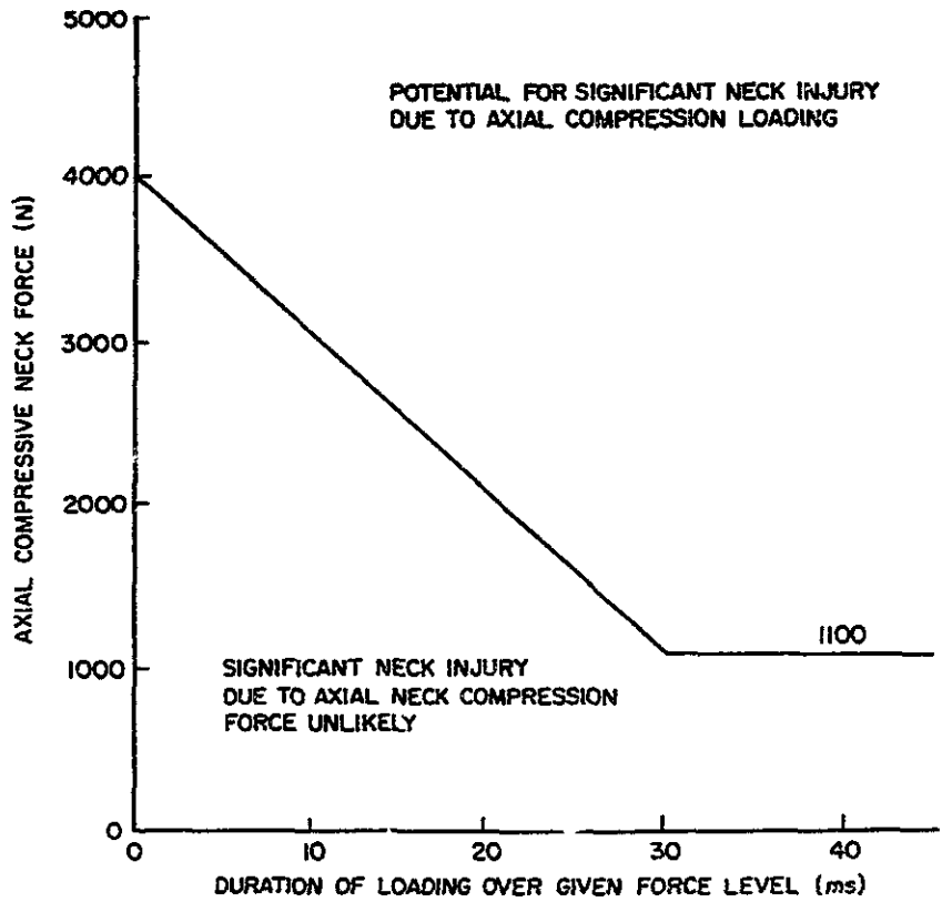
Figure 1 - Injury criterion for neck axial compressive loading (Mertz, et al., 1978)
